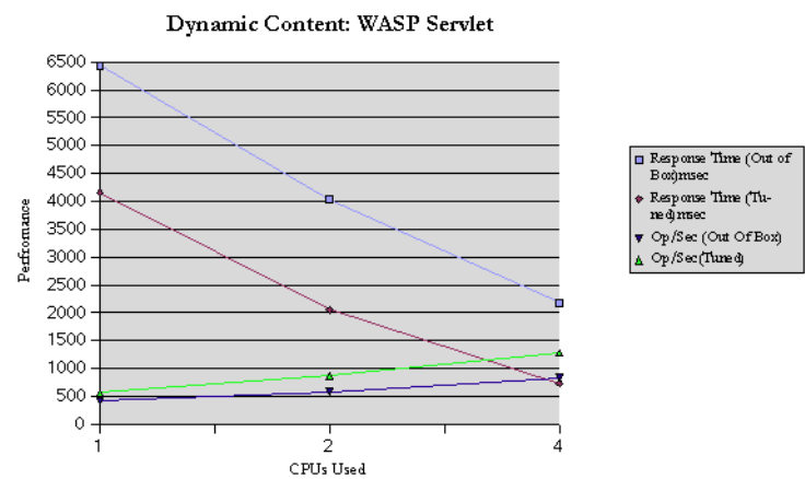
FIGURE 7-2 Dynamic Content Test: WASP Servlet
