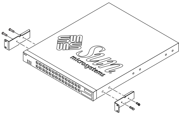
Figure 1 Removing the Rackmount Brackets
