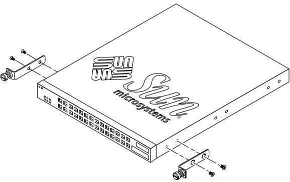
Figure 2 Installing the Thumbscrew Rack Brackets
