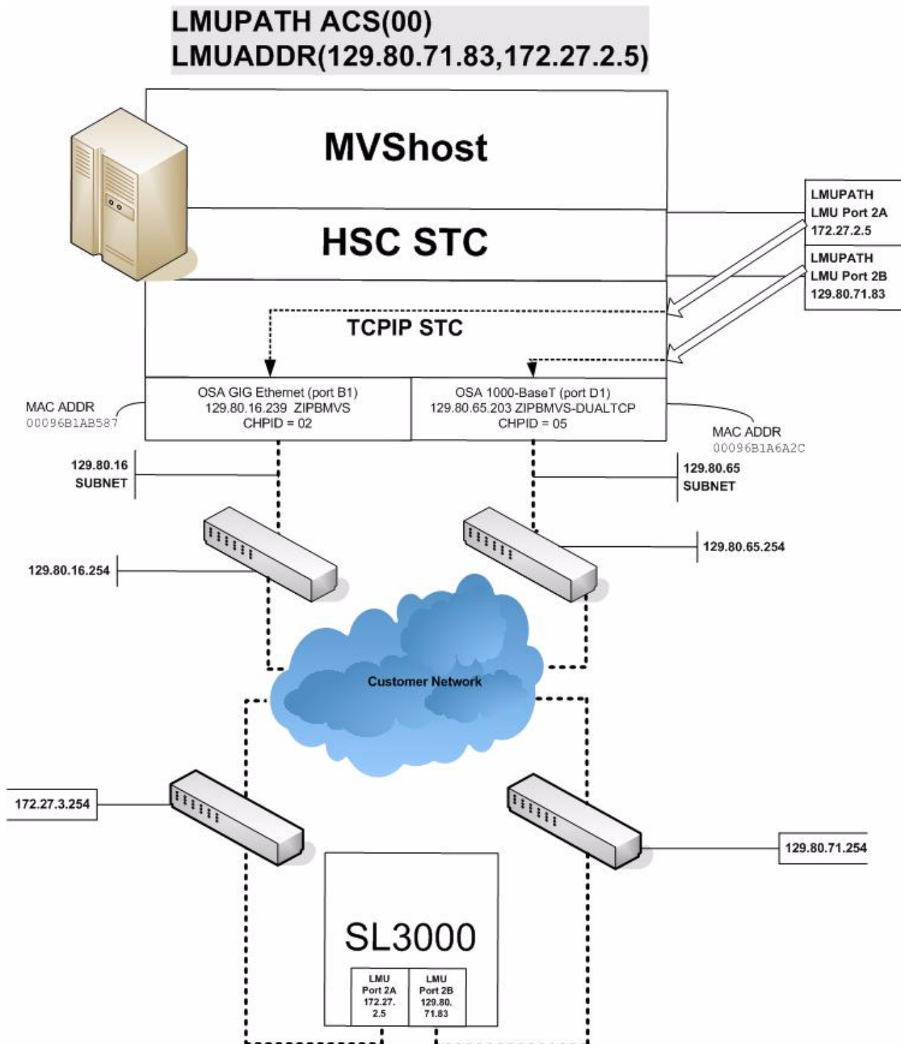
Figure 45. Dual IP Configuration Sample - Different Subnetworks
