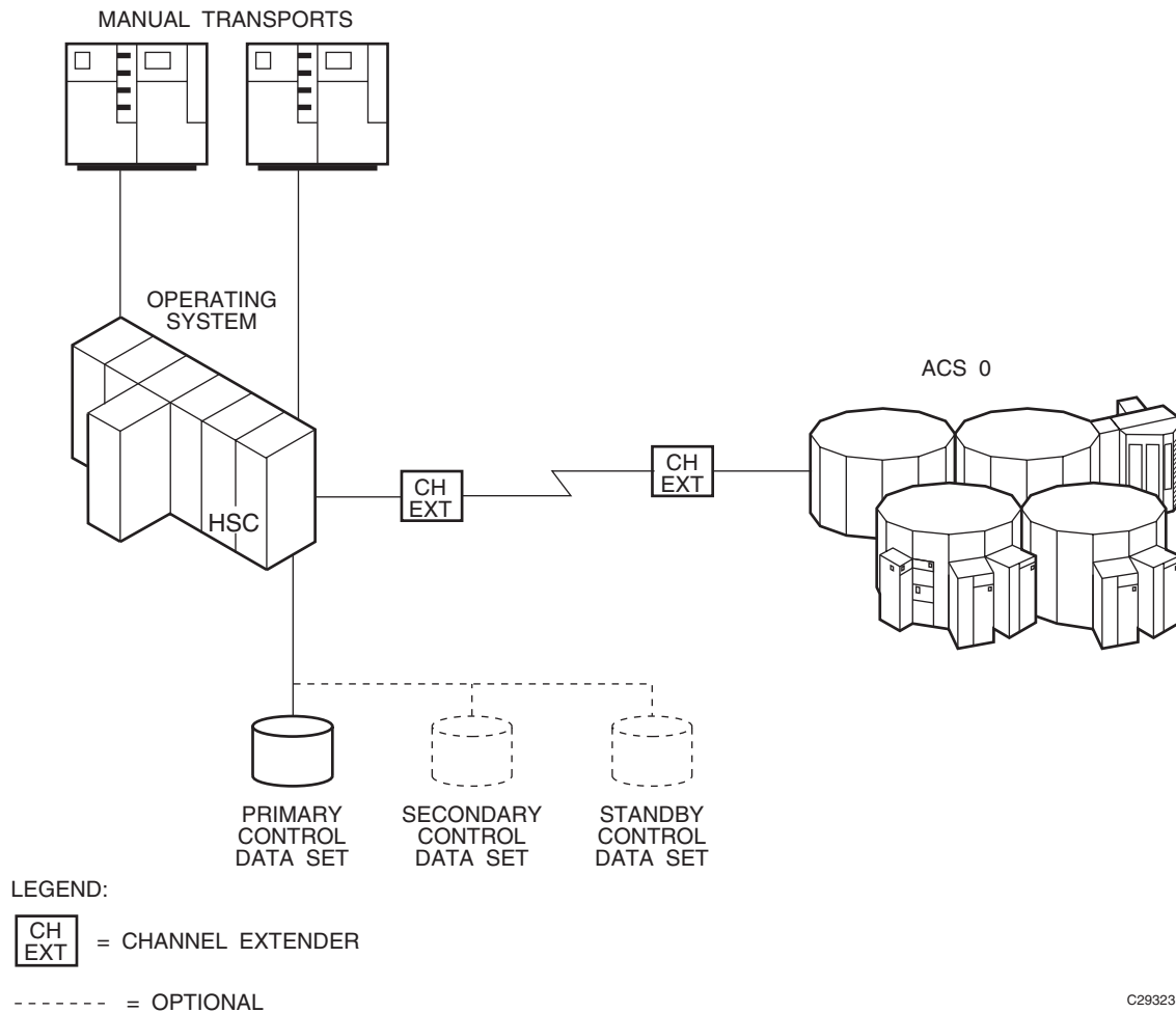
Figure 65. Configuration 1
