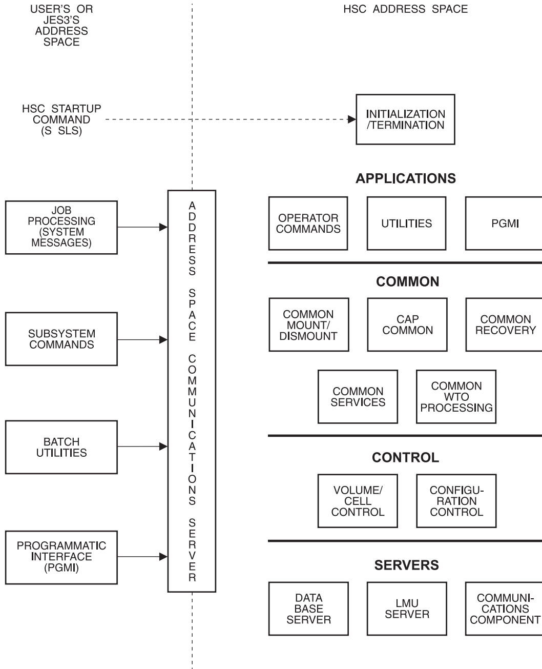
Figure 1. HSC Architecture
