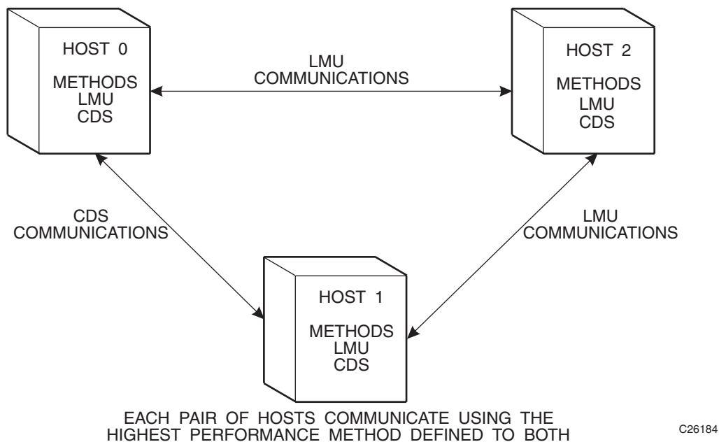
Figure 8. HSC Communication Methods Between Multiple Hosts
