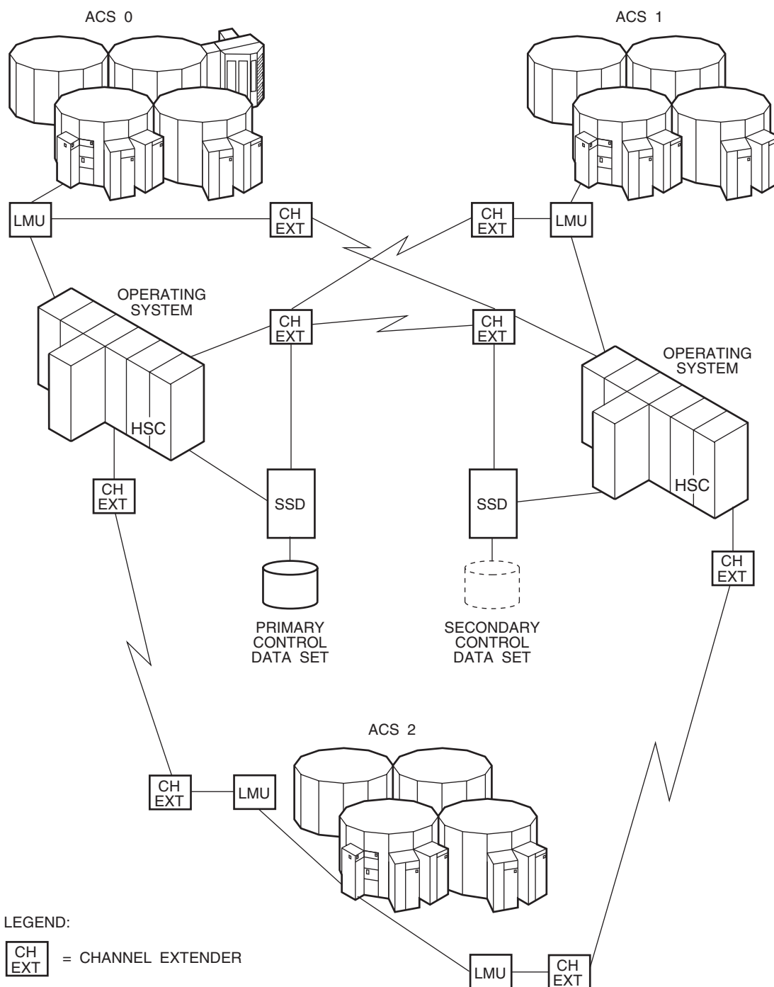
Figure 68. Configuration 5
