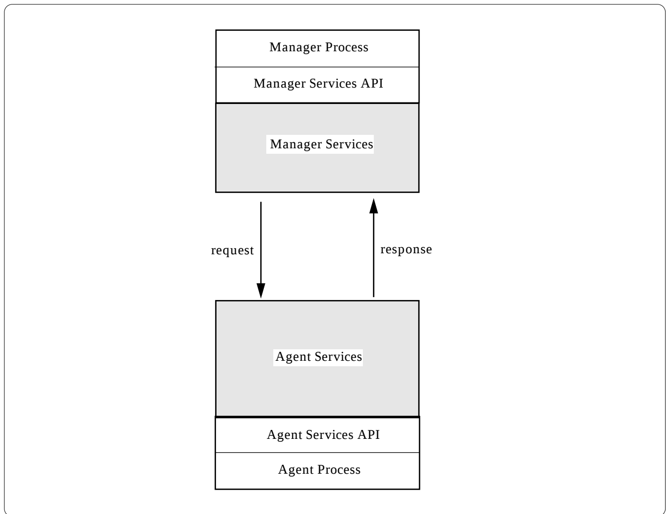
Figure 1-1 Manager/Agent Model
