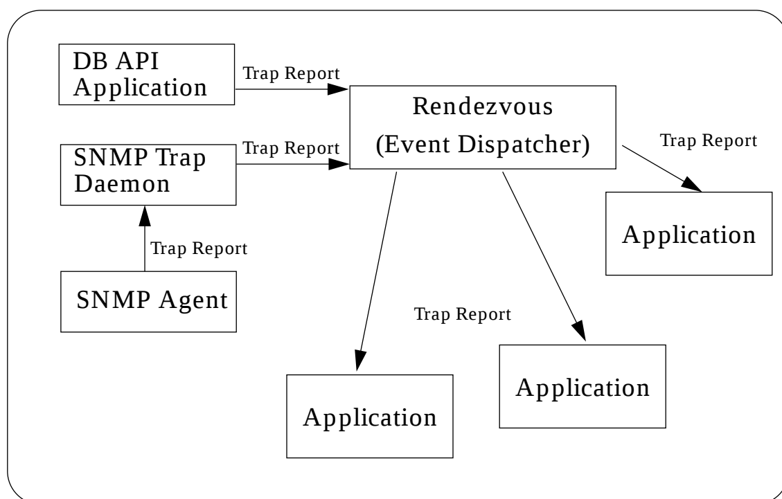
Figure 2-3 Trap Reporting
