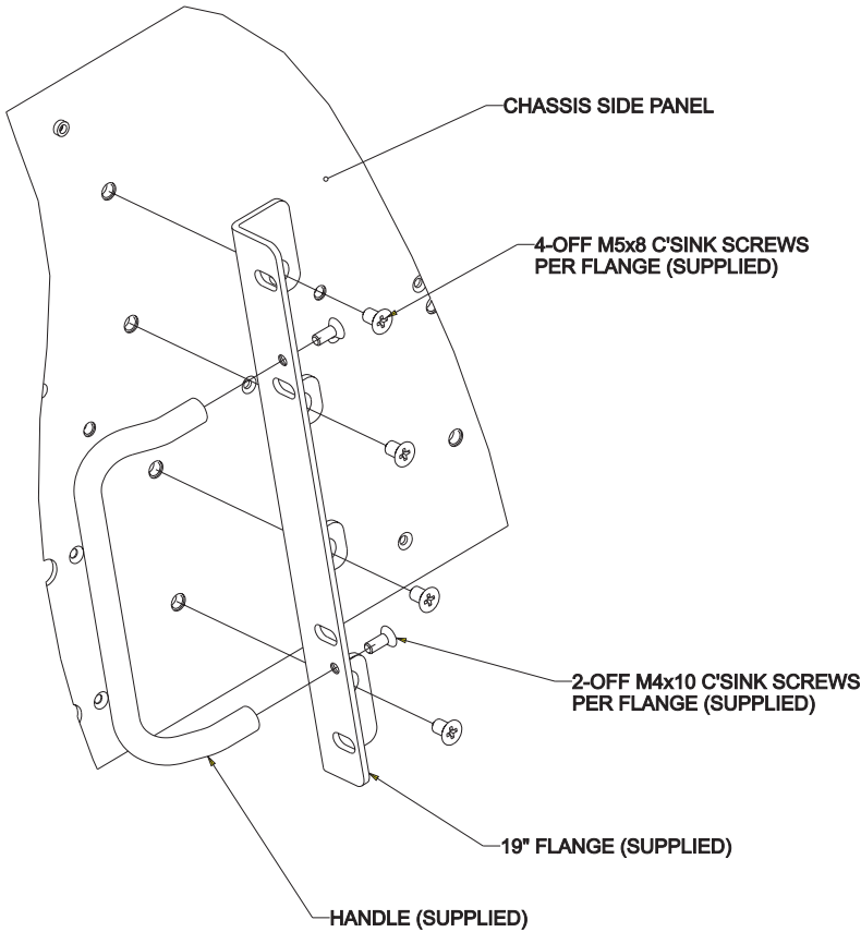
FIGURE 1 Flange Mount Assembly
