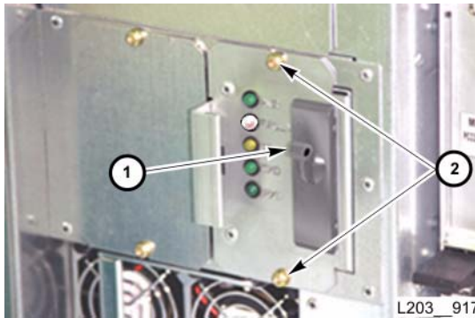
HBS Assembly
