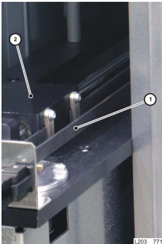
PTP mechanism removed for clarity. Shown with actuator (2) in fully retracted position.
