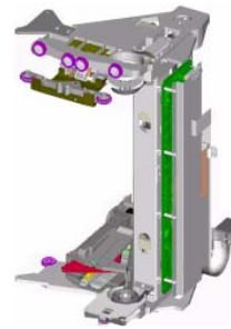
HandBot Assembly
