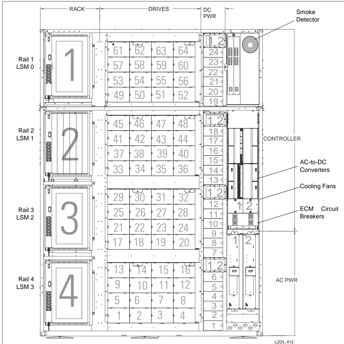
Figure 34. Drive and Electronics Module Planning
