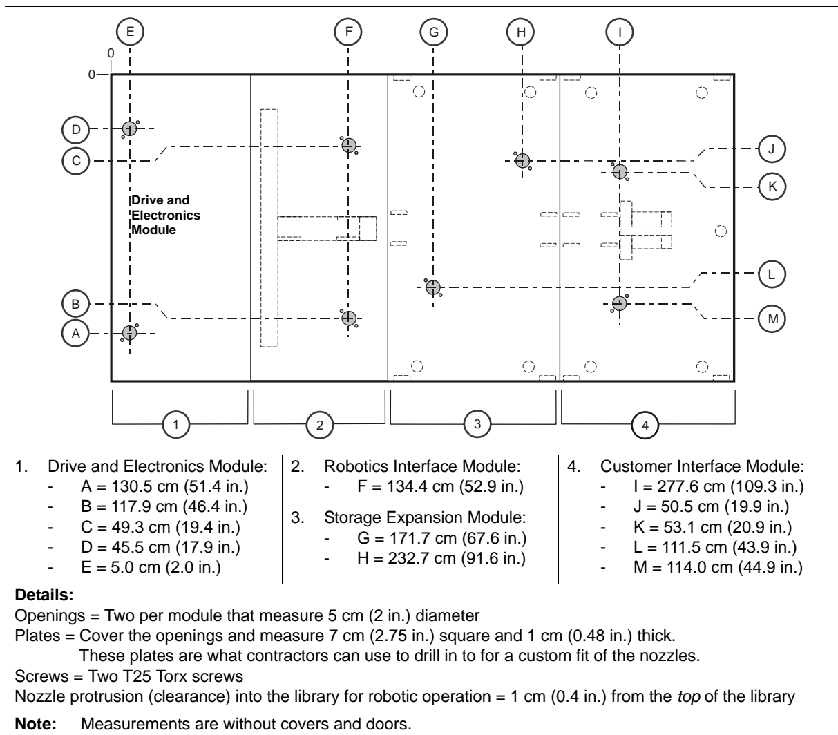
Figure 38. Fire Suppression Ceiling Access (Viewed from the top of the library)
