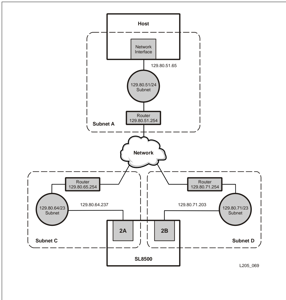
Figure 15. Single Interface Host and Multi-Homed SL8500
