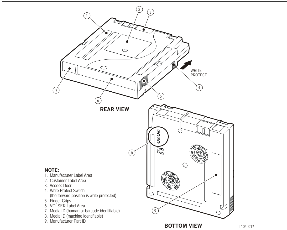
Figure 3. 9840 Tape Cartridge
