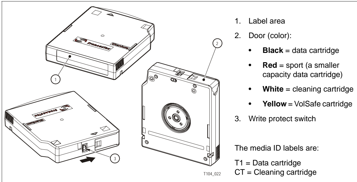
Figure 5. Tape Cartridge Types
