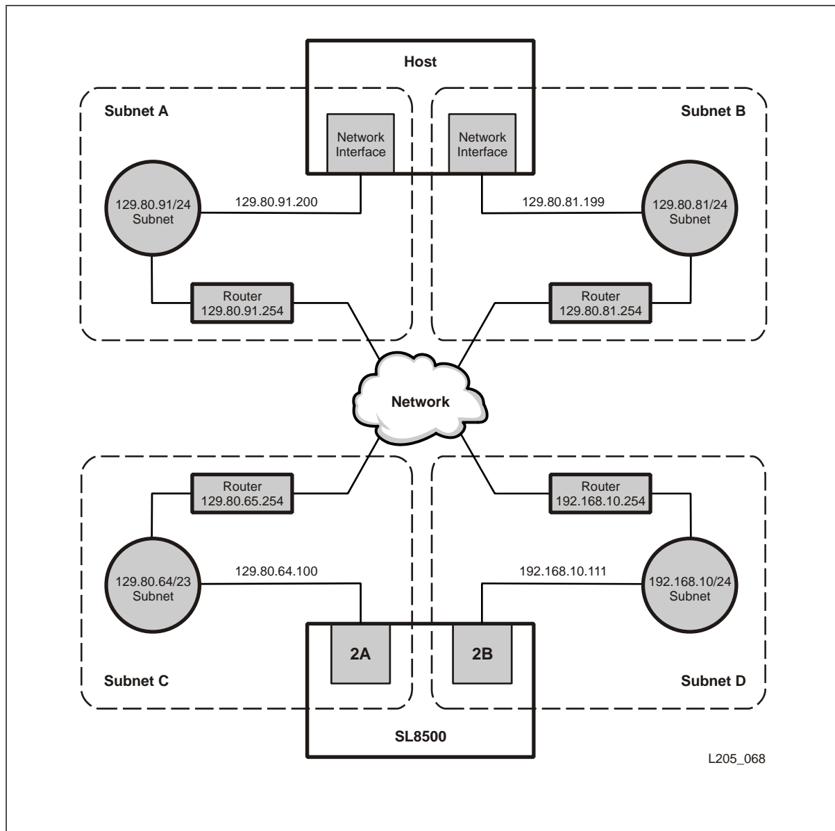
Figure 14. Multi-Homed Host, Multi-Homed SL8500, Interfaces on Different Subnets
