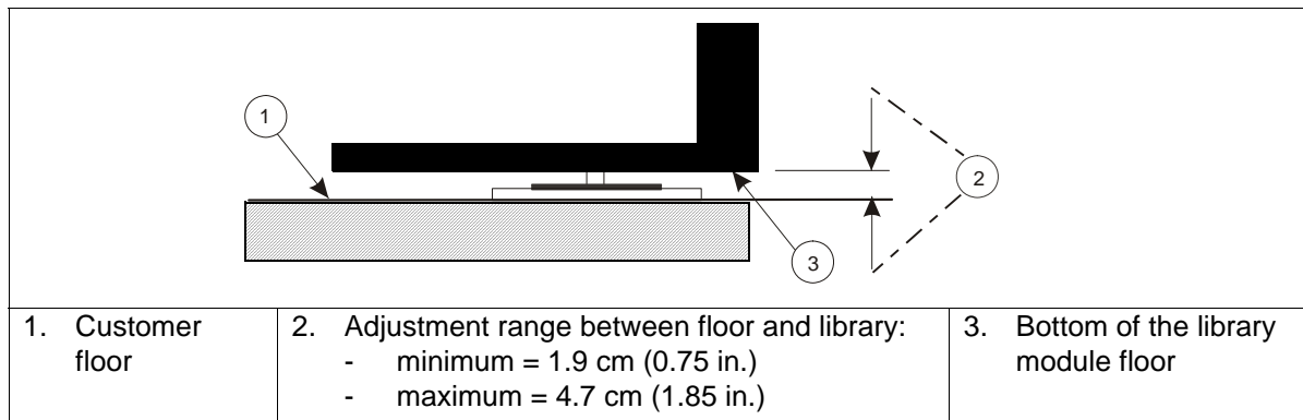
Figure 33. Minimum and Maximum Height Specifications
