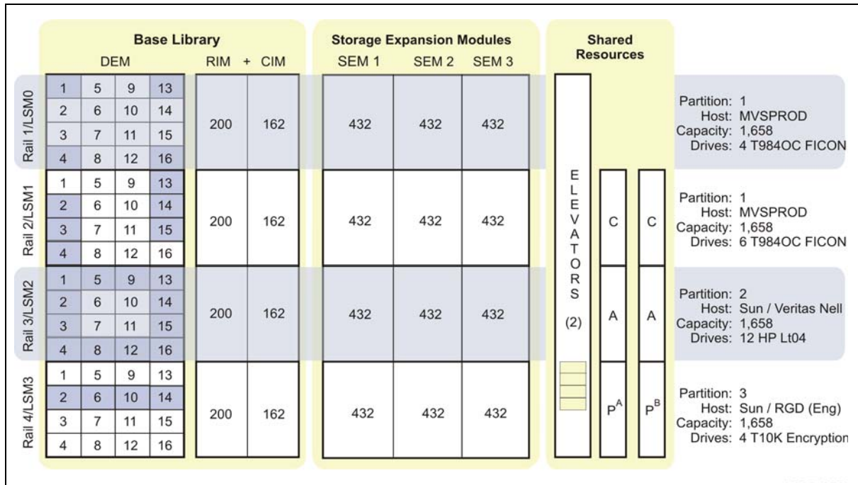
Figure 18. Partition Planning Example
