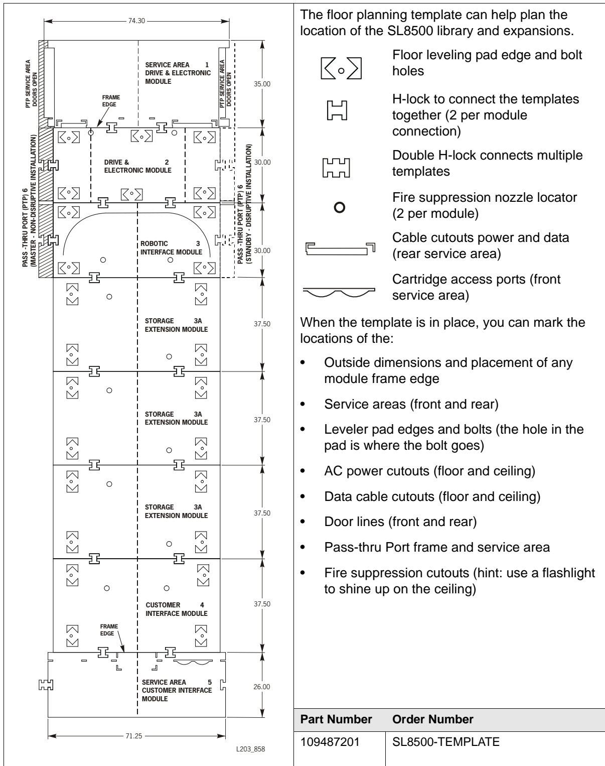
Figure 27. Floor Planning Template
