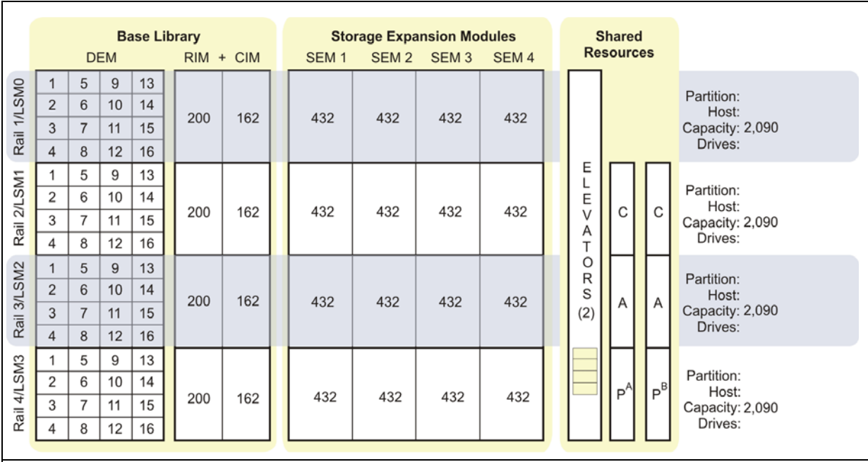
Figure 23. Four Expansion Modules Partition Planning
