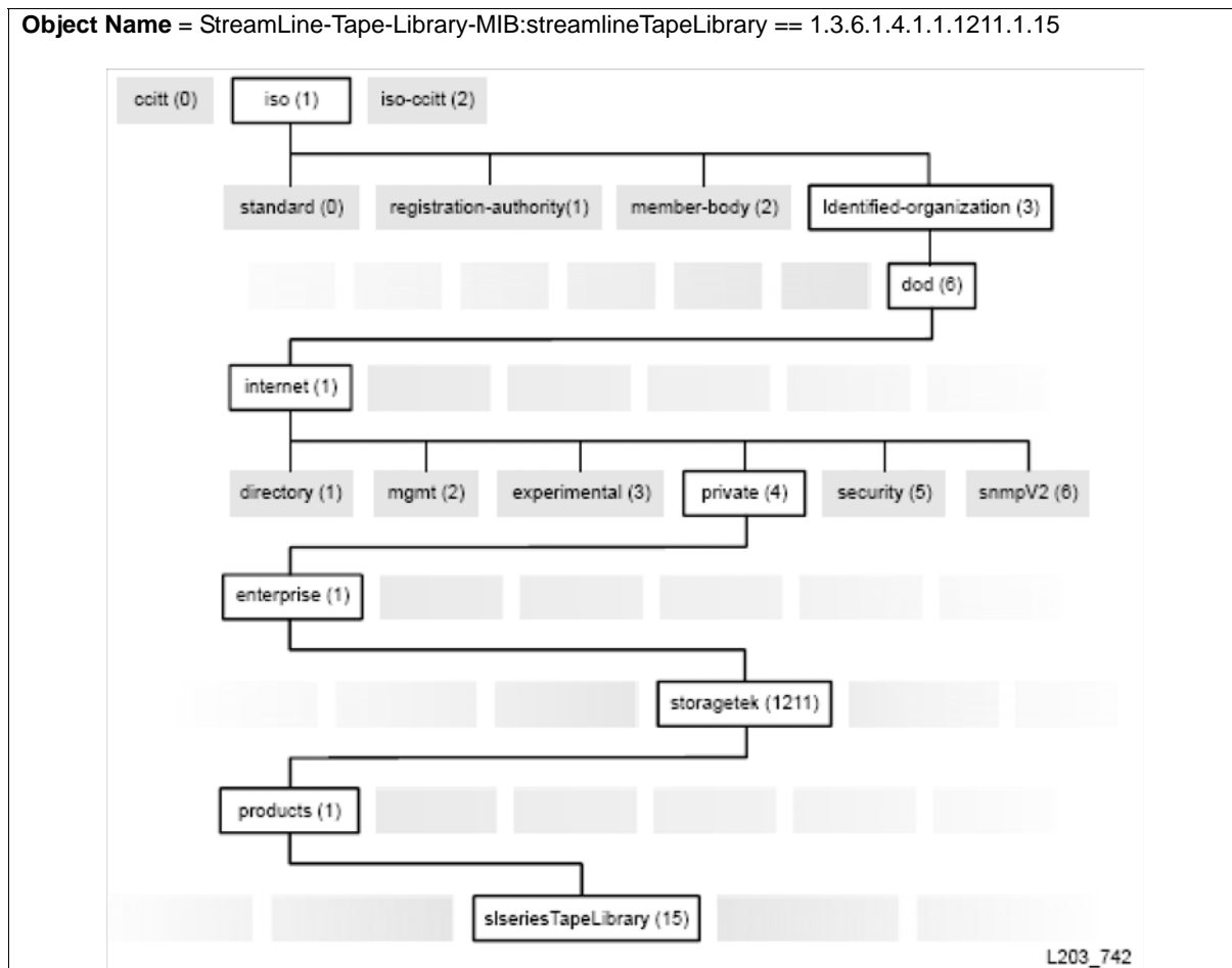
Figure 21. Management Information Base Hierarchy
