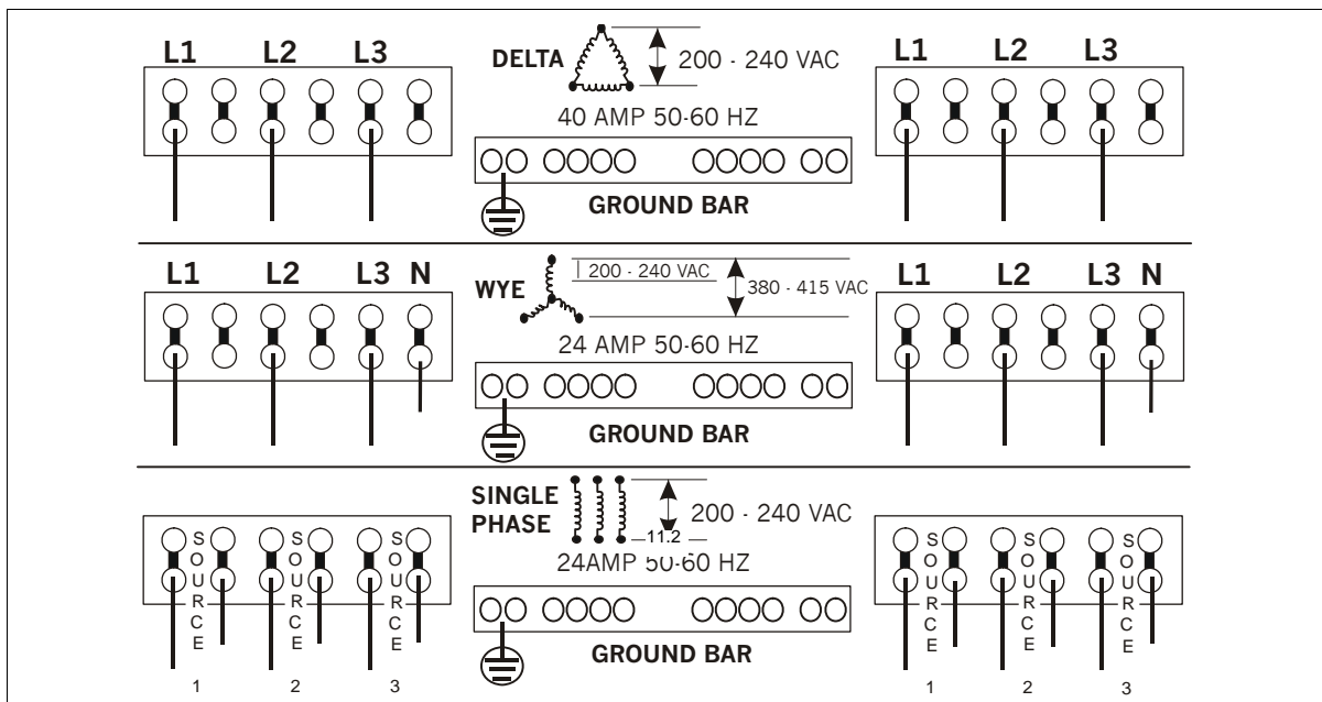
Figure 26. Terminal Block
