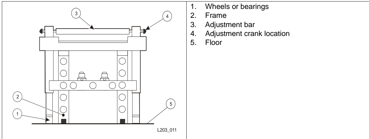
Figure 39. Adjustable Jack
