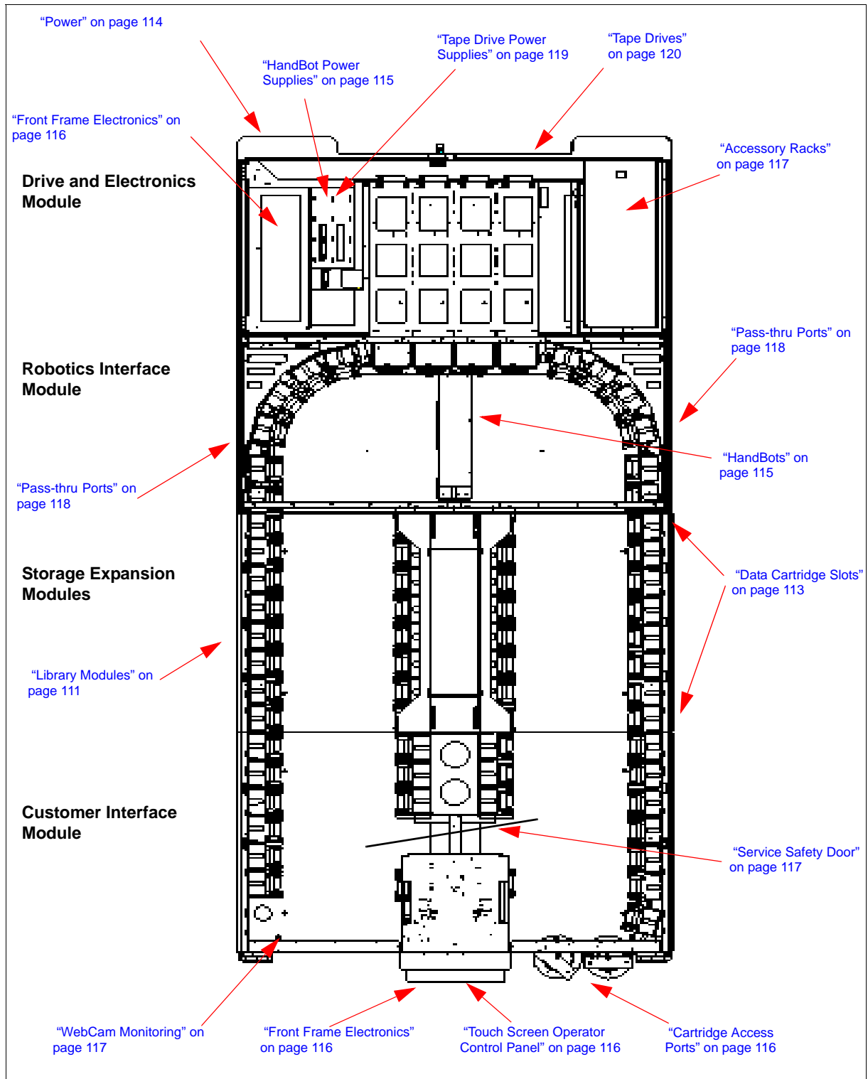
Figure 41. Features and Their Locations
