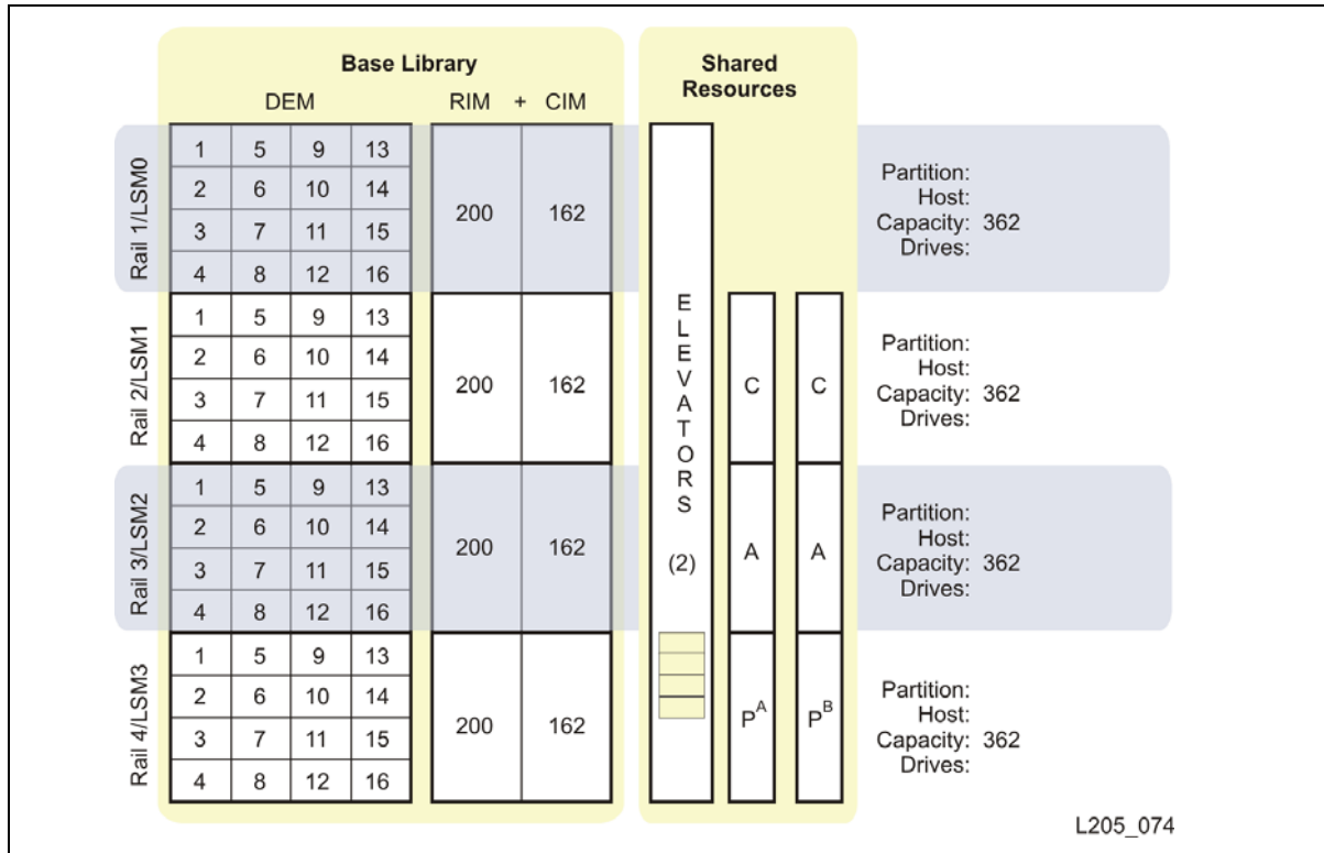
Figure 29. Partition Planning—Base Library
