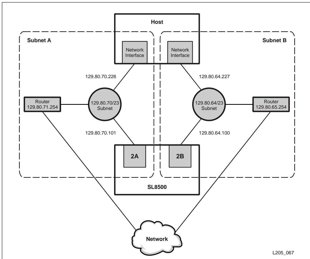
Figure 13. Multi-Homed Host, Multi-Homed SL8500 on Two Subnets
