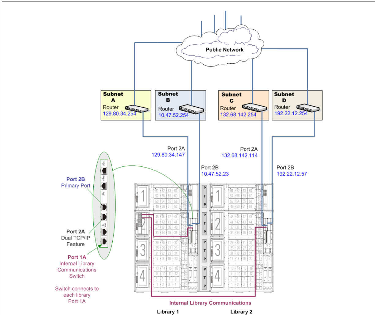
Figure 26. Multi-Host Configuration—Two Libraries with Four Host Connections
