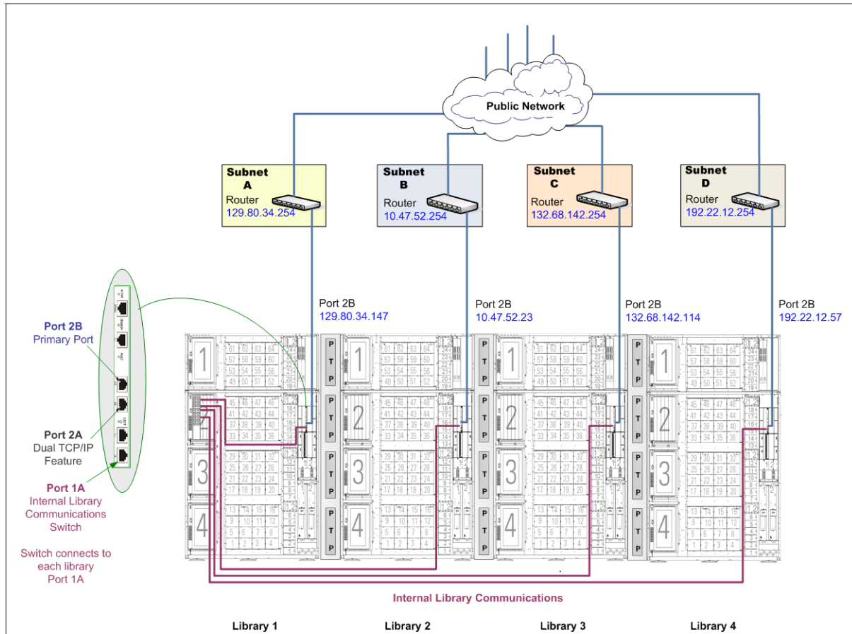
Figure 25. Multi-Host Configuration—Four Libraries with Four Host Connections
