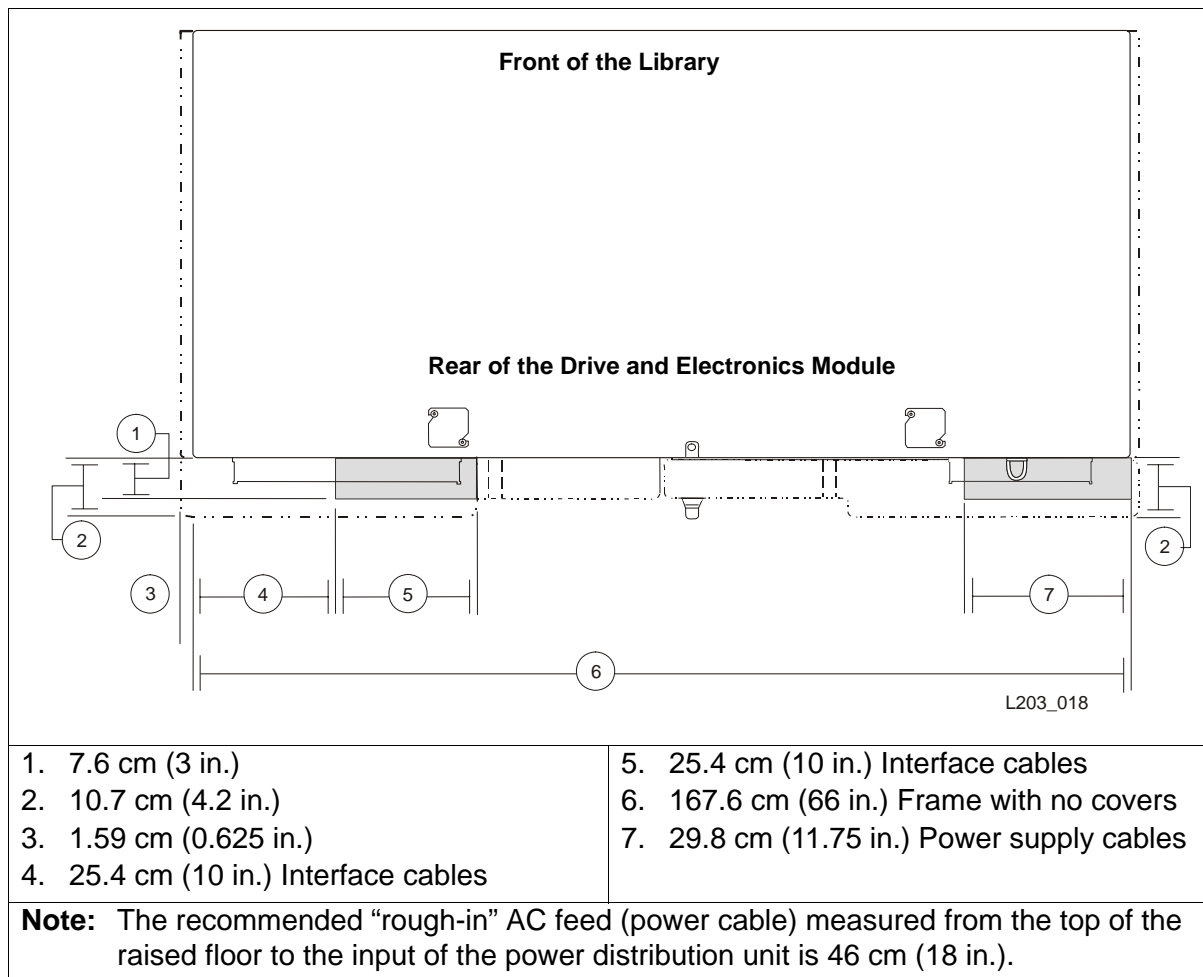
Figure 30. Floor Cutouts for Power and Signal Cables
