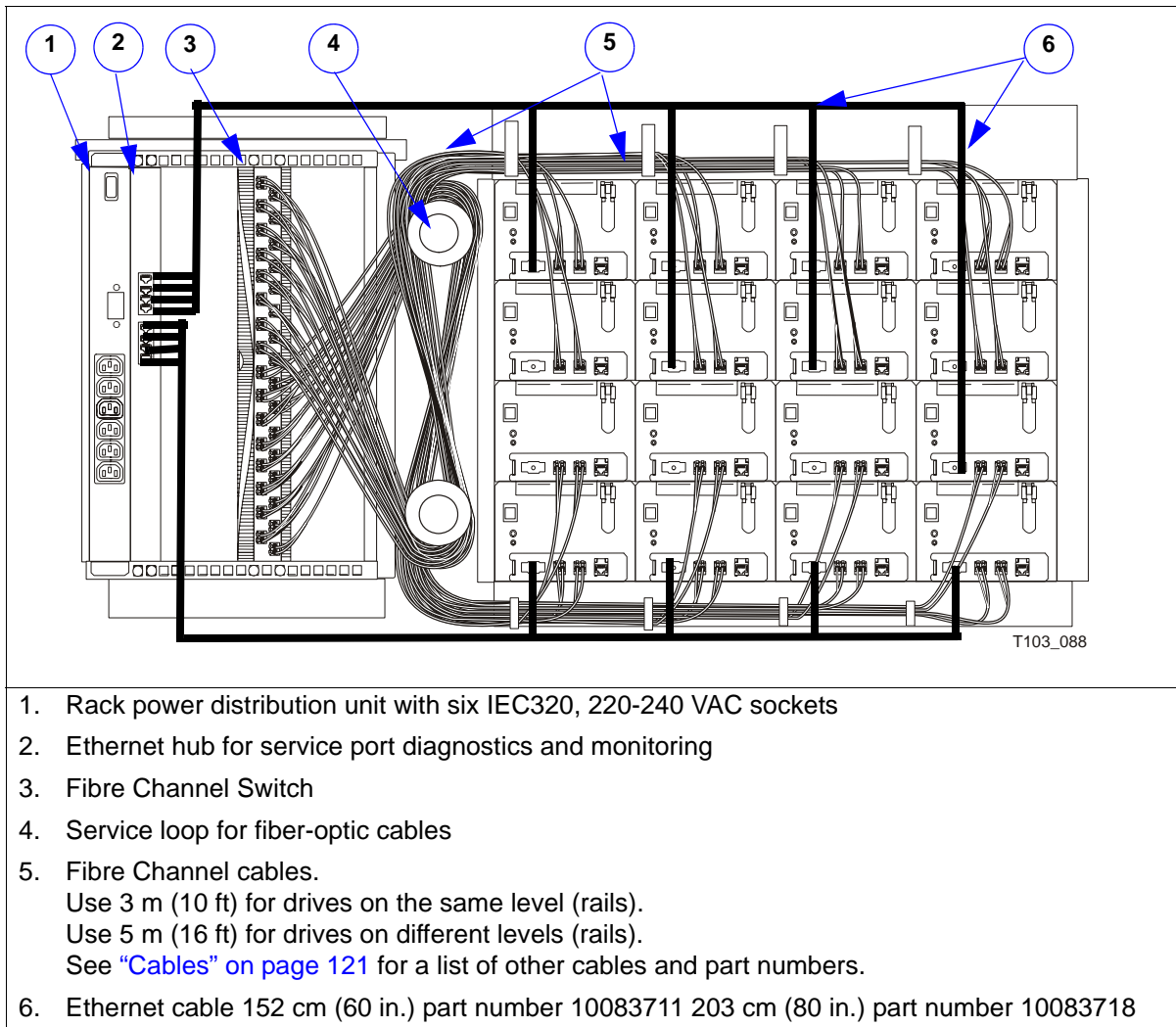
Figure 36. Cabling Tape Drives (Example, figure is not exact)
