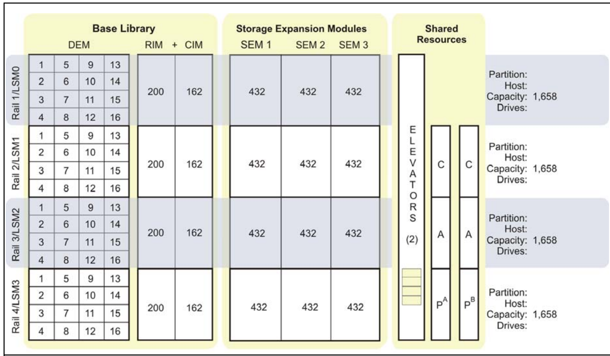
Figure 22. Three Expansion Modules Partition Planning
