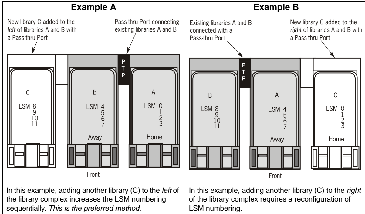
Figure 37. Pass-thru Port Planning Example
