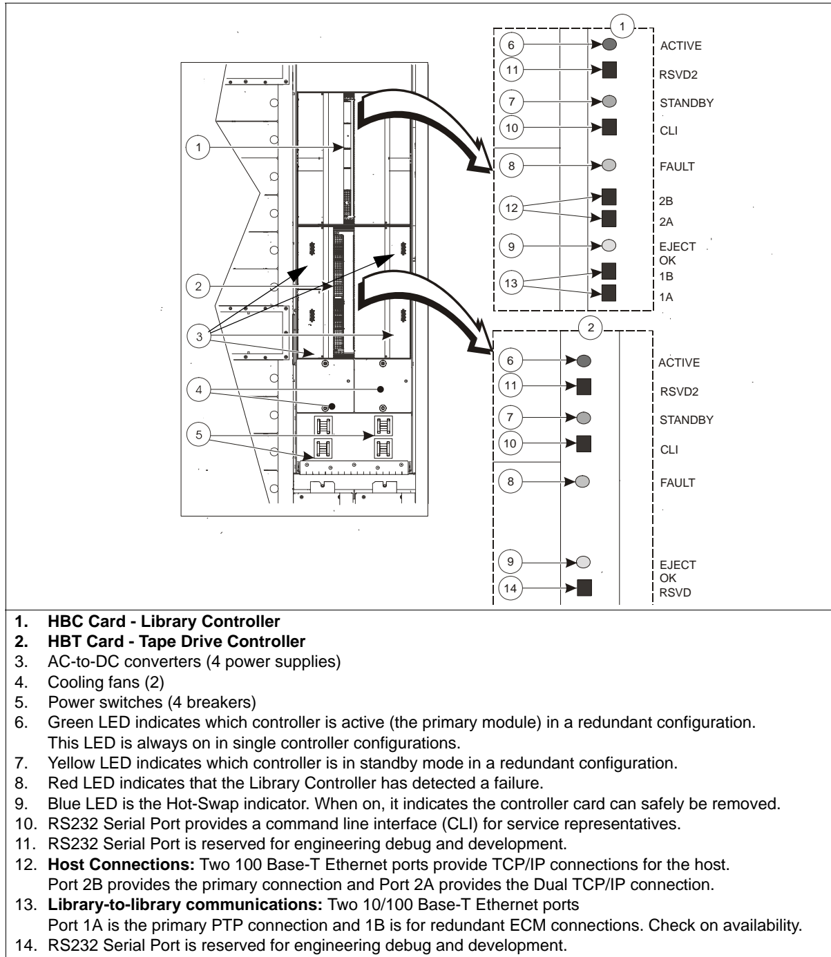
Figure 35. Electronic Control Module
