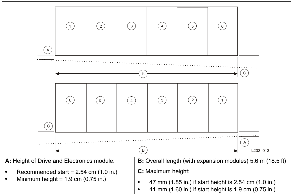
Figure 29. Co-planar – Floor Slope Diagram
