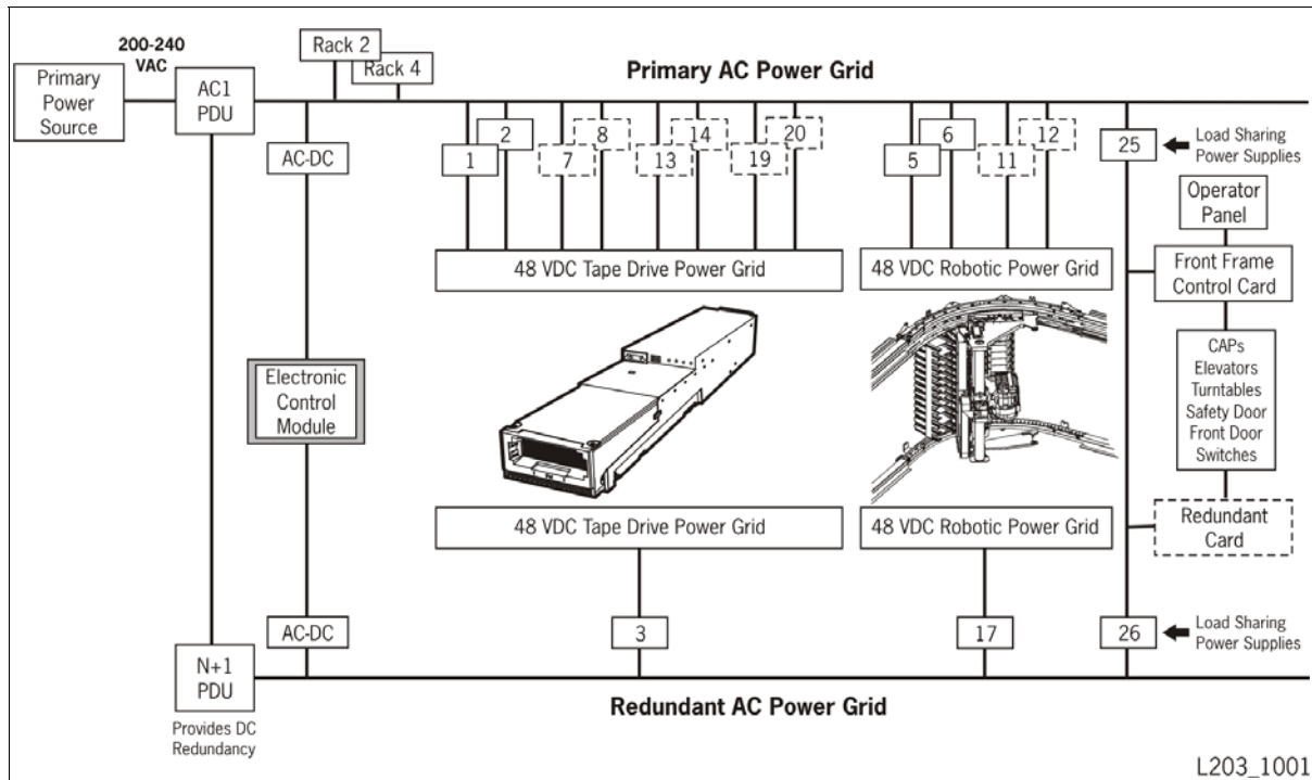
Figure 5. N+1 Power Configuration
