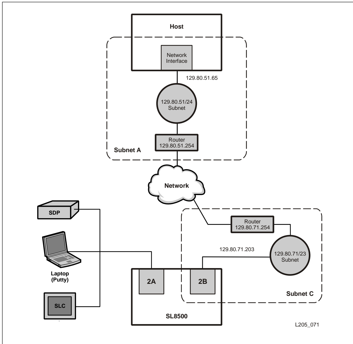
Figure 16. Dual TCP/IP Port 2A Service Connection
