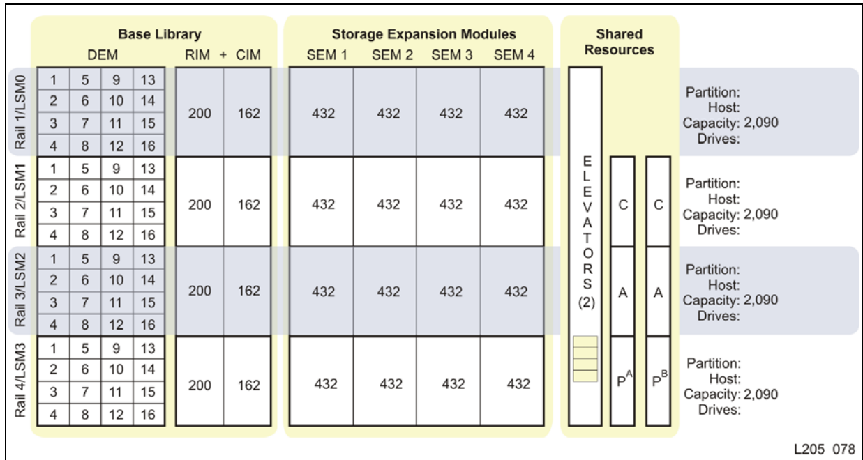
Figure 33. Partition Planning—Four Expansion Modules
