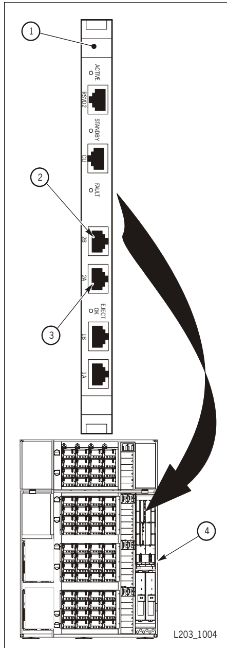
Figure 17. TCP/IP Connections
