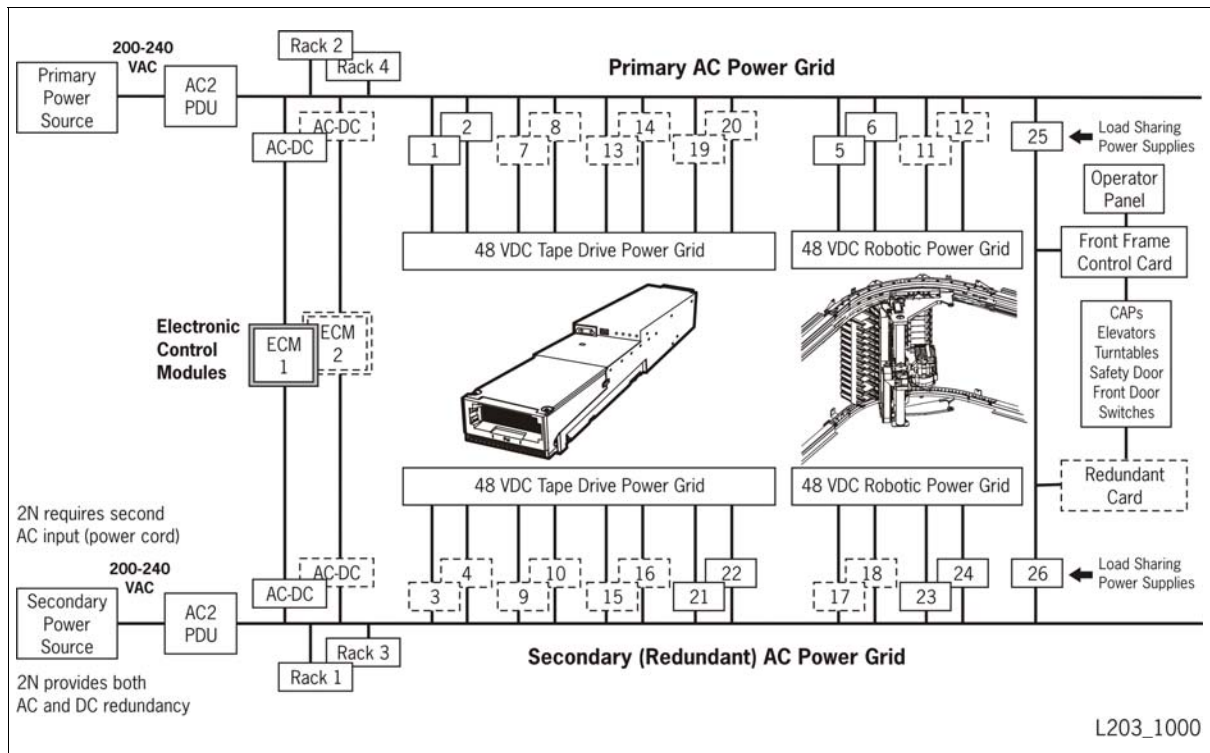
Figure 6. 2N Power Configuration (Optional Feature)
