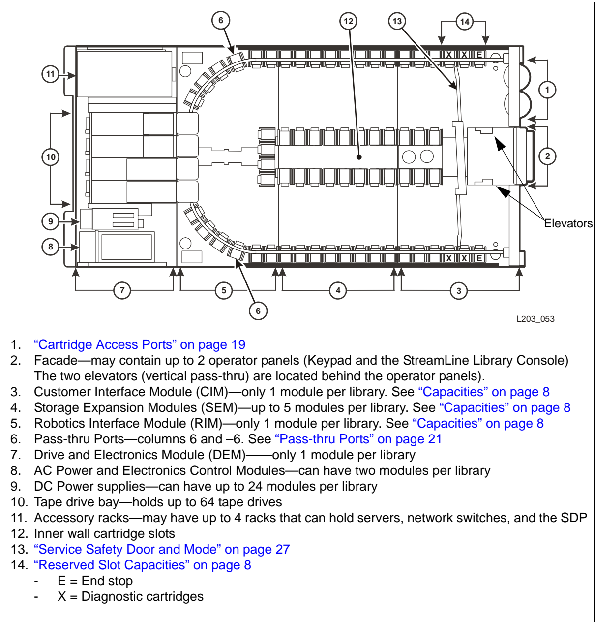
Figure 2. Library Modules
