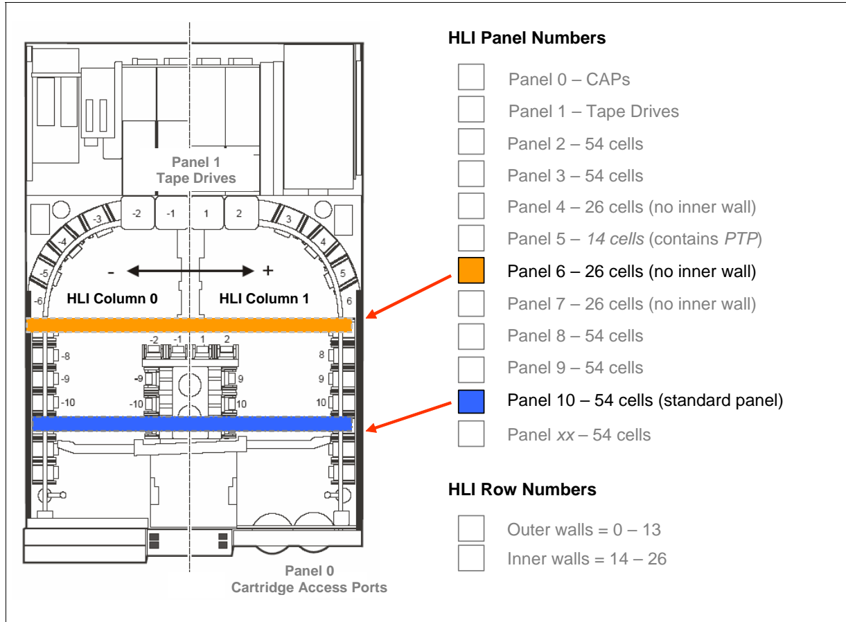
Figure 3. Panel Numbering
