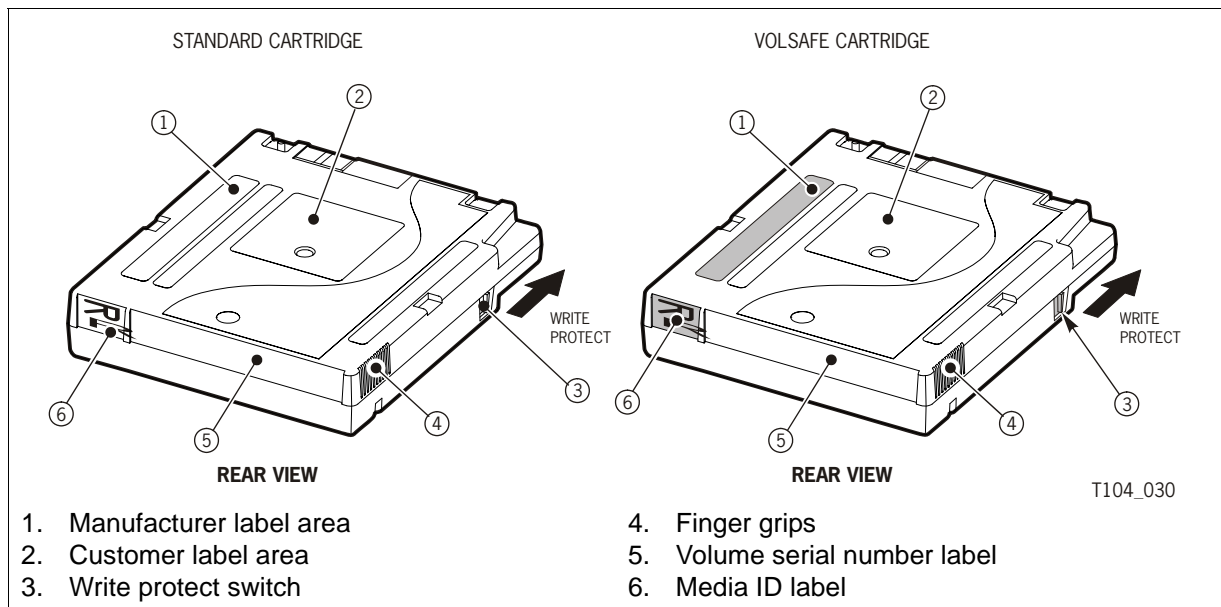
Figure 8. VolSafe/WORM Tape Cartridge Example
