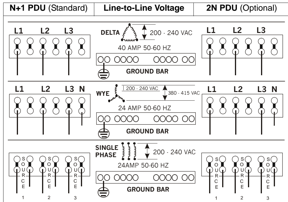
Figure 7. Delta or Wye?
