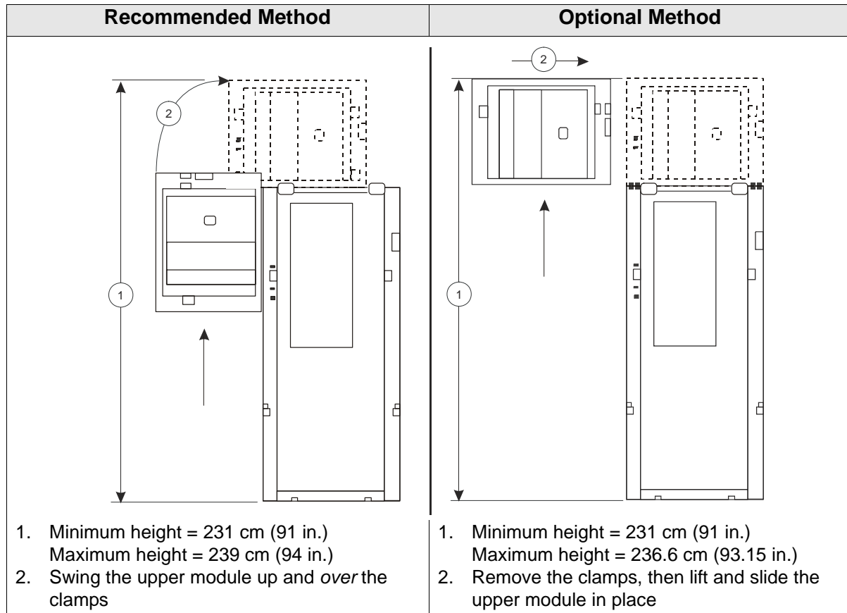
Figure 32. Upper Module Installation
