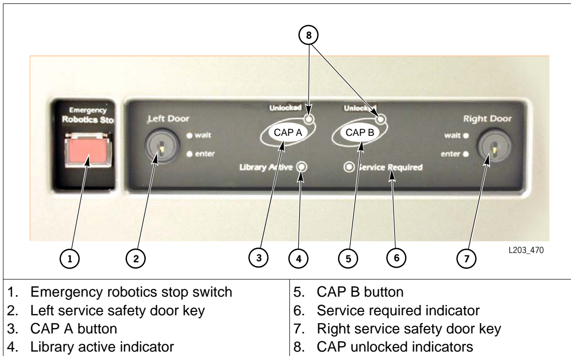
Figure 13. Keypad
