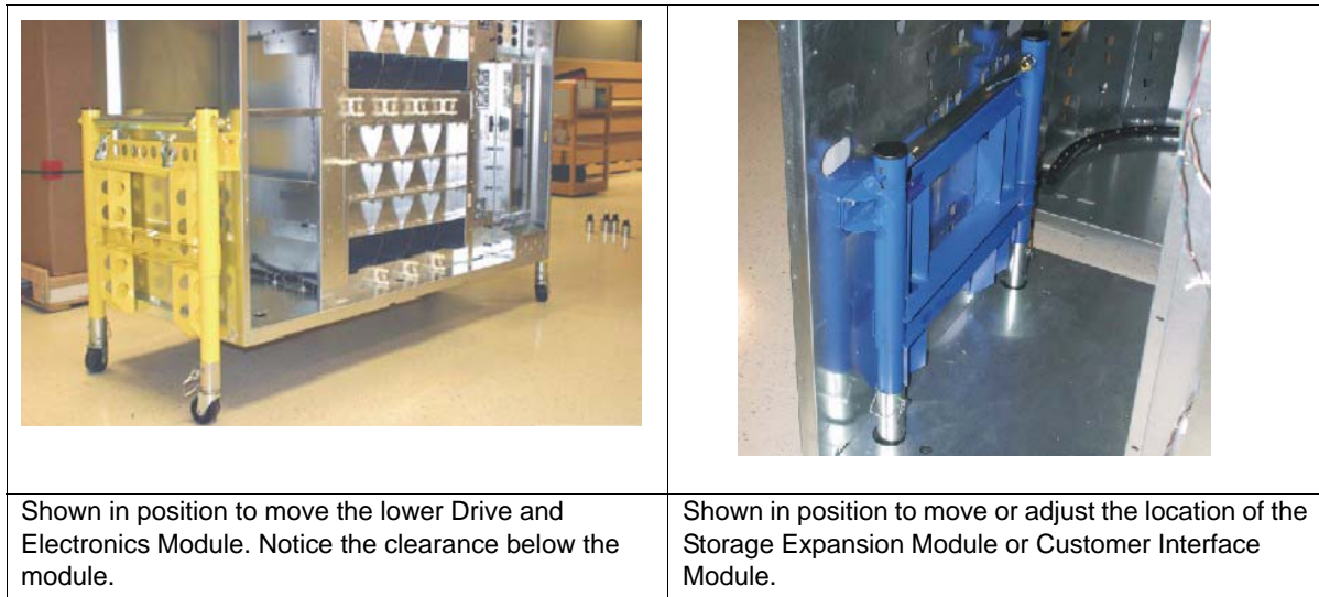
Figure 40. Jack Positioning
