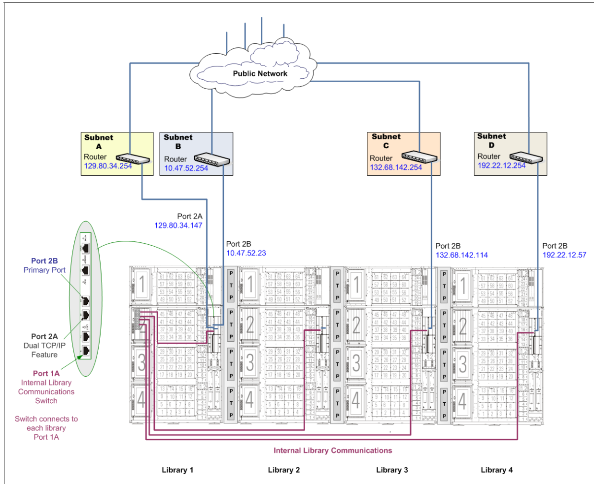
Figure 27. Multi-Host Configuration—with Two Plus Two Host Connections
