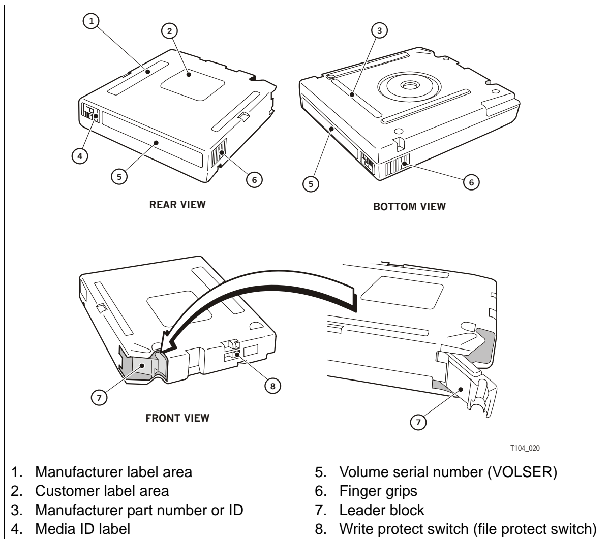
Figure 4. 9940 Tape Cartridge
