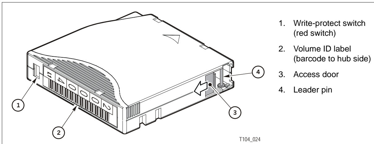
Figure 6. LTO Tape Cartridge
