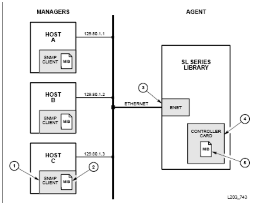
Figure 20. SNMP Block Diagram
