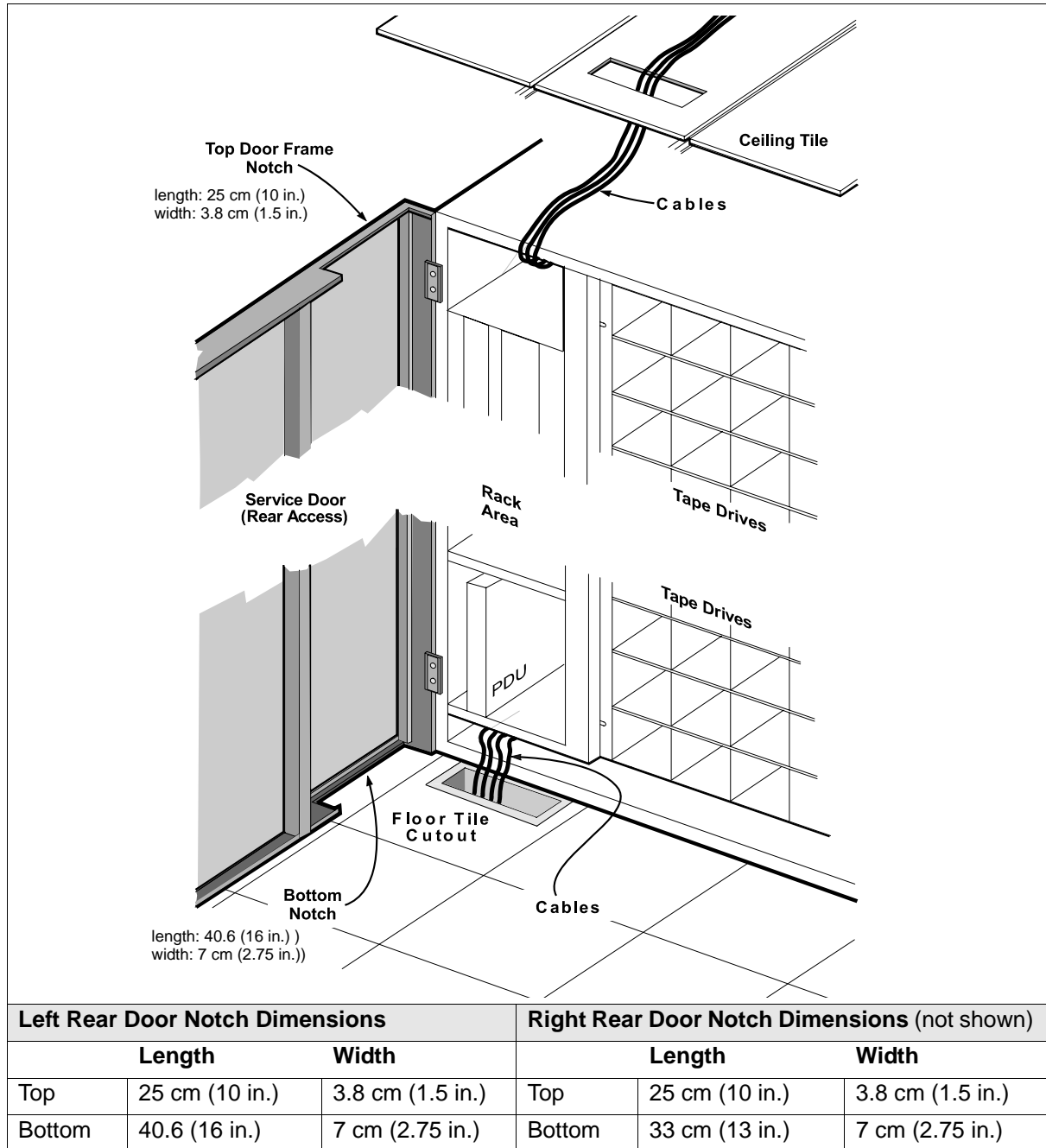
Figure 31. Cabling Routing
