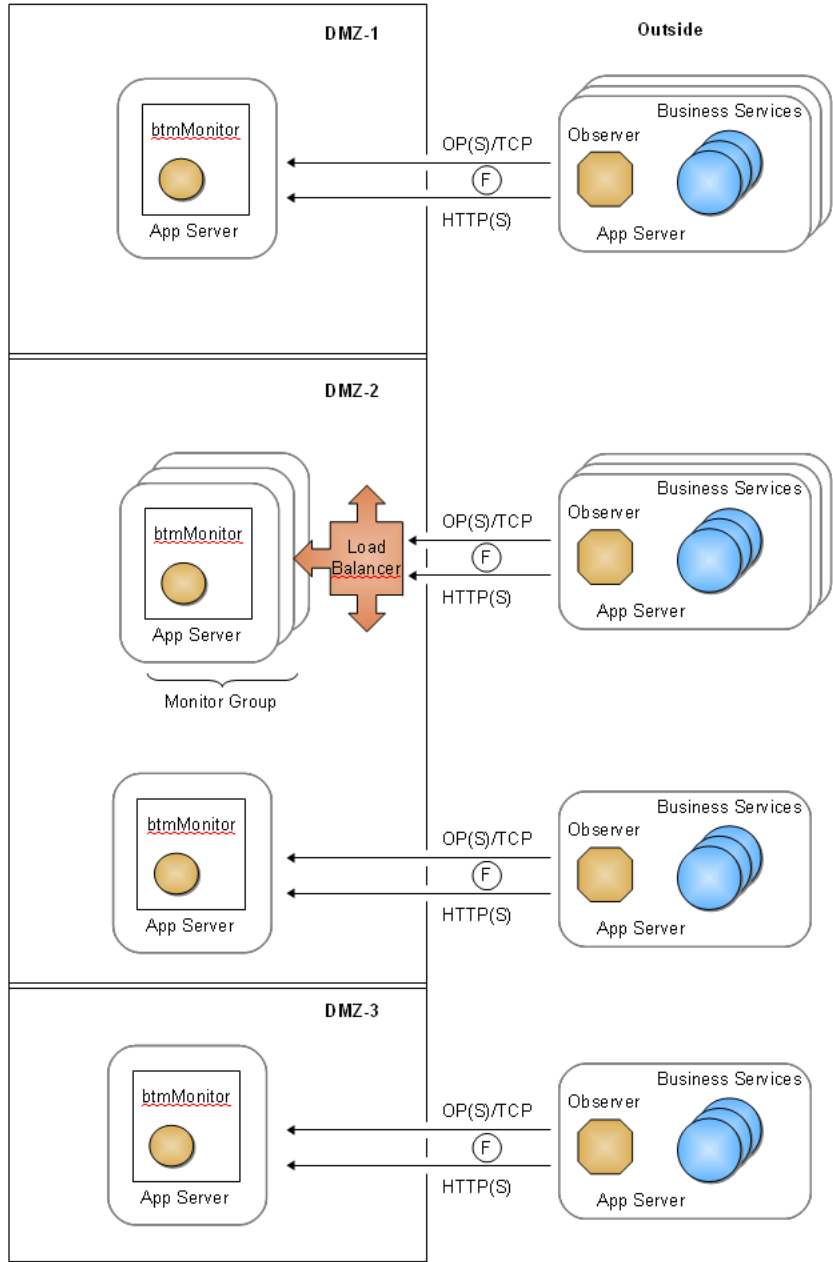
Figure 4-4 Communication Connections Between the Monitors and Observers
