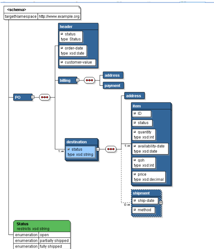
Figure 4–55 PO Schema for Tree Mode Rules Sample
