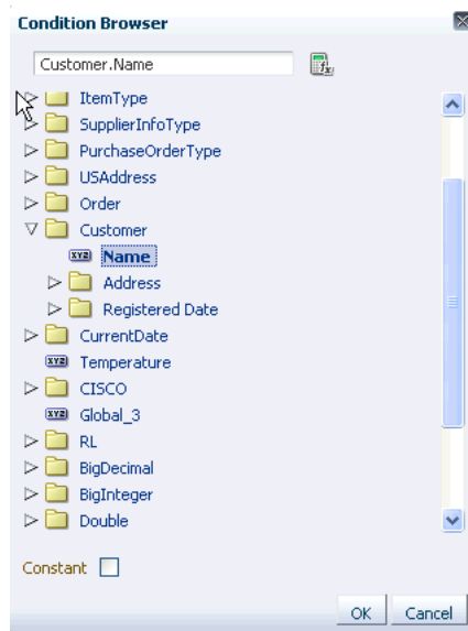
Figure 12–52 The Condition Browser
