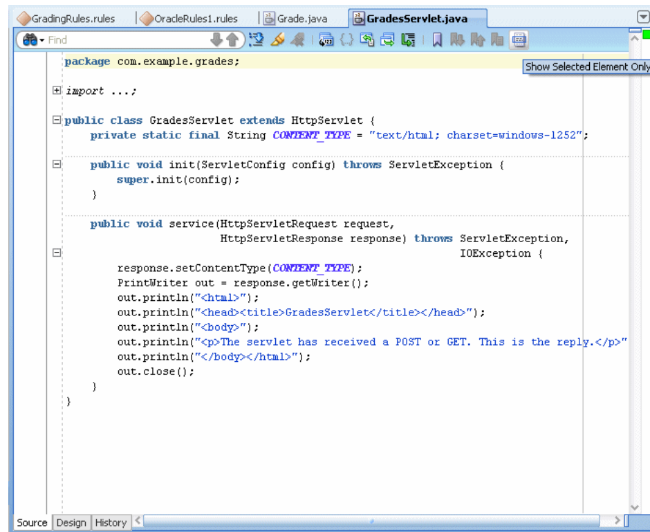
Figure 9–19 Generated GradesServlet.java
