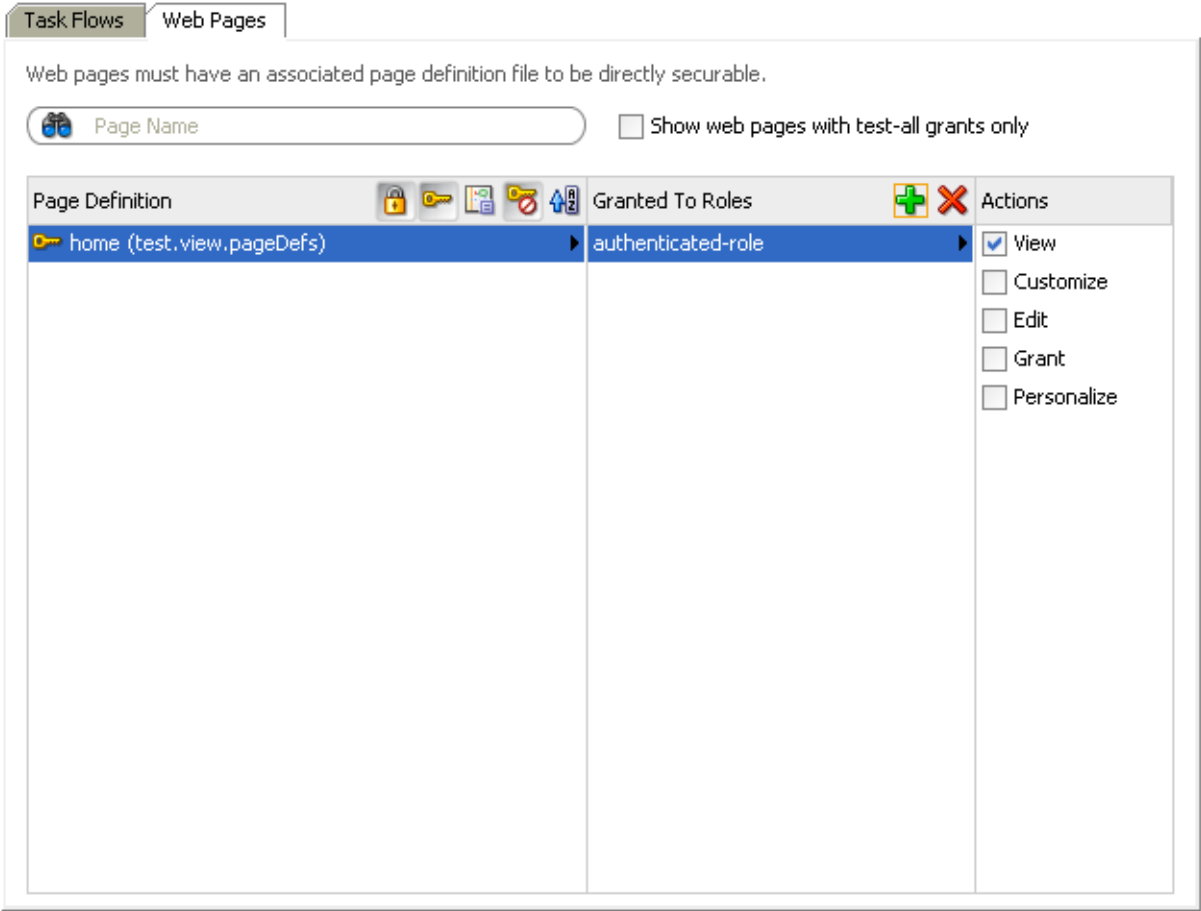
Figure 19–3 Adding Privileges to Page with the Page - Create New Task Flow
