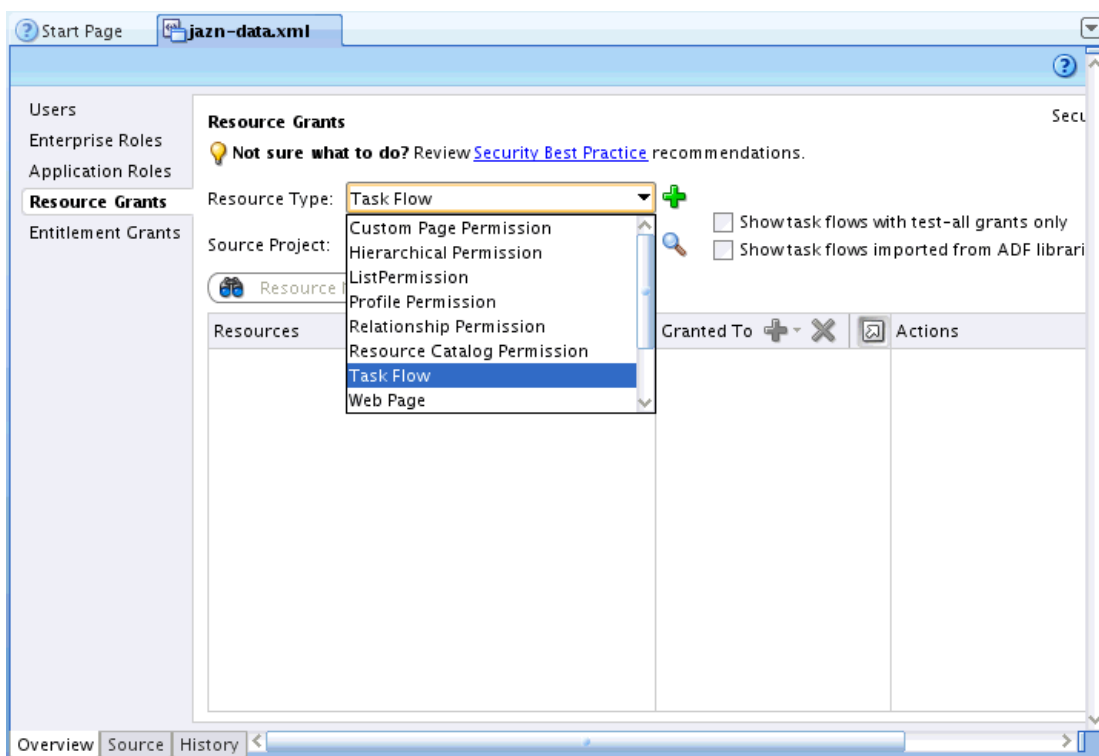
Figure 7-2 ADF Security Policies in the jazn-data.xml File
