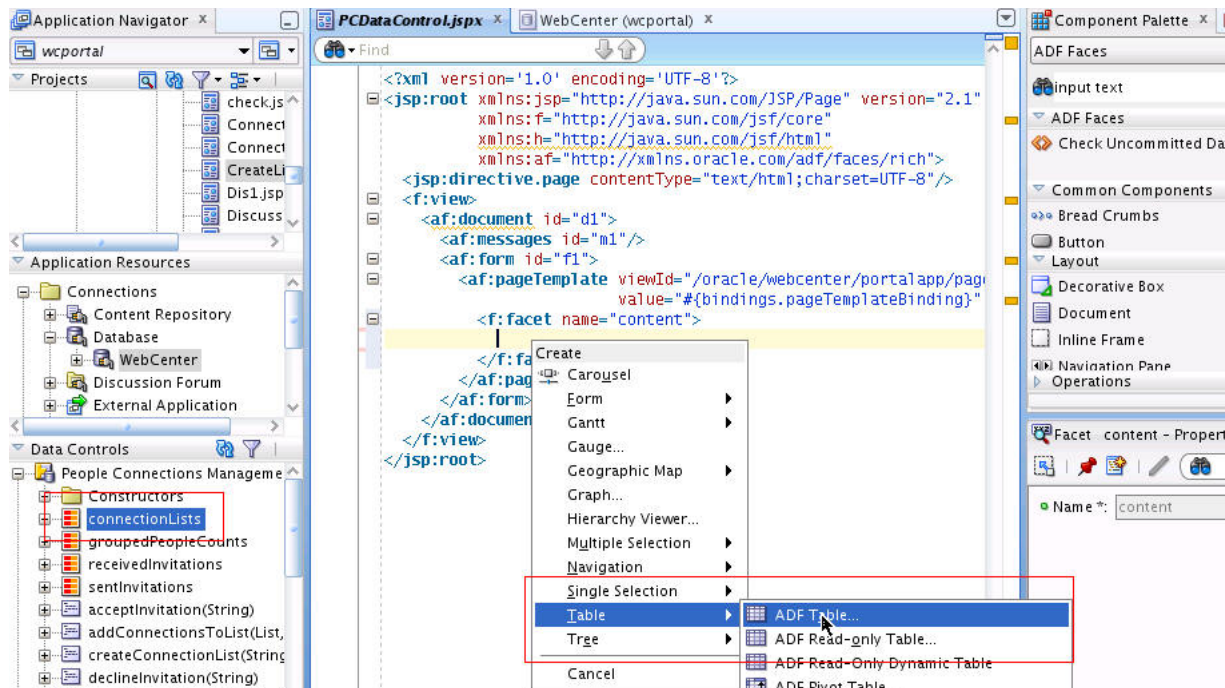
Figure 41-1 The Data Control Object Dragged and Dropped on to a .jspx Page With ADF Table Selected
