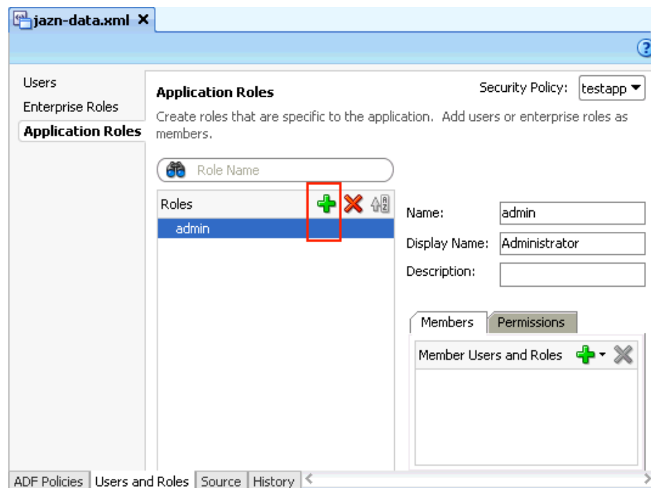
Figure 24–2 Roles Section in the jazn-data.xml File
