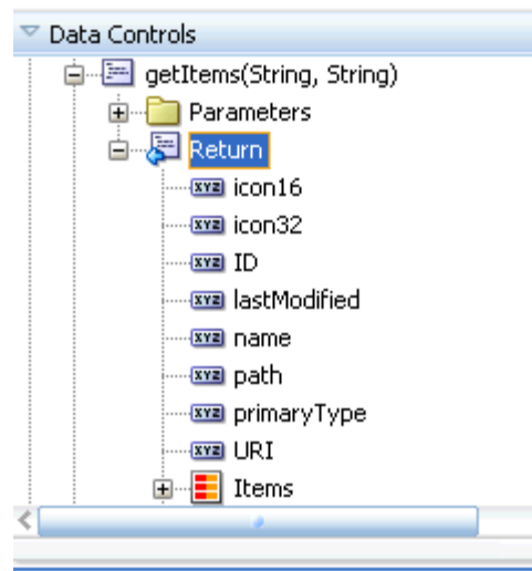
Figure 28–15 The Return node of the getItem method
