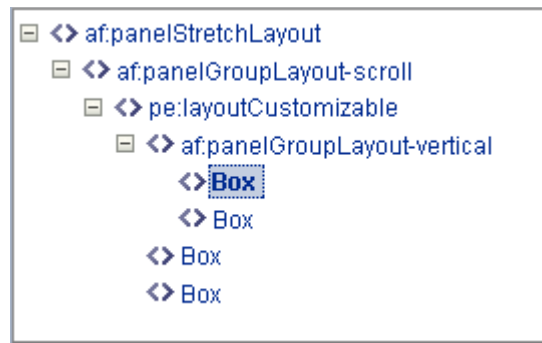
Figure 18–18 Box Component Added Below
