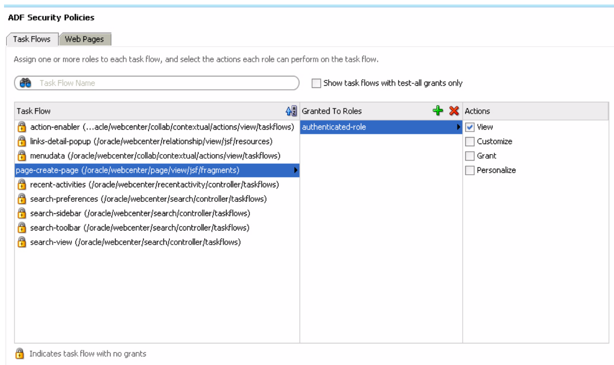
Figure 19–2 Adding Privileges to the Page - Create New Task Flow
