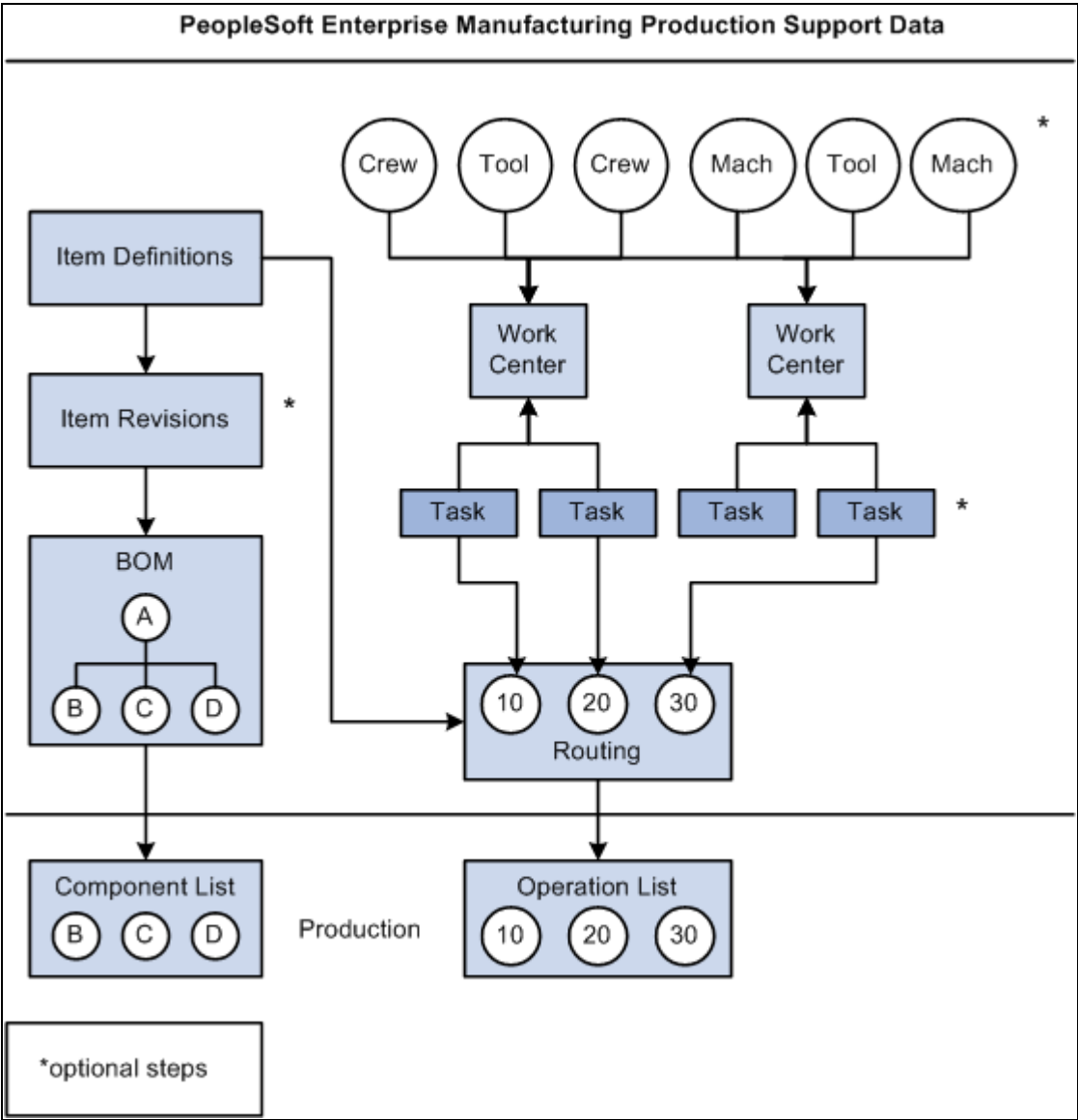
PeopleSoft Manufacturing production support data
