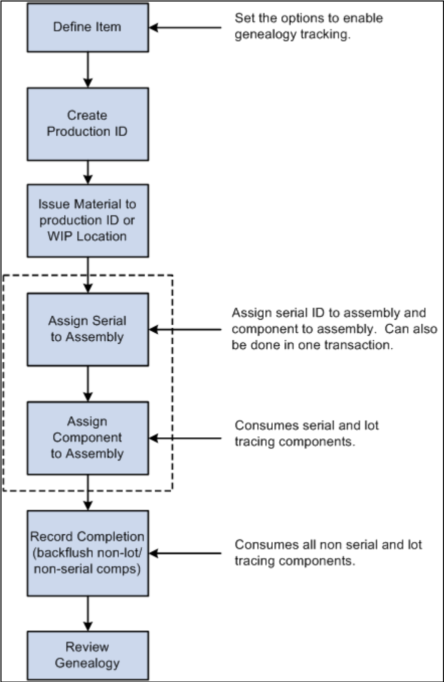
Serial Genealogy Process Flow
