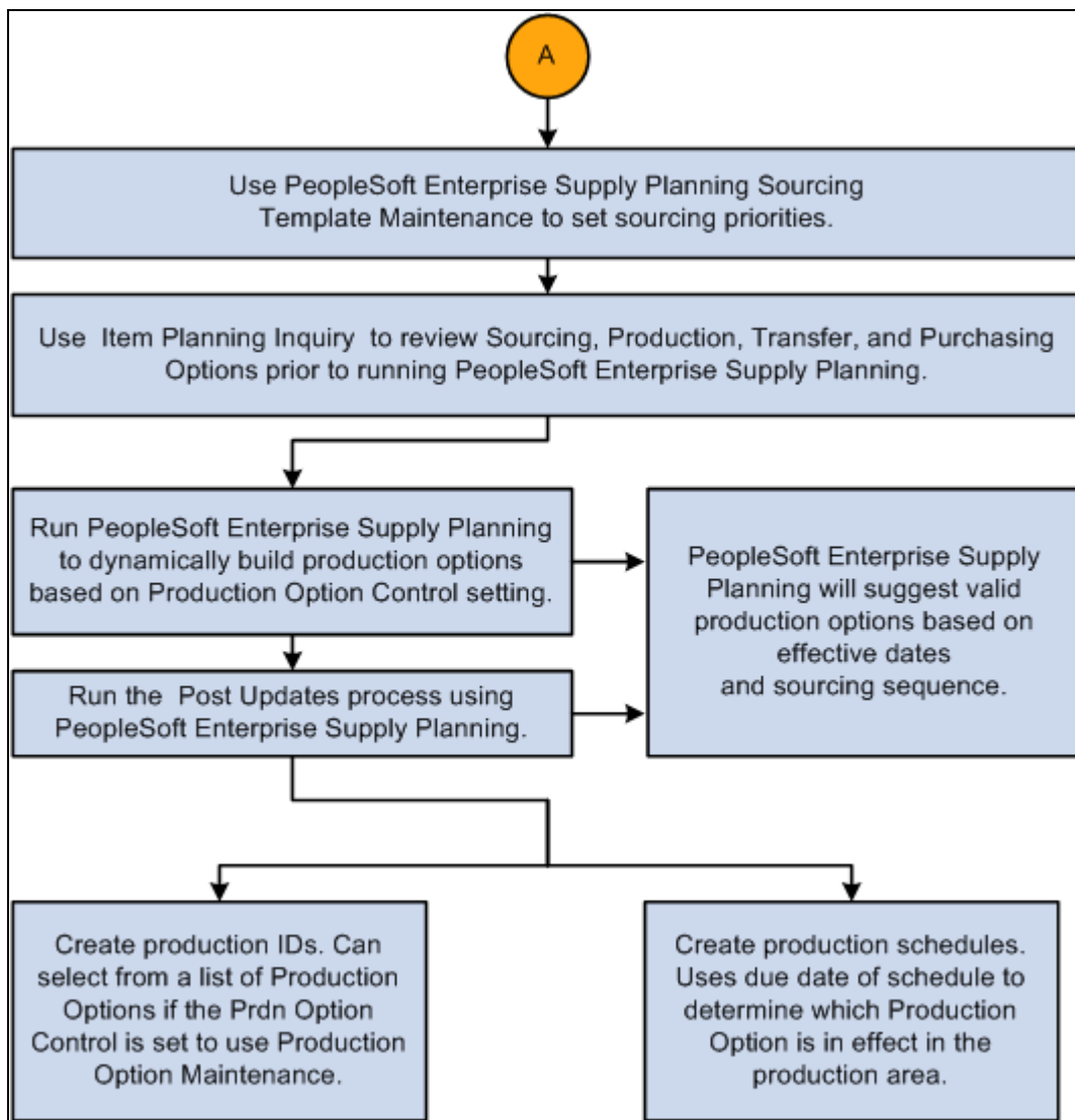
Production option business process overview (2 of 2)
