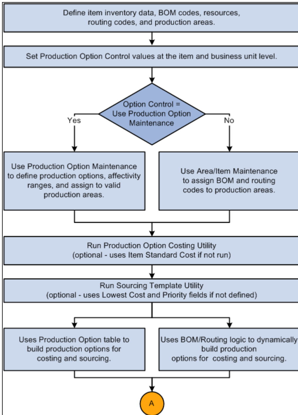
Production option business process overview (1 of 2)
