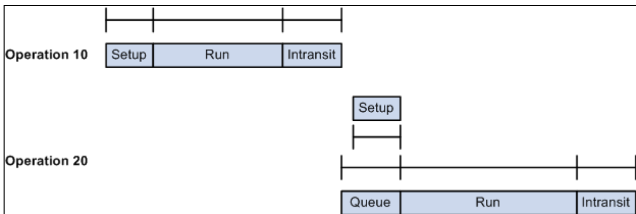
Example 3: Queue time takes three hours and setup takes one hour
