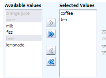
Figure 9–27 selectOrderShuttle Component
