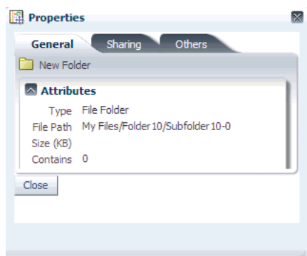
Figure 13–1 af:dialog Component
