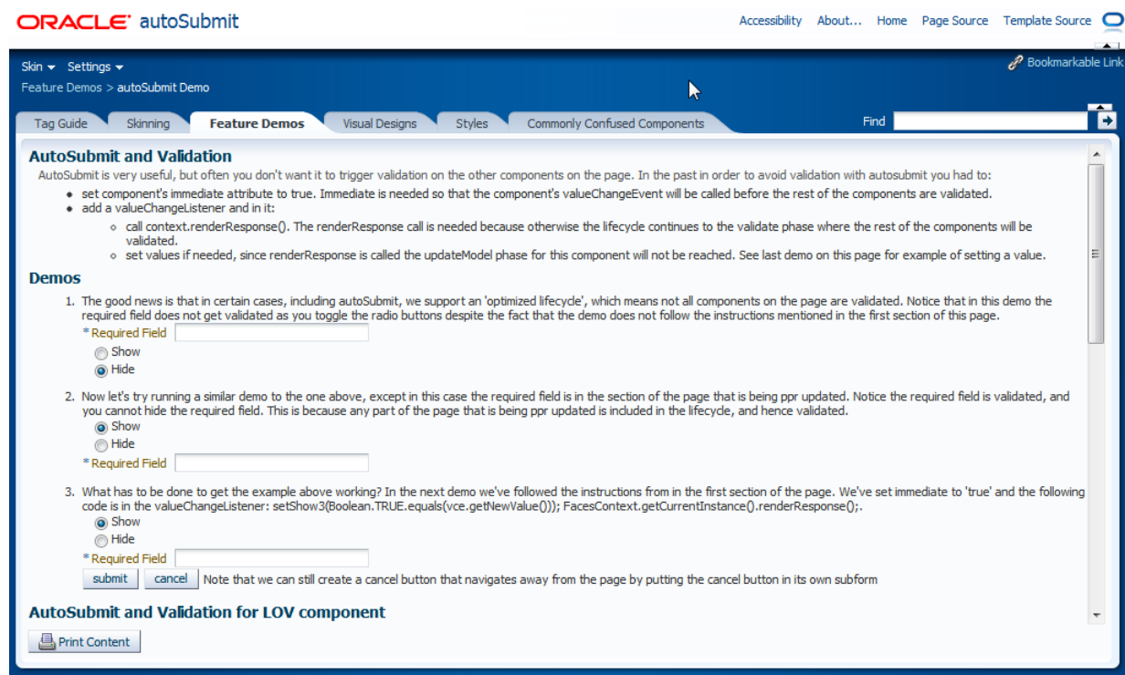
Figure 1–4 Framework Demonstration
