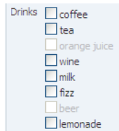
Figure 9–19 selectManyCheckbox Component
