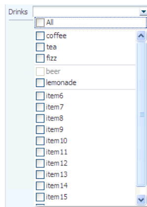
Figure 9-25 selectManyChoice Component
