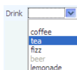
Figure 9–22 selectOneChoice Component
