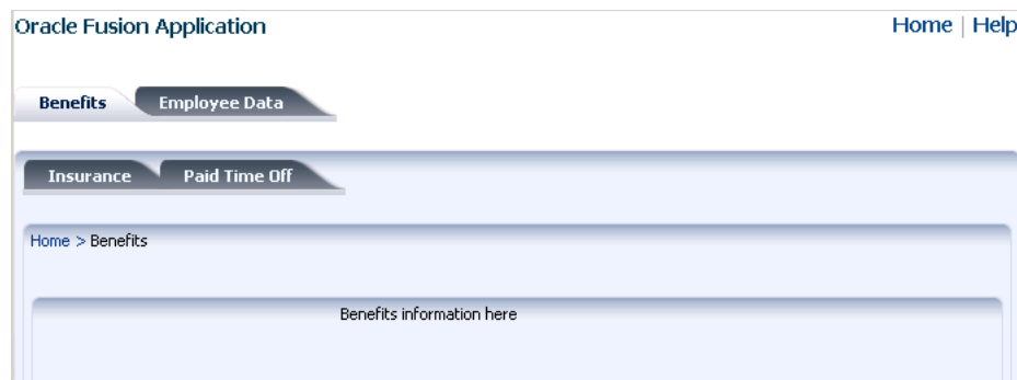
Figure 18–6 First-Level Page
