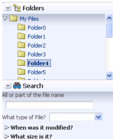
Figure 8–34 panelAccordion Panes
