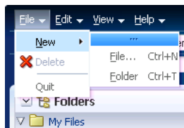
Figure 14–8 Detachable Menu
