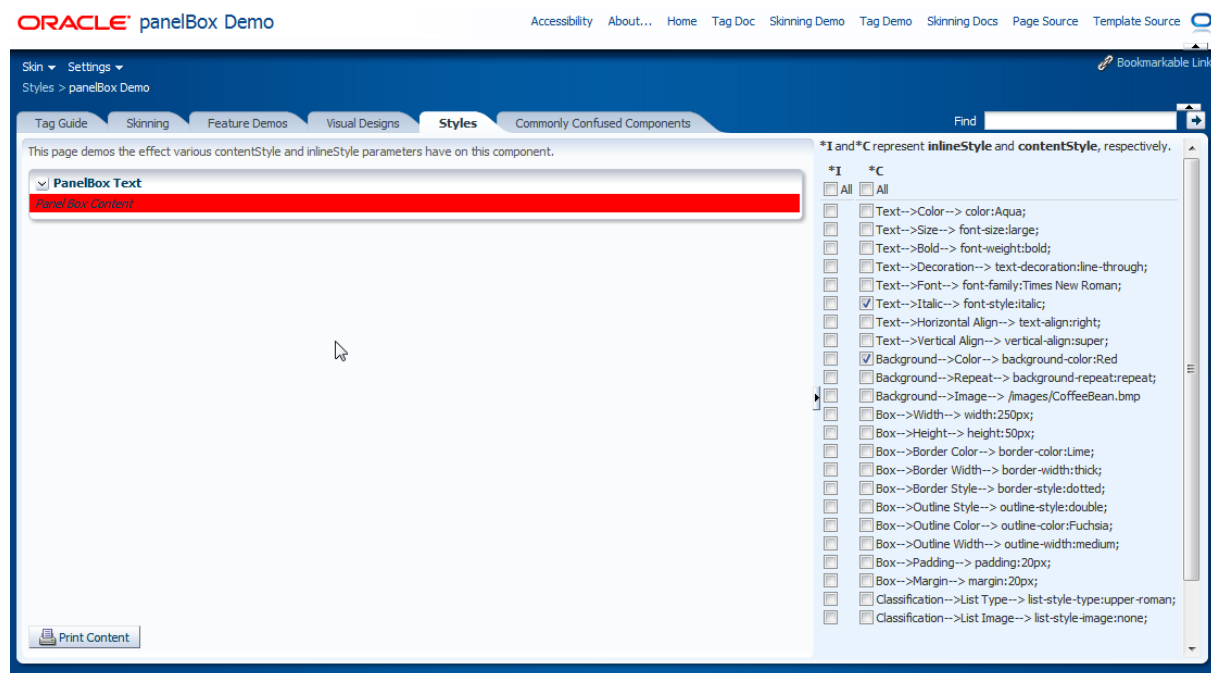
Figure 1–6 Styles Demonstration
