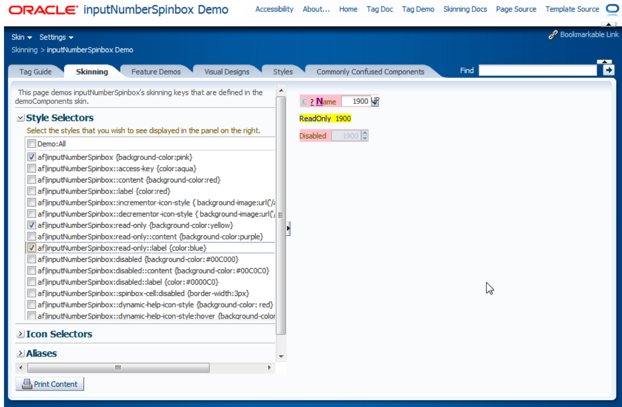
Figure 1–2 Skinning Demonstration
