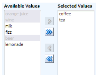
Figure 9–26 selectManyShuttle component
