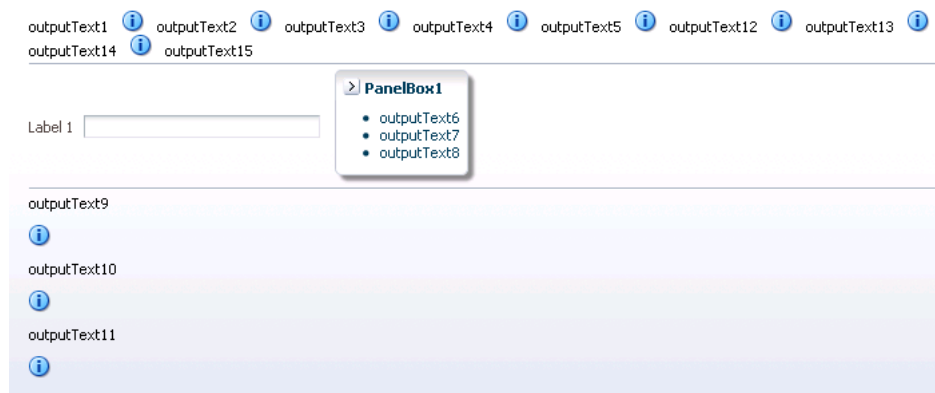
Figure 8–49 panelGroupLayout Arrangements
