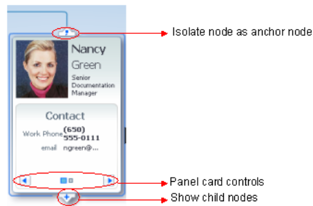
Figure 29–6 Node Controls
