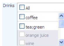
Figure 9–21 selectManyListbox Component
