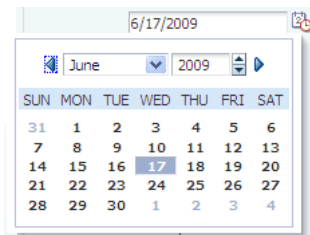
Figure 9–13 inputDate Component
