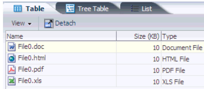
Figure 8–38 panelTabbed Panes
