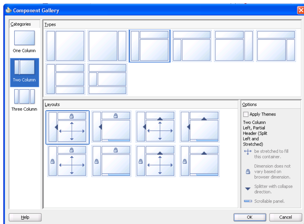
Figure 8–5 Quick Layouts
