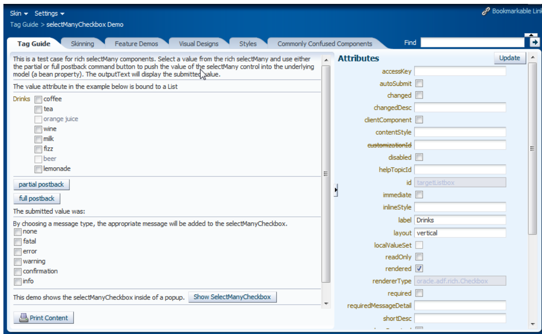
Figure 1–1 Tag Demonstration
