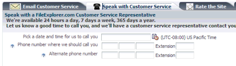
Figure 1–11 Help System
