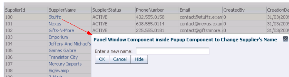
Figure 13–4 Popup Component Invoked by a Server-Side Method
