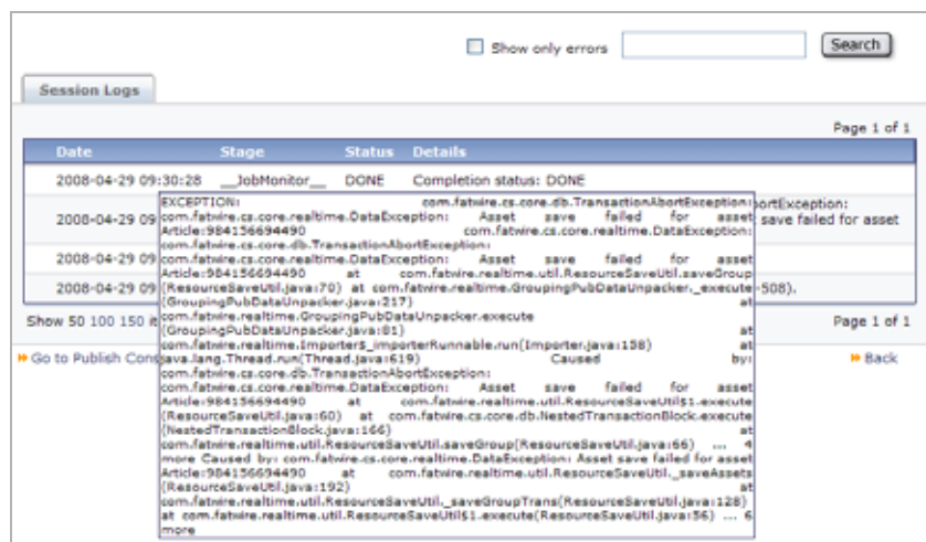
Figure 9: The Session Log is interactive; view a detailed entry by clicking the “show all” link next to the summary entry
