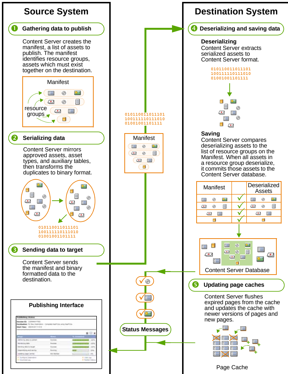
Figure 12: The Five Stages of Publishing
