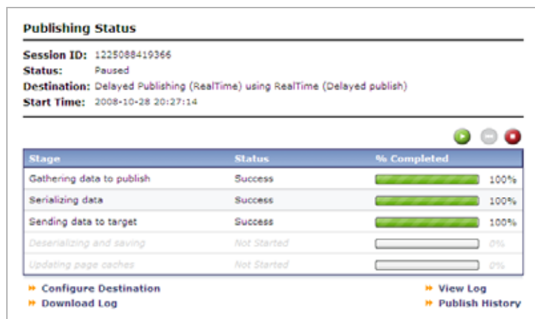
Figure 7: The 'Publishing Status' screen communicates up to the moment status information about active publishing sessions
