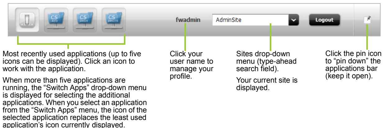
Figure 4: Applications bar
