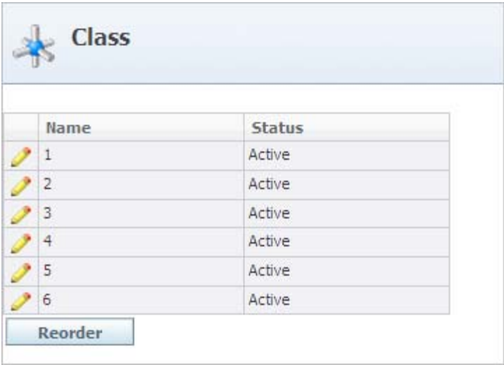
Figure 4-71 Class list
