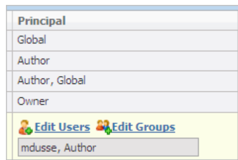
Figure 6-24 Added tokens
