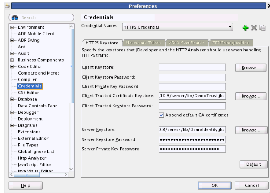
Figure 7–4 Credentials Pane
