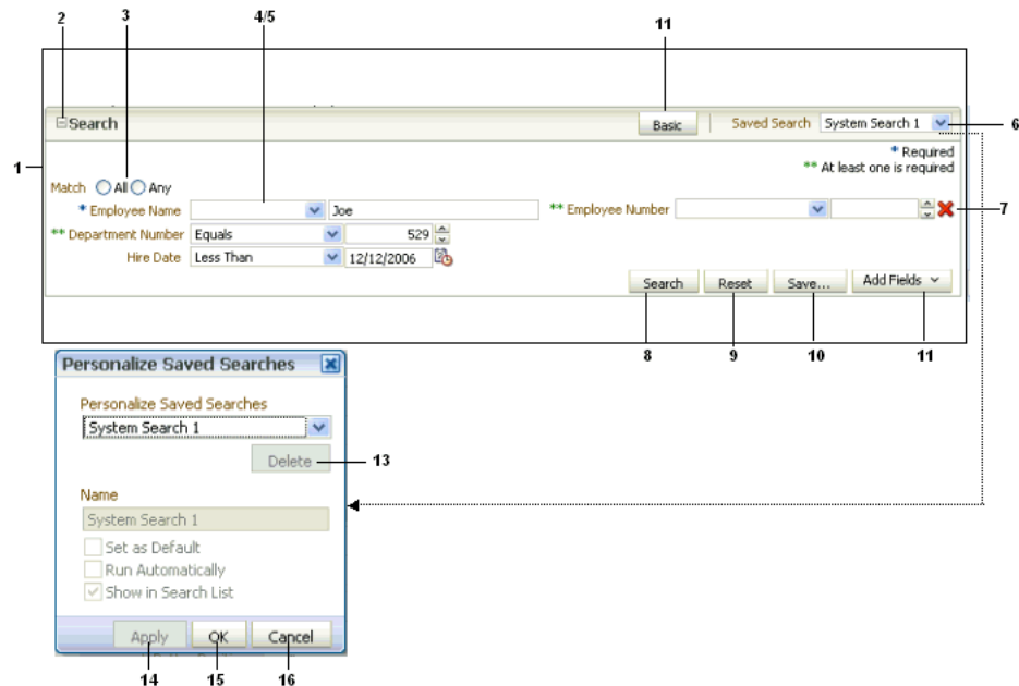
Figure 12–4 Query Component and Associated Popup Dialog
