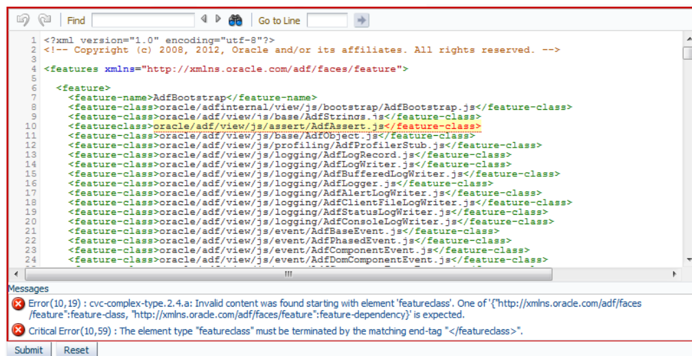
Figure 9–42 Message Pane of Code Editor
