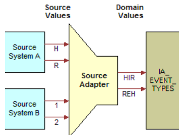
Figure 19–16 HIR and REH Values Populating the W_EVENT_TYPES Table
