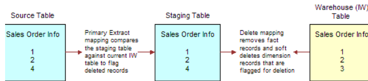
Figure 19–8 Primary Extract and Delete Mappings
