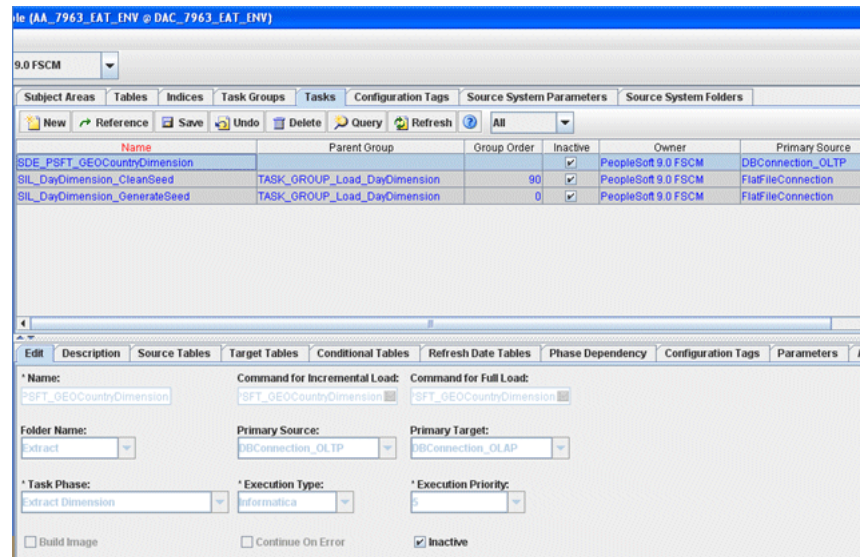
Figure 7–2 FSCM Tasks in DAC
