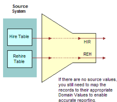
Figure 19-15 Source Values in Different Tables Translated to Domain Values
