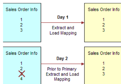
Figure 19–7 Extract and Load Mappings
