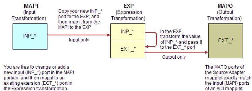
Figure 19–6 Components of the Source Adapter Maplet
