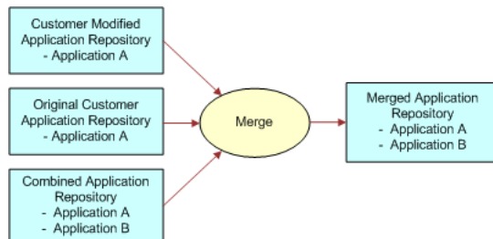
Figure 18–3 Merging with an Oracle BI Repository
