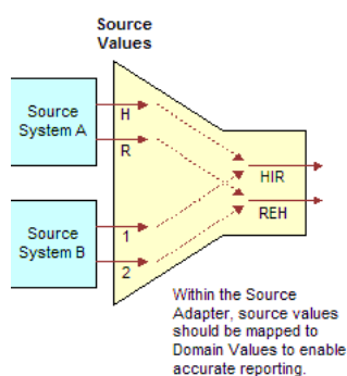
Figure 19-14 Source Values Translated to Domain Values
