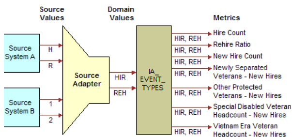
Figure 19-17 Metric Values From HIR and REH Domain Values
