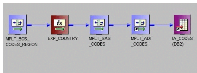
Figure 19–12 Example of a Code Mapping in Informatica PowerCenter Designer
