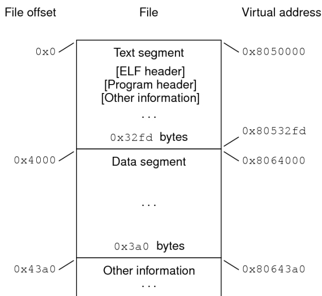
32-bit x86: Dynamic Executable File (64K alignment)
