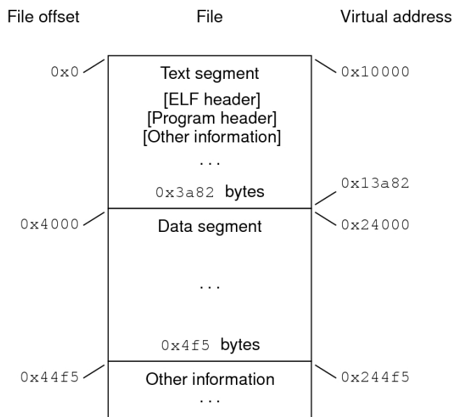
SPARC: Dynamic Executable File (64K alignment)
