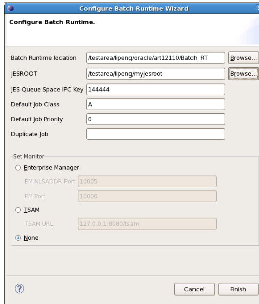
Figure B-13 Configure Batch Runtime
