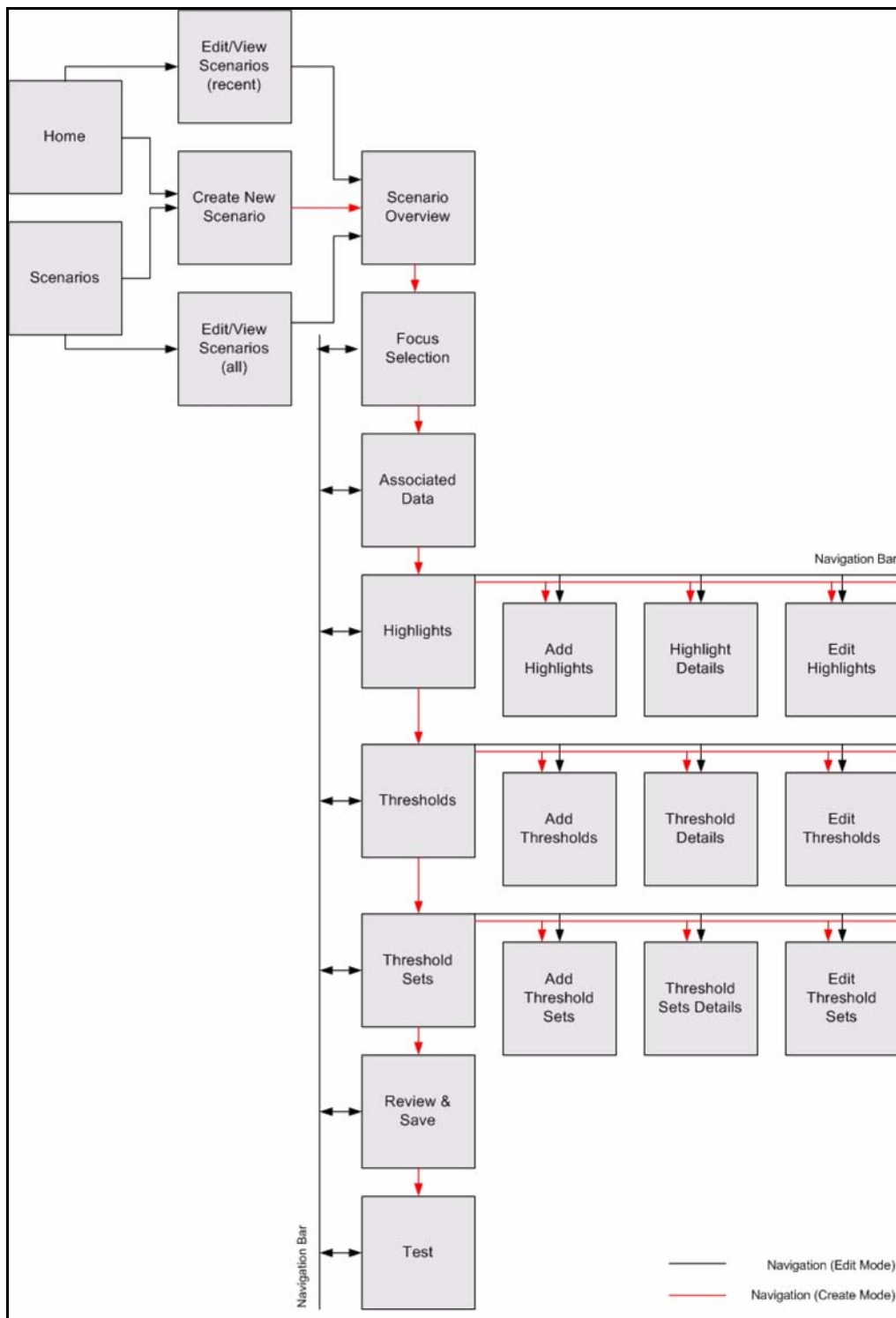
Figure 4. Scenario Wizard Workflow
