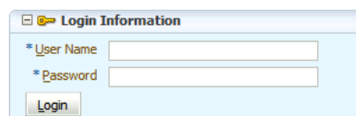
Figure 30–17 Login Page
