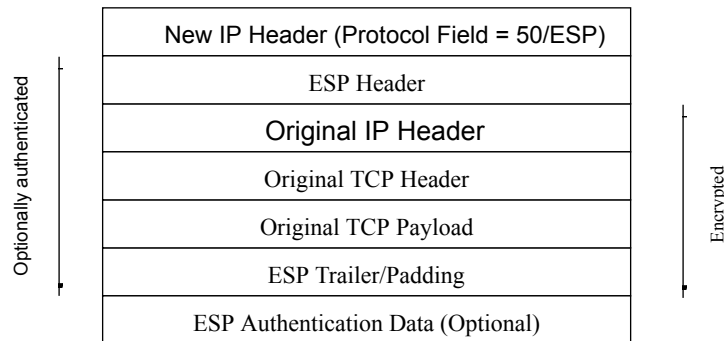
ESP Encapsulated Datagram
