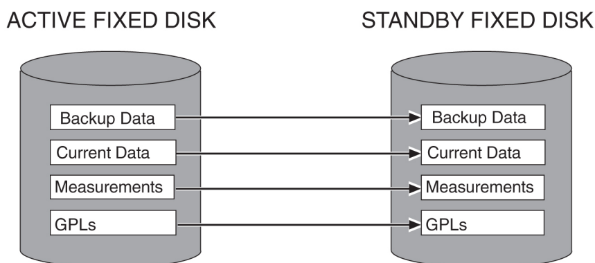
Figure 11: Action of the Copy Disk Procedure
