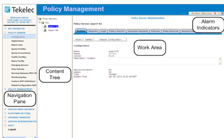
Figure 3: Structure of the CMP GUI
