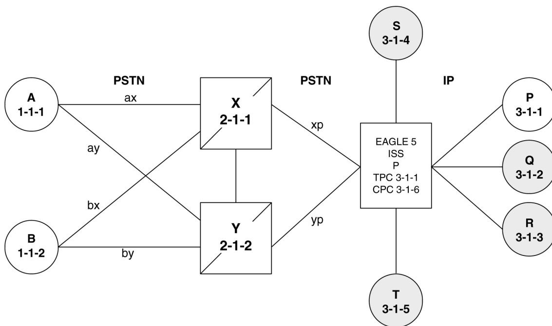
Figure 86: The EAGLE 5 ISS Simultaneously Acts as STP and End Office
