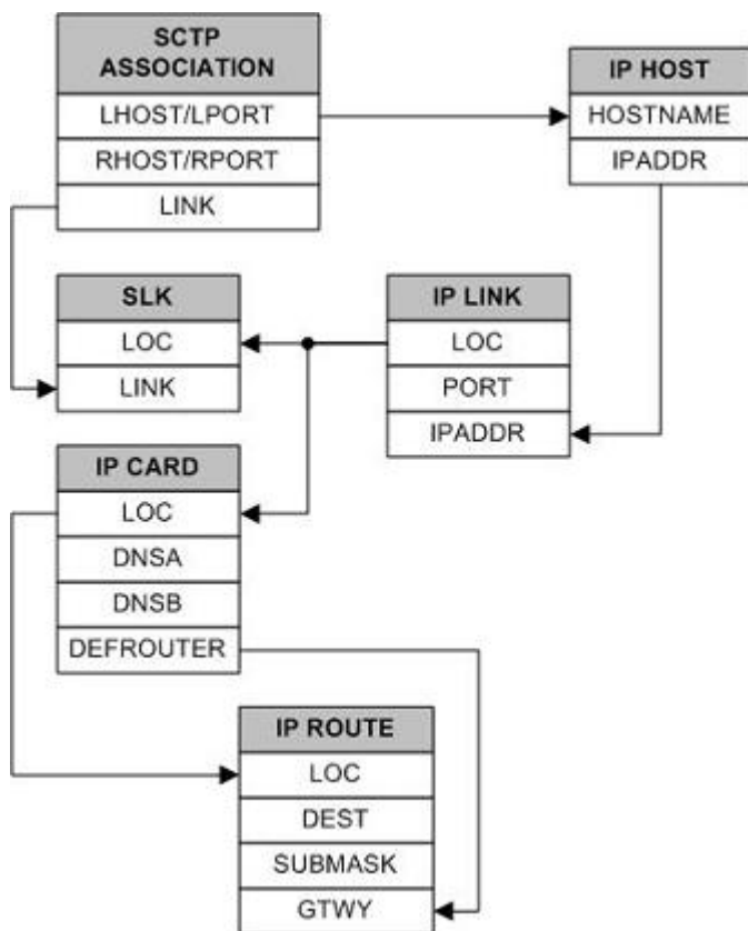
Figure 3: SCTP Association Database Relationships
