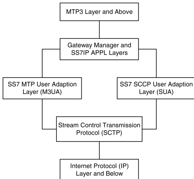
Figure 18: IPGWx Protocol Stack with SCTP as the Transport Layer
