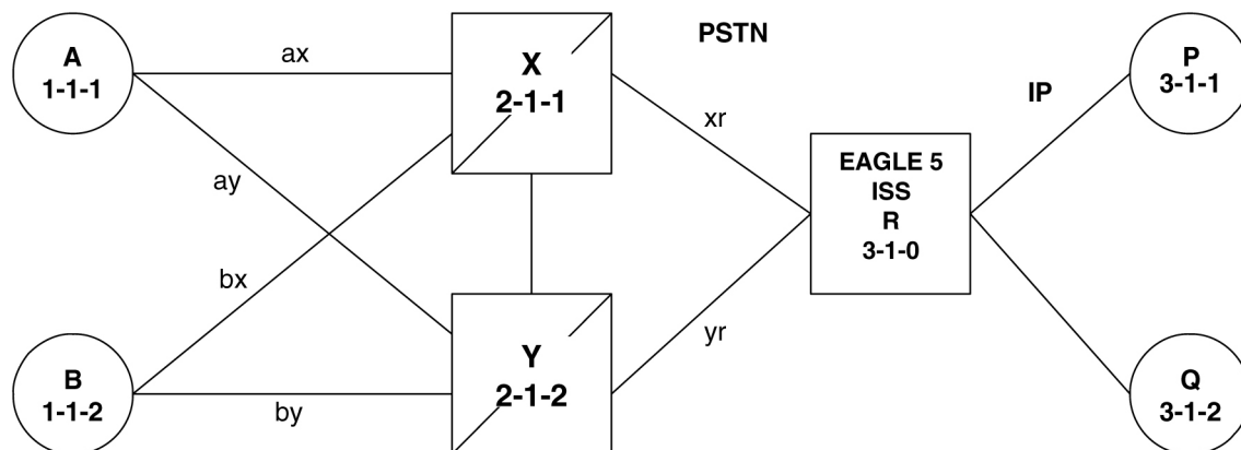
Figure 82: Original Network with Deployed EAGLE 5 ISS
