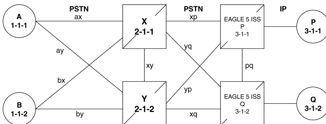
Figure 88: Mated Pair Supports Two End Office Nodes
