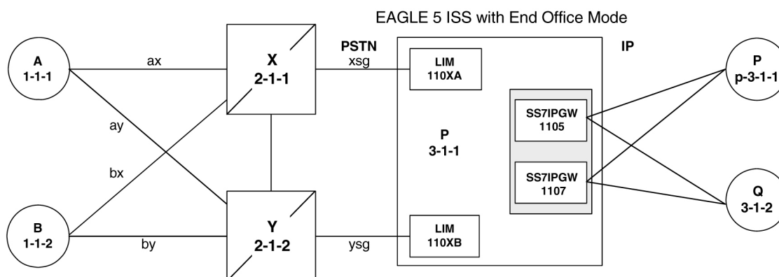
Figure 85: Network after Two Signaling End Points Migrate from PSTN to IP
