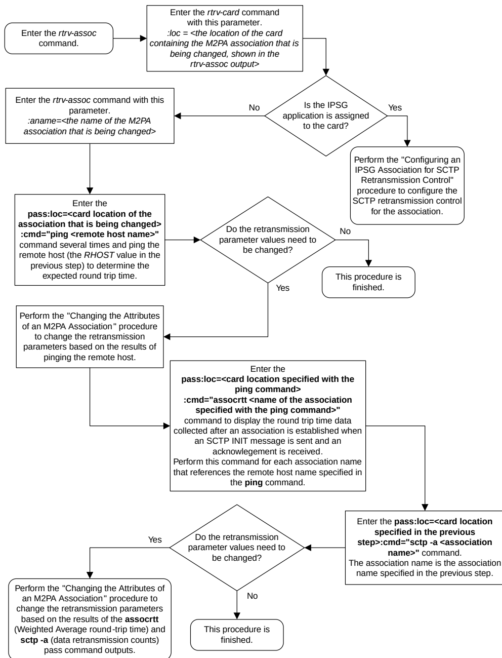
Figure 39: Configuring the SCTP Retransmission Control for a M2PA Association
