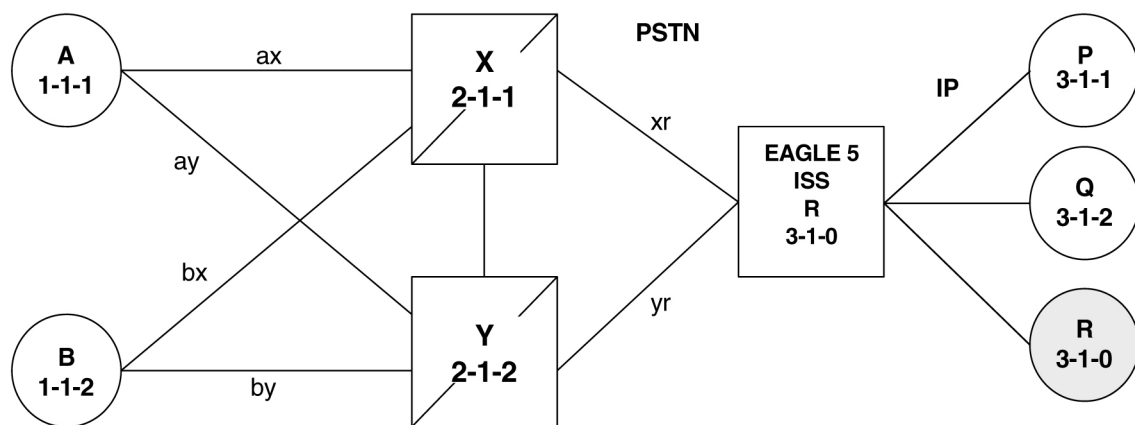
Figure 83: New Network with an EAGLE 5 ISS Using End Office and End Node R
