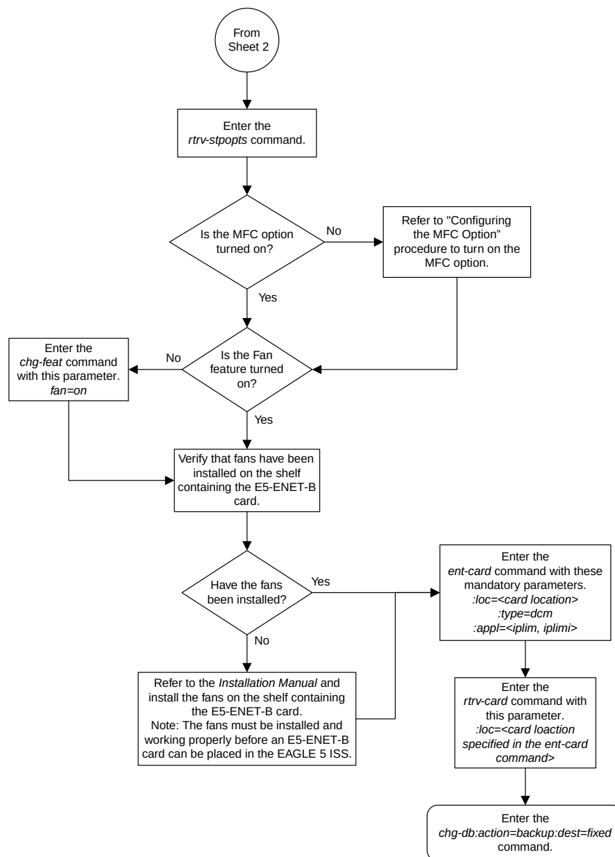
Figure 22: Adding an IPLIMx Card
