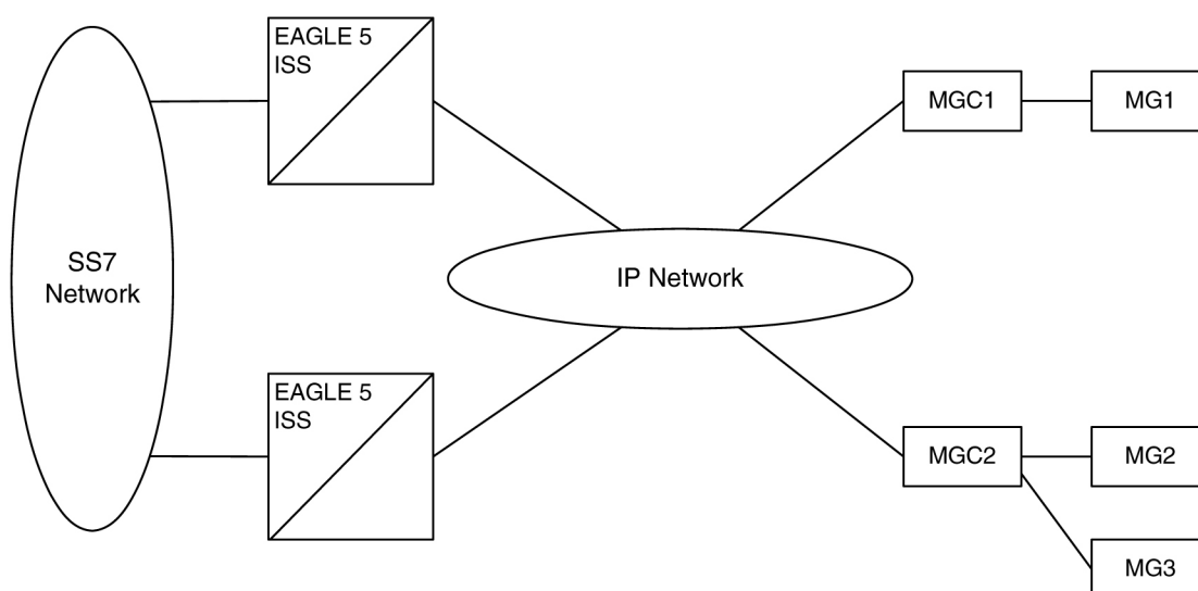
Figure 13: IP Network (SEP connectivity via ISUP, Q.BICC, and TUP-over-IP)
