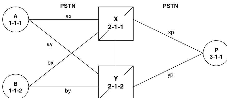
Figure 80: Network Before an EAGLE 5 ISS with End Office, Node P is to Migrate
