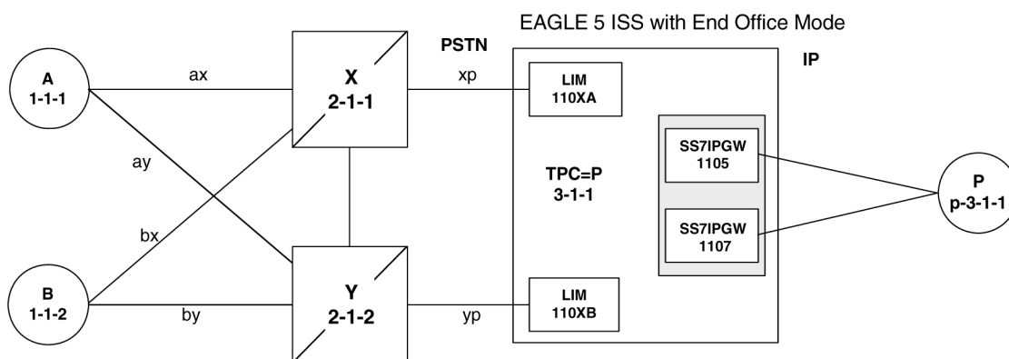
Figure 81: Network After an EAGLE 5 ISS with End Office, Node P has Migrated
