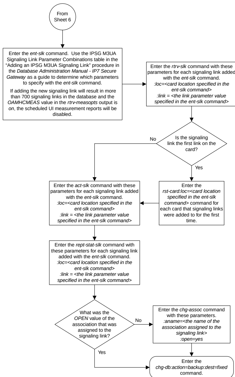
Figure 101: Adding an IPSG M3UA Signaling Link
