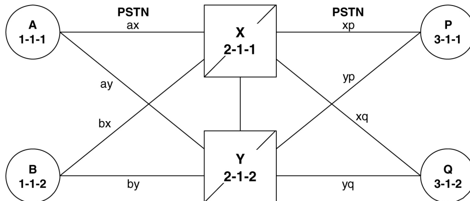
Figure 84: Network before Two Signaling End Points Migrate from PSTN to IP
