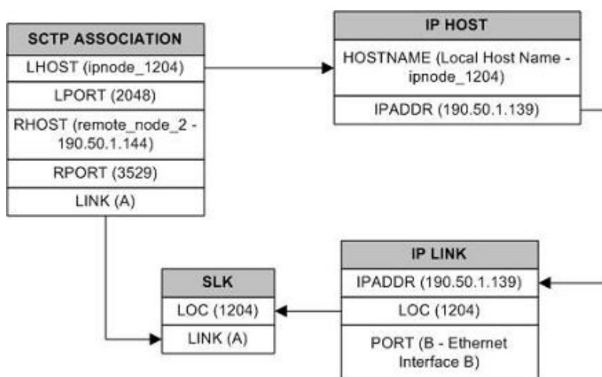
Figure 5: Typical SCTP Association Configuration
