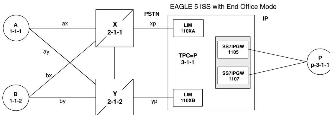
Figure 79: An EAGLE 5 ISS with End Office Support and VXI Node
