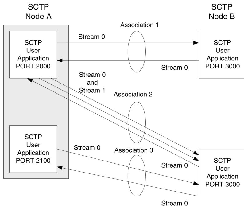
Figure 20: SCTP Connectivity
