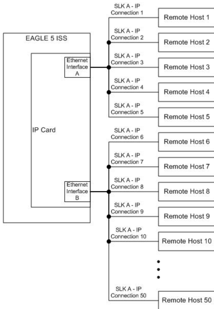
Figure 4: IP Connections using an EDCM or E5-ENET Card running the IPGWx Applications
