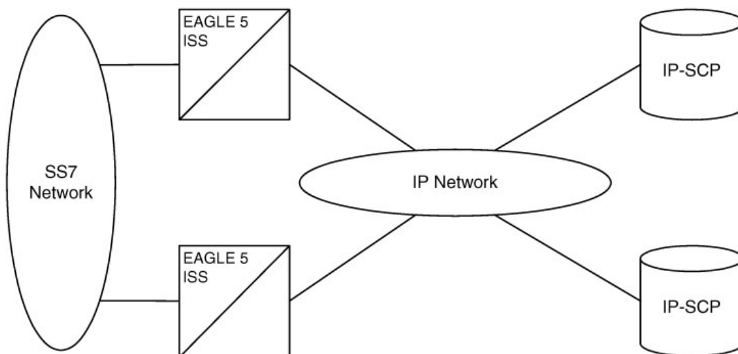
Figure 12: IP Network (SCP Connectivity via TCAP-over-IP)
