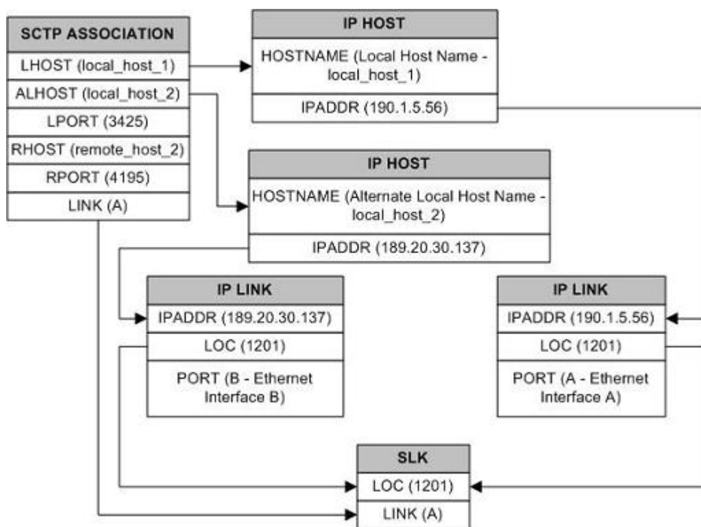
Figure 10: Multi-Homed Association Database Relationships
