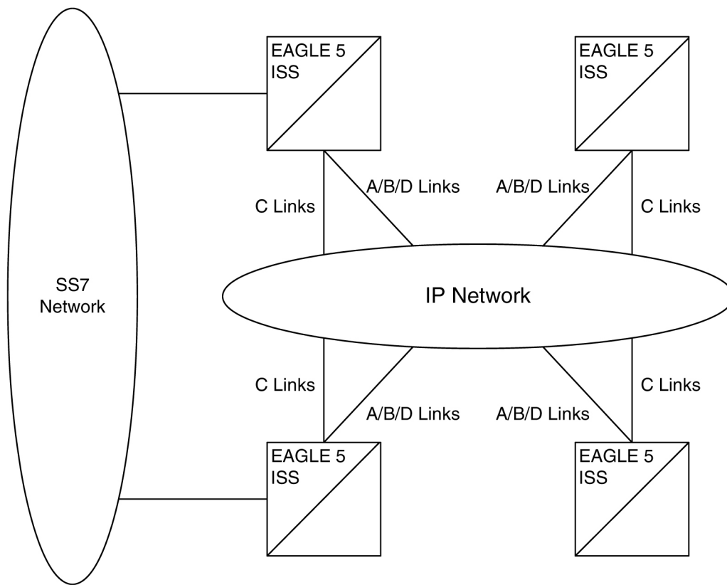
Figure 11: EAGLE 5 ISS Network (STP Connectivity via MTP-over-IP)
