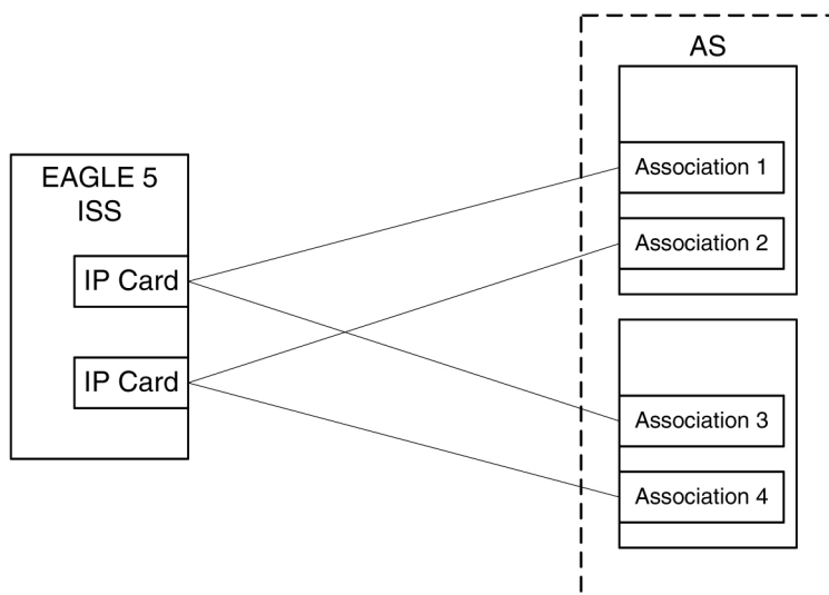
Figure 15: AS/Association Relationship
