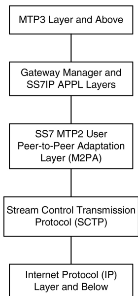
Figure 17: IPLIMx Protocol Stack with SCTP as the Transport Layer
