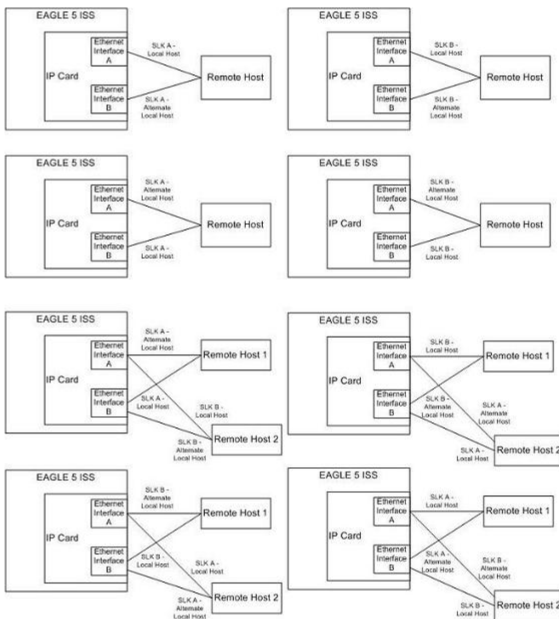
Figure 8: Multi-Homed Associations on EDCMs or E5-ENET Cards running the IPLIMx Applications
