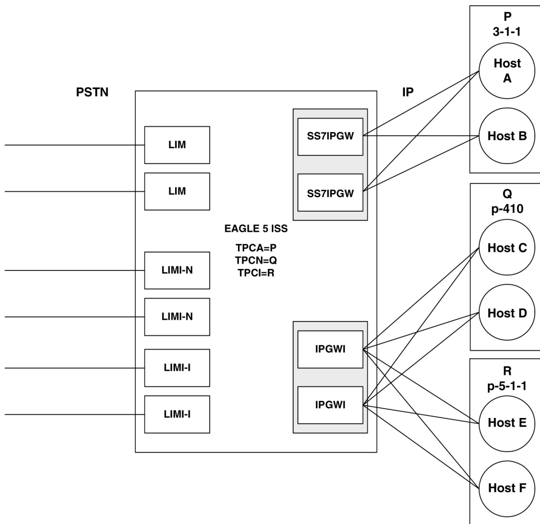
Figure 87: Three Multiple-Element End Office Nodes
