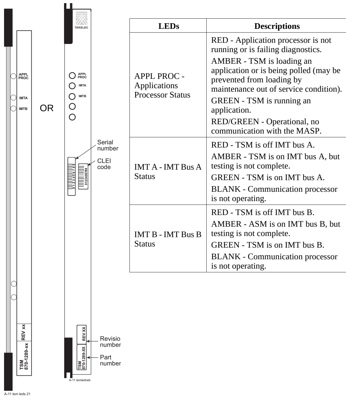
Figure A-11. TSM LEDs
