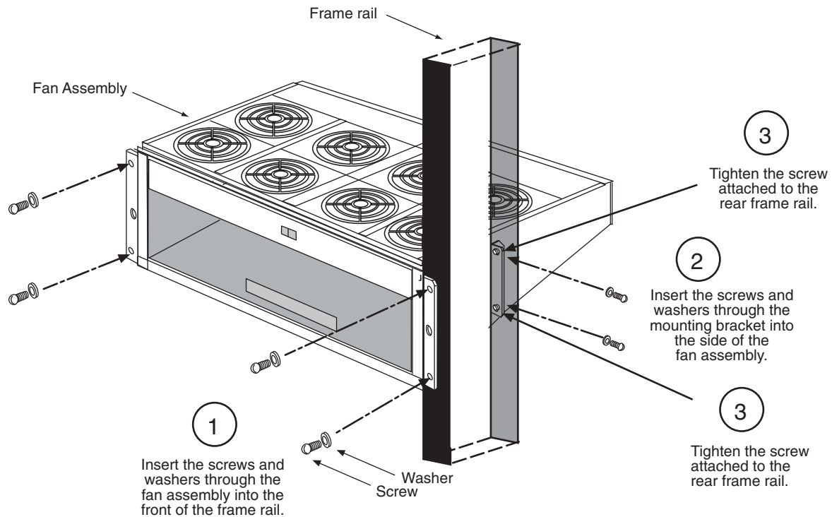
Figure A-35. Attach Fan Assembly to Front of Frame Rail
