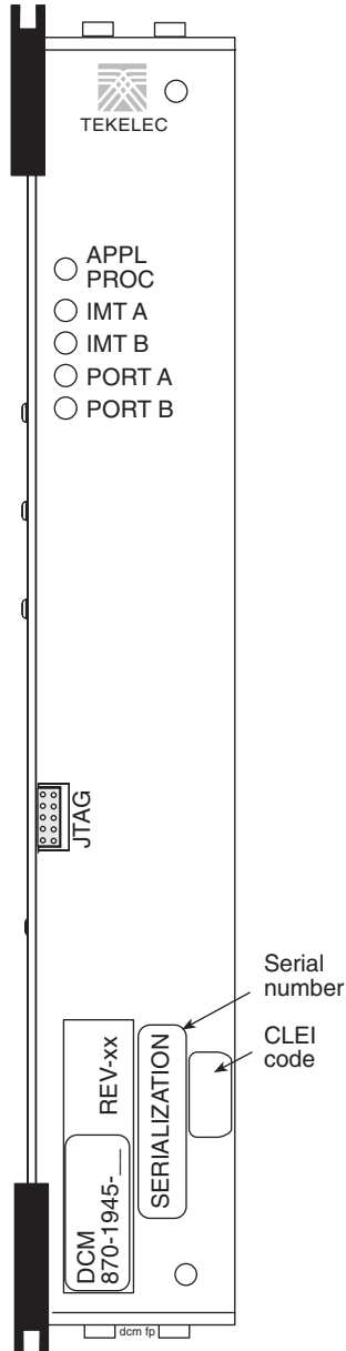
Figure A-13. DCM and DSM LEDs
