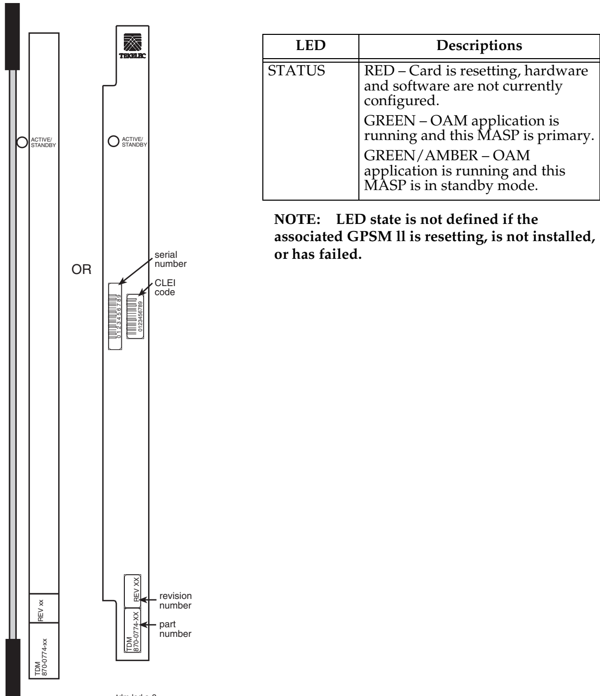
Figure A-15. TDM LED
