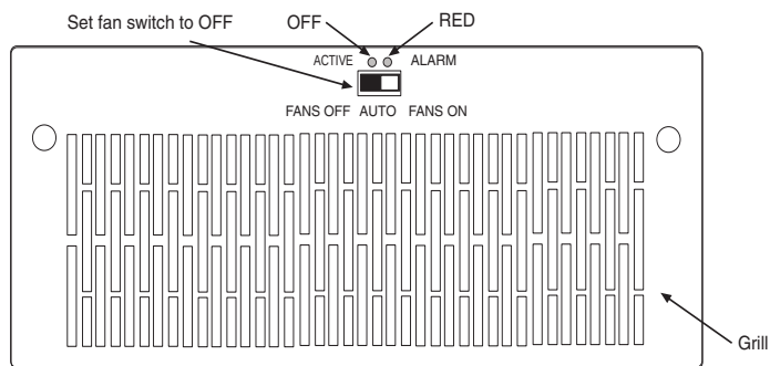
Figure A-30. Set Fan Switch to OFF
