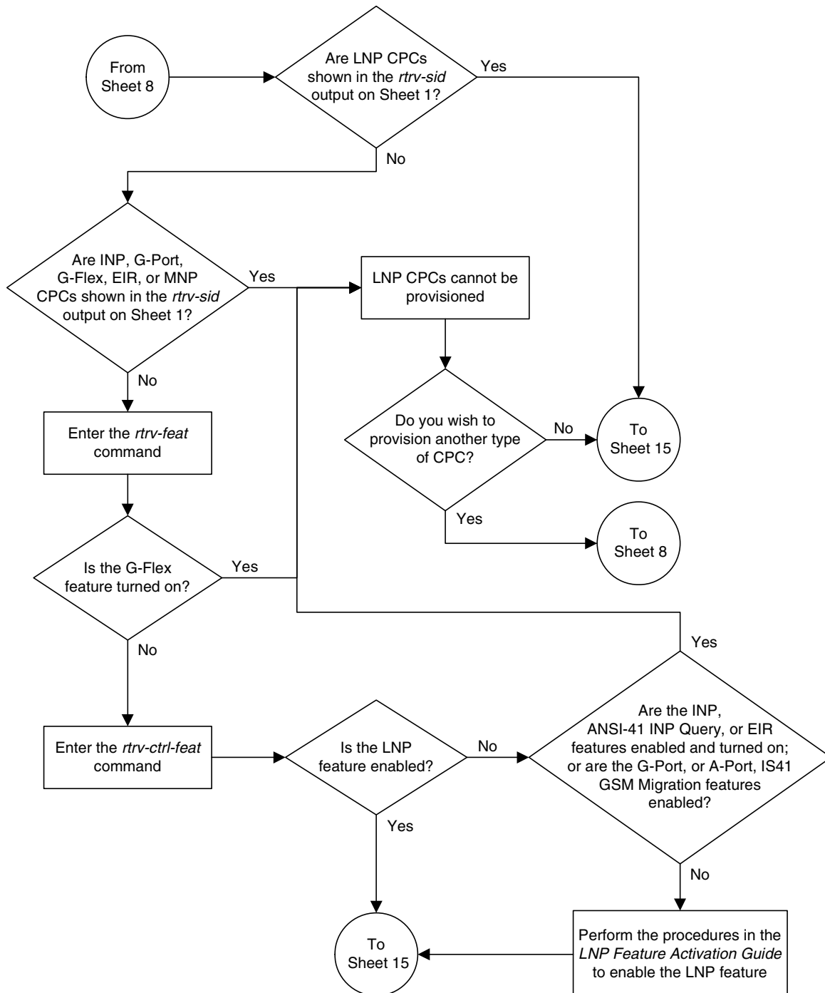
Flowchart 2-7. Changing the Self-Identification of the EAGLE 5 ISS (Sheet 14 of 18)
