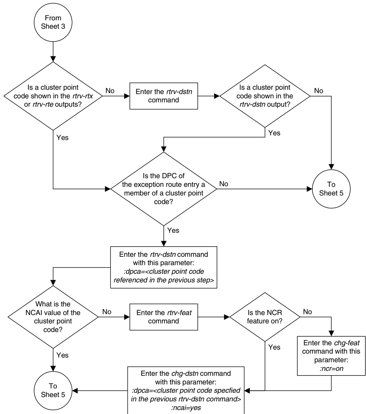
Flowchart 3-31. Adding an Exception Route Entry (Sheet 4 of 8)
