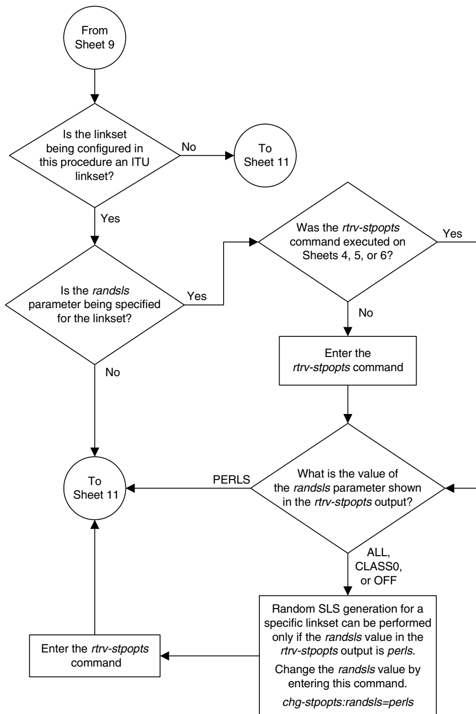
Flowchart 3-2. Adding an SS7 Linkset (Sheet 10 of 13)
