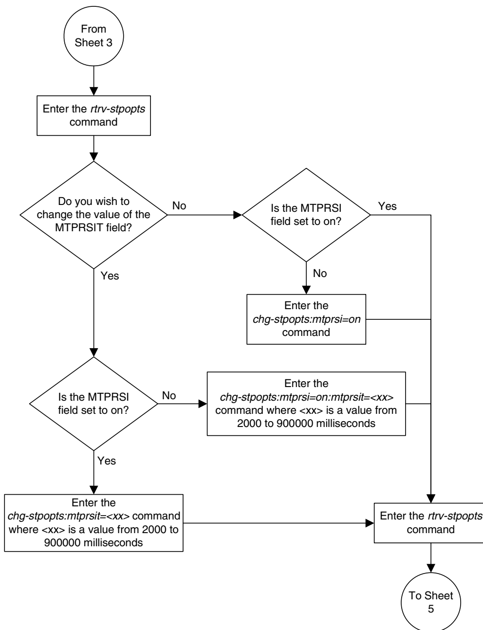
Flowchart 3-4. Changing an SS7 Linkset (Sheet 4 of 16)
