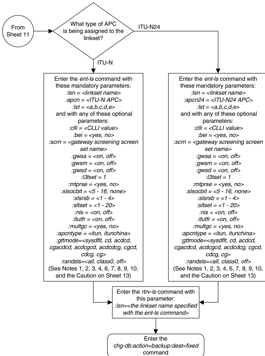
Flowchart 3-2. Adding an SS7 Linkset (Sheet 12 of 13)
