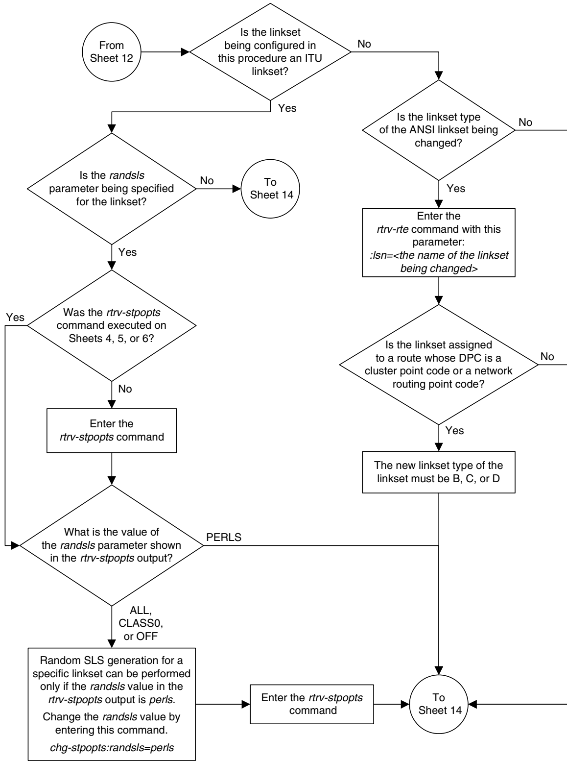
Flowchart 3-4. Changing an SS7 Linkset (Sheet 13 of 16)
