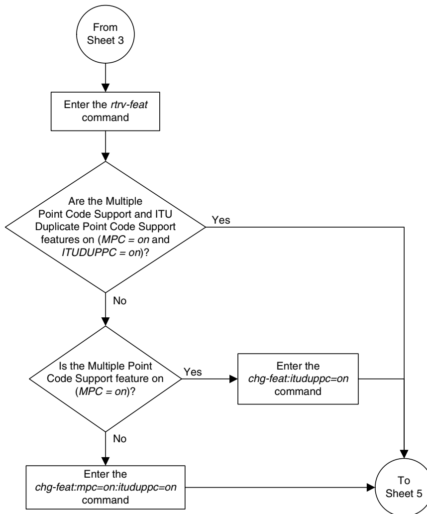
Flowchart 2-7. Changing the Self-Identification of the EAGLE 5 ISS (Sheet 4 of 18)
