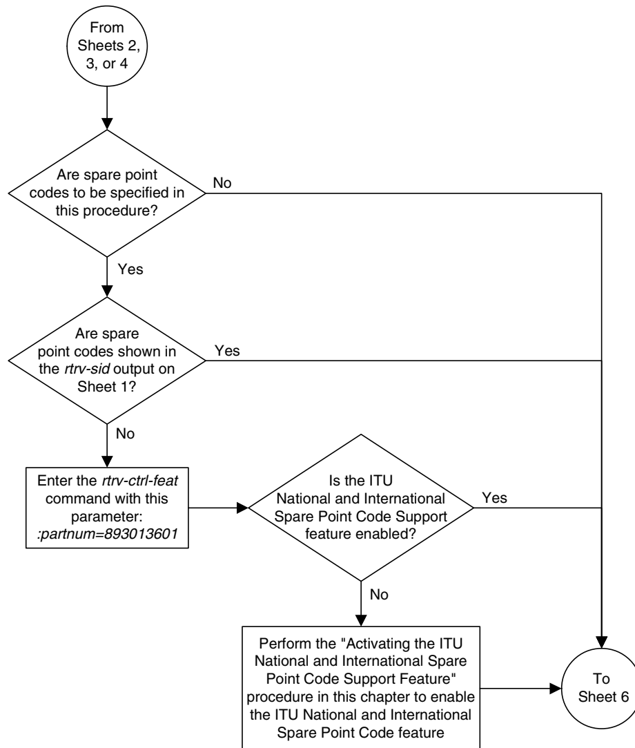
Flowchart 2-7. Changing the Self-Identification of the EAGLE 5 ISS (Sheet 5 of 18)
