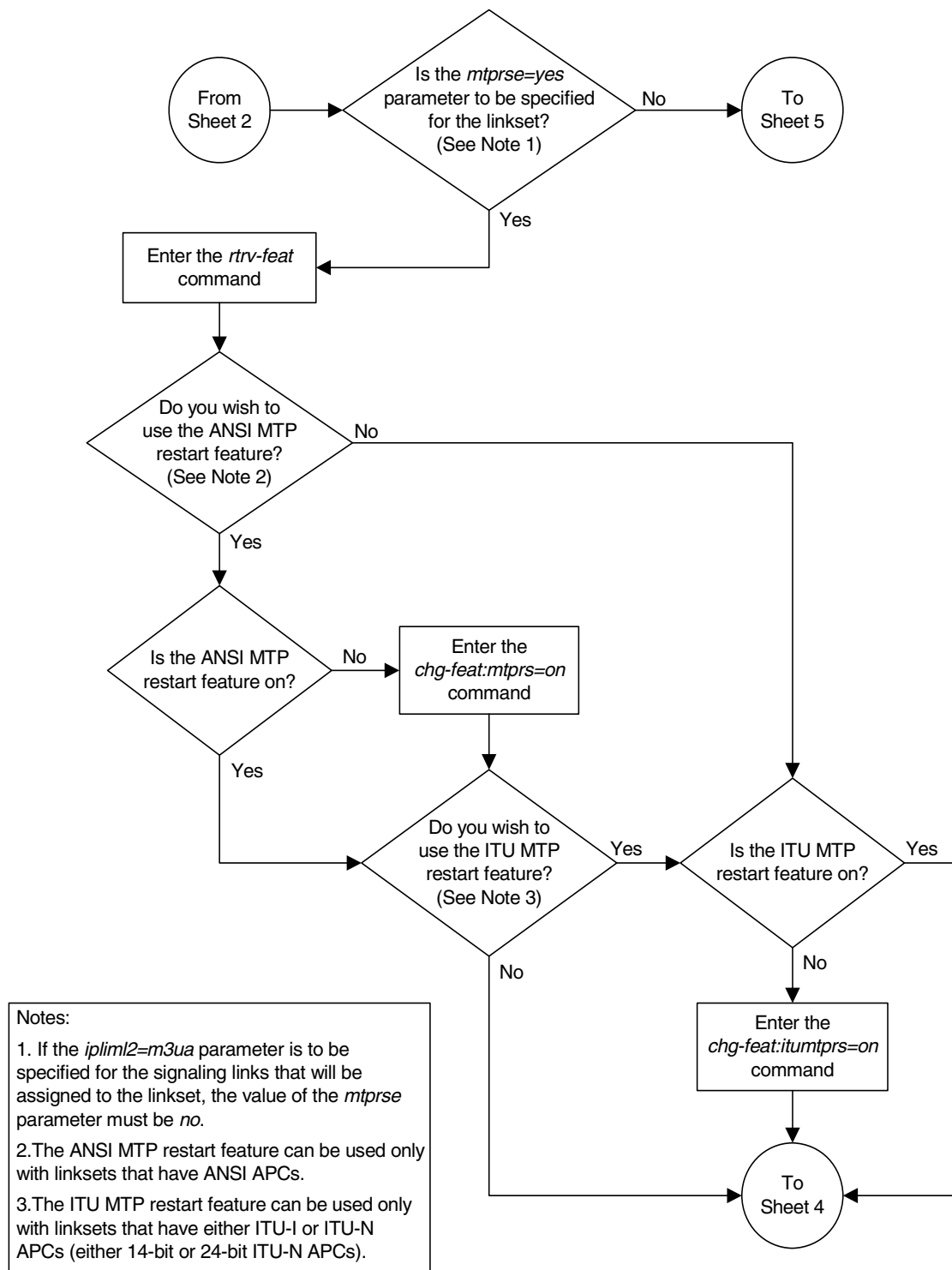
Flowchart 3-2. Adding an SS7 Linkset (Sheet 3 of 13)
