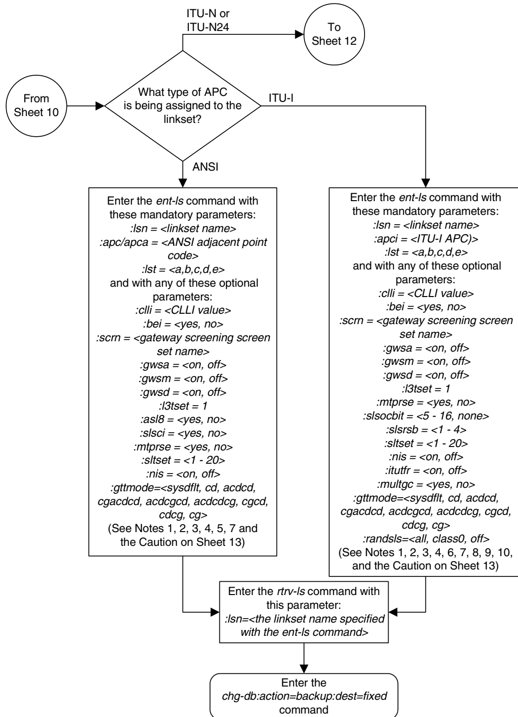
Flowchart 3-2. Adding an SS7 Linkset (Sheet 11 of 13)
