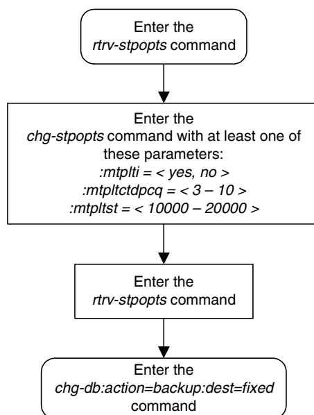
Flowchart 3-17. Configuring the System to Detect Circular Routing
