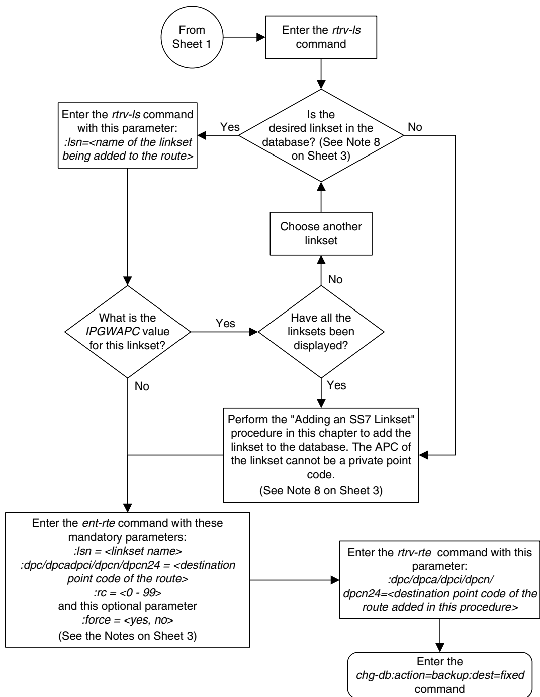
Flowchart 3-8. Adding a Route Containing an SS7 DPC (Sheet 2 of 3)
