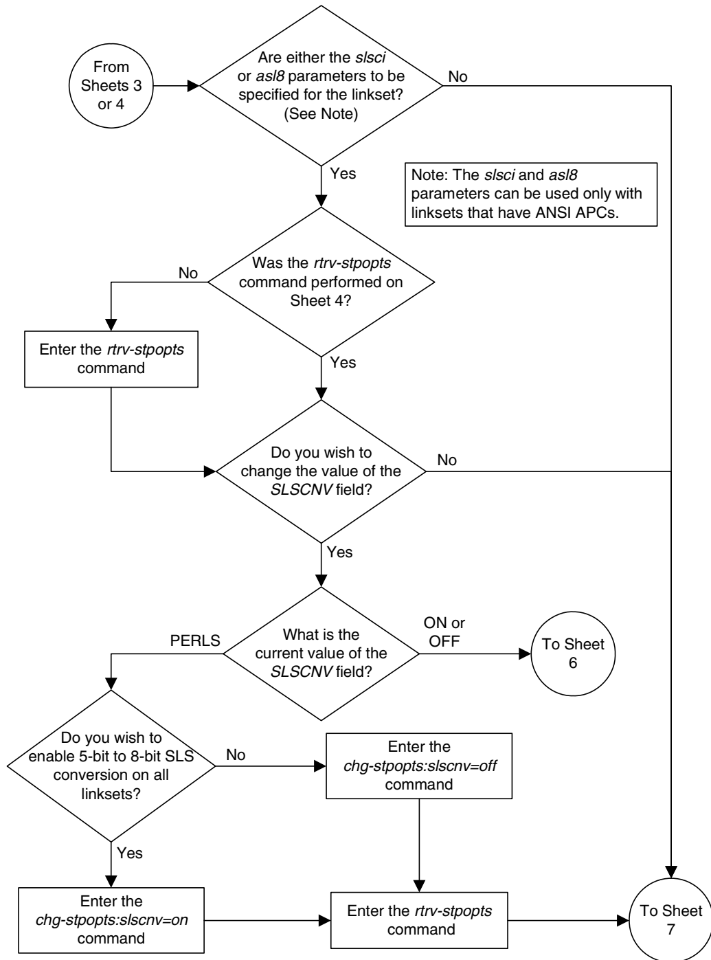
Flowchart 3-4. Changing an SS7 Linkset (Sheet 5 of 16)
