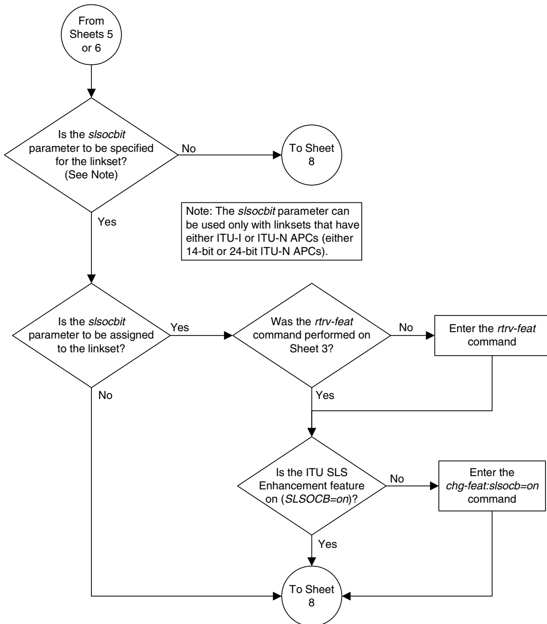
Flowchart 3-2. Adding an SS7 Linkset (Sheet 7 of 13)
