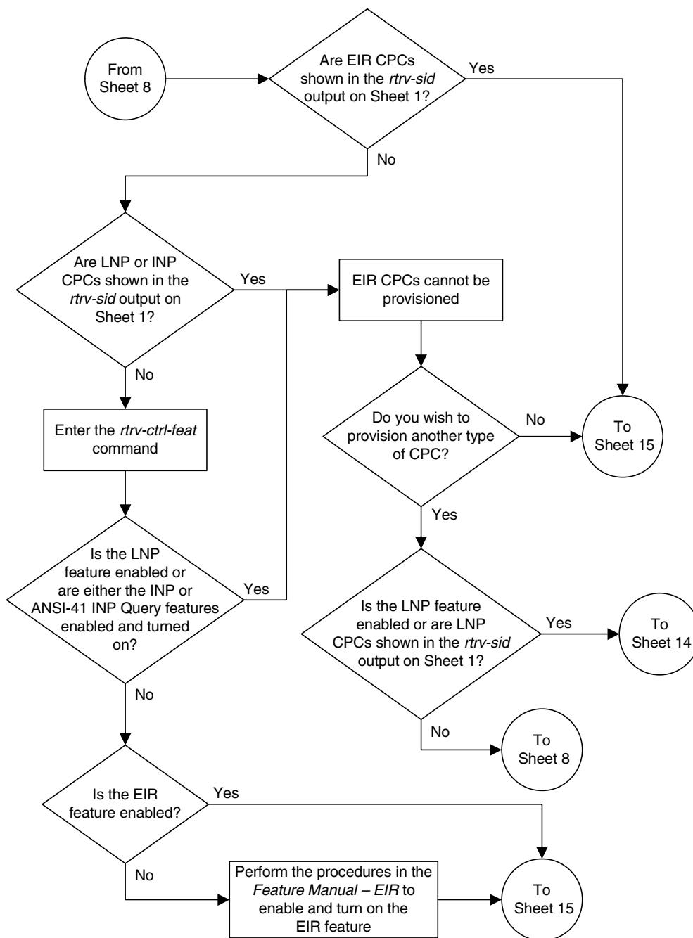
Flowchart 2-7. Changing the Self-Identification of the EAGLE 5 ISS (Sheet 12 of 18)
