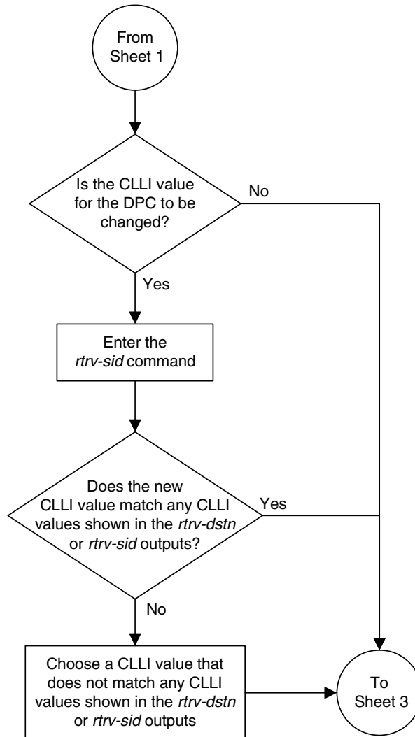
Flowchart 2-13. Changing a Destination Point Code (Sheet 2 of 9)
