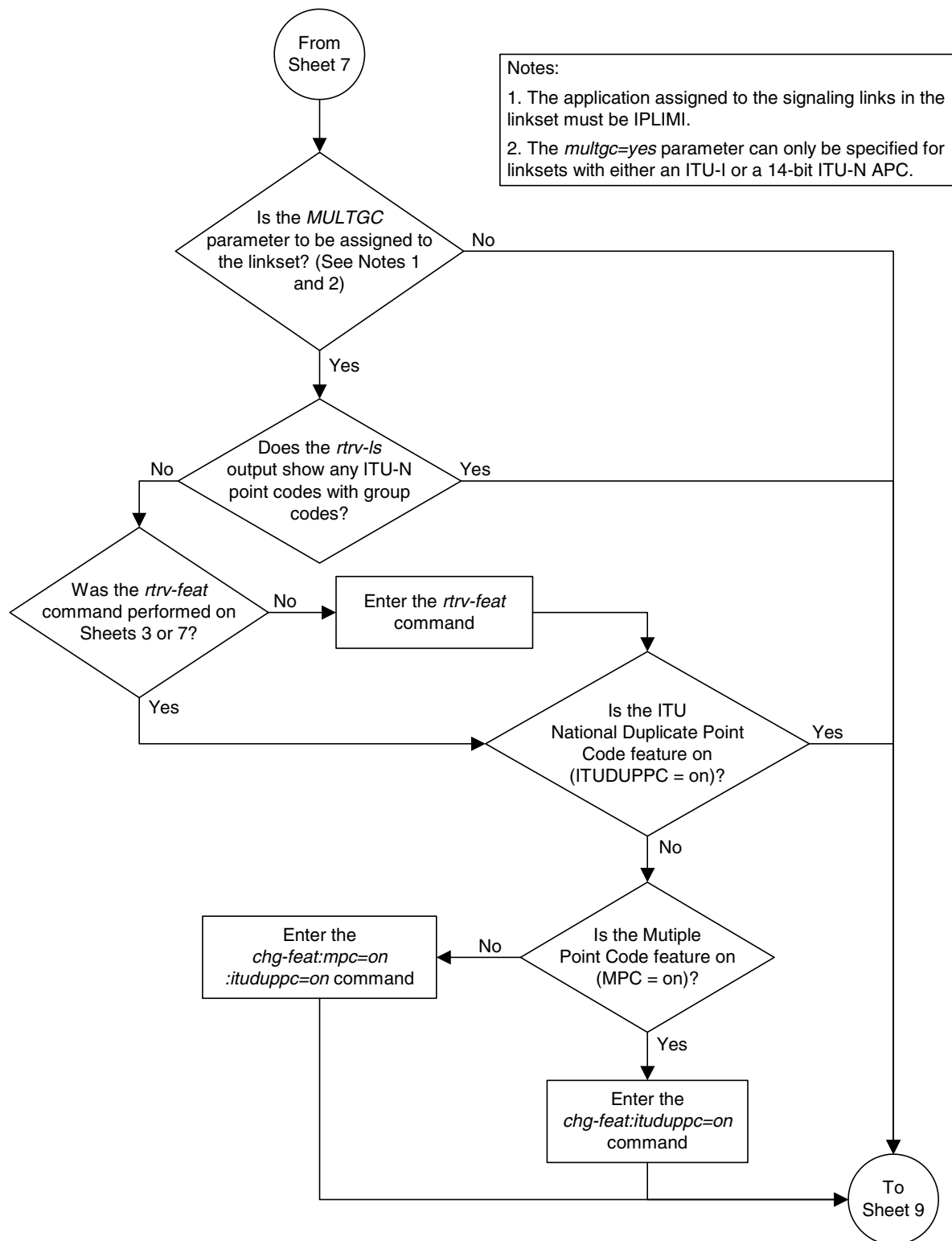
Flowchart 3-2. Adding an SS7 Linkset (Sheet 8 of 13)
