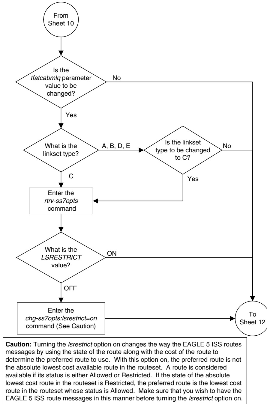
Flowchart 3-4. Changing an SS7 Linkset (Sheet 11 of 16)
