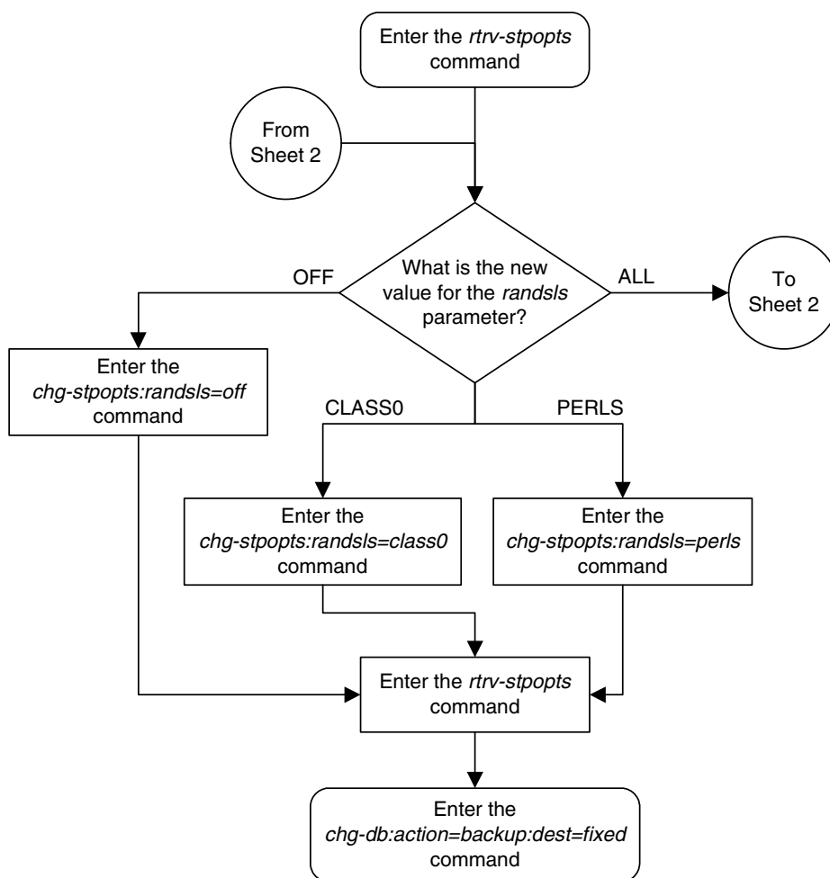
Flowchart 3-24. Configuring the System for Random SLS Generation (Sheet 1 of 2)
