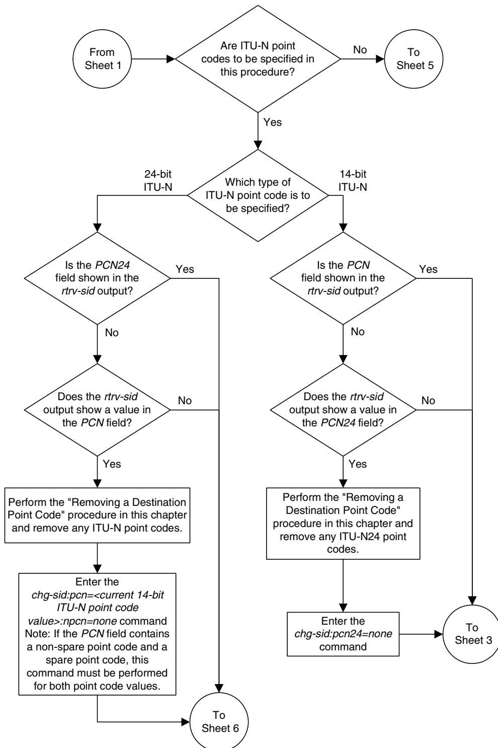
Flowchart 2-7. Changing the Self-Identification of the EAGLE 5 ISS (Sheet 2 of 18)
