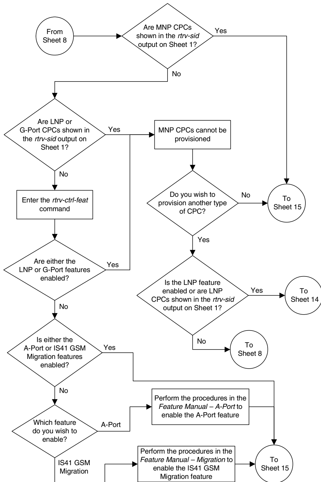
Flowchart 2-7. Changing the Self-Identification of the EAGLE 5 ISS (Sheet 13 of 18)
