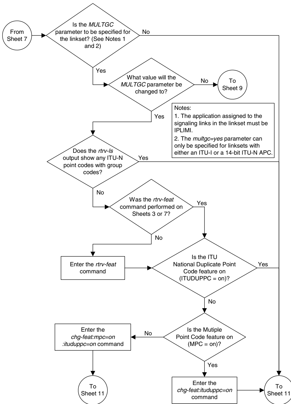
Flowchart 3-4. Changing an SS7 Linkset (Sheet 8 of 16)
