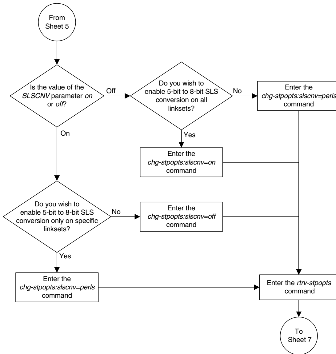
Flowchart 3-4. Changing an SS7 Linkset (Sheet 6 of 16)
