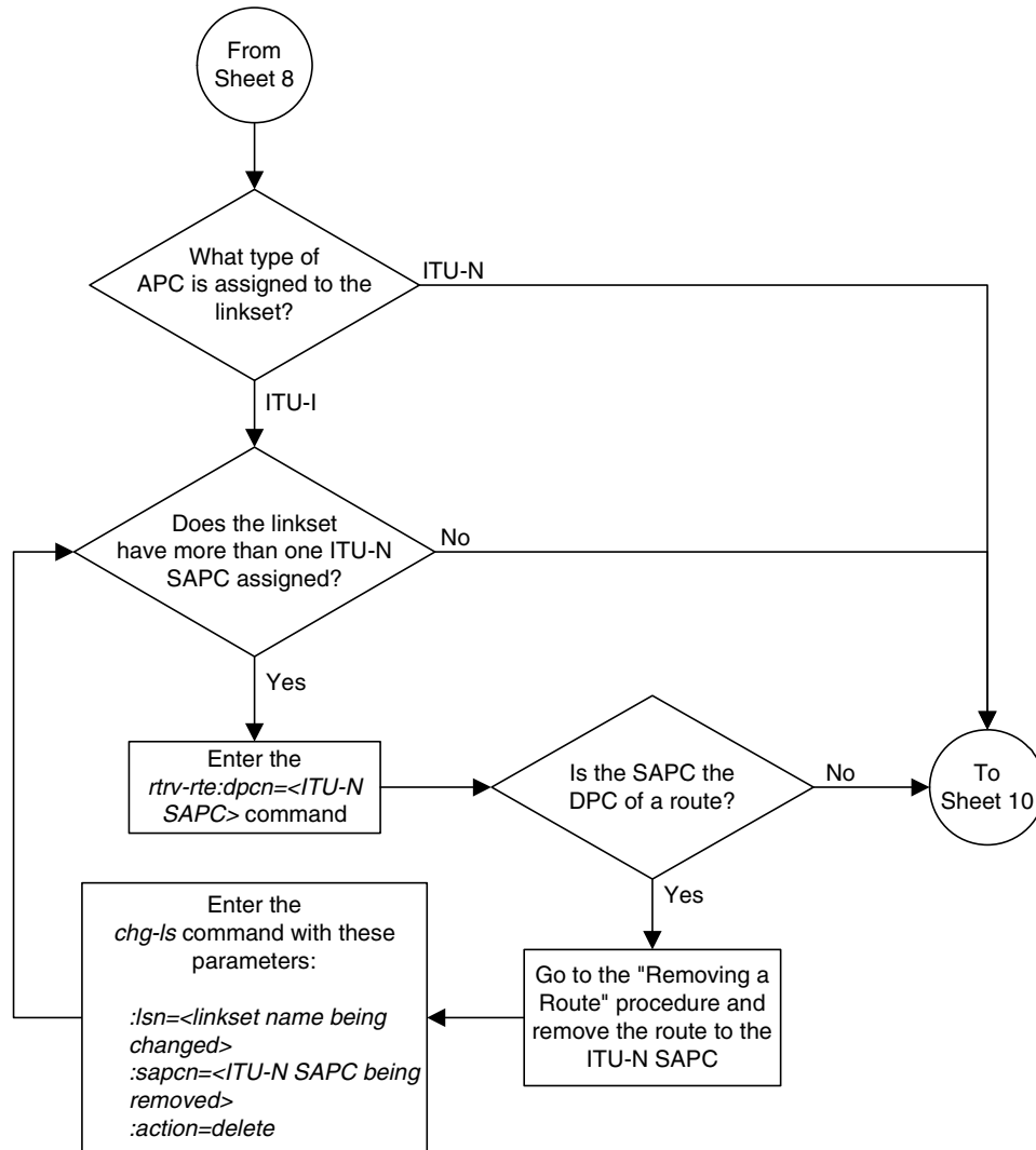
Flowchart 3-4. Changing an SS7 Linkset (Sheet 9 of 16)
