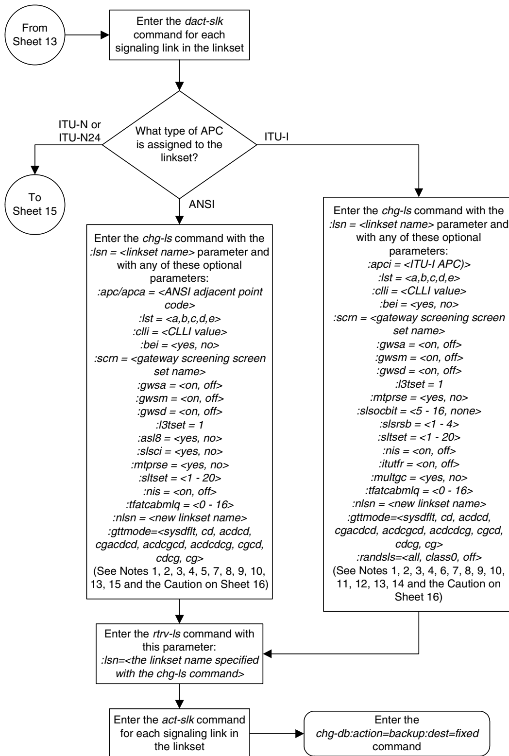
Flowchart 3-4. Changing an SS7 Linkset (Sheet 14 of 16)
