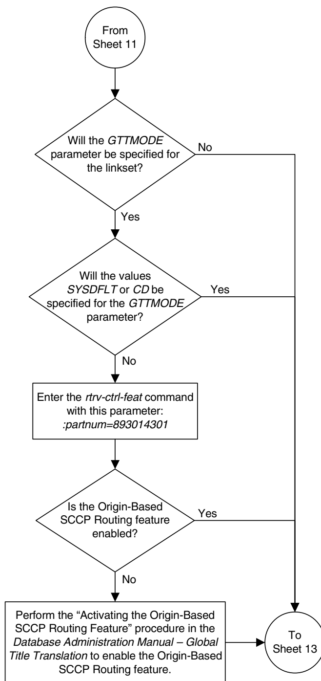
Flowchart 3-4. Changing an SS7 Linkset (Sheet 12 of 16)
