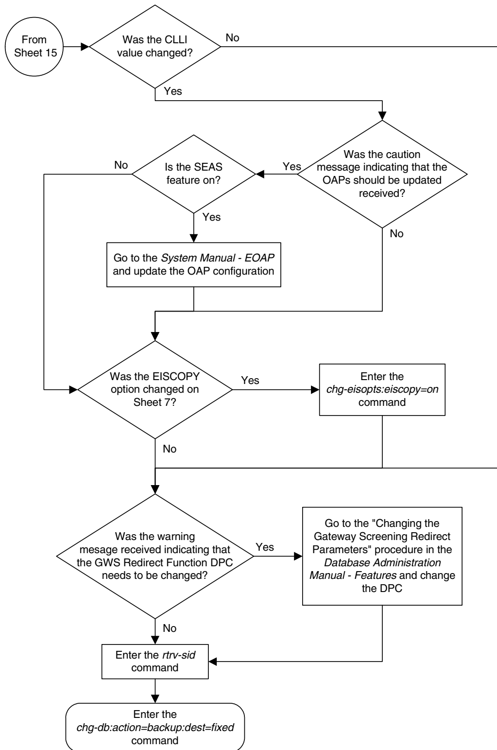
Flowchart 2-7. Changing the Self-Identification of the EAGLE 5 ISS (Sheet 16 of 18)
