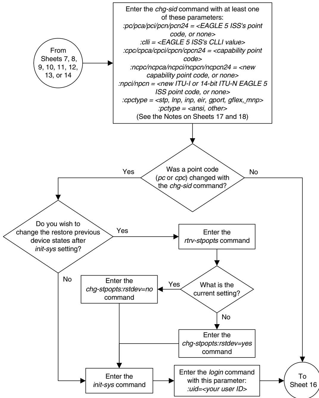
Flowchart 2-7. Changing the Self-Identification of the EAGLE 5 ISS (Sheet 15 of 18)
