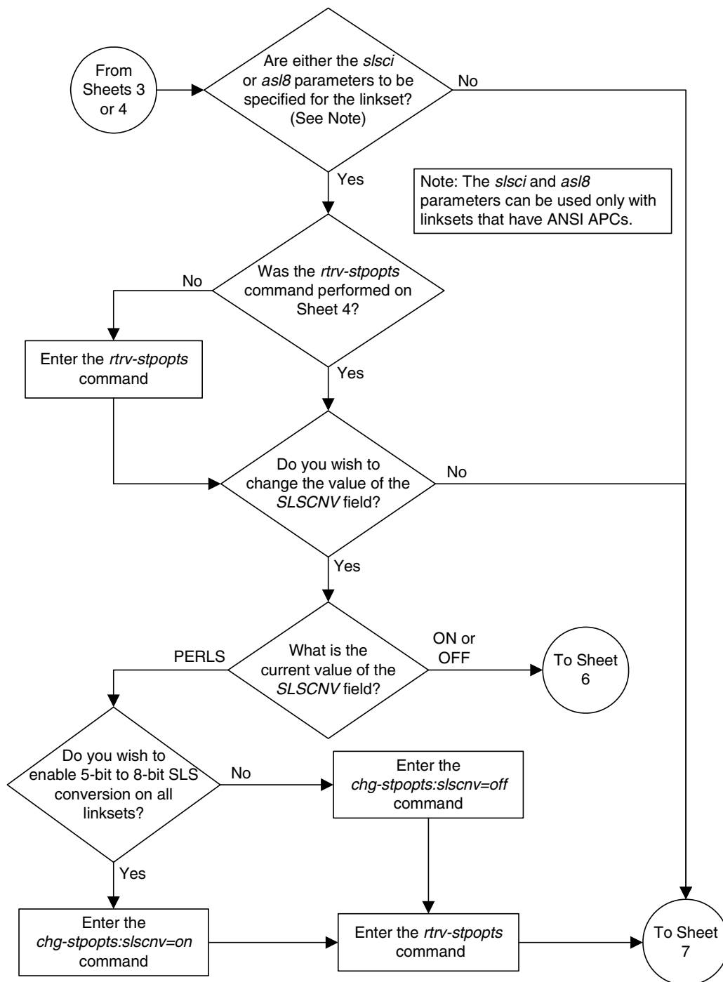
Flowchart 3-2. Adding an SS7 Linkset (Sheet 5 of 13)
