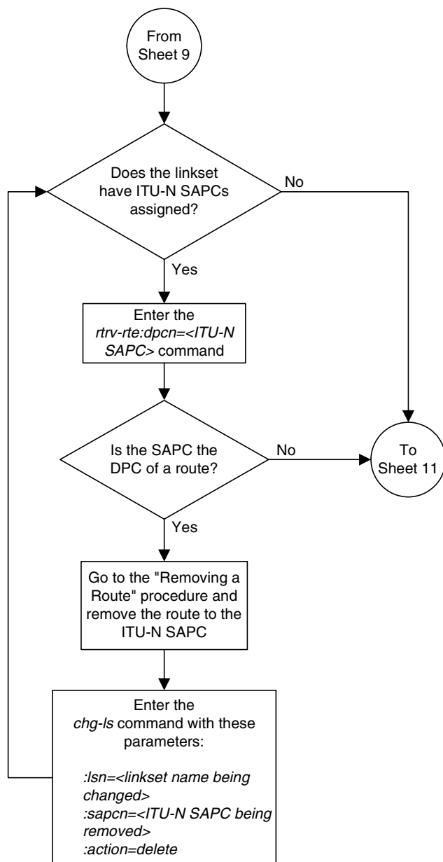
Flowchart 3-4. Changing an SS7 Linkset (Sheet 10 of 16)
