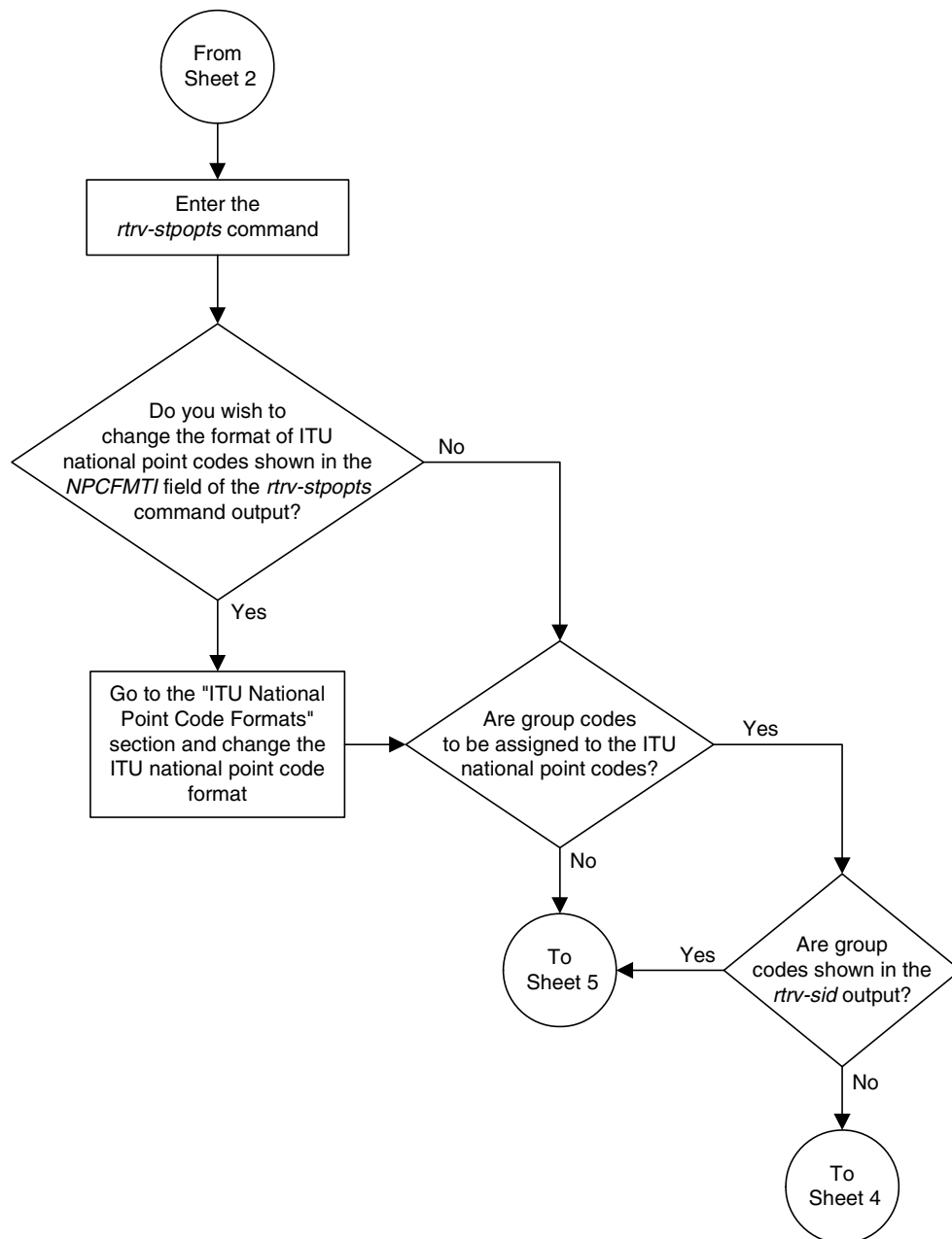
Flowchart 2-7. Changing the Self-Identification of the EAGLE 5 ISS (Sheet 3 of 18)
