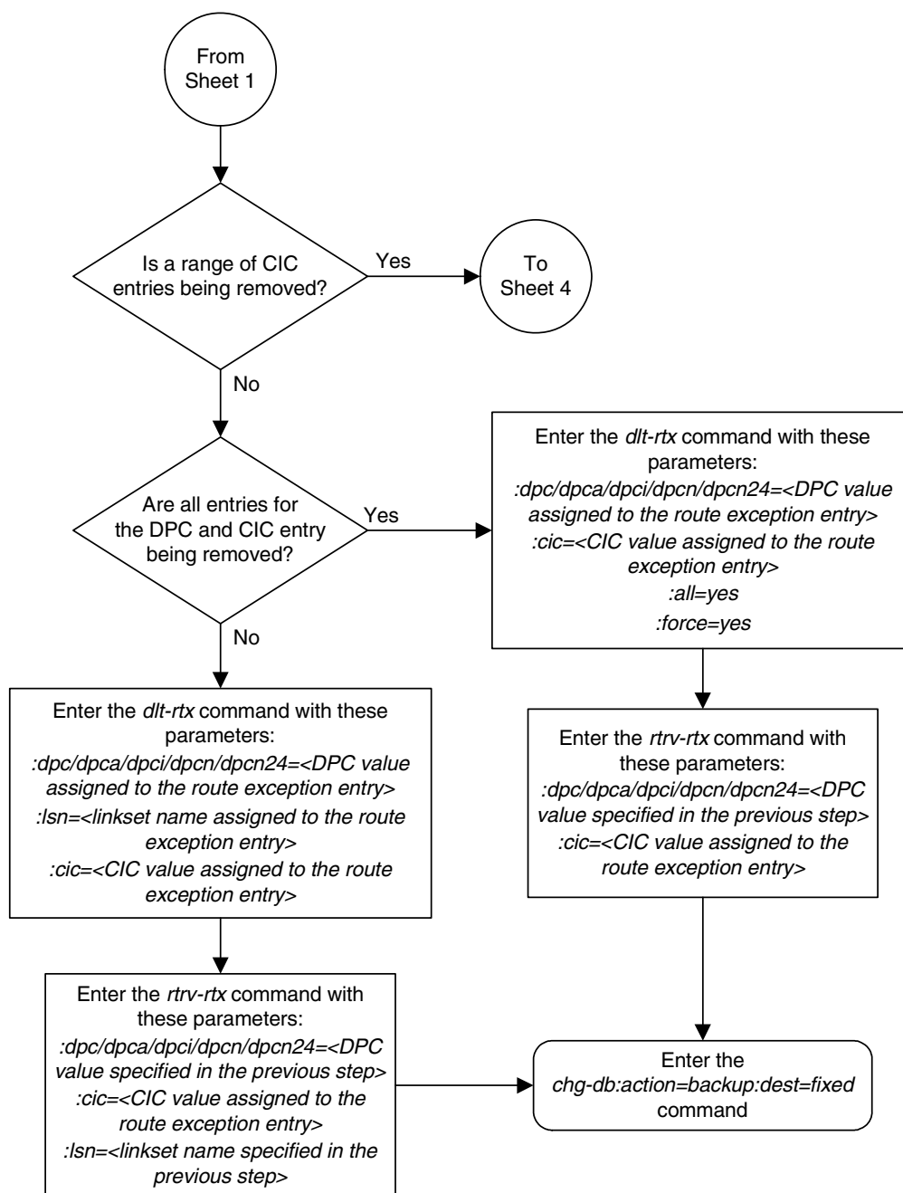
Flowchart 3-32. Removing a Route Exception Entry (Sheet 3 of 5)
