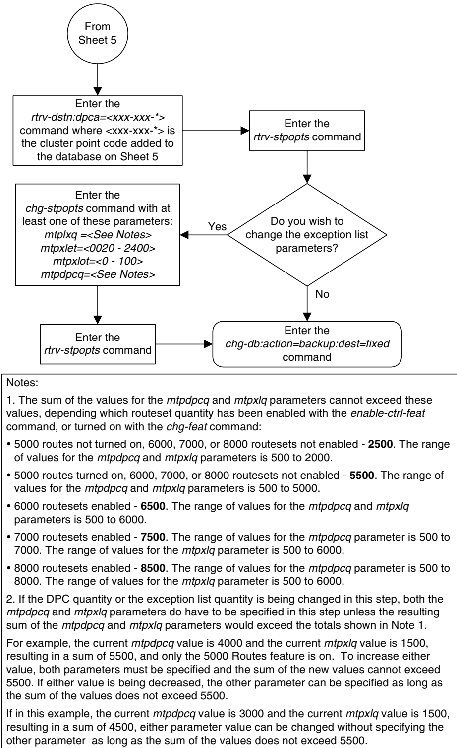
Flowchart 2-8. Adding a Cluster Point Code (Sheet 6 of 6)
