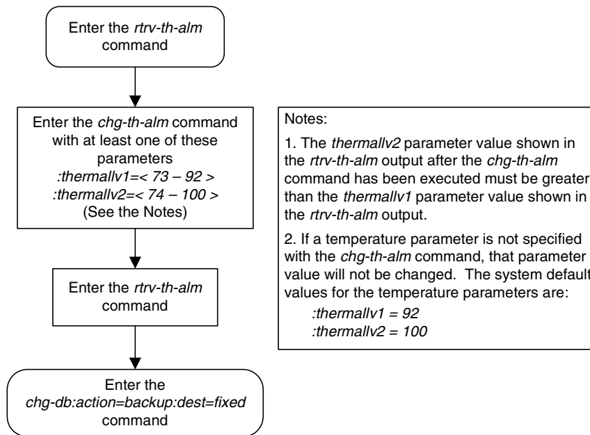
Flowchart 3-28. Changing the High-Capacity Card Temperature Alarm Thresholds
