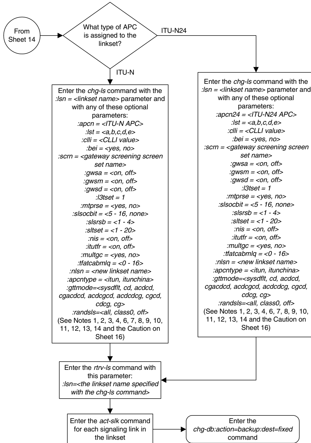
Flowchart 3-4. Changing an SS7 Linkset (Sheet 15 of 16)
