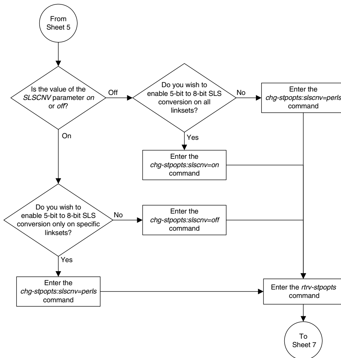
Flowchart 3-2. Adding an SS7 Linkset (Sheet 6 of 13)
