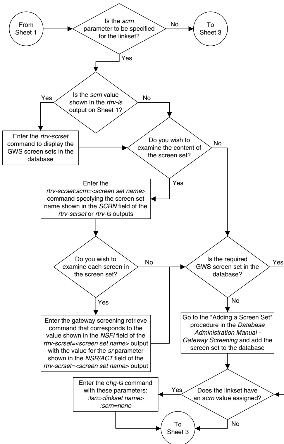
Flowchart 3-4. Changing an SS7 Linkset (Sheet 2 of 16)
