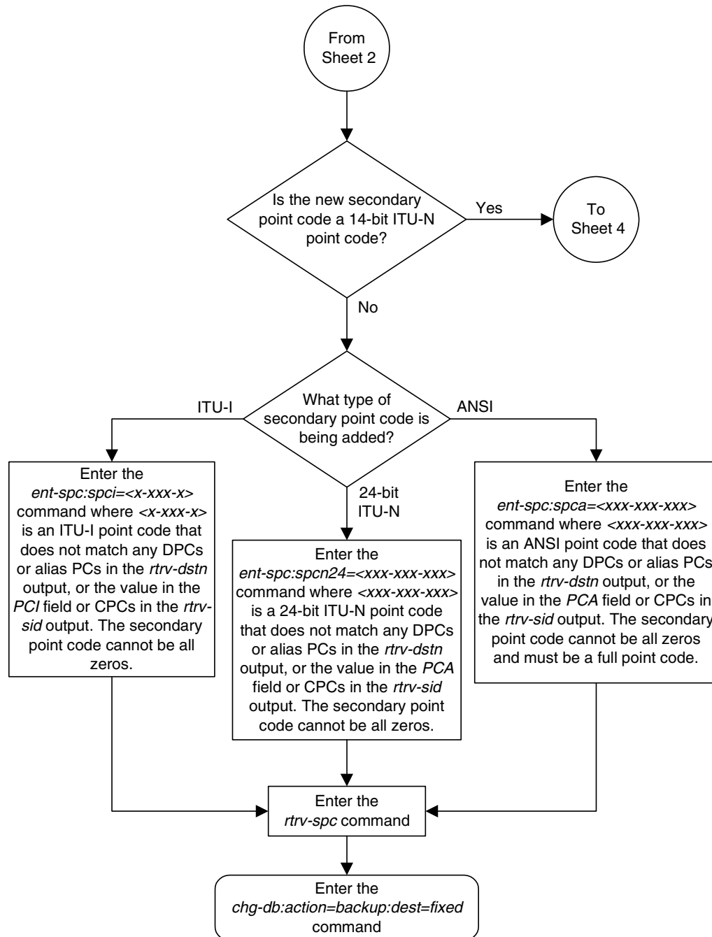
Flowchart 2-4. Adding a Secondary Point Code (Sheet 3 of 4)
