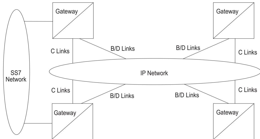
Figure 5-18. STP Connectivity via MTP over IP
