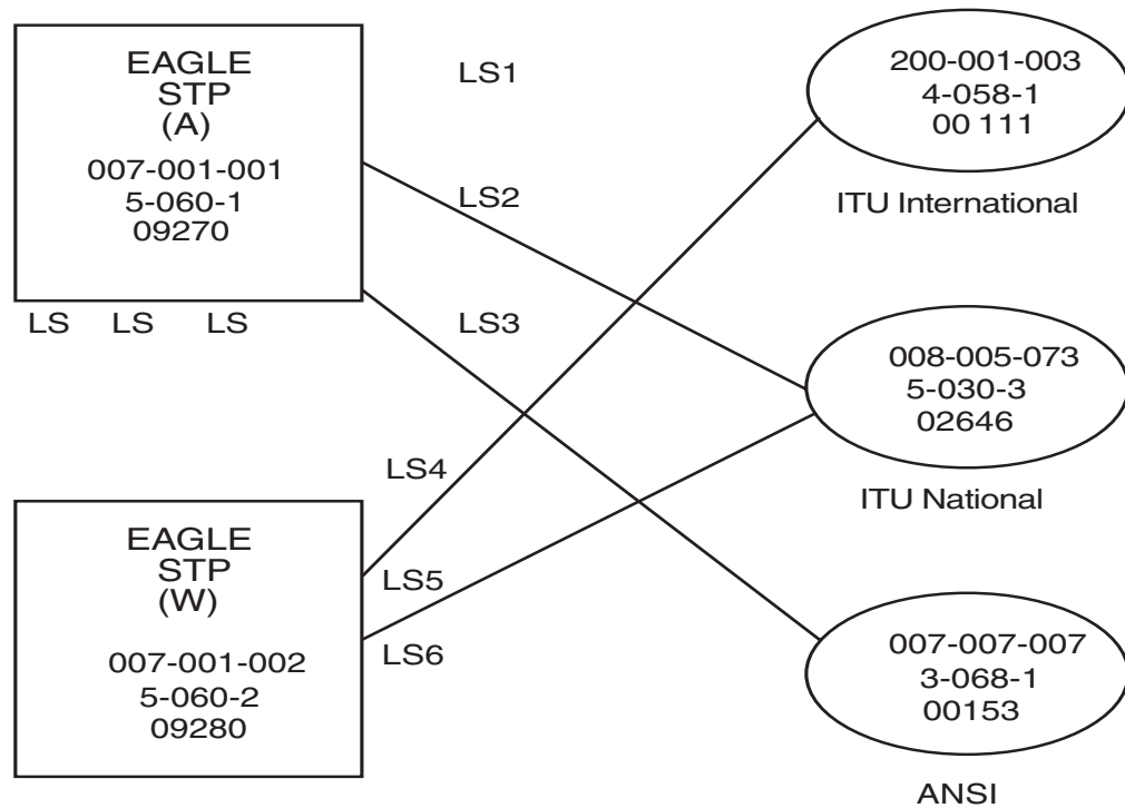
Figure 2-5. Sample Gateway STP Network
