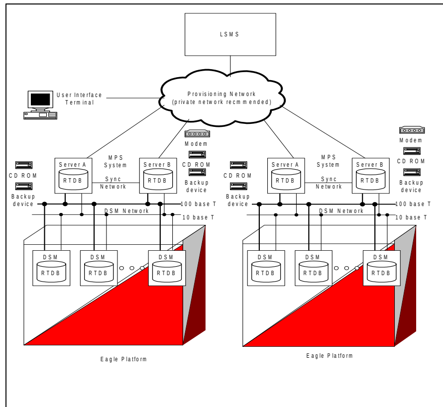
Figure 4-6. LNP 48/96 Million System Architectural Overview
