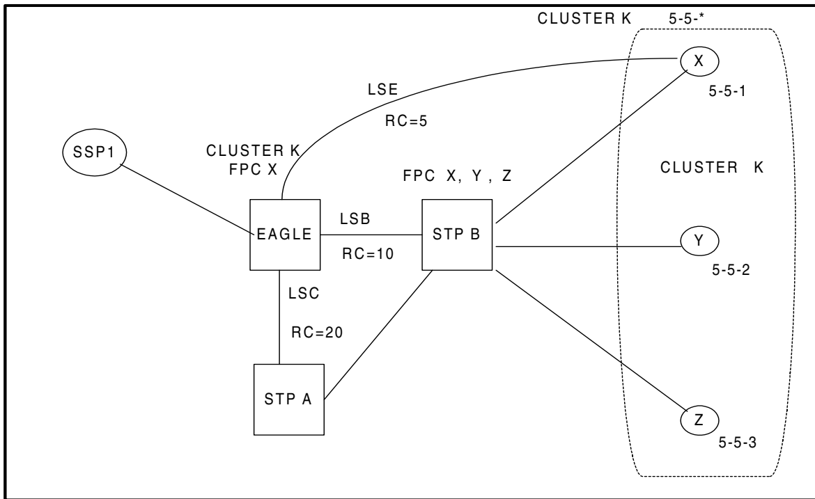
Figure 4-31. Nested Cluster Example #1
