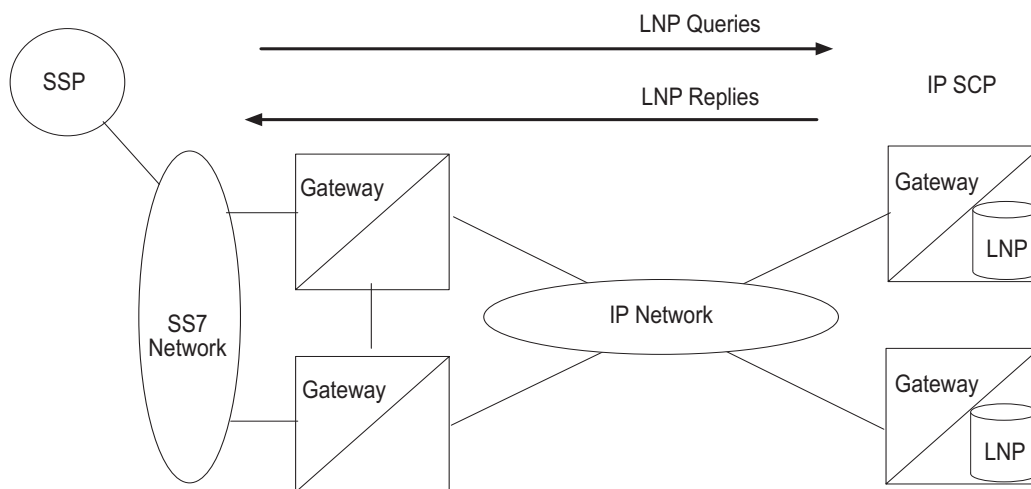
Figure 3-11. IP Connected LNP Application (Lab Only)
