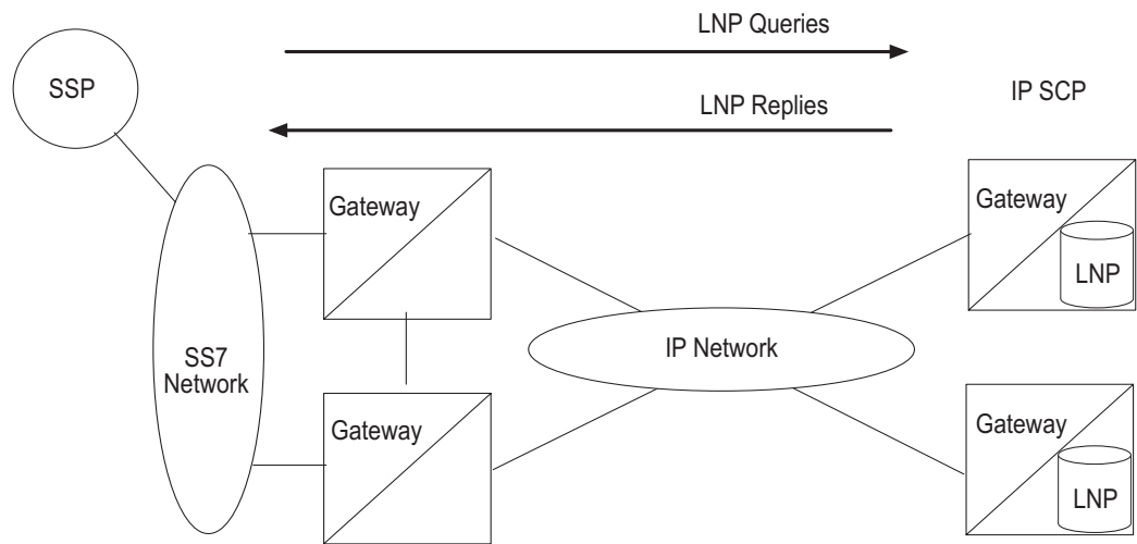
Figure 3-10. IP Connected LNP Application (Lab Only)
