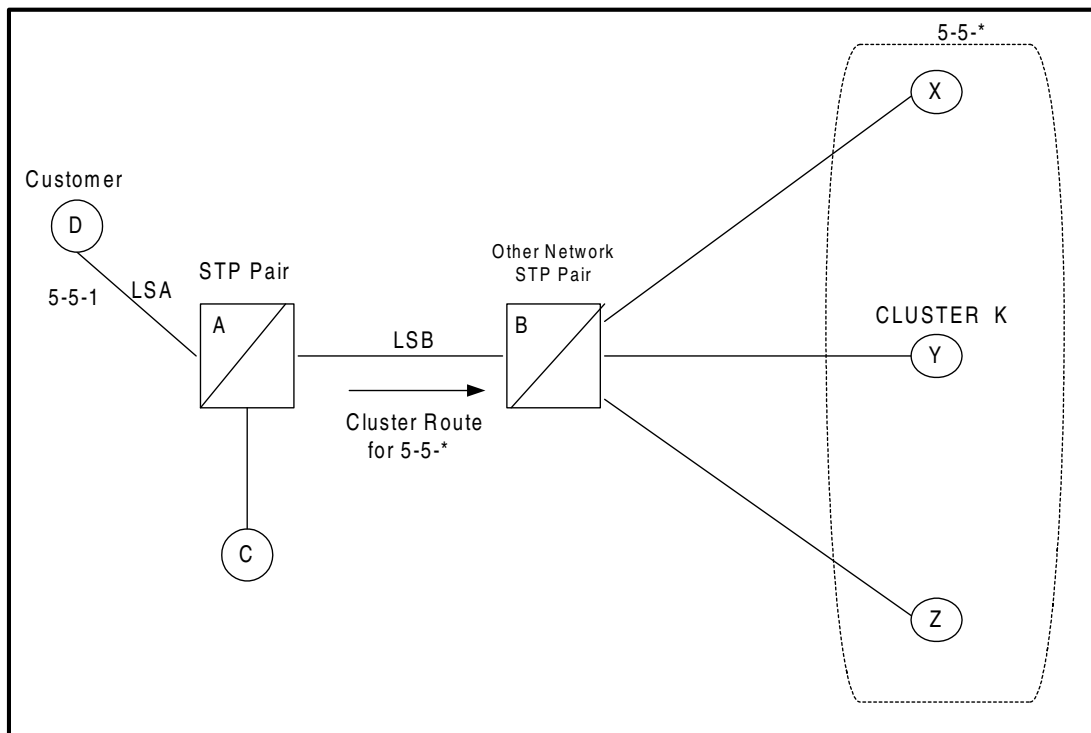
Figure 4-28. Cluster Network Configuration
