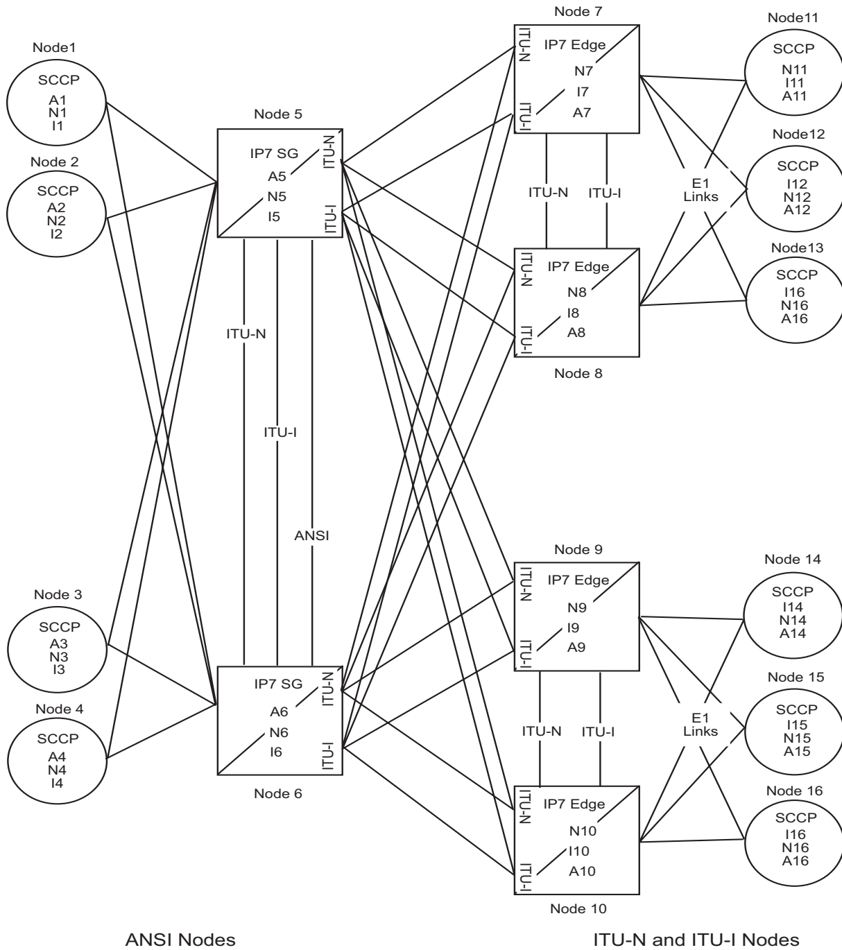
Figure 5-1. Complex Network with ANSI, ITU-I, and ITU-N Nodes
