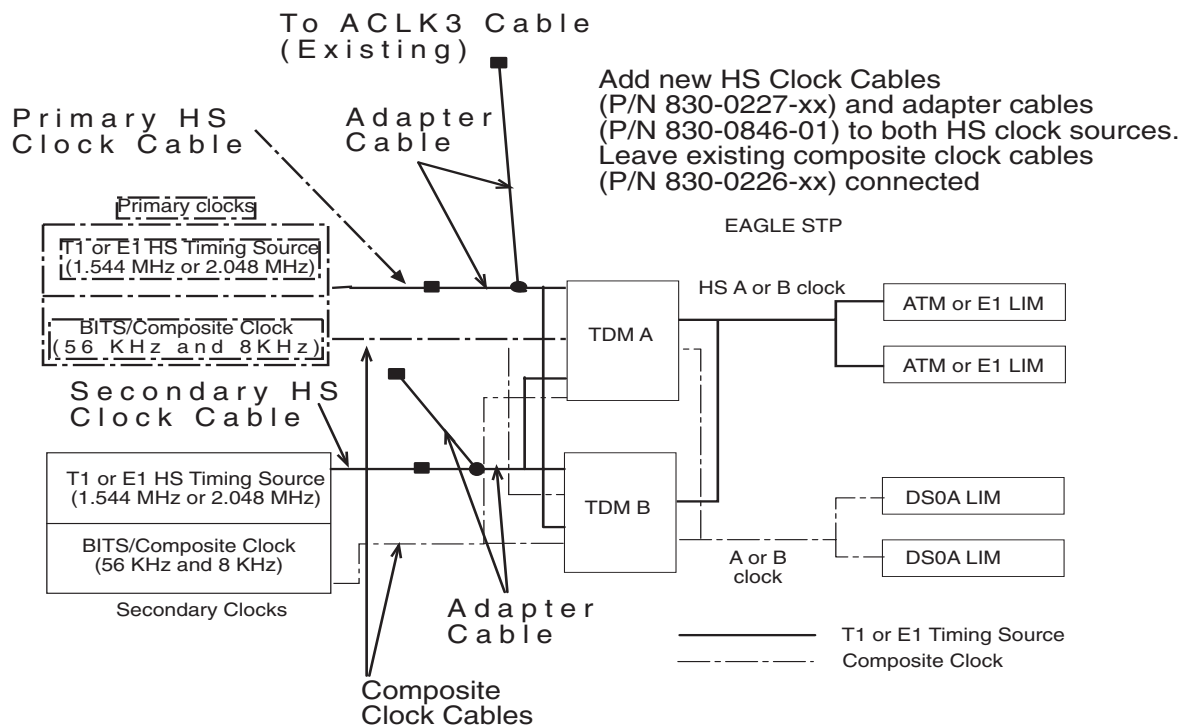
Figure 3-7. HS Master Timing Concept using Control Shelf Backplane (P/N 850-0330-03/04)
