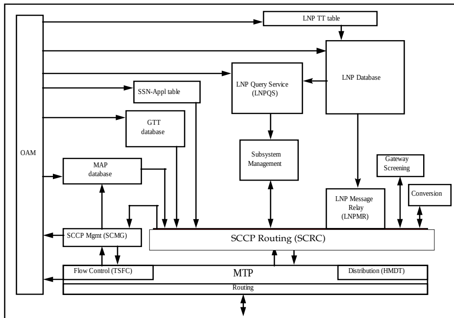
Figure 4-13. LNP Block Diagram
