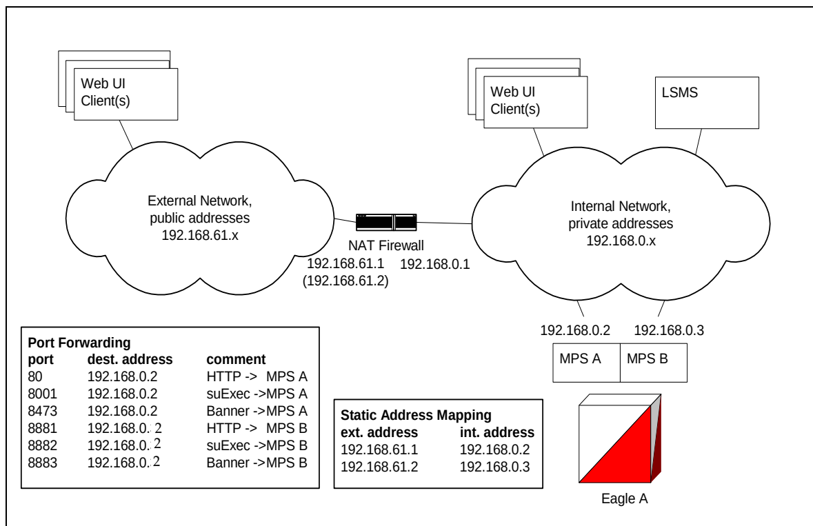
Figure 2-17. Network Address Translation on MPS
