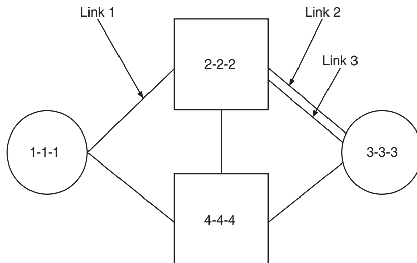
Figure 2-4. Example Network for Problem Description
