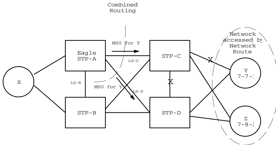
Figure 4-34. Potential Routing Network Failure
