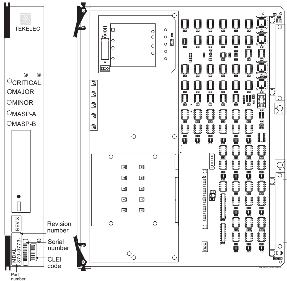
Figure 3-29. Maintenance Disk and Alarm Card
