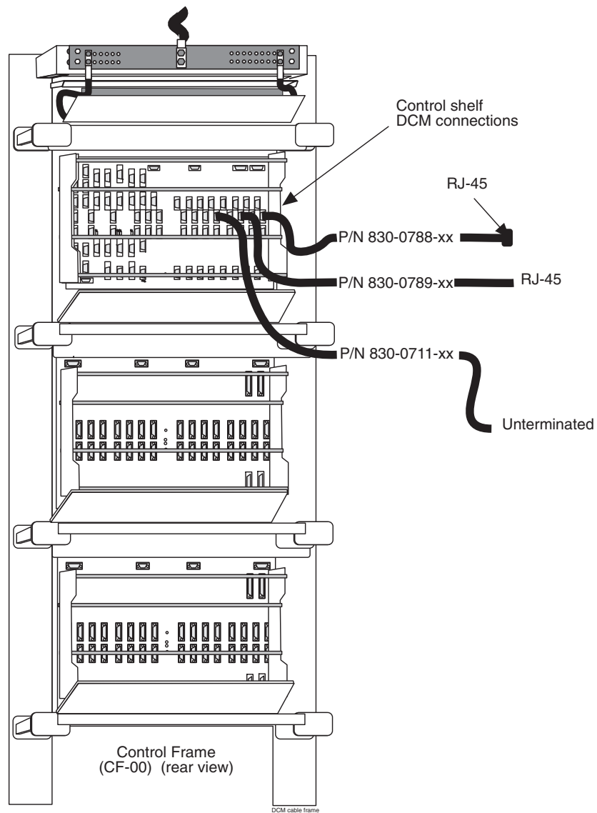
Figure 5-4. Database Communications Cabling in System
