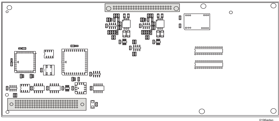
Figure 3-32. Digital Signal Level-0 Applique
