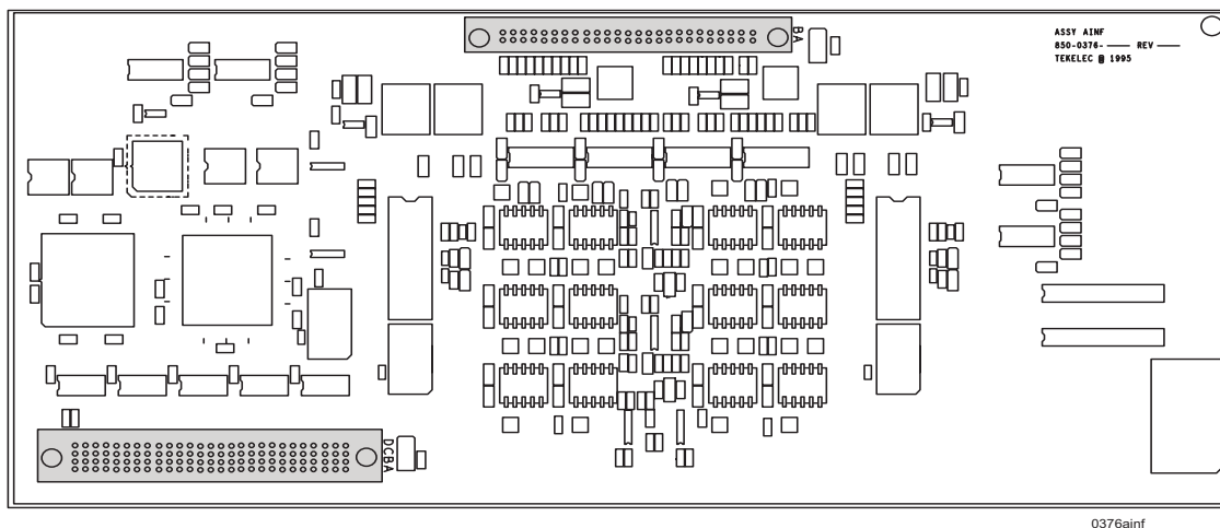
Figure 3-35. Application Interface Applique
