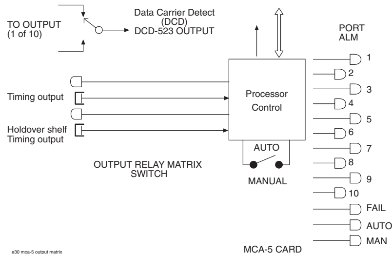
Figure 3-77. MCA-5 Card and Output Protection Matrix
