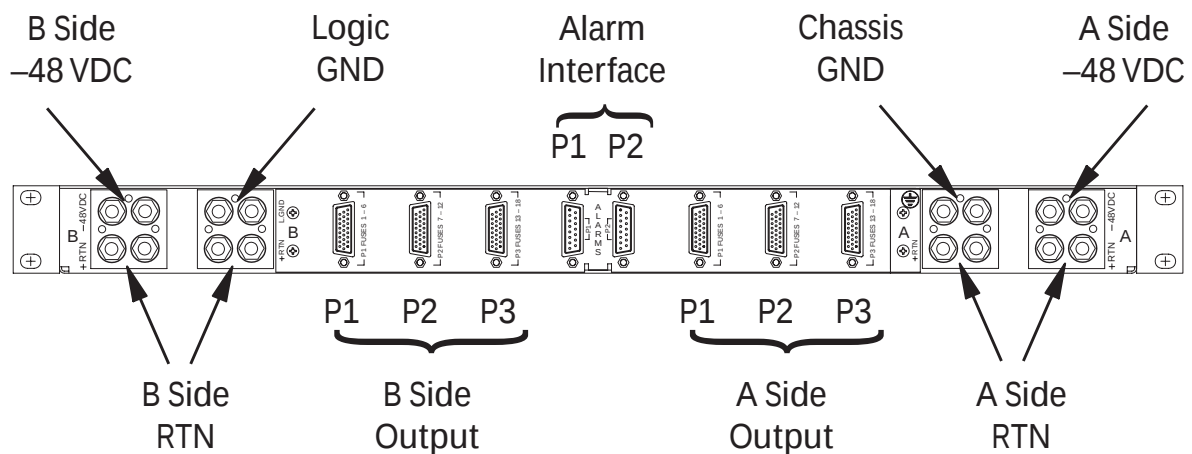
Figure 3-67. Fuse and Alarm Panel Rear (P/N 870-2804-01).
