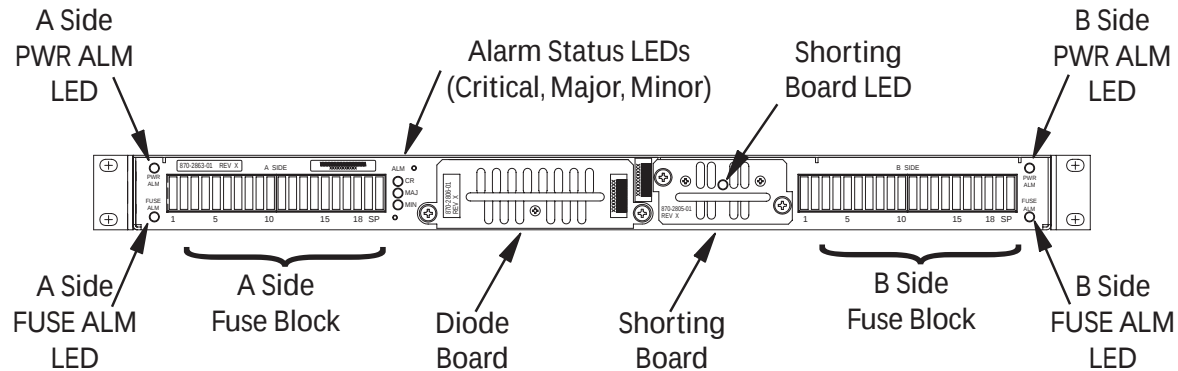
Figure 3-66. Fuse and Alarm Panel Front (P/N 870-2804-01).
