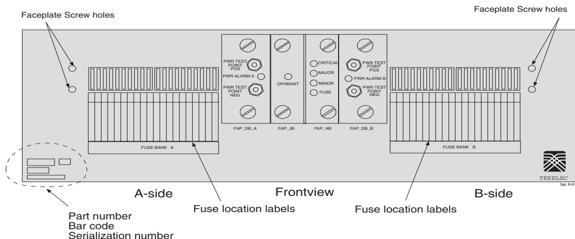
Figure 3-68. Fuse and Alarm Panel (P/N 870-1606-xx/870-2320-xx) Front
