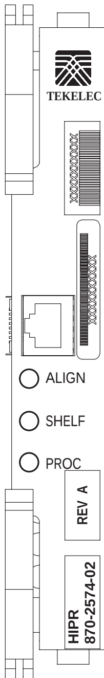
Figure 3-26. HIPR LEDs
