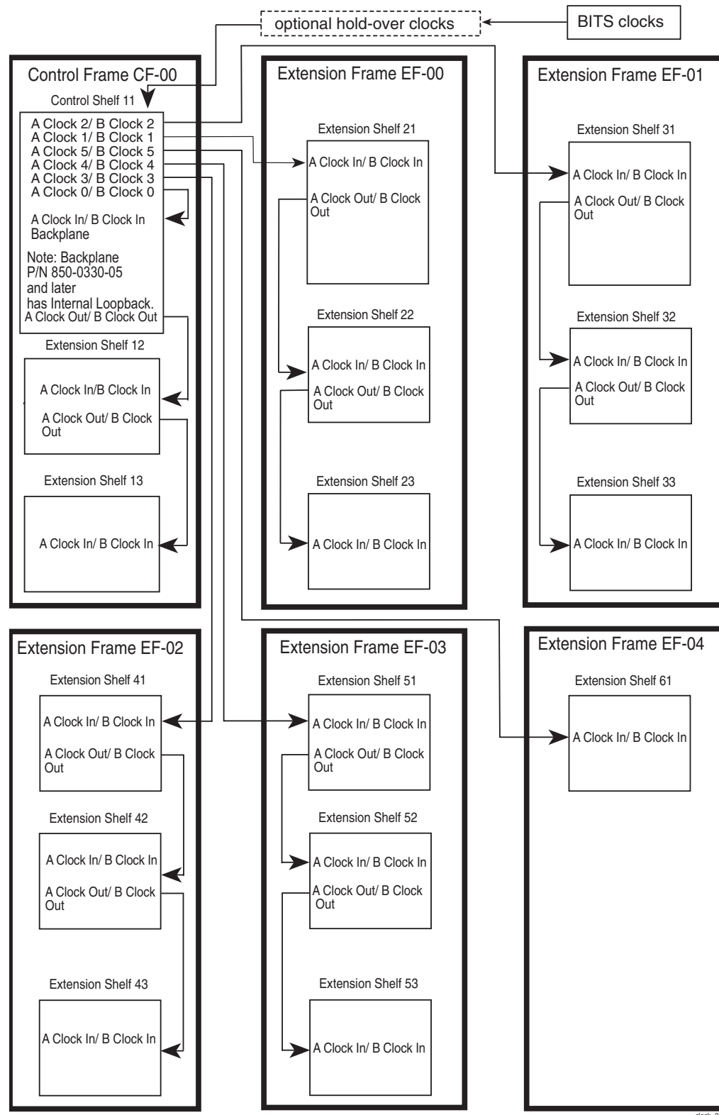
Figure 2-2. Clock Routing
