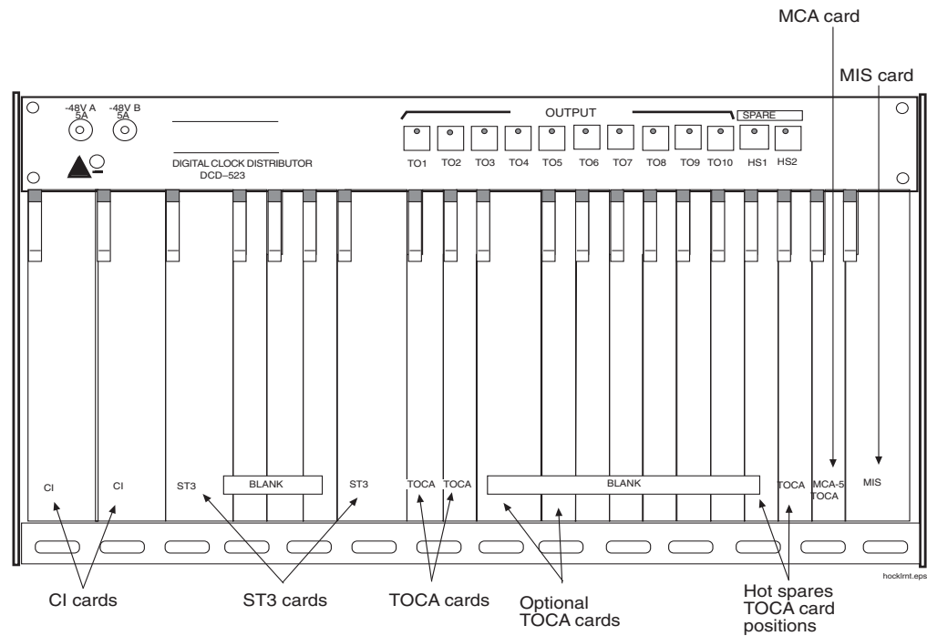
Figure 3-74. Holdover Clock
