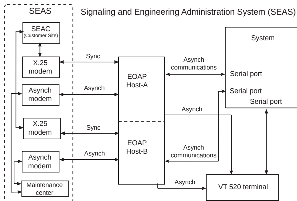
Figure 2-3. EOAP Hosts in an EAGLE 5 ISS
