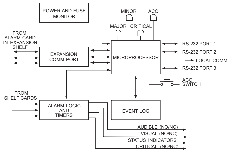
Figure 3-76. Maintenance Interface System Card Block Diagram
