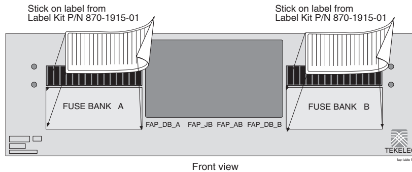
Figure 3-71. FAP, Fuse Label Kit (P/N 870-1915-02)
