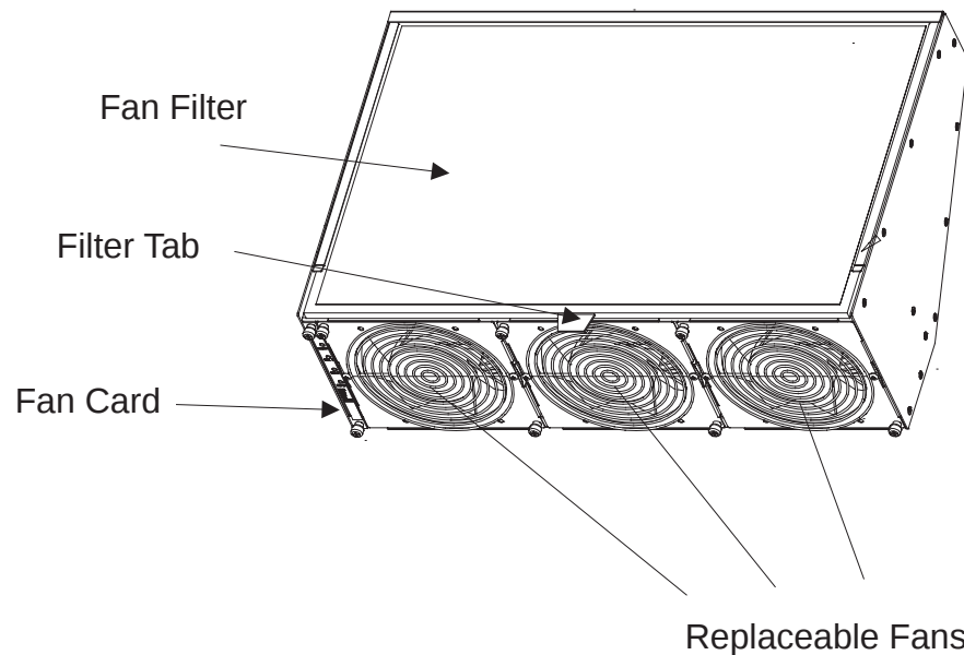
Figure 3-64. Fan Tray
