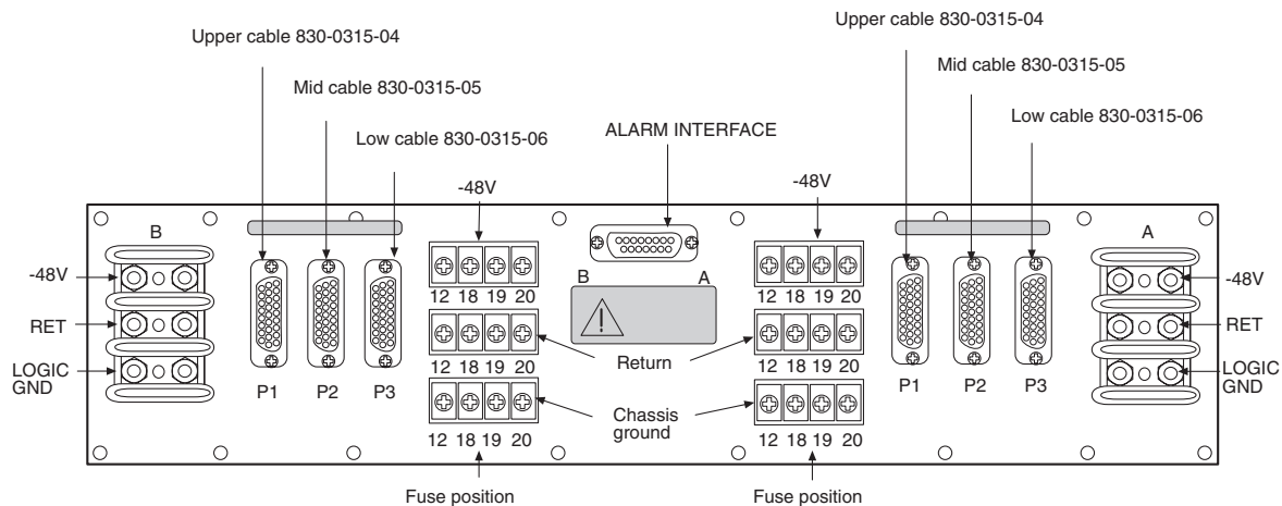
Figure 3-69. Fuse and Alarm Panel (P/N 870-1606-xx/870-2320-xx) Rear.
