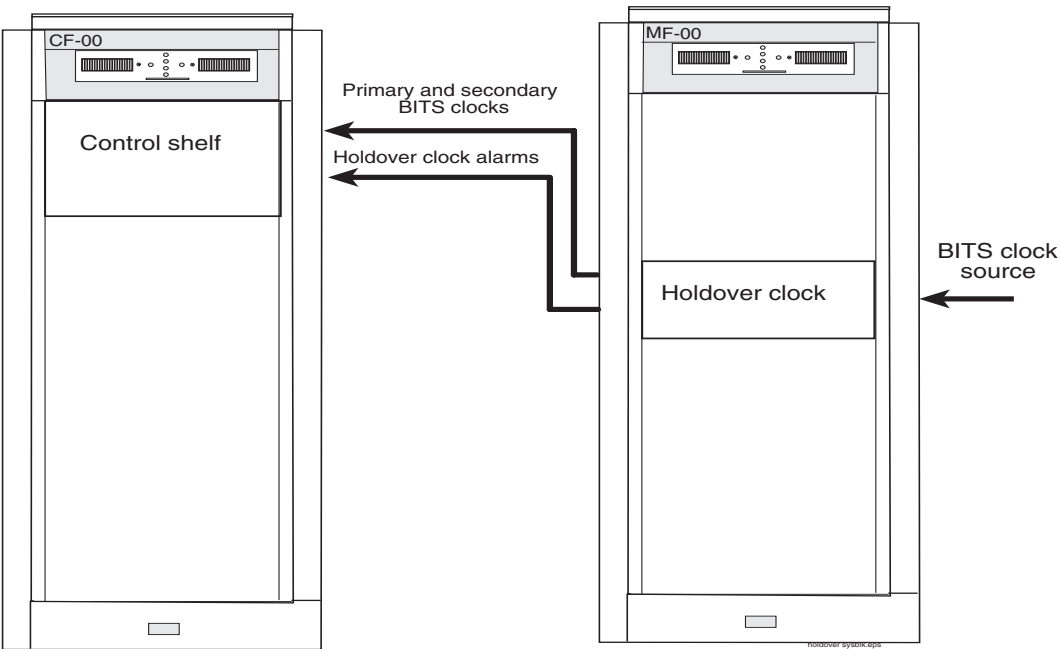
Figure 3-75. Holdover Clock
