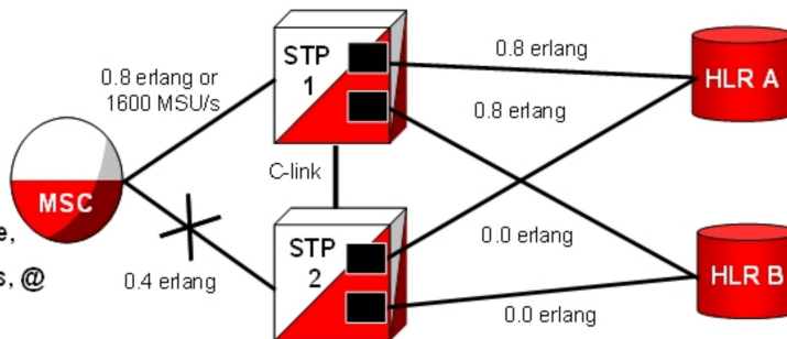
Figure 5-4. EAGLE 5 ISS: Failover at 0.8 erlang and 1600 MSU/s
