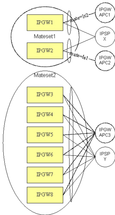
Figure A-10. Eight IPGWx cards, two mates, three linksets
