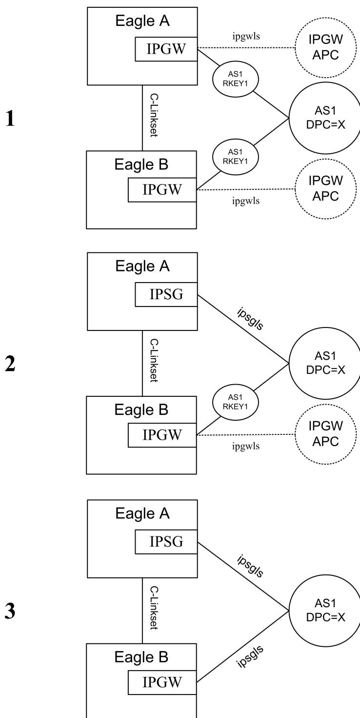
Figure 6-1. PGWx to IPSG-M3UA Conversion Strategy Example 1
