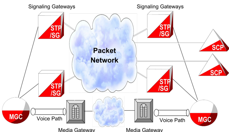
Figure 2-3. SS7-over-IP network.
