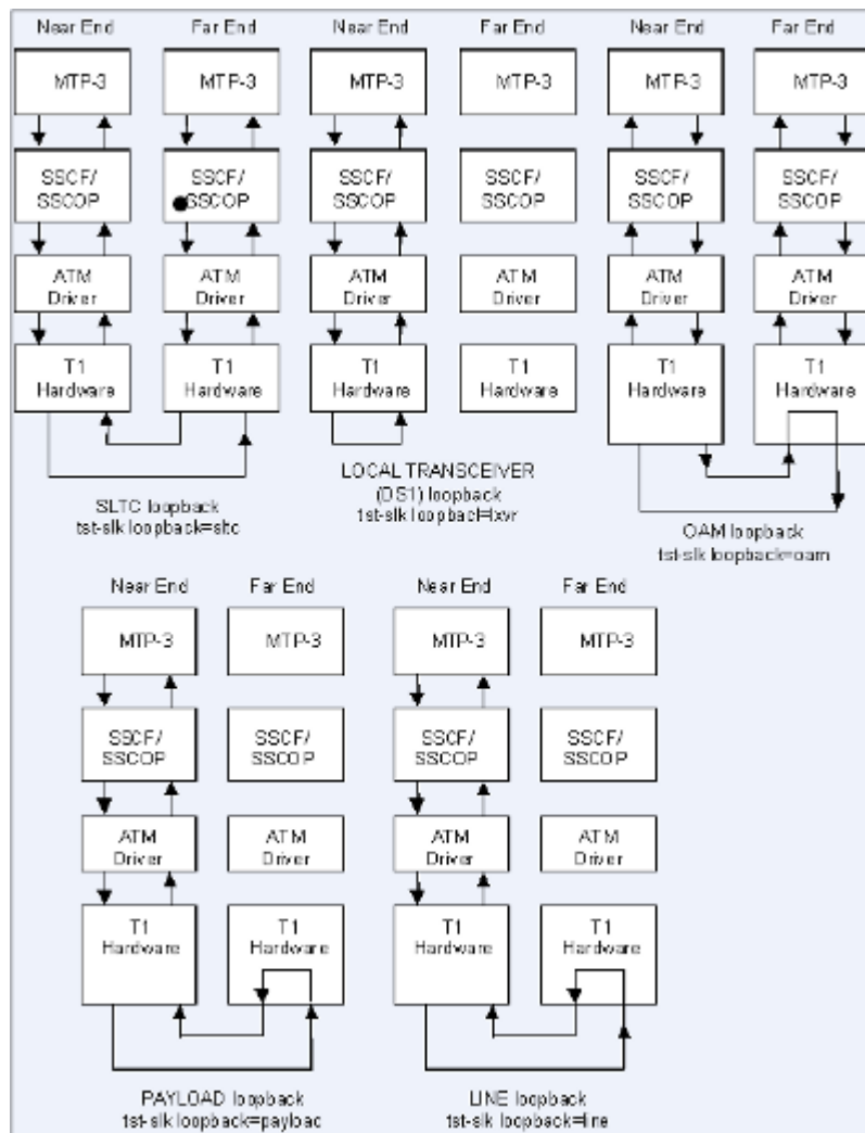
Figure 12: ATM Loopback Tests
