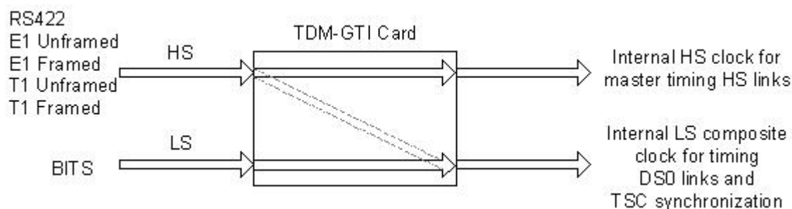
Figure 4: Eagle Input and Internal Clocks with TDM-GTI
