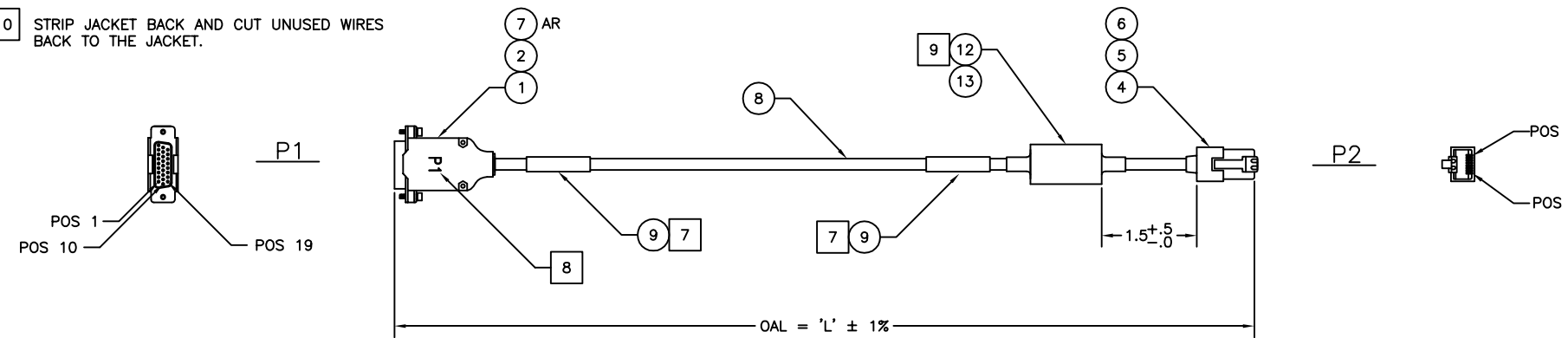
ASSEMBLY DIAGRAM
