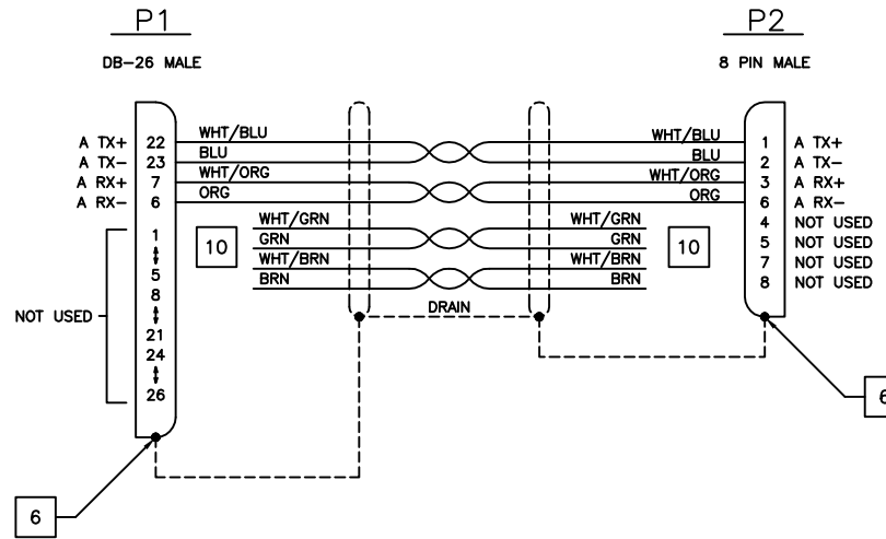
WIRING DIAGRAM
