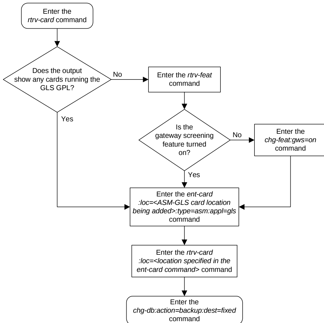
Flowchart 2-1. Adding an ASM-GLS Card to the Database
