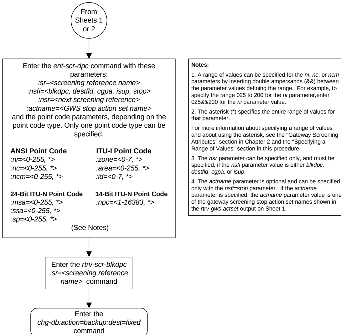
Flowchart 9-2. Adding an Allowed DPC Screen (Sheet 3 of 3)
