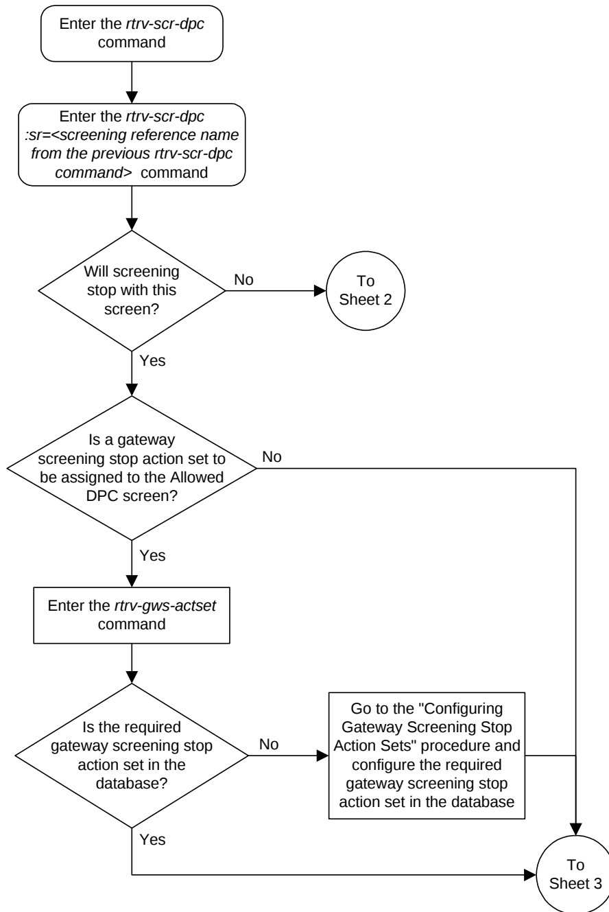
Flowchart 9-4. Changing an Allowed DPC Screen (Sheet 1 of 3)
