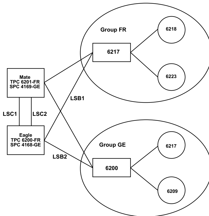
Figure 2-1. Sample Network Showing Gateway Screening Using Duplicate ITU National Point Codes
