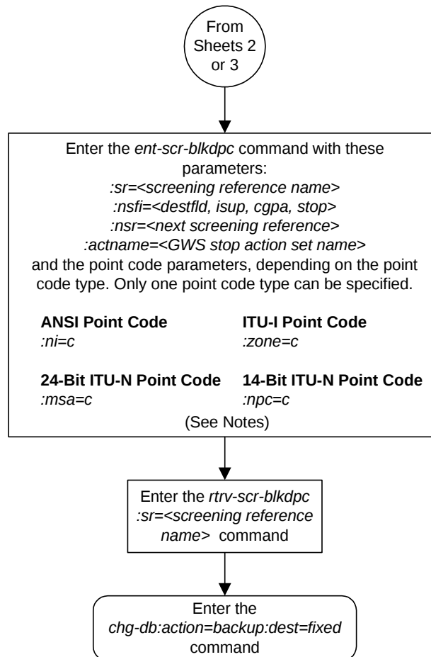
Flowchart 8-2. Adding a Blocked DPC Screen (Sheet 4 of 4)
