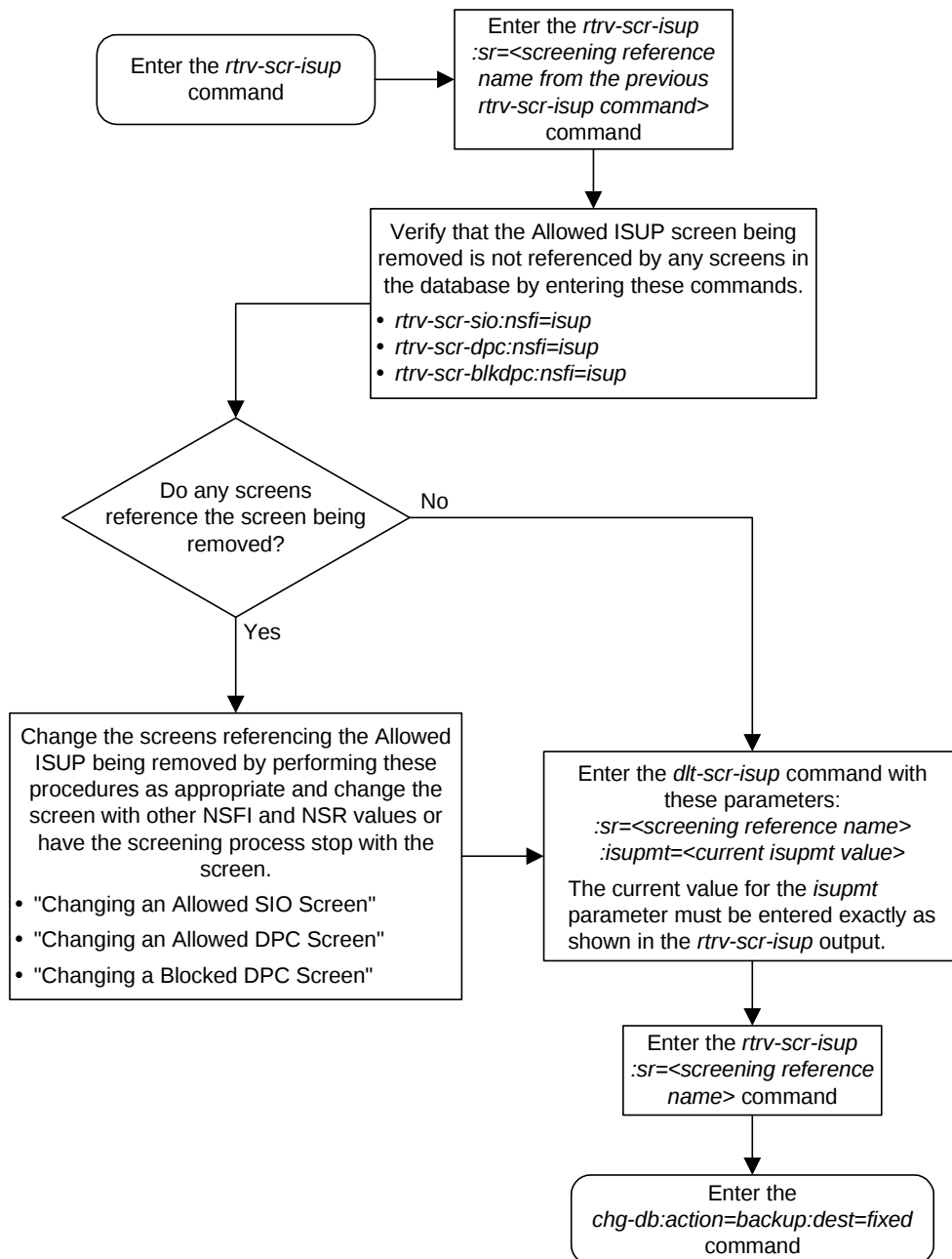
Flowchart 15-3. Removing an Allowed ISUP Message Type Screen
