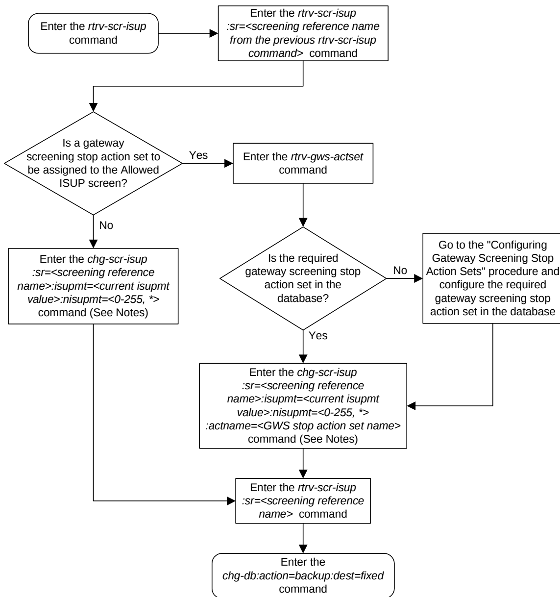
Flowchart 15-4. Changing an Allowed ISUP Message Type Screen
