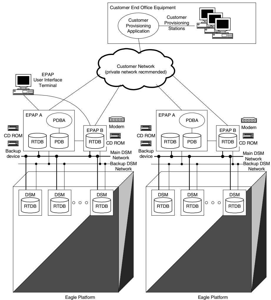
Figure 2-3. MPS/EPAP System Configuration
