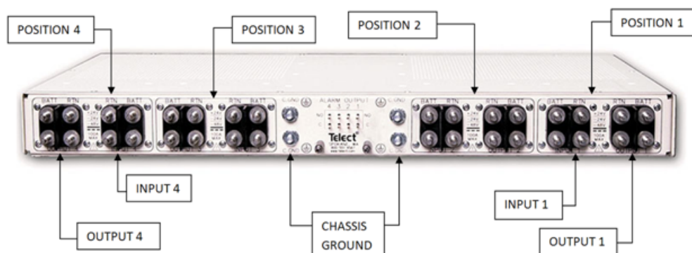
Figure 78: High Current Demarcation Panel - front and rear views
