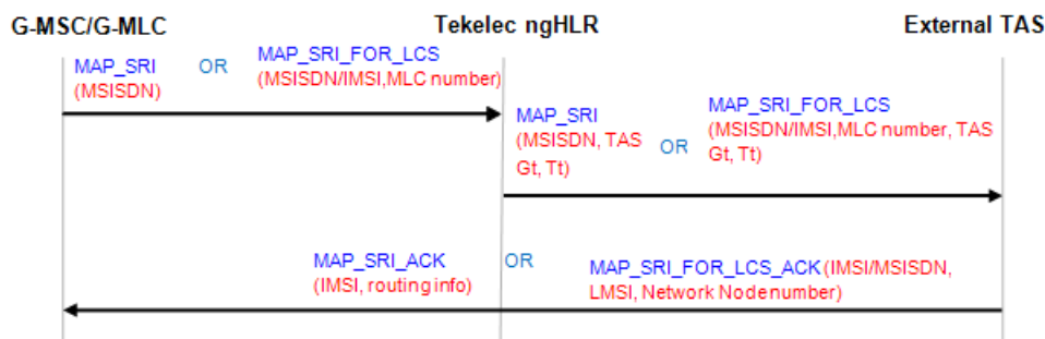
Figure 44: Call flow for SRI/SRI-LCS Relay to the external TAS within the IMS Network
