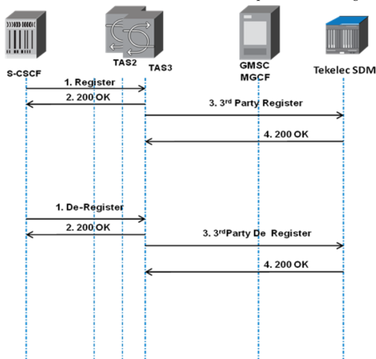
Figure 56: Register/De-register call flow in the IMS Domain for 3rd party registration from TAS node.
