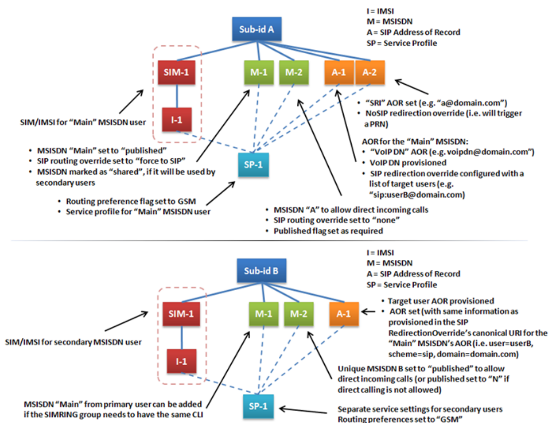
Figure 30: SimRing configuration
