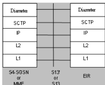
Figure 11: Diameter stack
