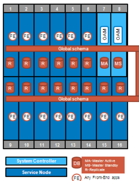
Figure 73: Example of HP c-Class architecture
