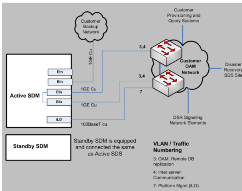
Figure 67: SDM rackmount configuration using dedicated uplink for NetBackup
