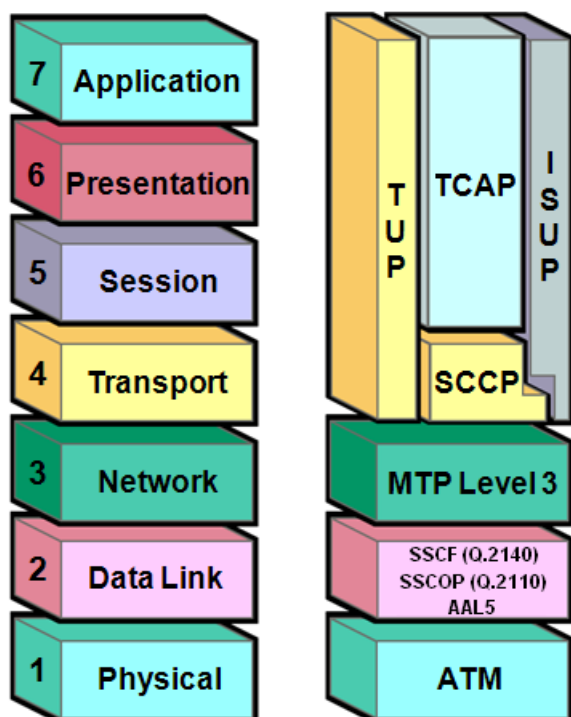
Figure 3: The OSI Reference Model and the SS7 Protocol Stack using SAAL
