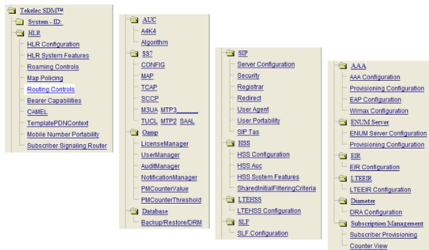
Figure 14: WebCI main menu expanded
