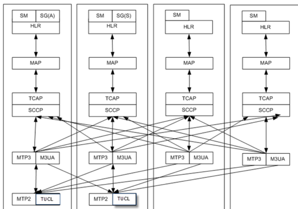
Figure 10: Scalability of SS7 and SIGTRAN layers within the HLR Service for a four blade system
