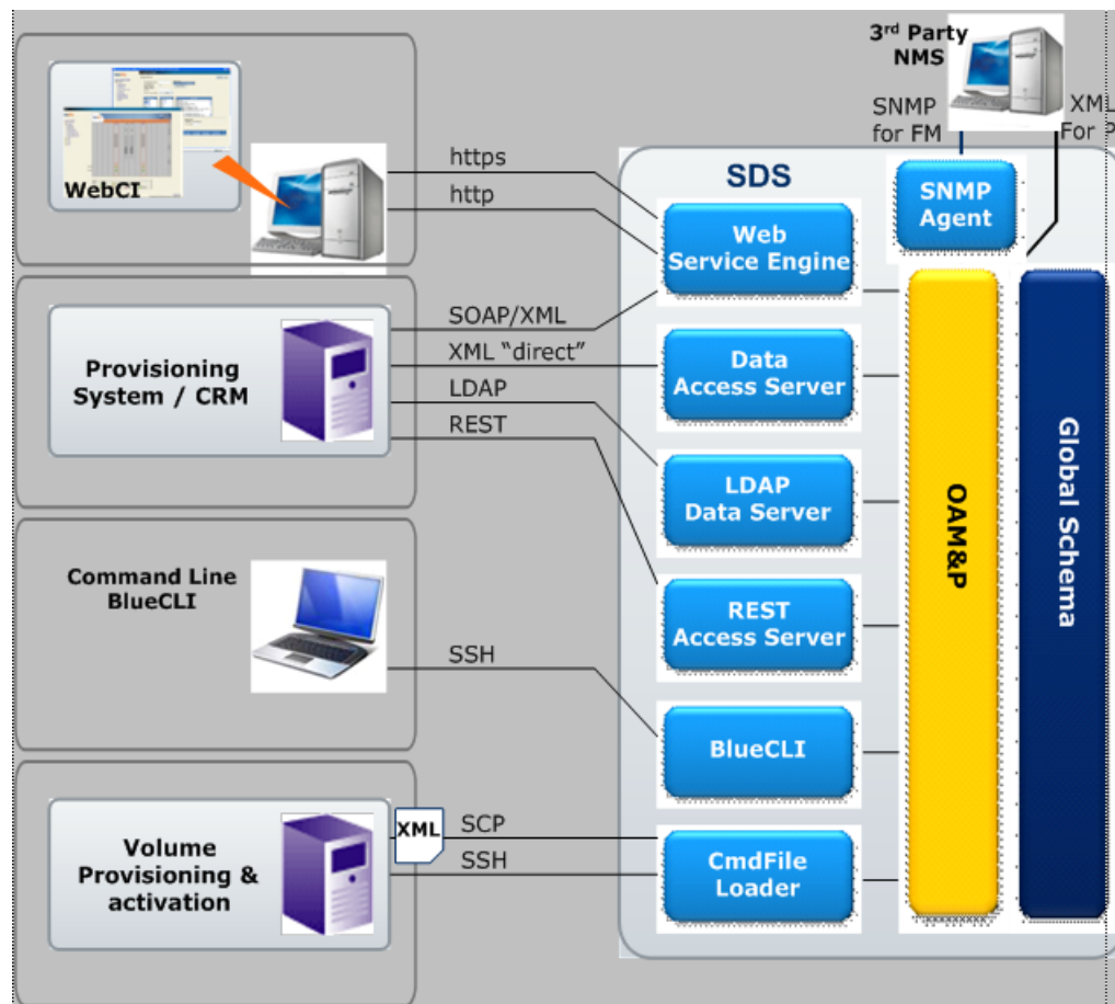
Figure 64: OAM&P interfaces
