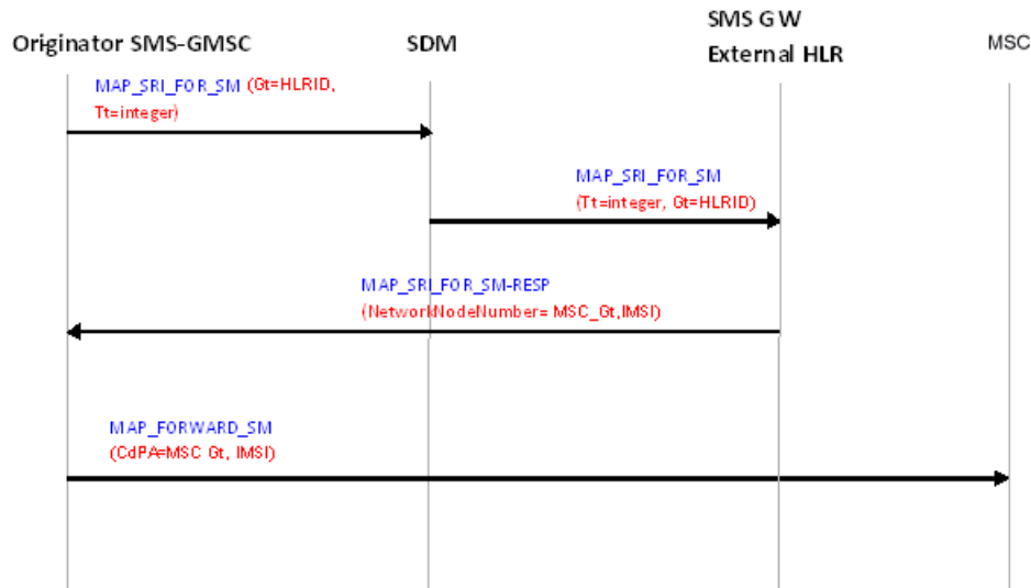
Figure 34: Call flow for MT-SMS Relay to the external HLR within the GSM Network
