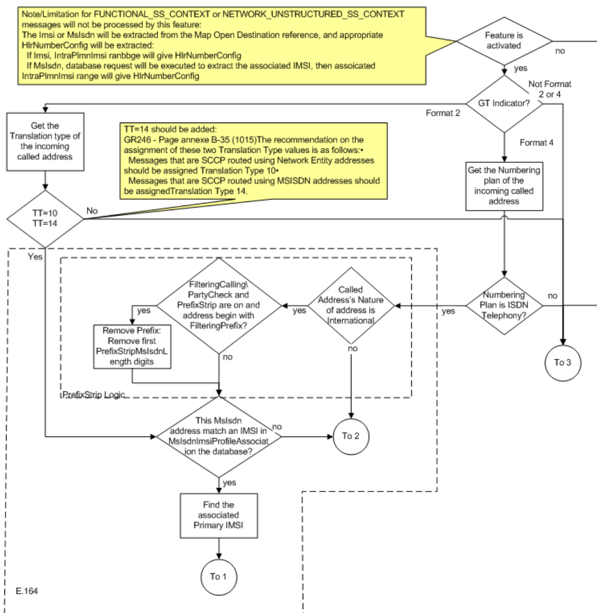
Figure 27: SCCP Routing for ITU and ANSI Calls
