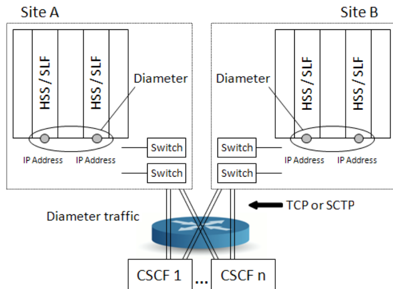
Figure 20: IMS-HSS network connections in a geo-redundant deployment.
