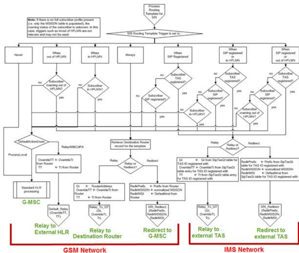
Figure 38: SRI message routing in the Tekelec ngHLR
