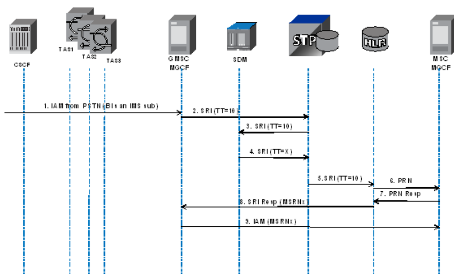
Figure 57: SRI message routing call flow in the IMS Domain for a 3rd party SIP registered subscriber.
