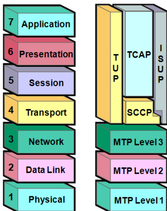
Figure 2: The OSI Reference Model and the SS7 Protocol Stack using MTP 1 and 2 Layers
