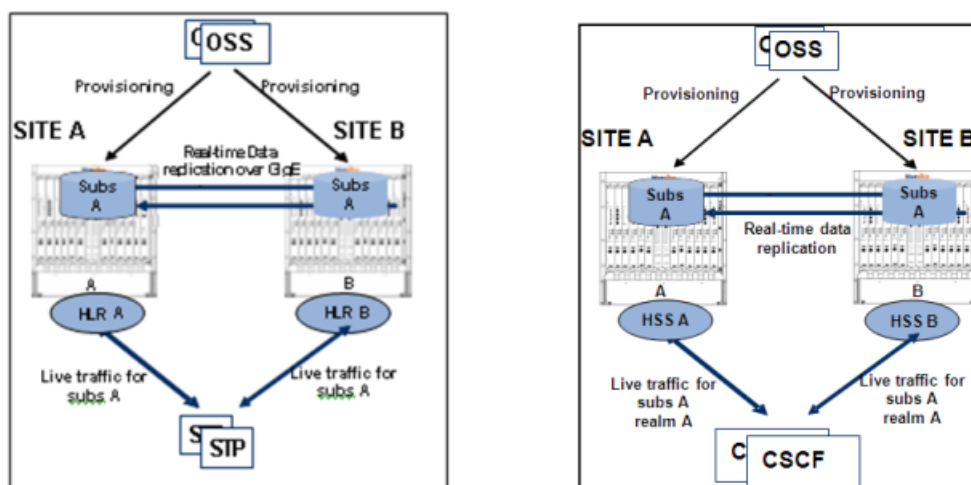
Figure 17: Geo Redundancy logic for the HLR and HSS services.
