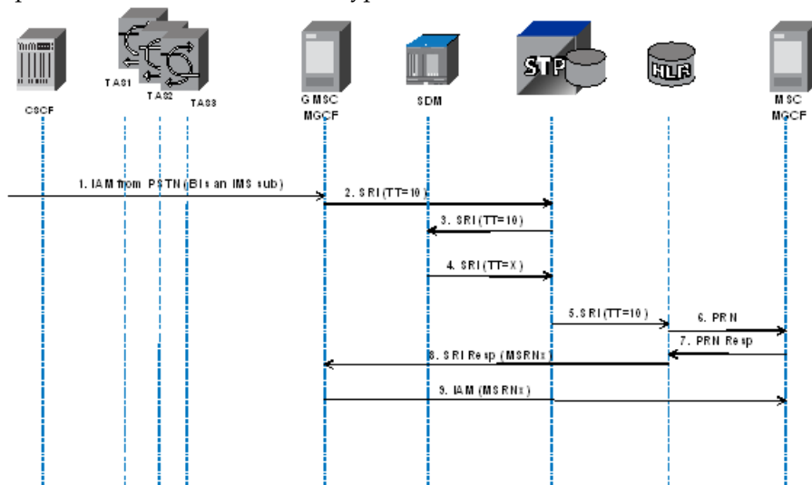
Figure 58: SRI message routing call flow in the IMS Domain for a subscriber with no 3rd party SIP registration.
