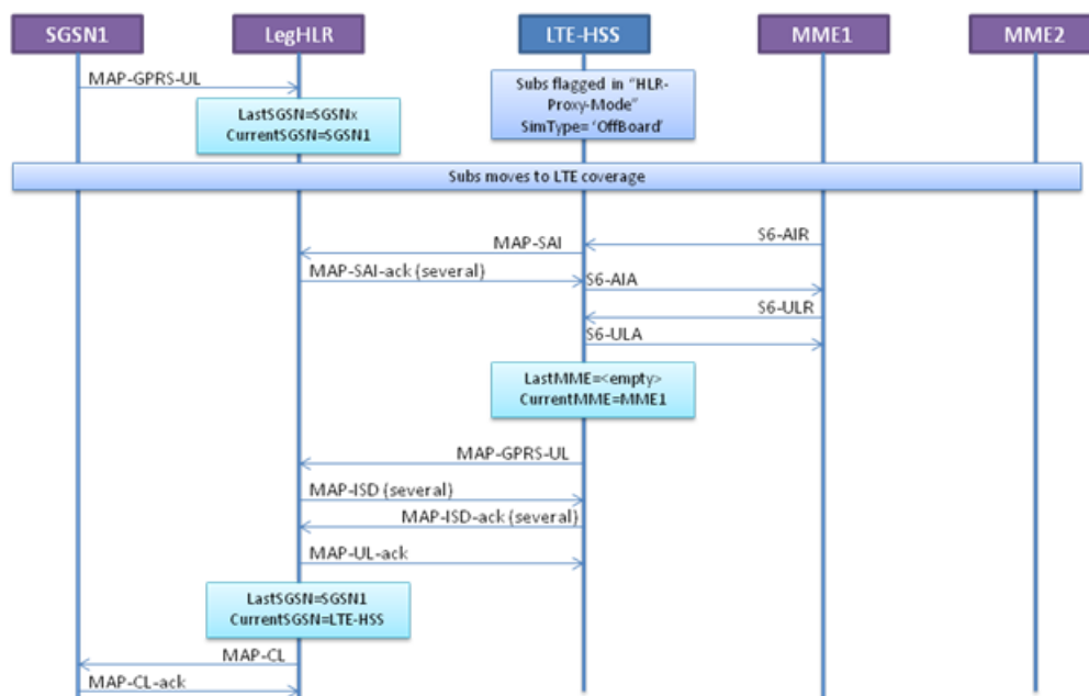
Figure 60: 3G&gt;LTE Mobility
