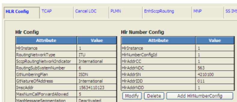
Figure 16: WebCI window tabs
