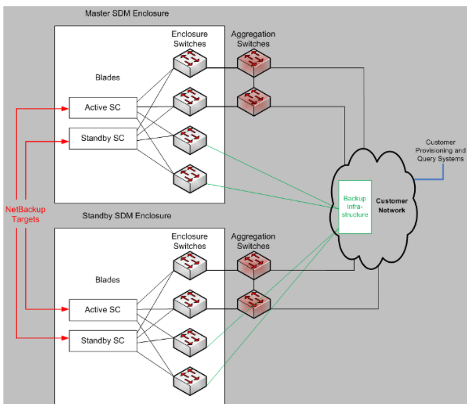
Figure 68: SDM C-Class configuration using dedicated uplink for NetBackup
