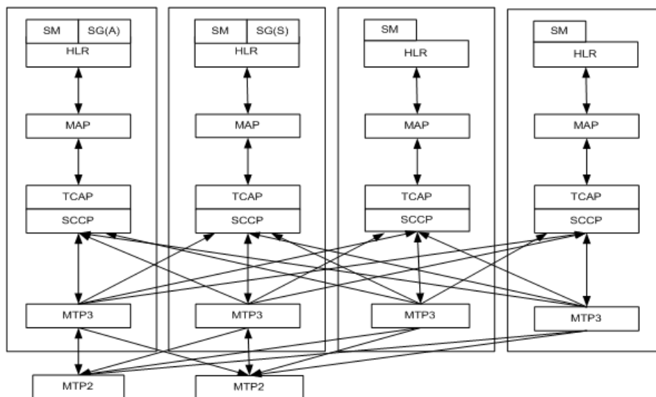
Figure 9: Scalability of SS7 layers within the Hlr service for a four blade system
