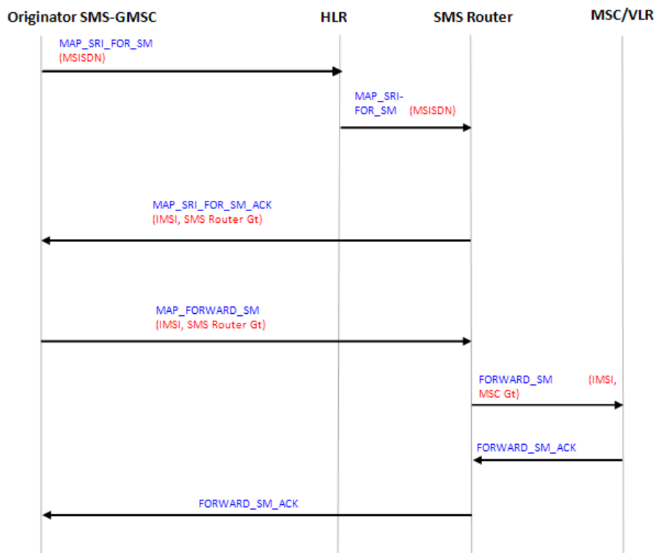
Figure 33: Call flow for MT-SMS Relay to the Destination Router within the GSM Network
