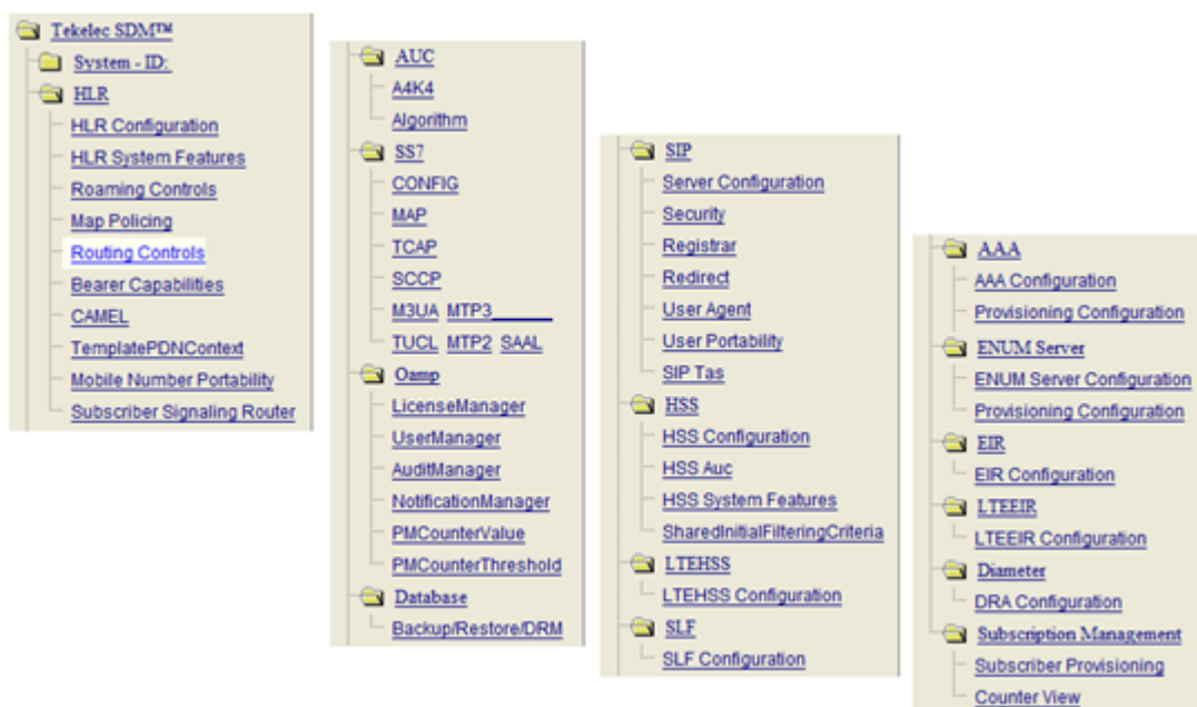
Figure 15: WebCI main menu expanded
