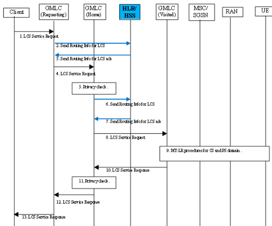
Figure 23: SRI-LCS Call Flow
