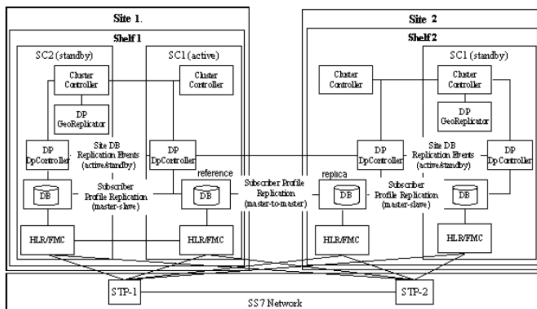
Figure 19: Data replication between two geo-redundant sites at the process level.
