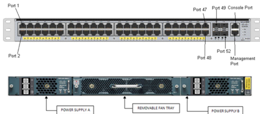
Figure 79: Cisco 4948E-F Aggregation Switch - front and rear views
