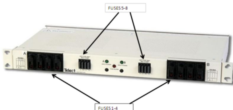
Figure 76: Telect 100A 4/4 fuse panel - front view
