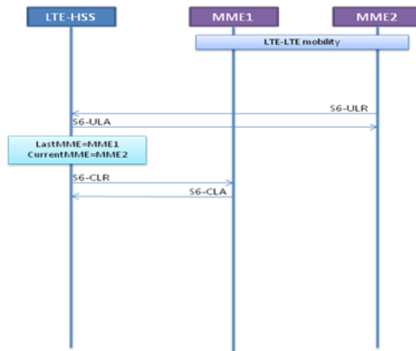
Figure 62: LTE>LTE Mobility
