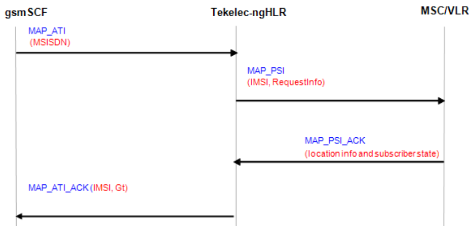
Figure 52: Call flow for Standard ATI Routing
