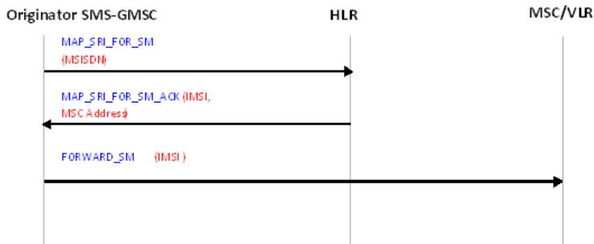
Figure 32: Call flow for Standard MT-SMS Routing
