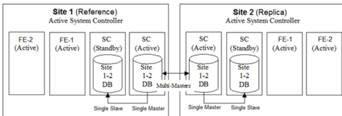
Figure 18: Data replication between two geo-redundant sites.
