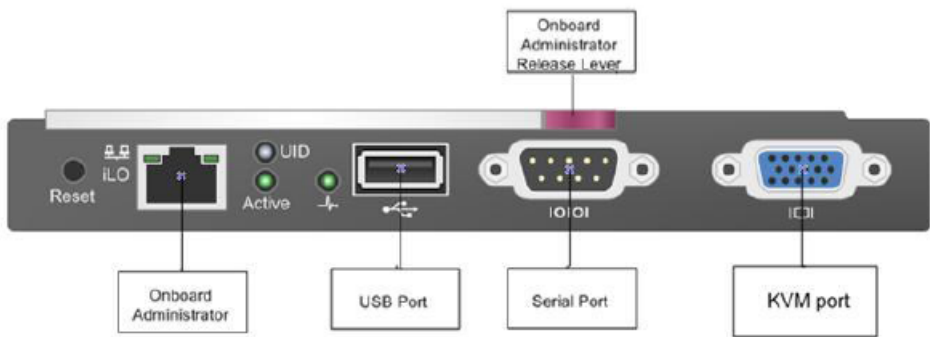
Figure 90: HP c7000 enclosure onboard administrator
