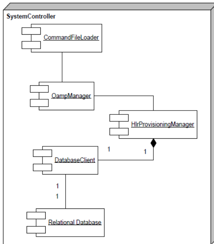
Figure 69: CommandFileLoader component diagram
