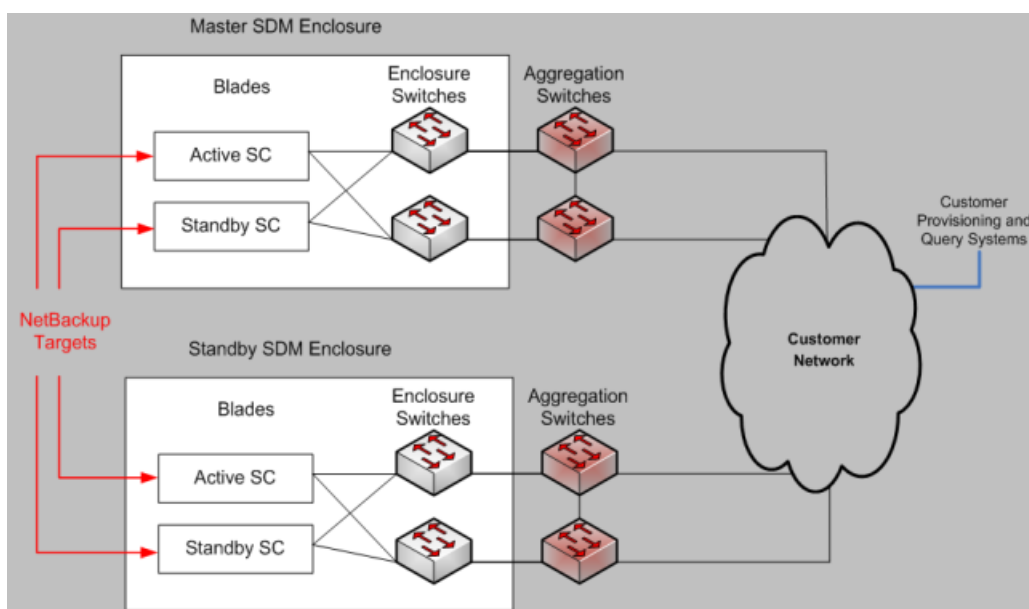
Figure 66: SDM C-Class configuration using XMI for NetBackup
