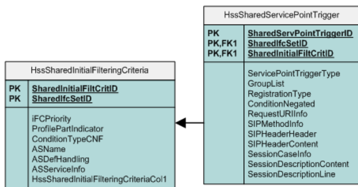
Figure 59: The CSCF's database schema for the support of Shared IFC
