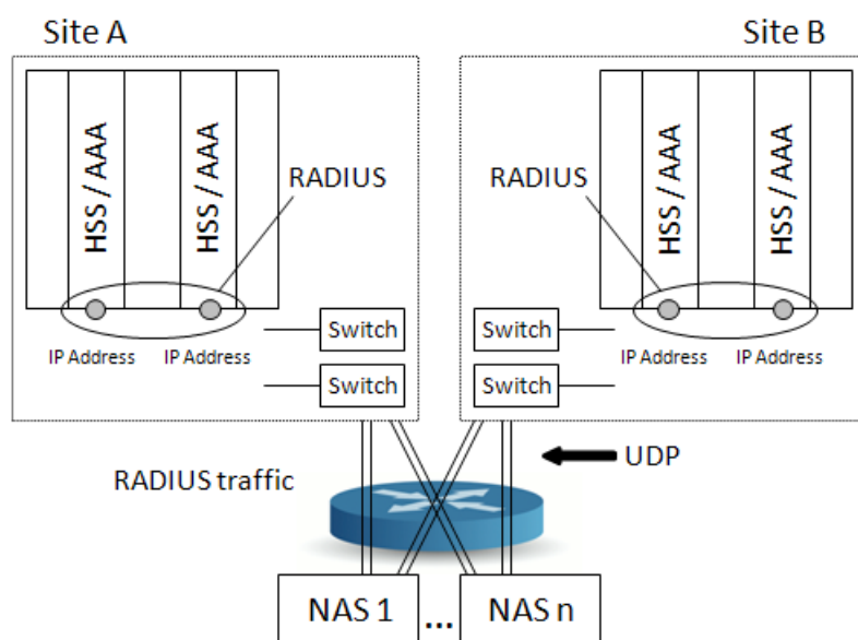
Figure 21: AAA network connections in a geo-redundant deployment.
