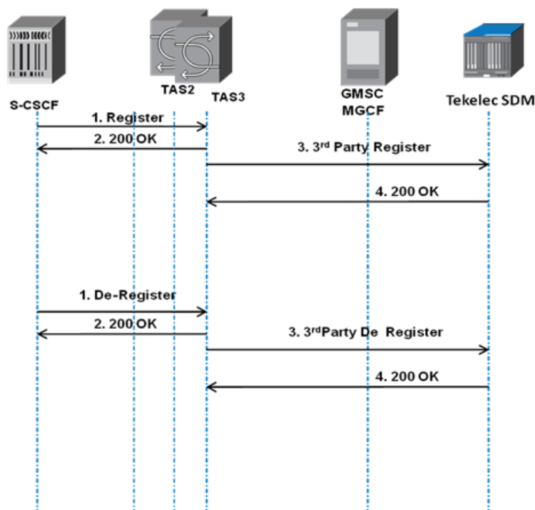
Figure 31: Register/De-Register Call Flow in the IMS Domain for 3rd Party Registration from TAS Node
