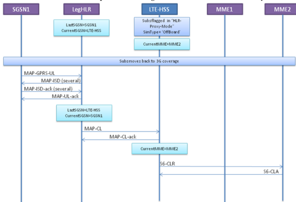
Figure 61: LTE&gt;3G Mobility
