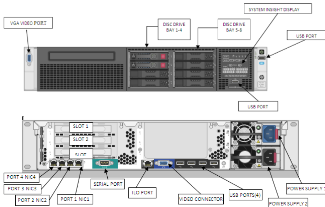
Figure 82: HP DL380 Gen8 rackmount servers - front and rear views
