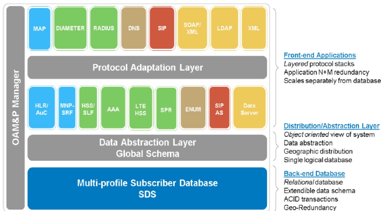
Figure 6: SDM high level software architecture
