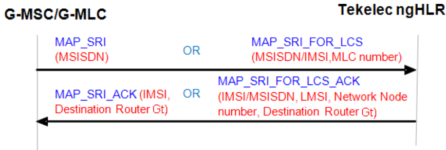
Figure 48: Call flow for SRI/SRI-LCS Redirect to the MSC/VLR (in the GSM network)
