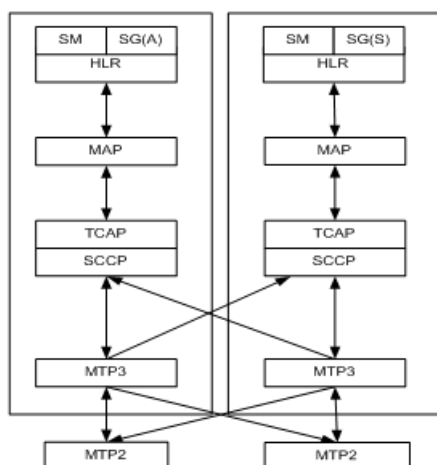
Figure 8: Scalability of SS7 layers within the Hlr service for a two blade system
