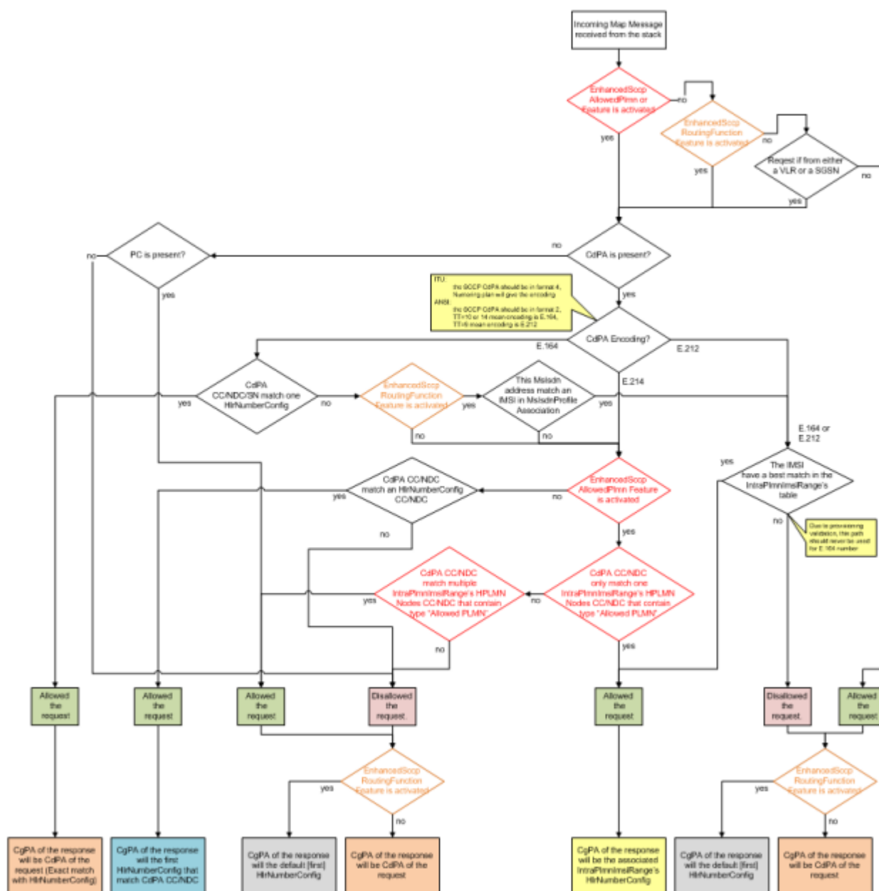
Figure 28: Enhanced SCCP Allowed PLMN flow
