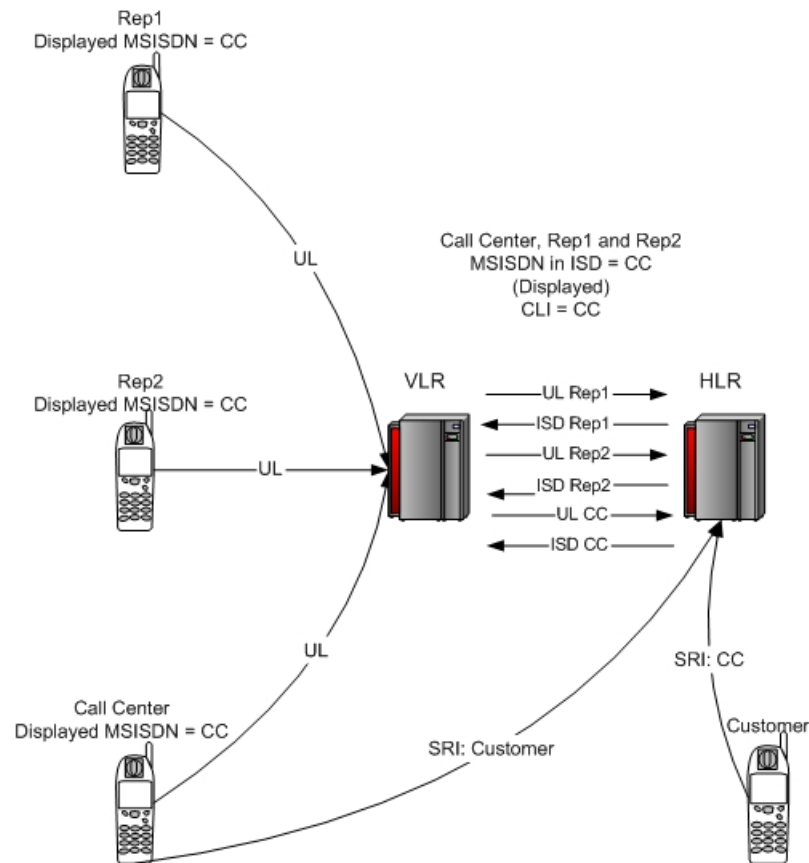
Figure 24: Example using Shared MSISDN across CLI
