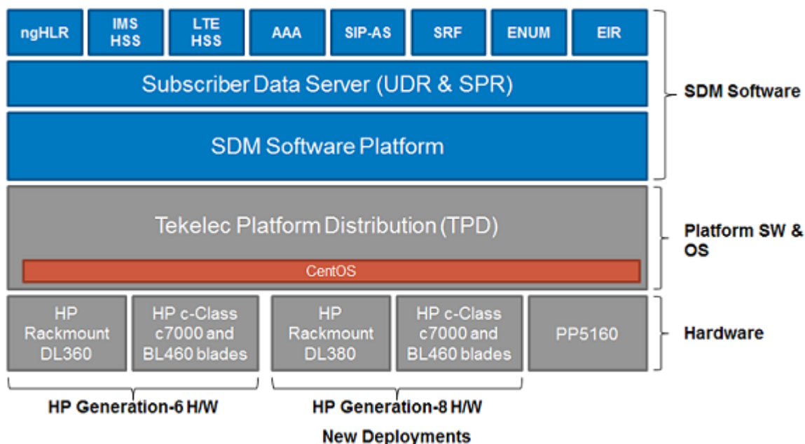
Figure 72: Subscriber Data Management (SDM) architecture
