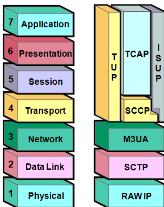
Figure 4: OSI Reference Model and the SIGTRAN Stack using SCTP/M3UA protocols
