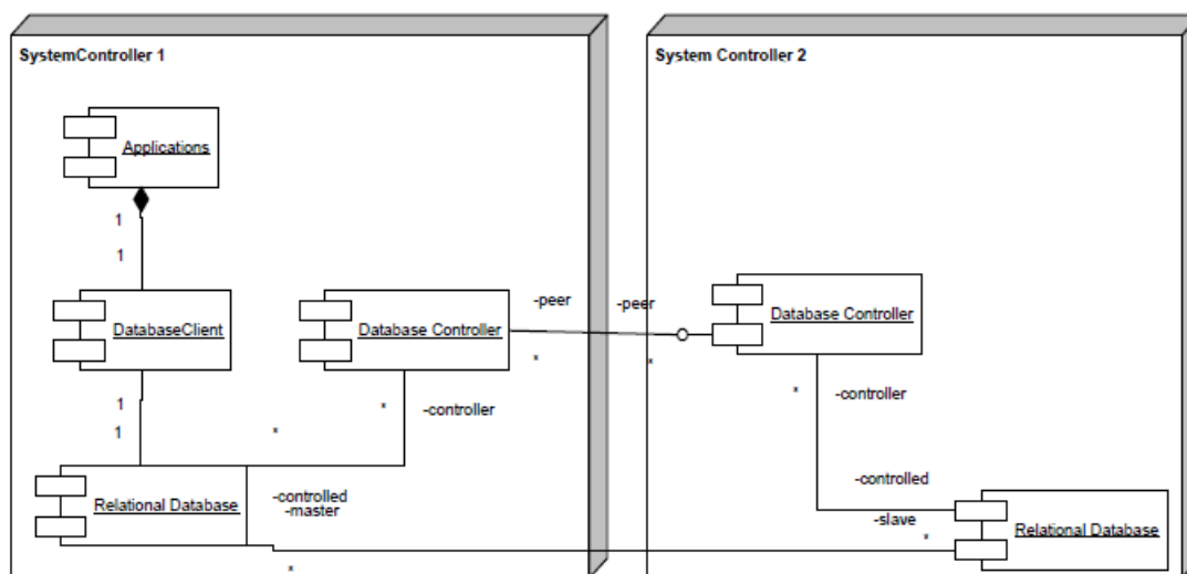
Figure 12: Database component diagram
