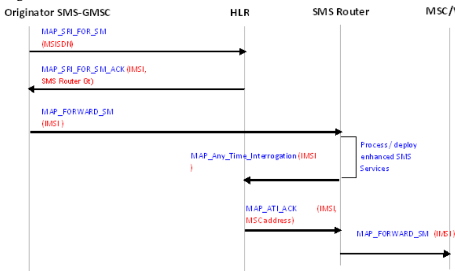
Figure 36: Call flow for MT-SMS Redirect to the MSC/VLR (in the GSM network)
