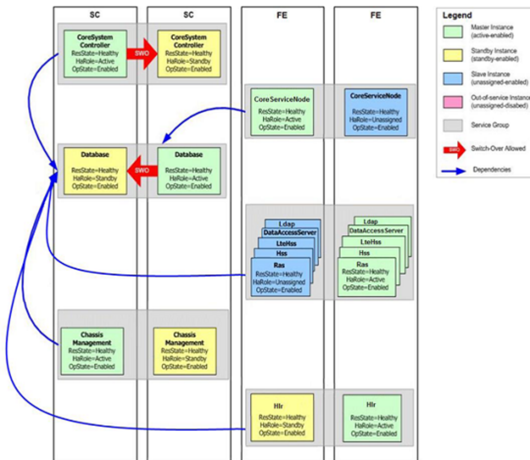
Figure 7: Services on four-blade system
