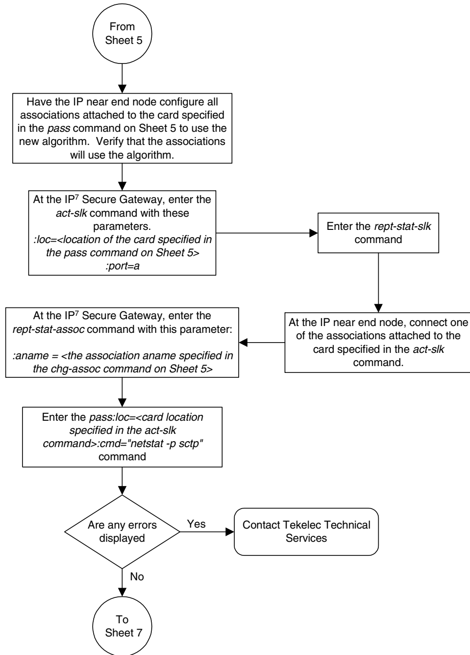
Flowchart 3-41. Changing the SCTP Checksum Option (Sheet 6 of 7)
