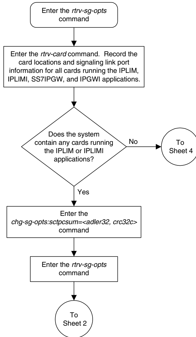
Flowchart 3-41. Changing the SCTP Checksum Option (Sheet 1 of 7)
