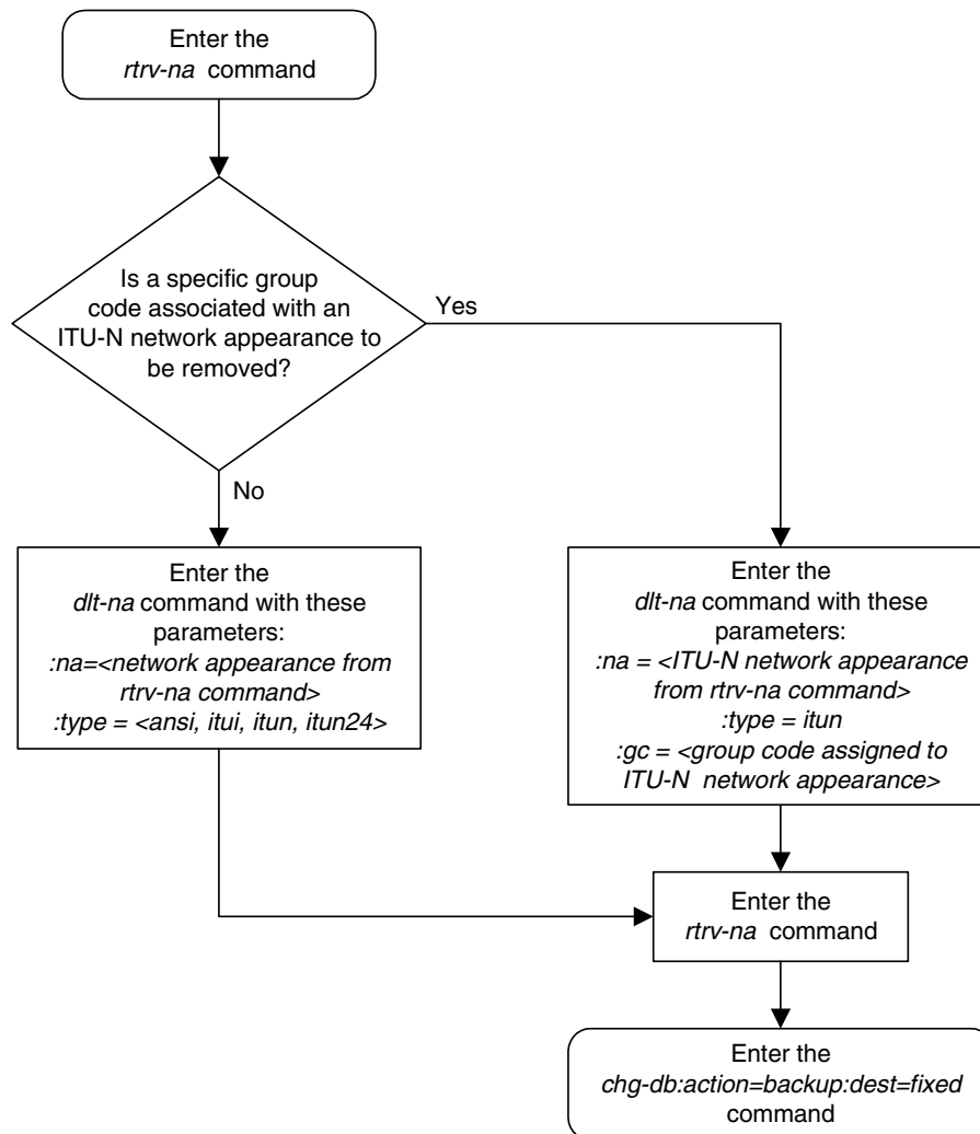
Flowchart 3-40. Removing a Network Appearance
