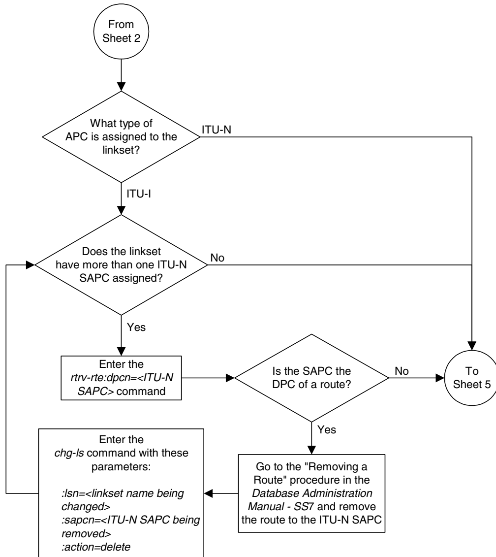
Flowchart 3-3. Configuring an IPGWx Linkset (Sheet 4 of 6)
