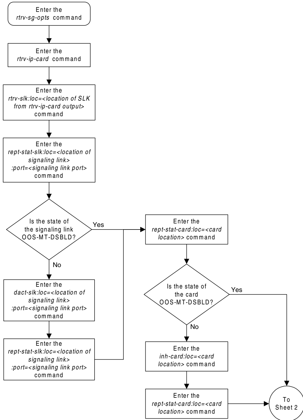
Flowchart 3-9. Changing the IP Protocol Option (Sheet 1 of 2)
