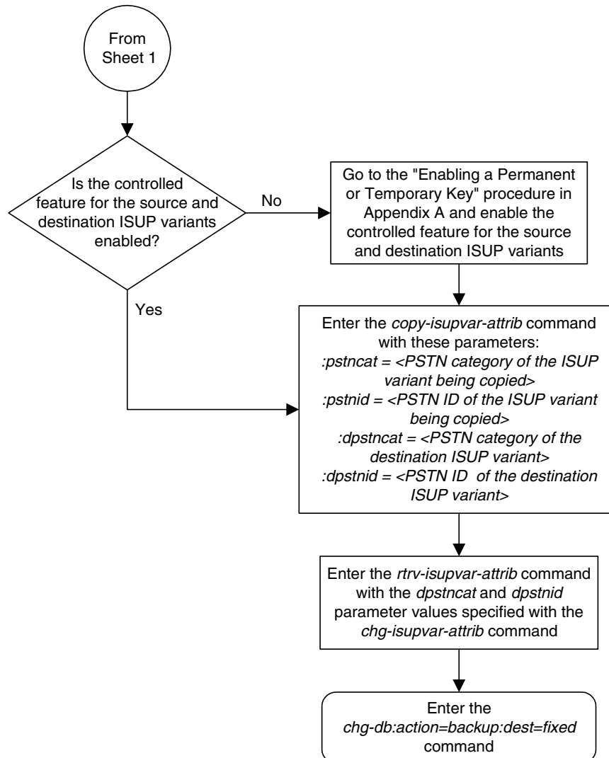
Flowchart 4-5. Copying ISUP Attribute Values (Sheet 2 of 2)
