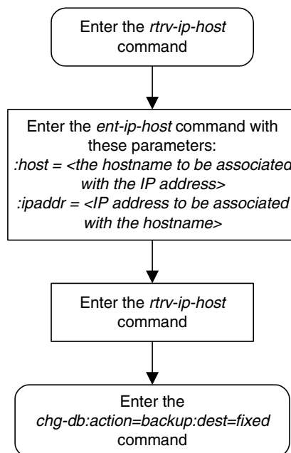
Flowchart 3-11. Adding an IP Host
