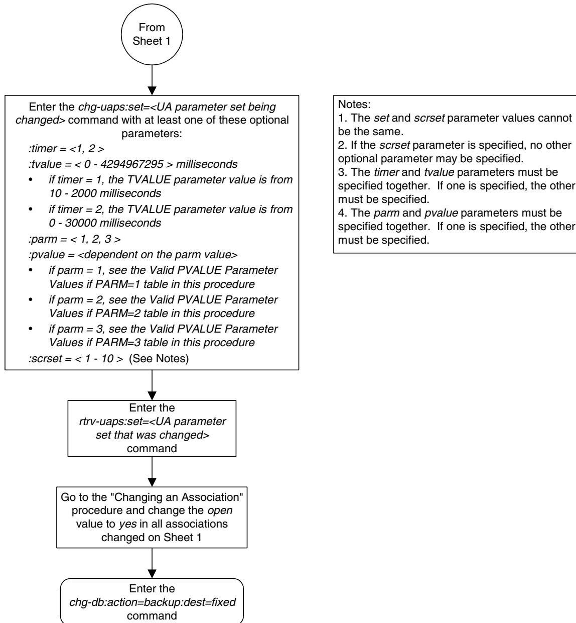
Flowchart 3-42. Changing a UA Parameter Set (Sheet 2 of 2)
