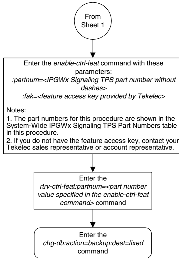
Flowchart 3-26. Increasing the IPGWx Signaling TPS (Sheet 1 of 2)
