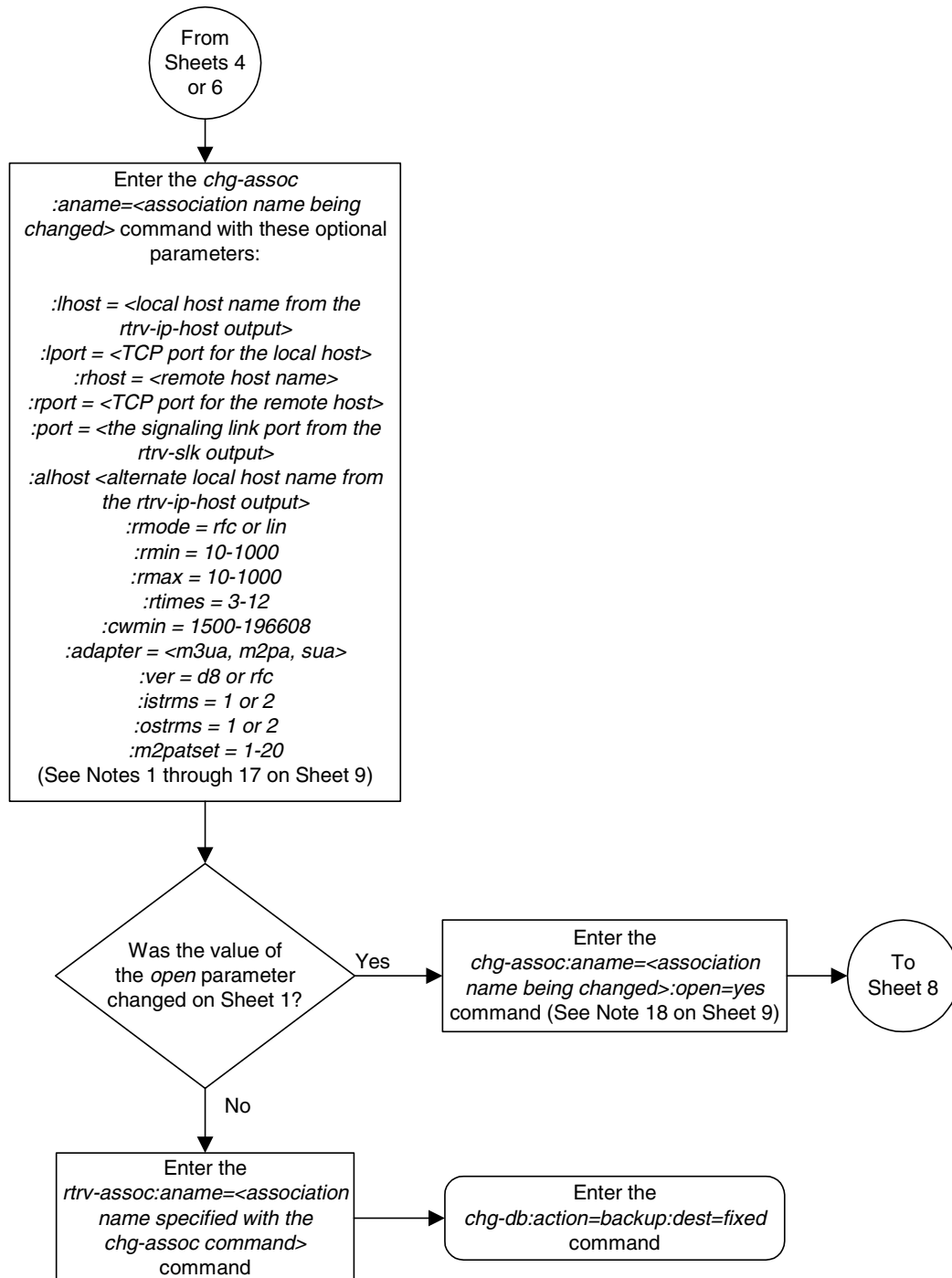
Flowchart 3-30. Changing an Association (Sheet 7 of 9)
