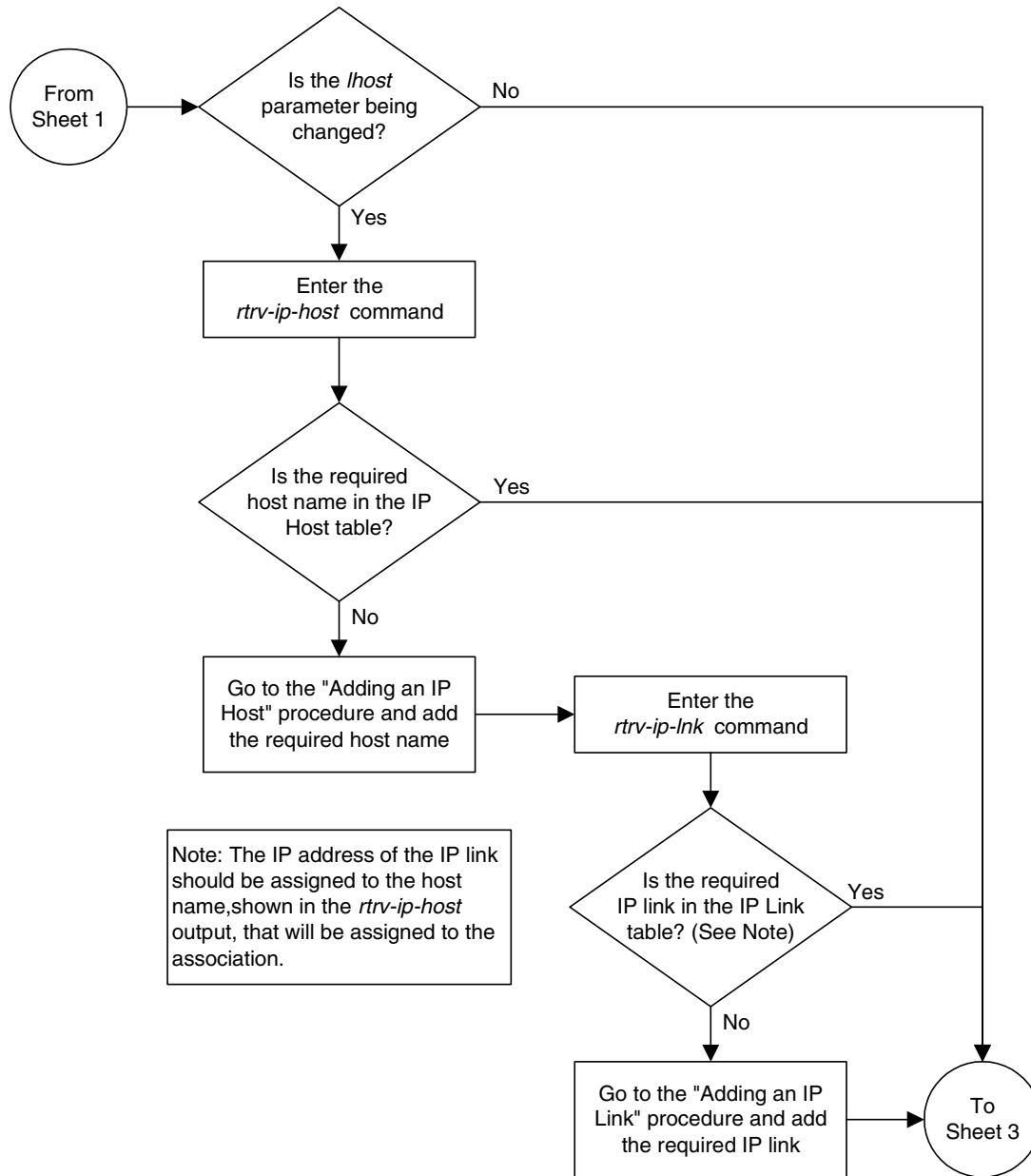
Flowchart 3-30. Changing an Association (Sheet 2 of 9)
