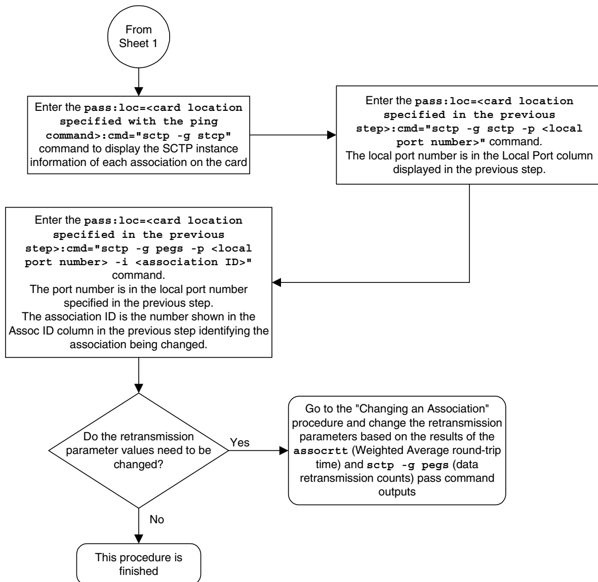
Flowchart 3-31. Configuring an Association for SCTP Retransmission Control (Sheet 2 of 2)
