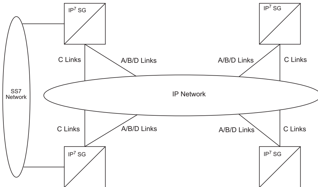
Figure 2-11. IP 7 Secure Gateway Network (STP Connectivity via MTP-over-IP)
