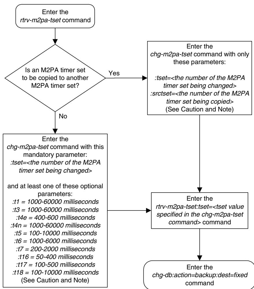
Flowchart 3-32. Changing an M2PA Timer Set
