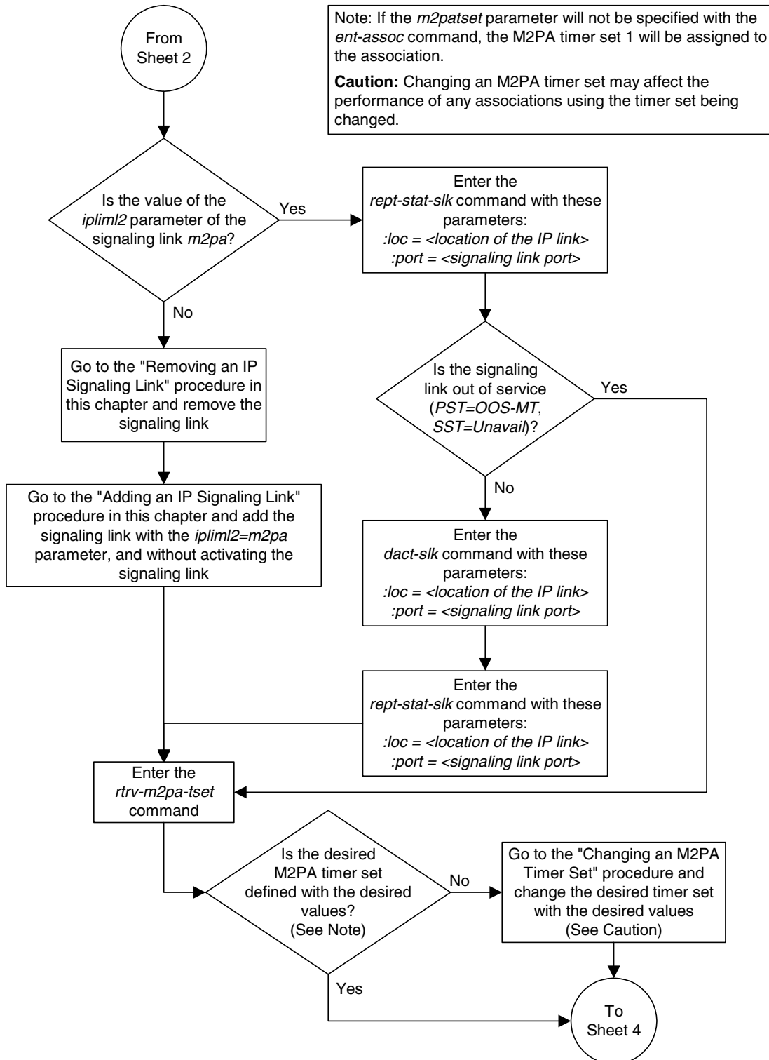
Flowchart 3-28. Adding an Association (Sheet 3 of 5)
