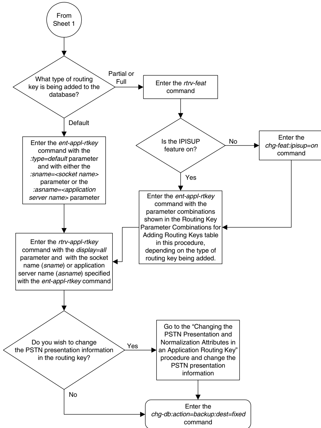
Flowchart 3-22. Adding an Application Routing Key (Sheet 2 of 2)
