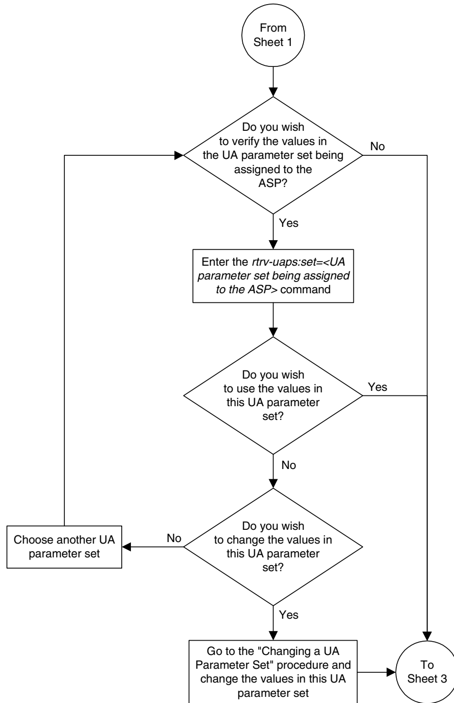
Flowchart 3-35. Changing an Application Server Process (Sheet 2 of 3)
