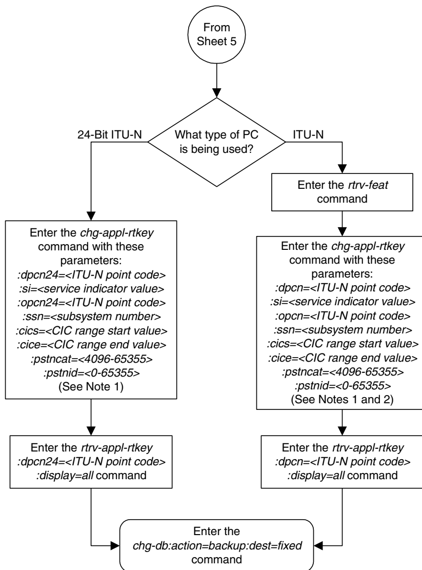
Flowchart 3-25. Changing the PSTN Presentation and Normalization Attributes in an Application Routing Key (Sheet 6 of 6)
