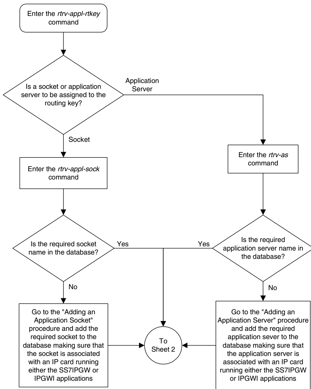
Flowchart 3-22. Adding an Application Routing Key (Sheet 1 of 2)
