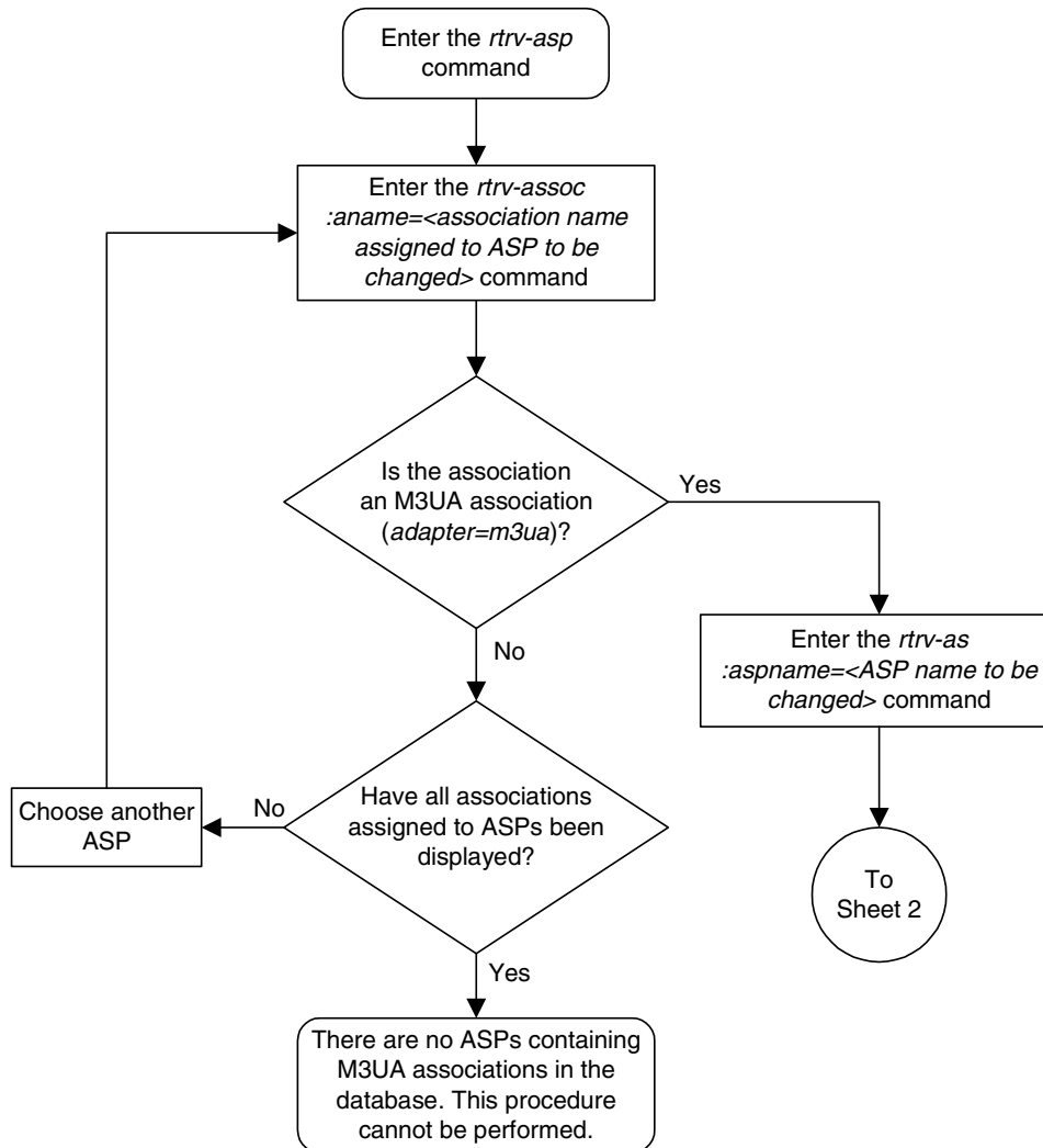
Flowchart 3-35. Changing an Application Server Process (Sheet 1 of 3)
