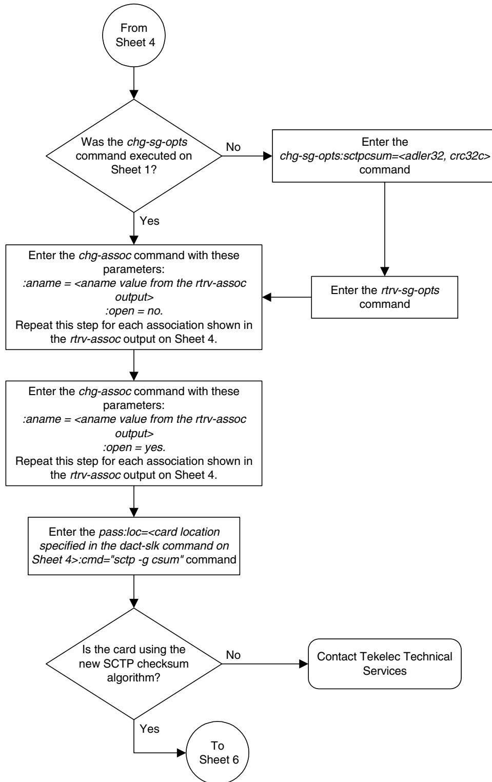
Flowchart 3-41. Changing the SCTP Checksum Option (Sheet 5 of 7)
