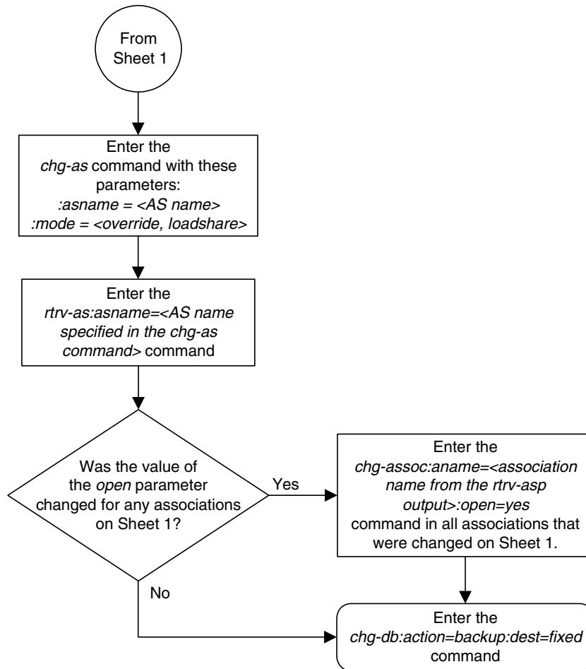
Flowchart 3-38. Changing an Application Server (Sheet 2 of 2)
