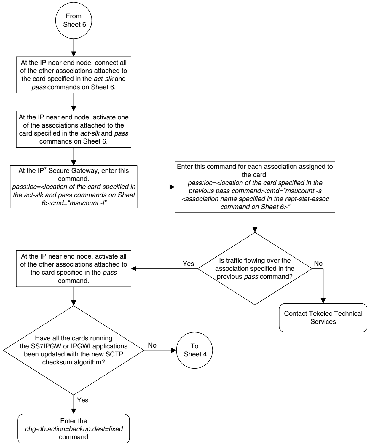
Flowchart 3-41. Changing the SCTP Checksum Option (Sheet 7 of 7)
