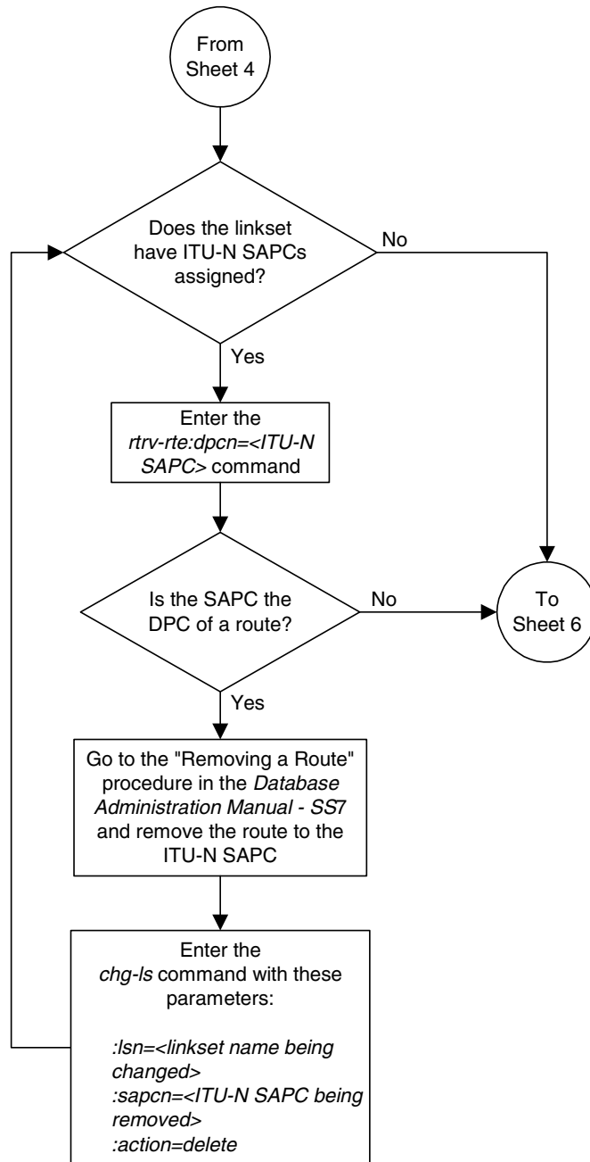
Flowchart 3-3. Configuring an IPGWx Linkset (Sheet 5 of 6)
