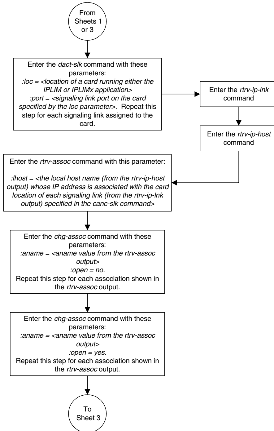
Flowchart 3-41. Changing the SCTP Checksum Option (Sheet 2 of 7)
