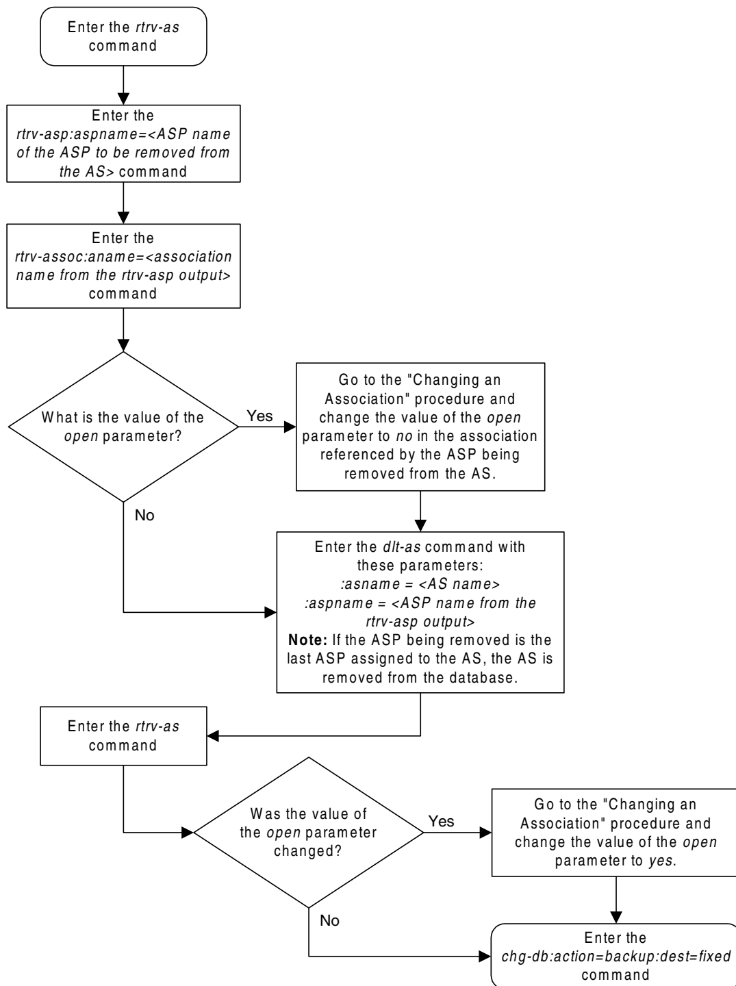
Flowchart 3-37. Removing an Application Server
