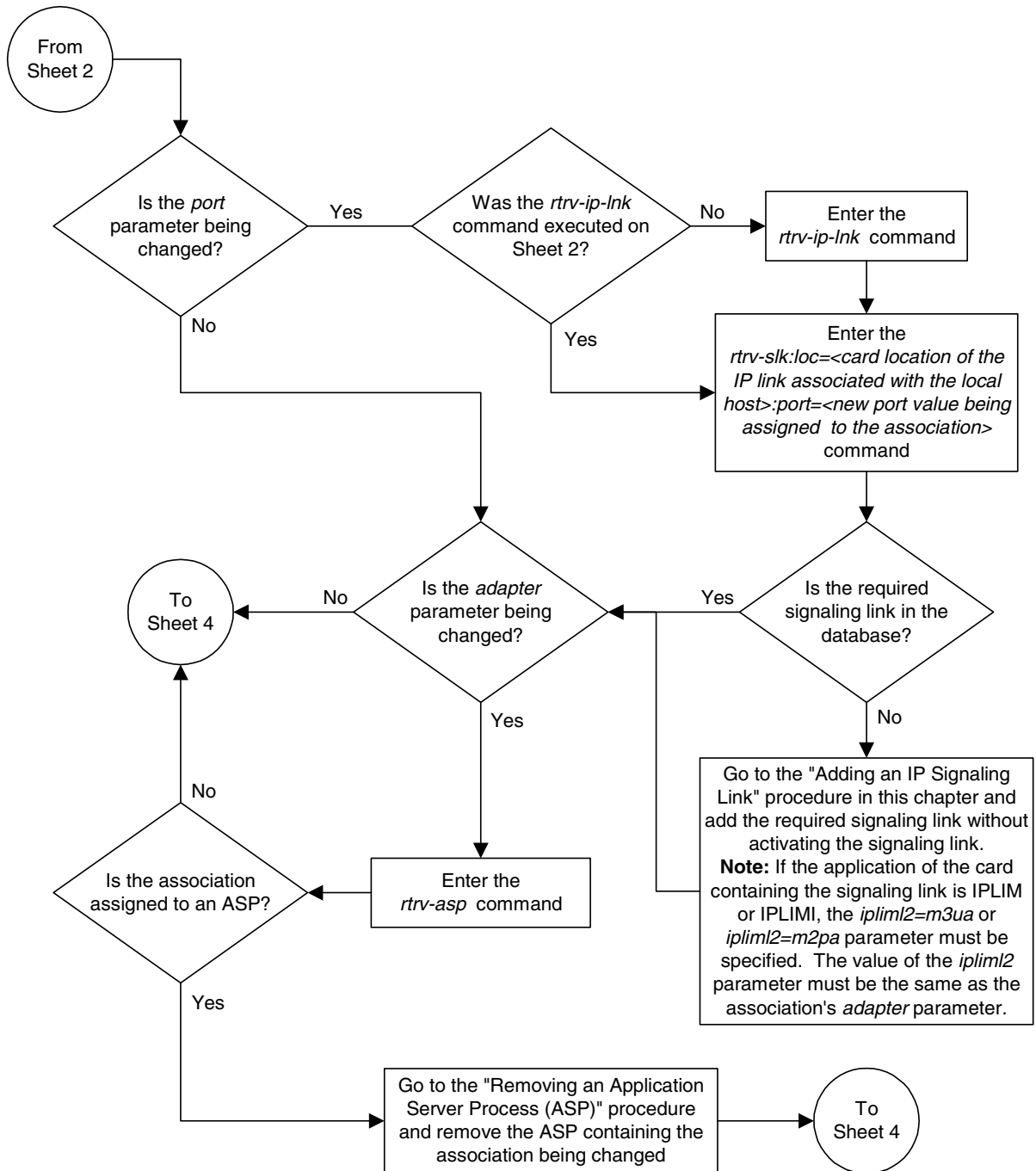
Flowchart 3-30. Changing an Association (Sheet 3 of 9)
