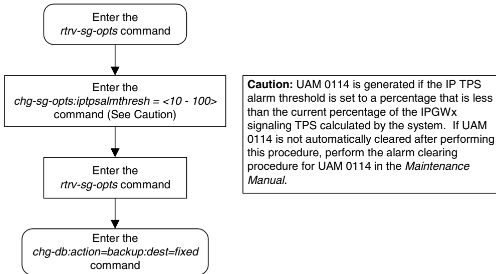
Flowchart 3-27. Configuring the IP TPS Alarm Threshold
