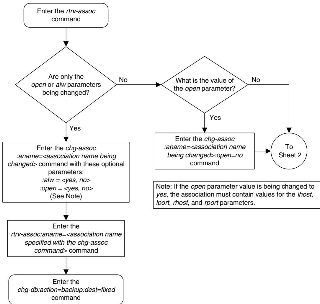
Flowchart 3-30. Changing an Association (Sheet 1 of 9)
