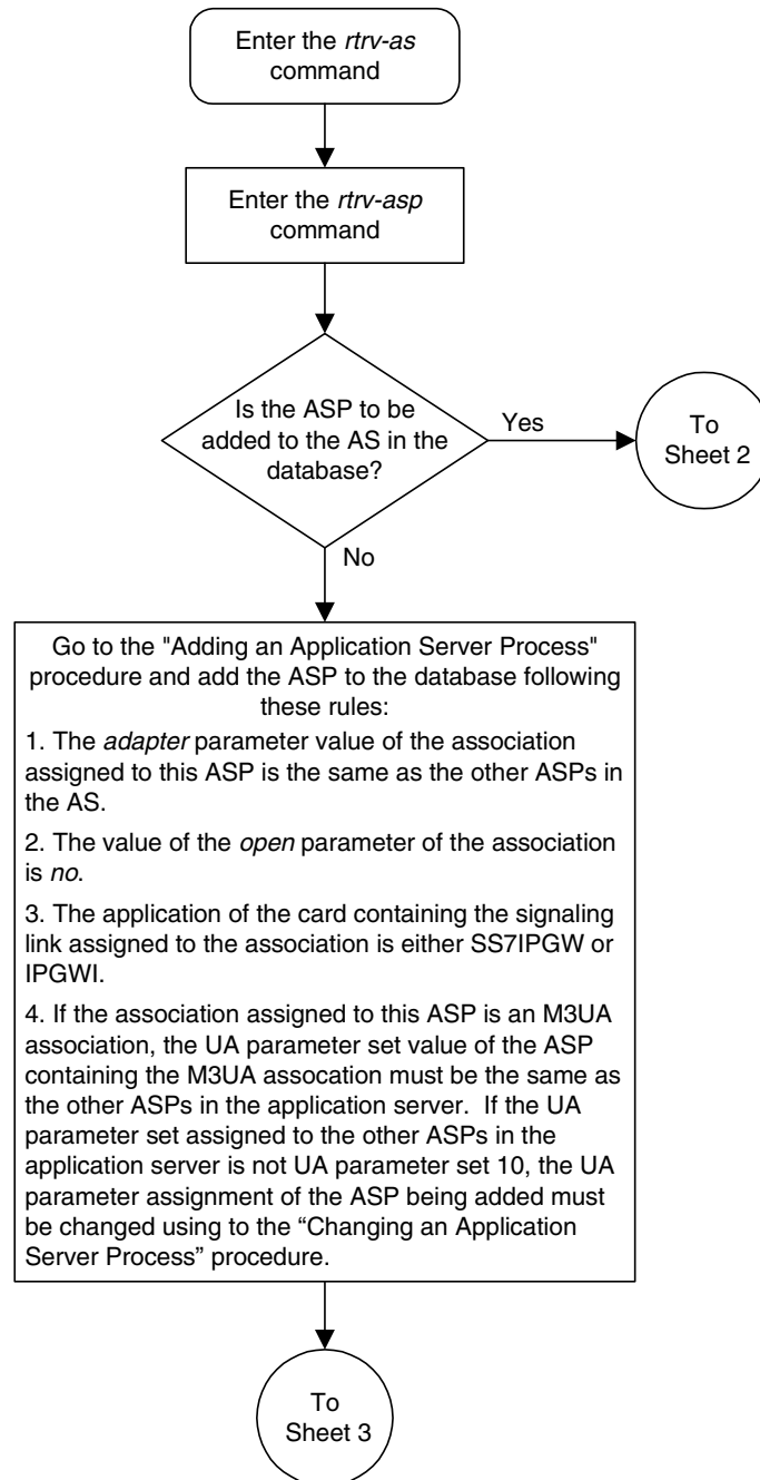
Flowchart 3-36. Adding an Application Server (Sheet 1 of 3)
