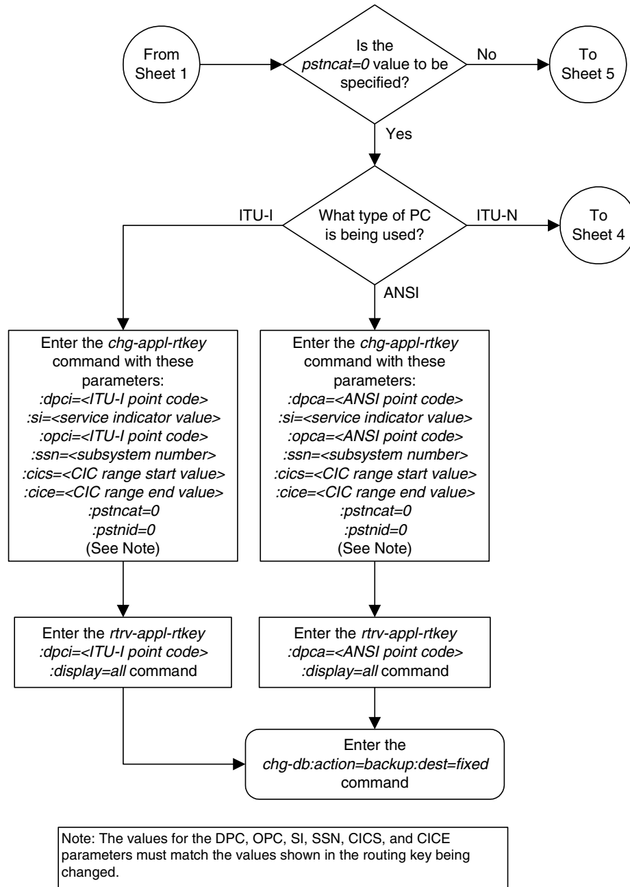
Flowchart 3-25. Changing the PSTN Presentation and Normalization Attributes in an Application Routing Key (Sheet 3 of 6)
