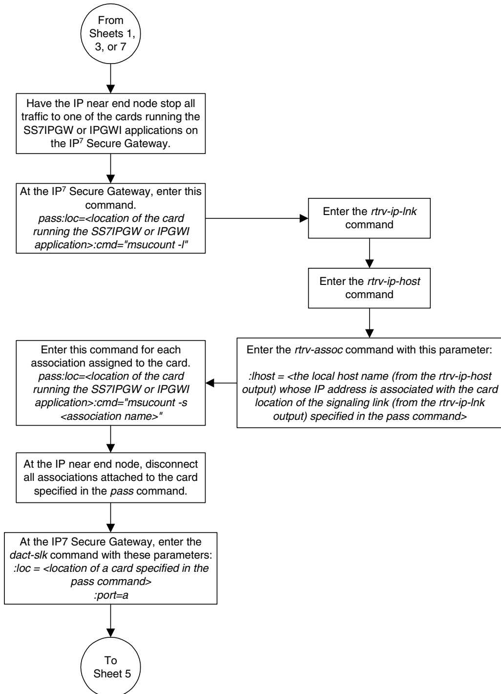
Flowchart 3-41. Changing the SCTP Checksum Option (Sheet 4 of 7)
