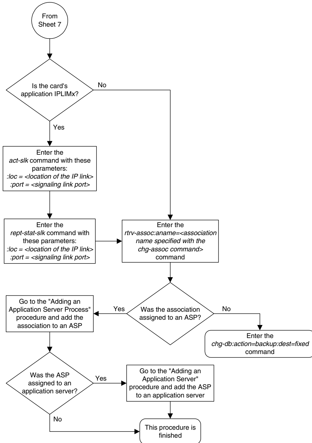
Flowchart 3-30. Changing an Association (Sheet 8 of 9)
