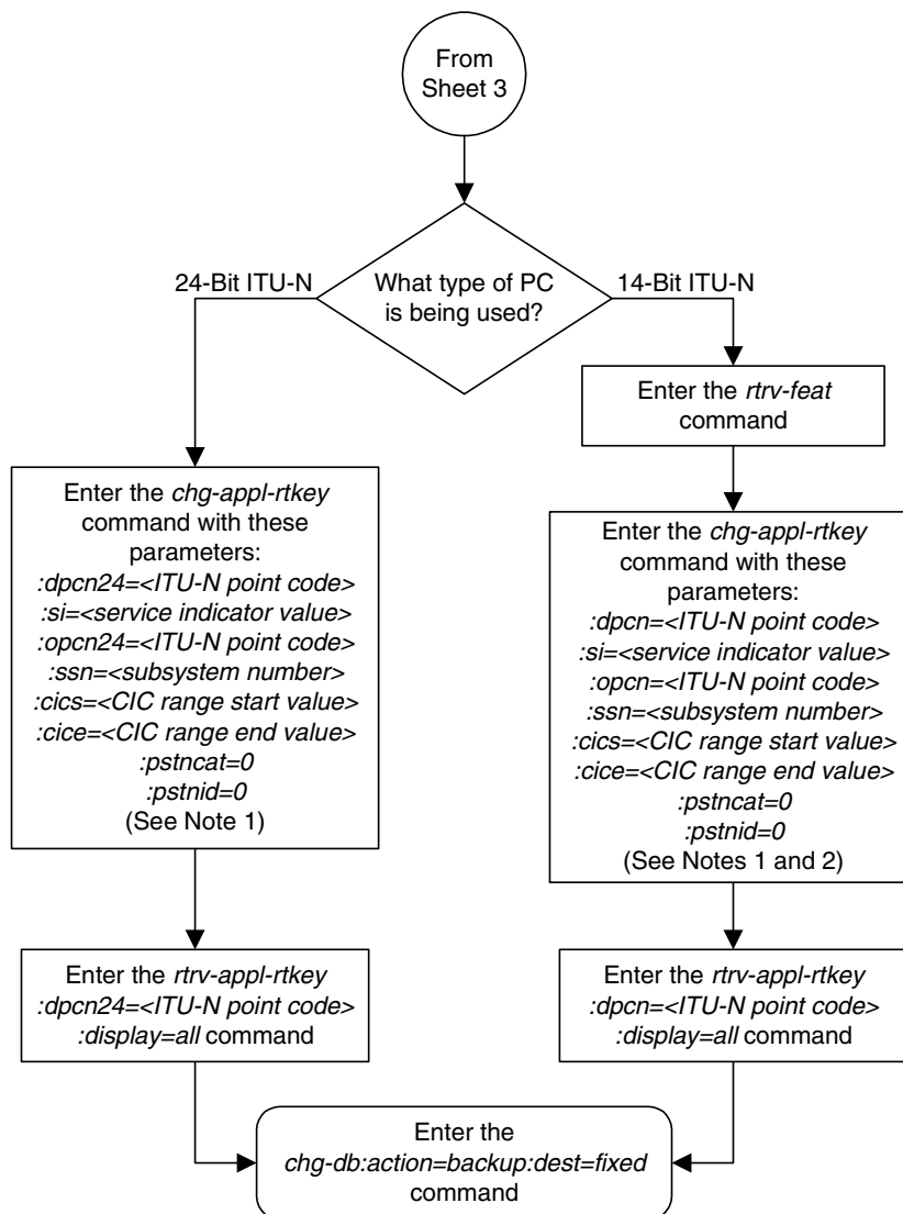
Flowchart 3-25. Changing the PSTN Presentation and Normalization Attributes in an Application Routing Key (Sheet 4 of 6)
