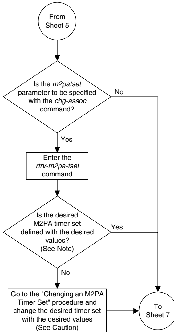
Flowchart 3-30. Changing an Association (Sheet 6 of 9)
