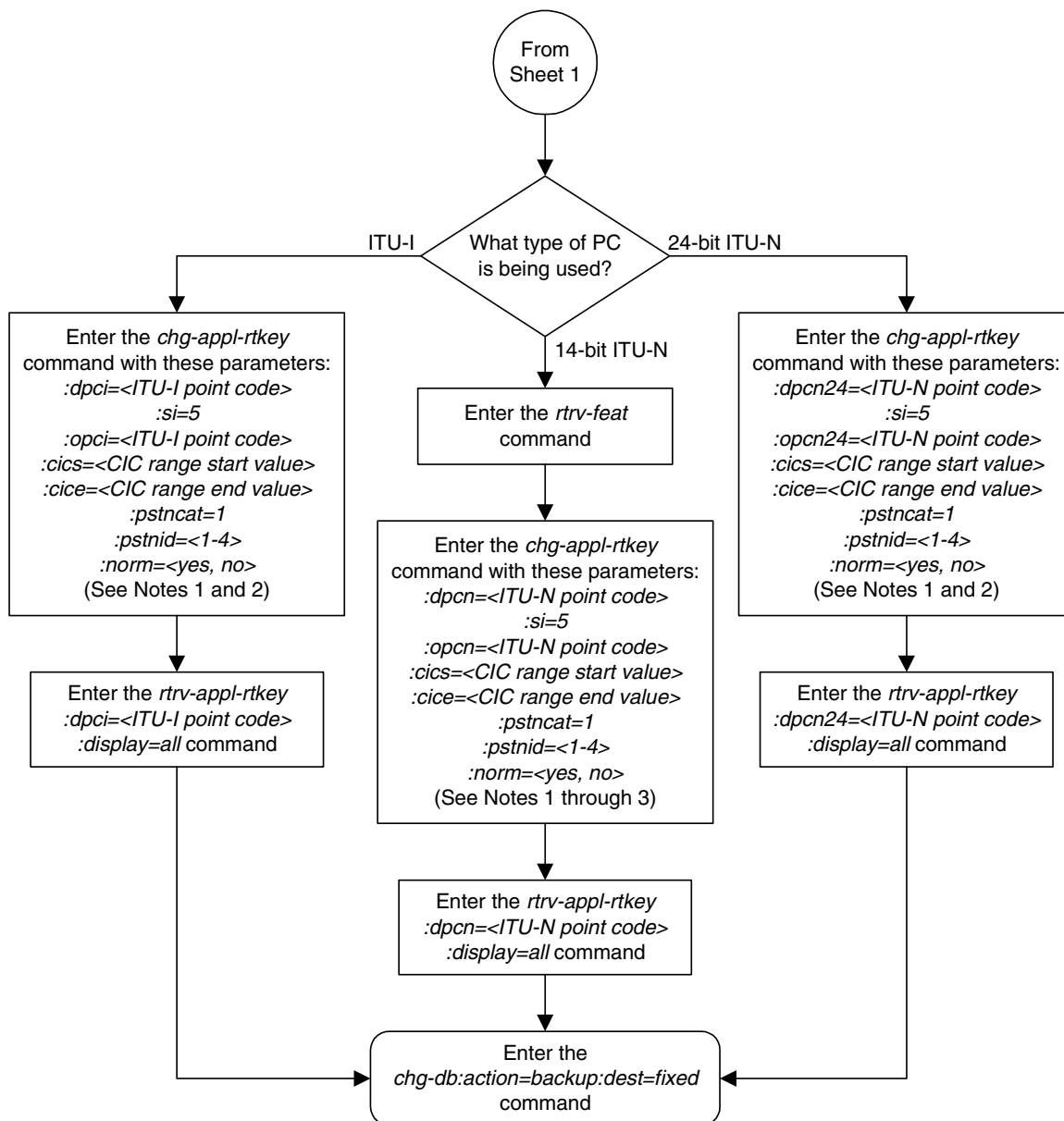
Flowchart 3-25. Changing the PSTN Presentation and Normalization Attributes in an Application Routing Key (Sheet 2 of 6)
