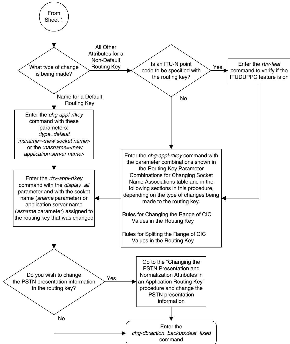
Flowchart 3-24. Changing a Static Application Routing Key (Sheet 2 of 2)
