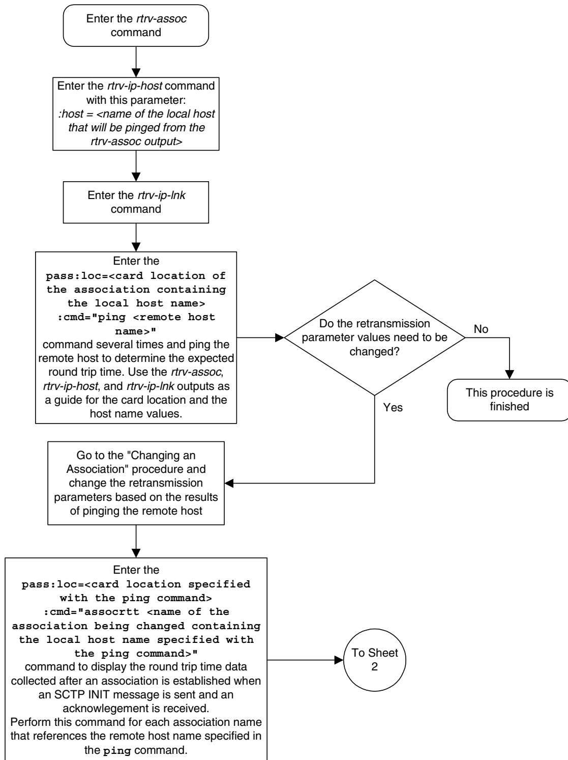
Flowchart 3-31. Configuring an Association for SCTP Retransmission Control (Sheet 1 of 2)
