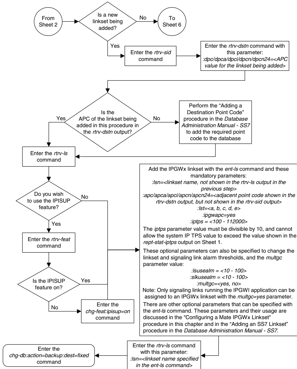
Flowchart 3-3. Configuring an IPGWx Linkset (Sheet 3 of 6)
