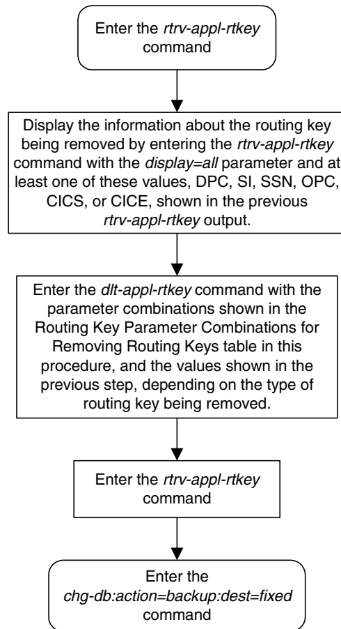
Flowchart 3-23. Removing an Application Routing Key
