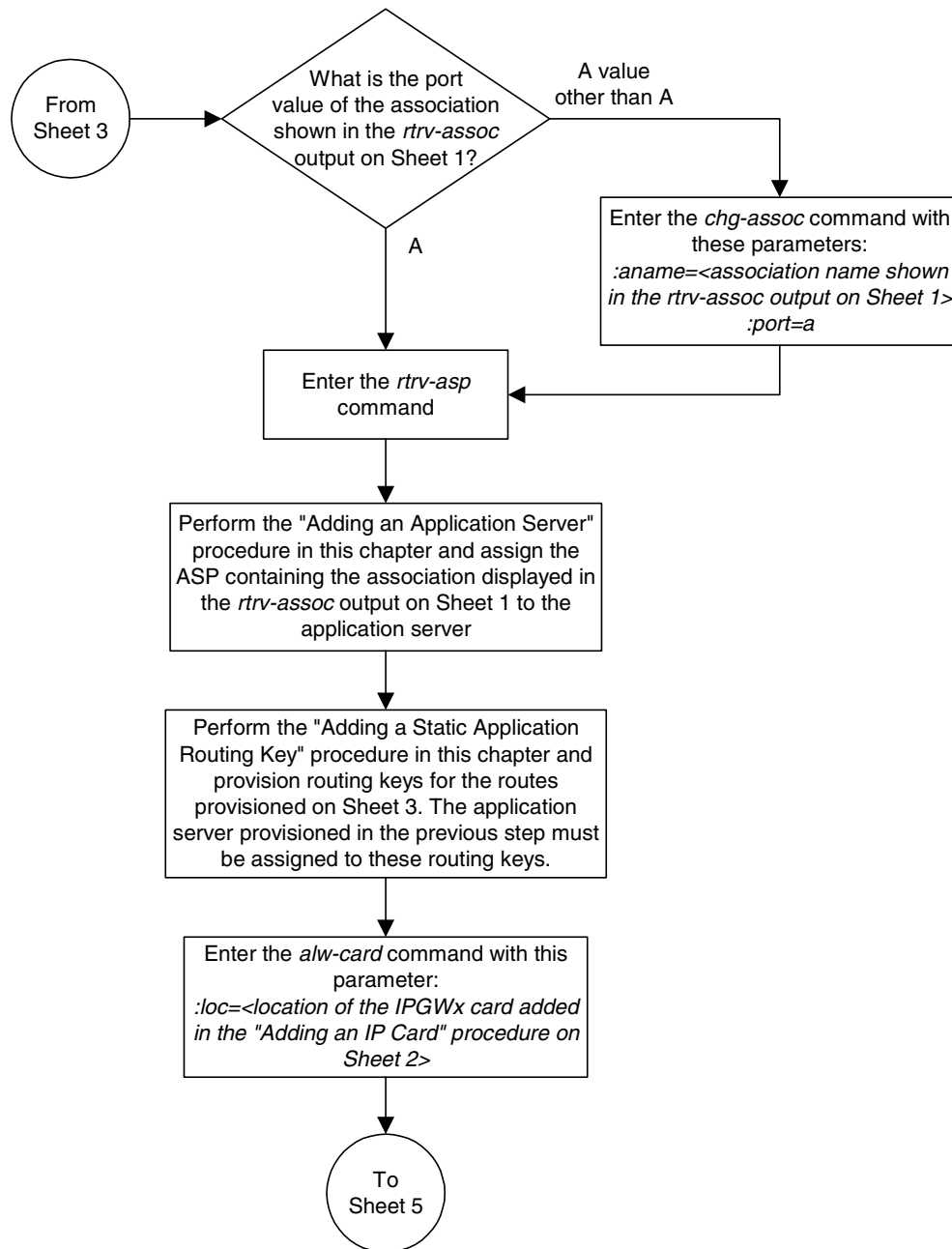
Flowchart 3-8. Migrating IPLIMx M3UA Signaling Links to IPGWx M3UA Connections (Sheet 4 of 6)
