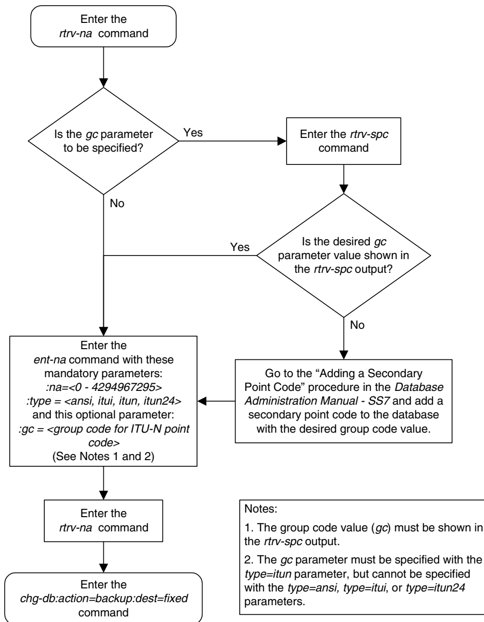
Flowchart 3-39. Adding a Network Appearance
