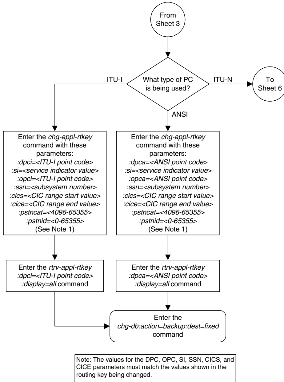
Flowchart 3-25. Changing the PSTN Presentation and Normalization Attributes in an Application Routing Key (Sheet 5 of 6)
