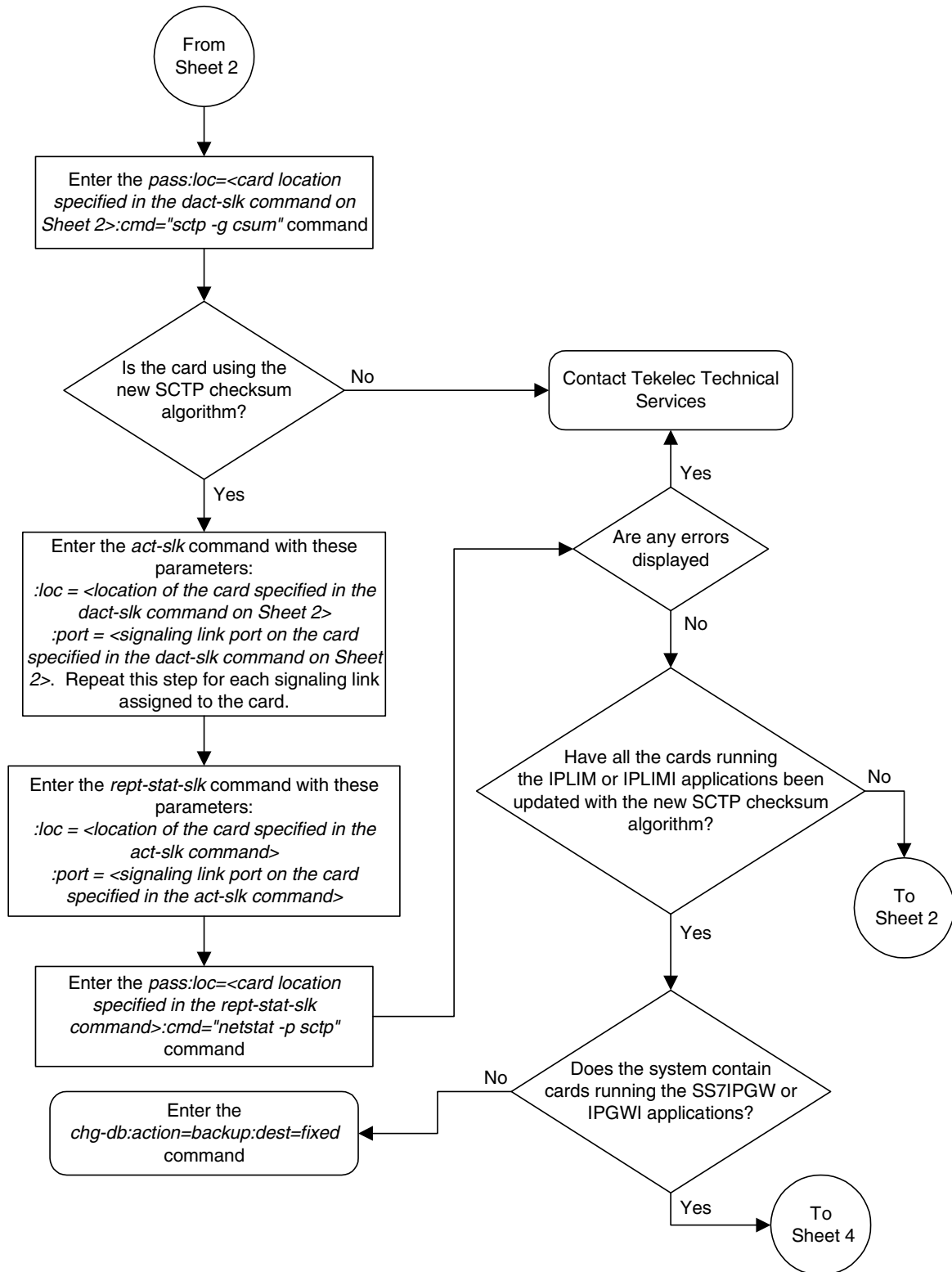
Flowchart 3-41. Changing the SCTP Checksum Option (Sheet 3 of 7)
