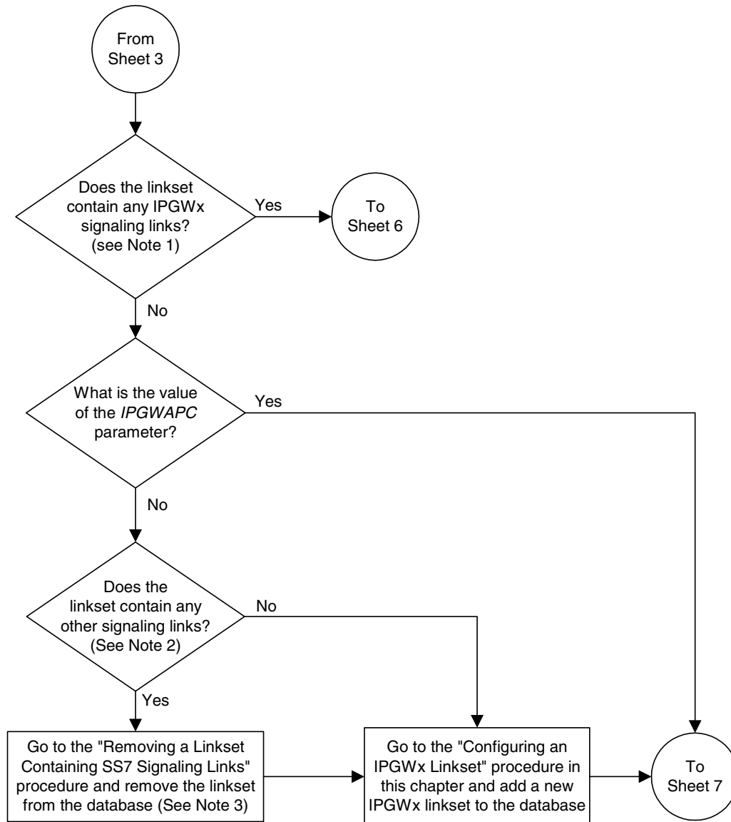
Flowchart 3-5. Adding an IP Signaling Link (Sheet 5 of 7)
