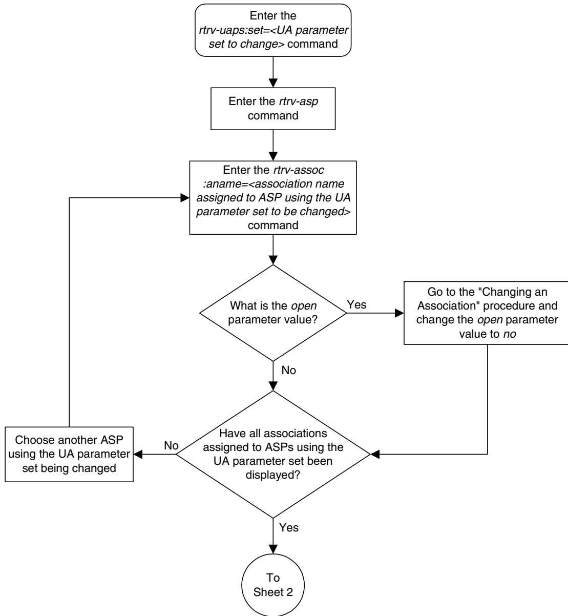
Flowchart 3-42. Changing a UA Parameter Set (Sheet 1 of 2)
