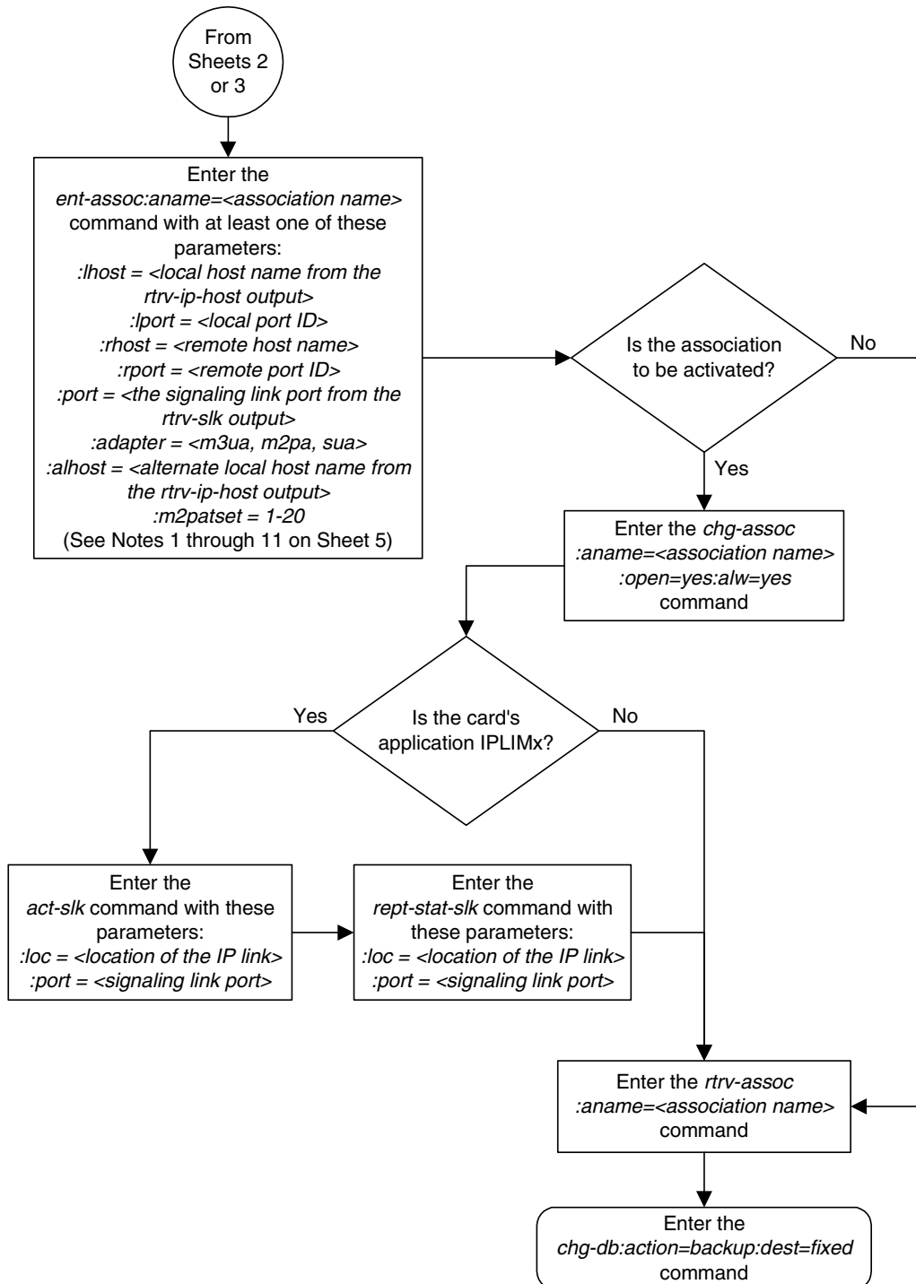
Flowchart 3-28. Adding an Association (Sheet 4 of 5)
