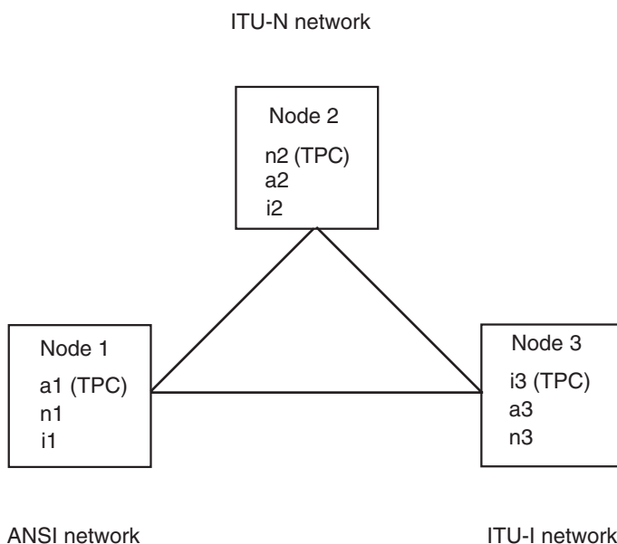
Figure 3-1. Mixed Network with ANSI, ITU-I, and ITU-N Nodes
