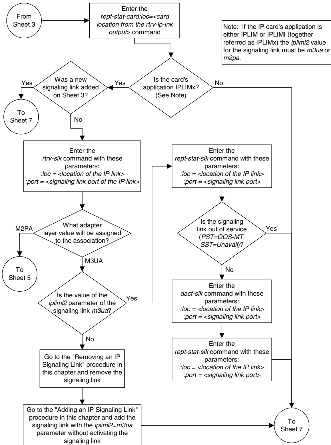
Flowchart 3-30. Changing an Association (Sheet 4 of 9)
