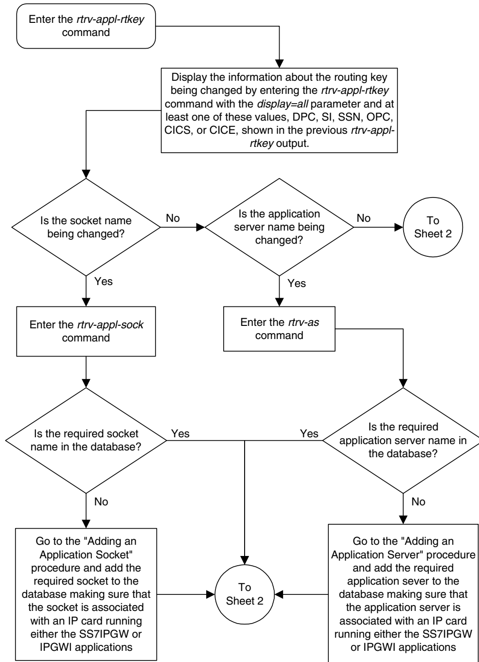
Flowchart 3-24. Changing a Static Application Routing Key (Sheet 1 of 2)
