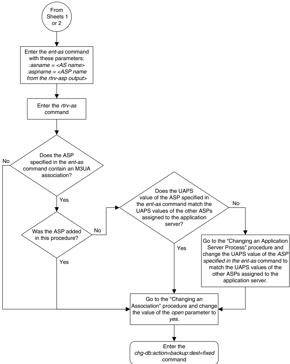
Flowchart 3-36. Adding an Application Server (Sheet 3 of 3)
