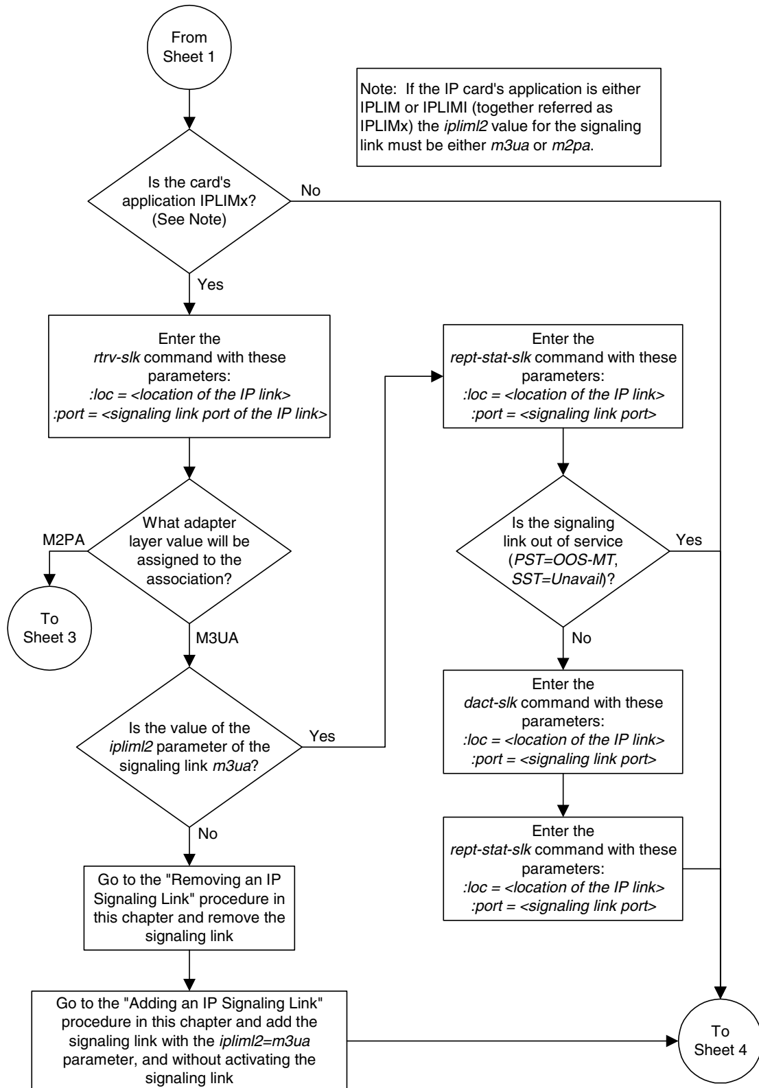
Flowchart 3-28. Adding an Association (Sheet 2 of 5)
