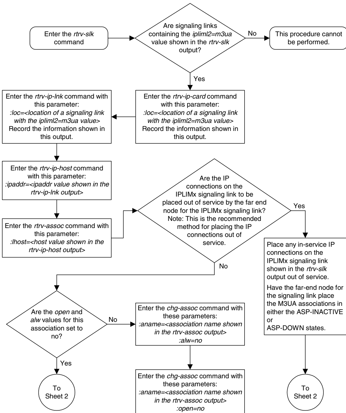
Flowchart 3-8. Migrating IPLIMx M3UA Signaling Links to IPGWx M3UA Connections (Sheet 1 of 6)
