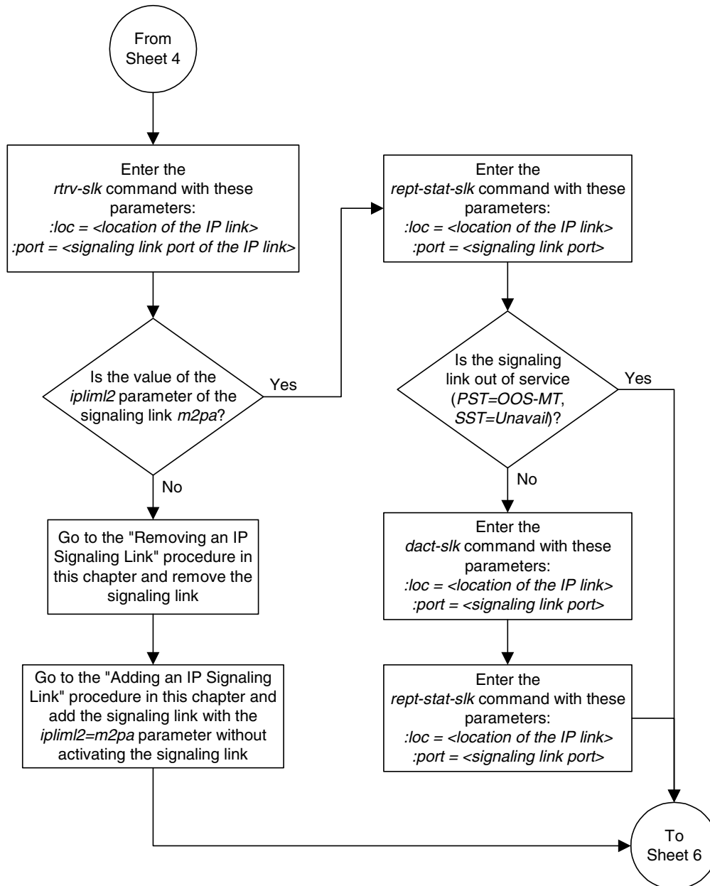
Flowchart 3-30. Changing an Association (Sheet 5 of 9)
