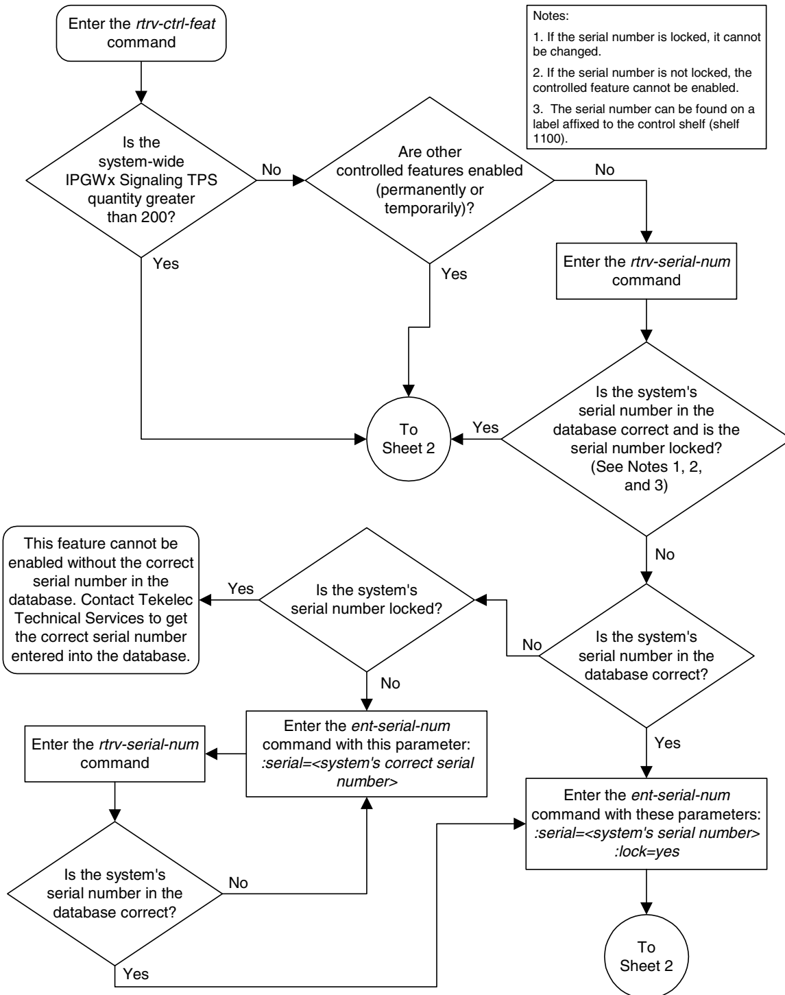
Flowchart 3-26. Increasing the IPGWx Signaling TPS (Sheet 1 of 2)
