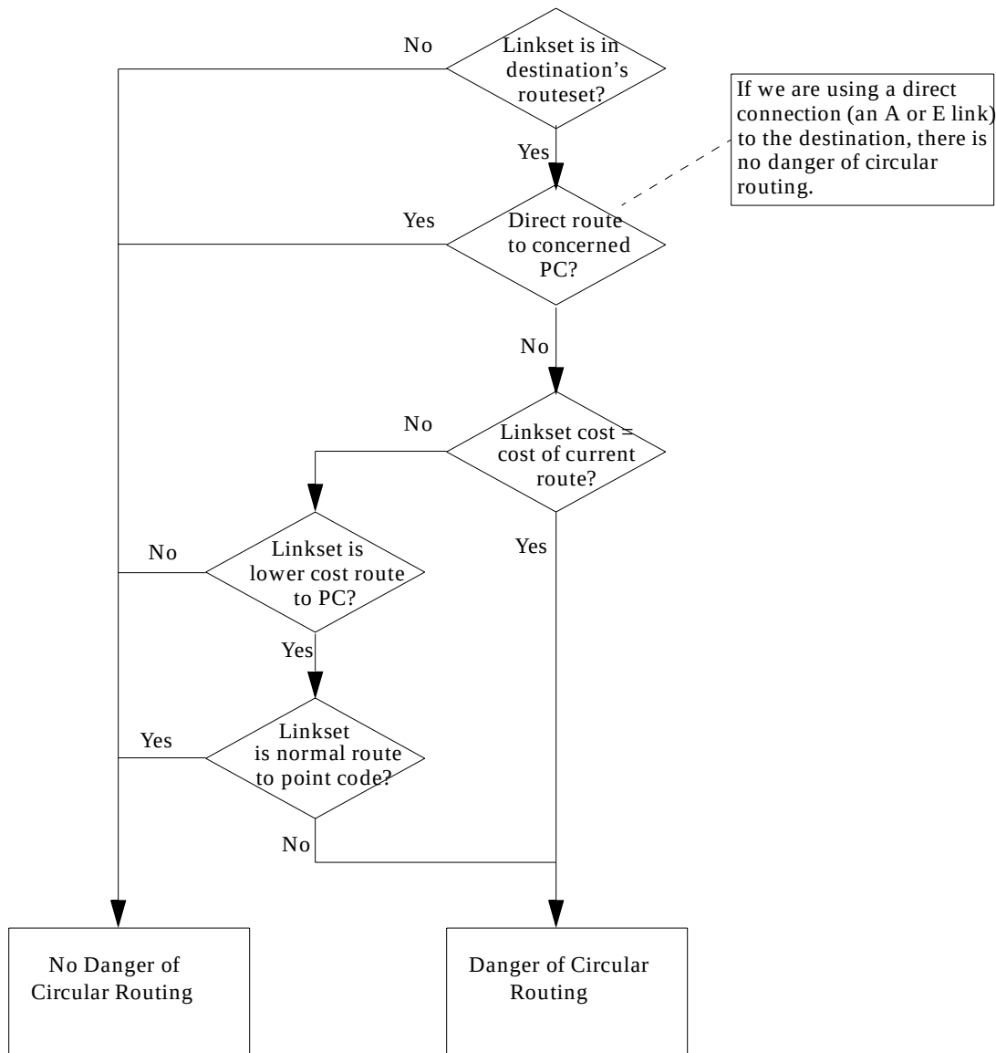
Figure 4-27. Determining If Danger of Circular Routing Exists
