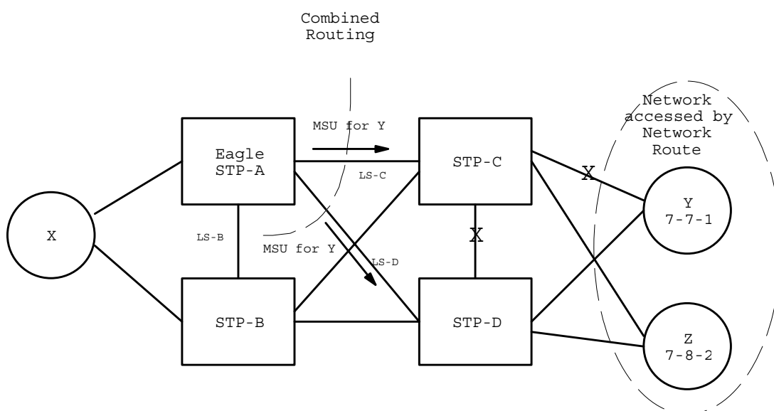
Figure 4-32. Potential Routing Network Failure
