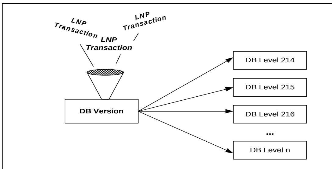
Figure 5-25. Database Levels
