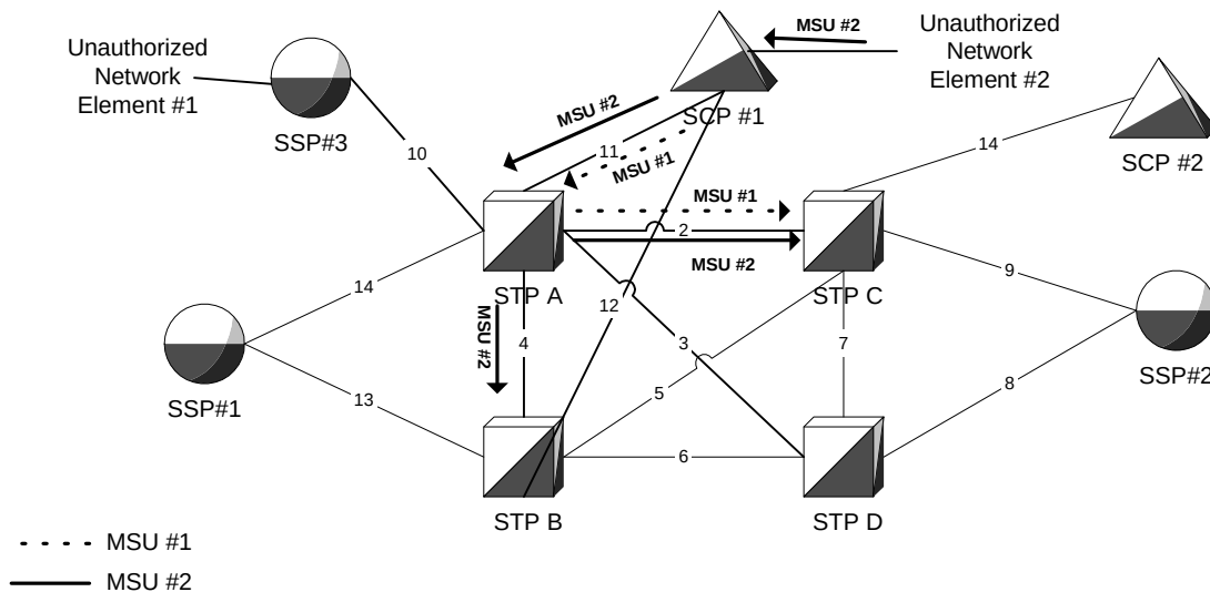
Figure 4-37. SECSCCPSCMG Option Diagram
