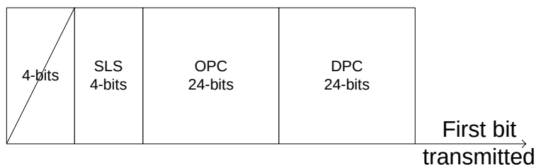
Figure 2-1. Routing Label Structure
