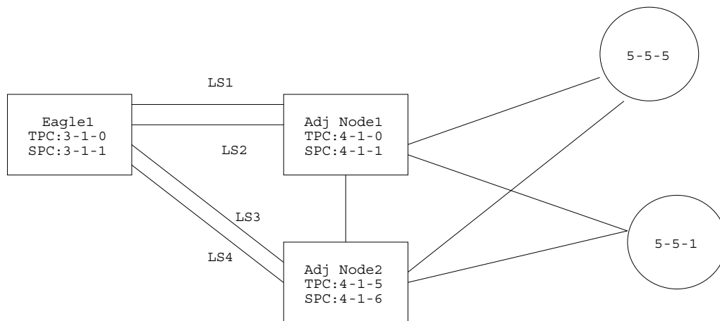
Figure 4-24. Multiple Linkset Example
