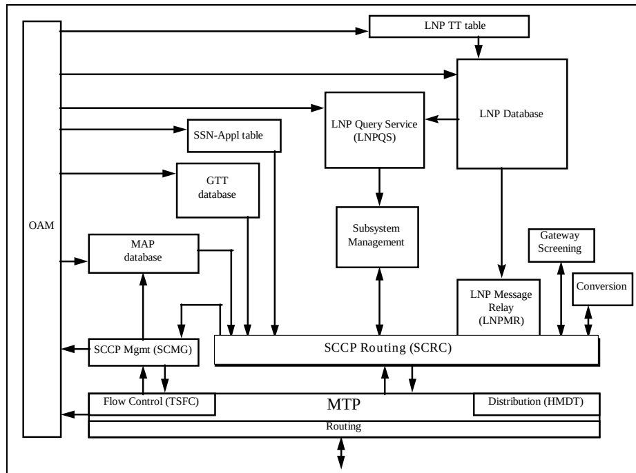
Figure 4-11. LNP Block Diagram
