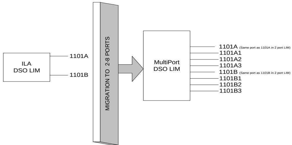
Figure 4-25. Multi-Port LIM to 2-Port LIM Relationship
