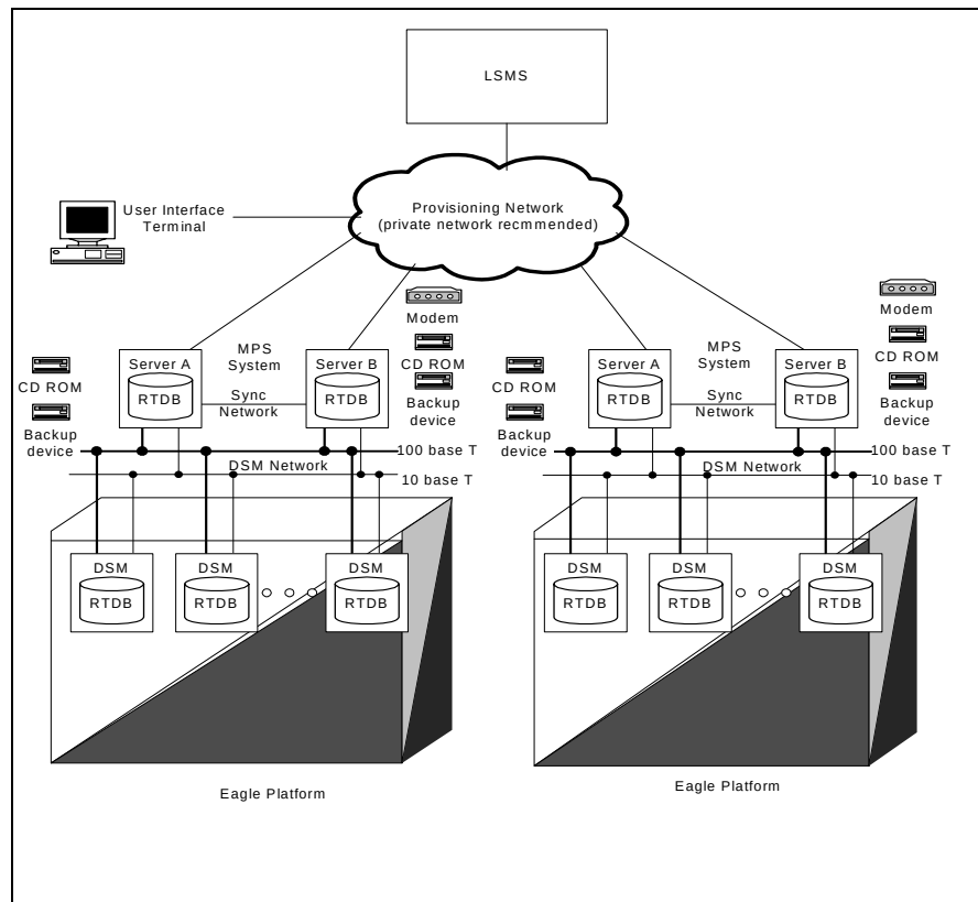
Figure 4-4. LNP 48/96 Million System Architectural Overview
