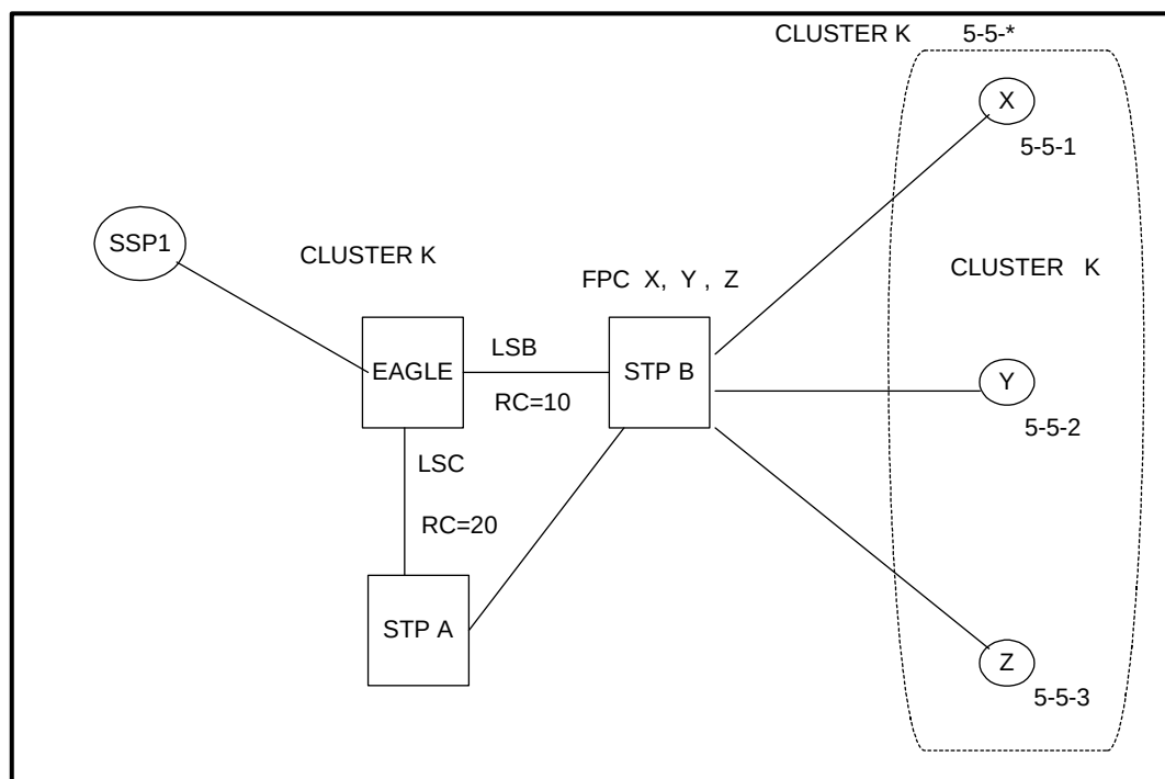
Figure 4-28. Preventive TCP Example
