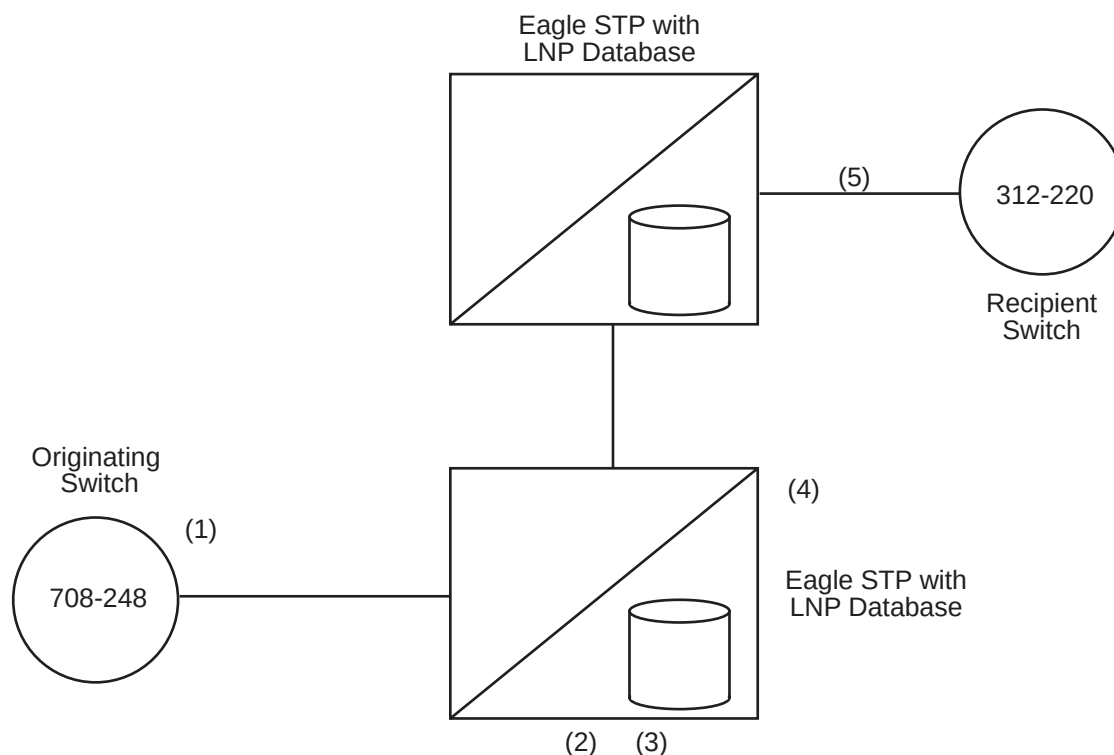
Figure 4-14. Internetwork Class Query
