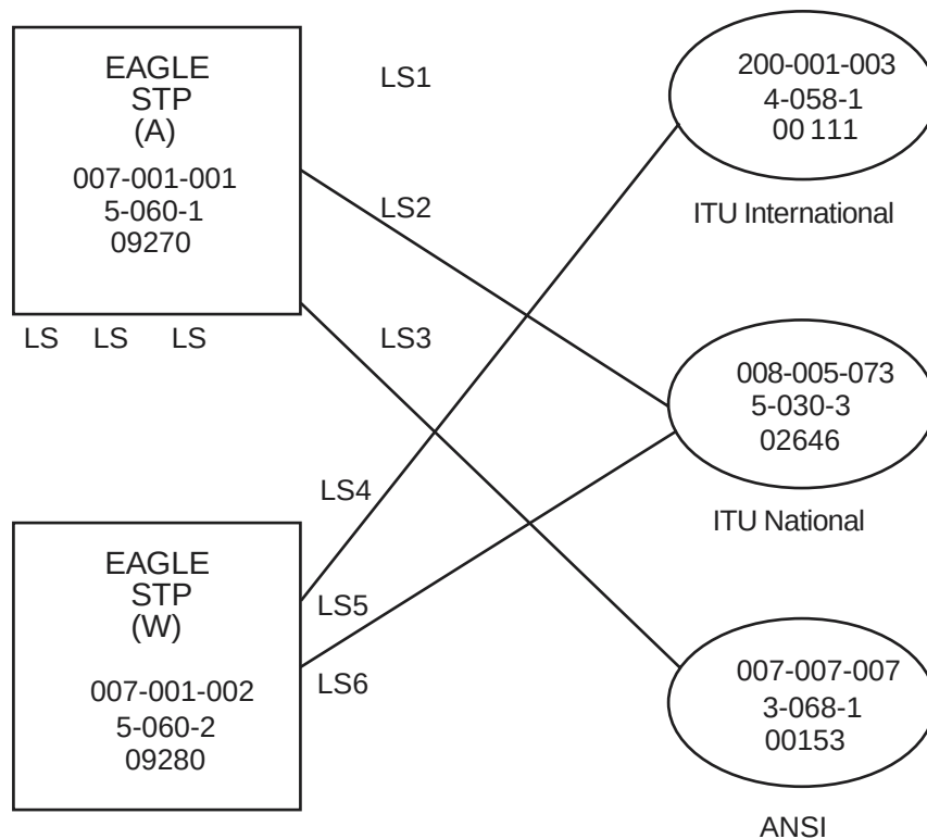
Figure 2-5. Sample Gateway STP Network
