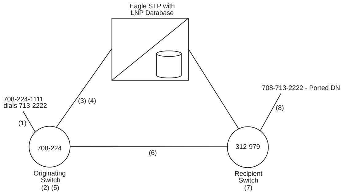
Figure 4-16. LNP Query Routed as a Non-Final Global Title Translation
