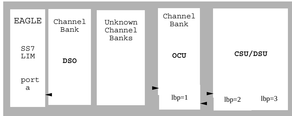
Figure 4-21. OCU/DCU link LBPs for NLT
