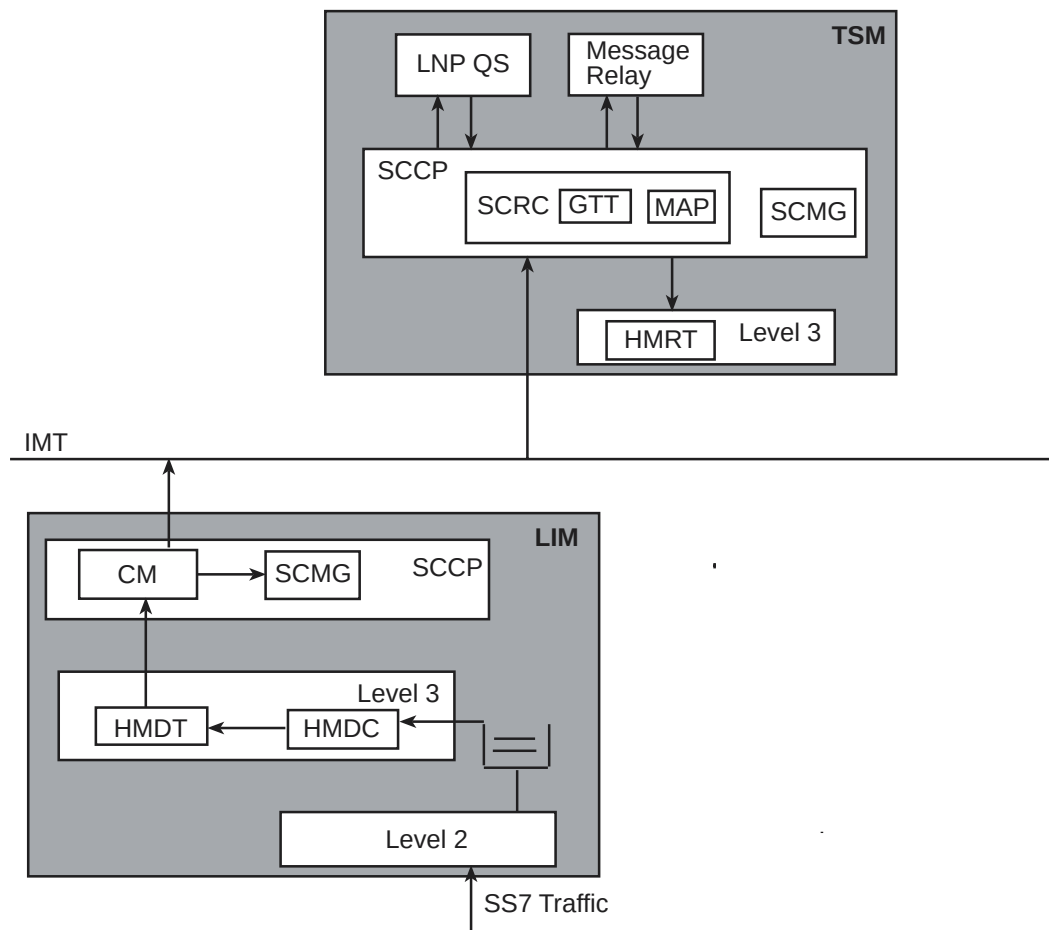
Figure 4-17. SCMG on the LIM
