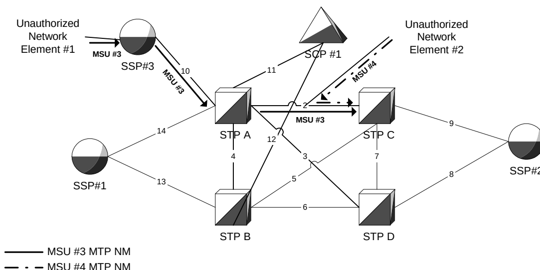
Figure 4-36. SECMTPSNM B-C-D link Option Diagram
