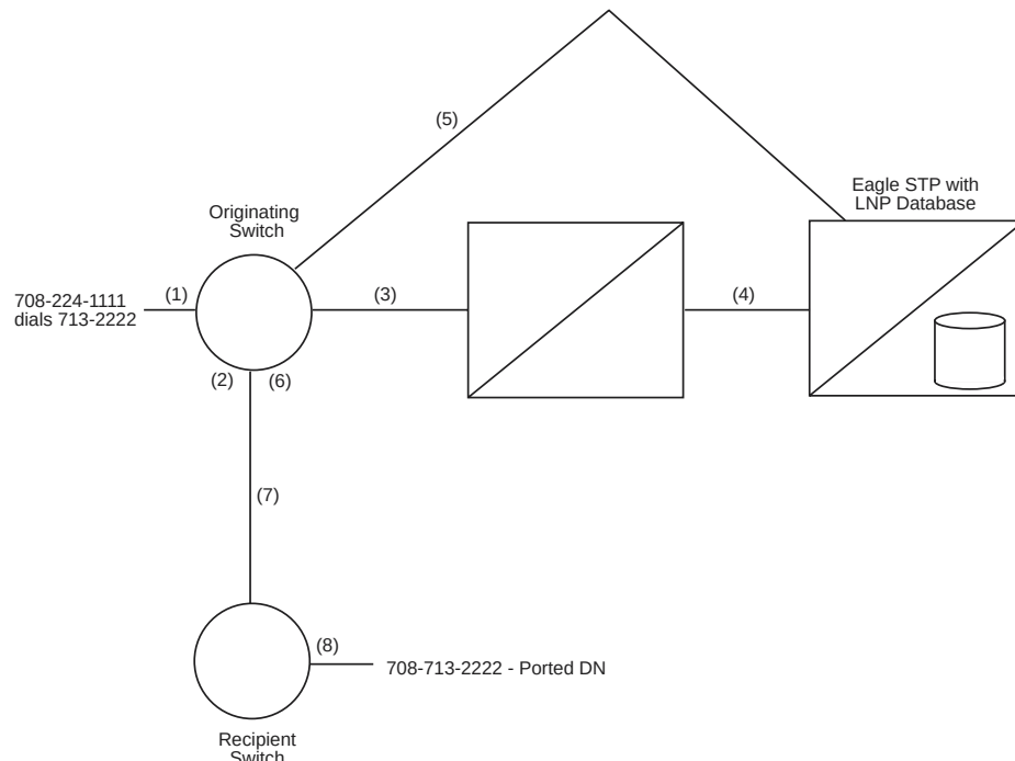
Figure 4-13. LNP Query Routed as Final Global Title Translation
