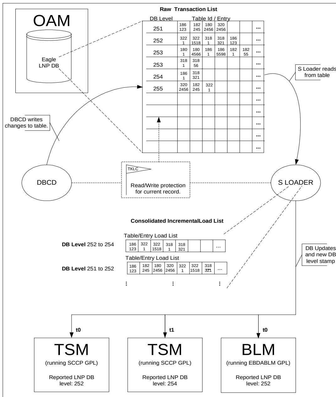
Figure 5-27. LNP Data Tracking and Loading Overview
