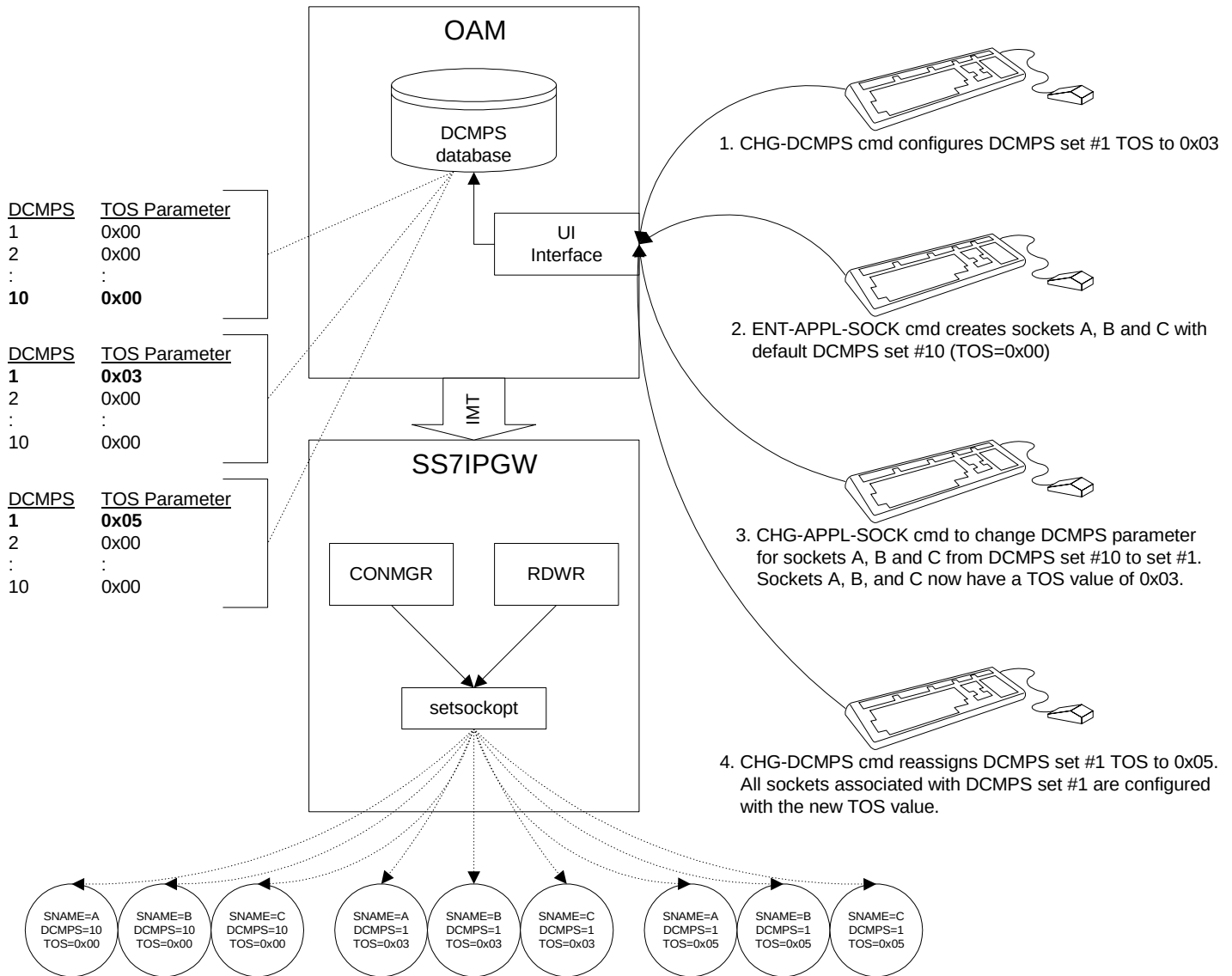
Figure 5-13. ToS Setup
