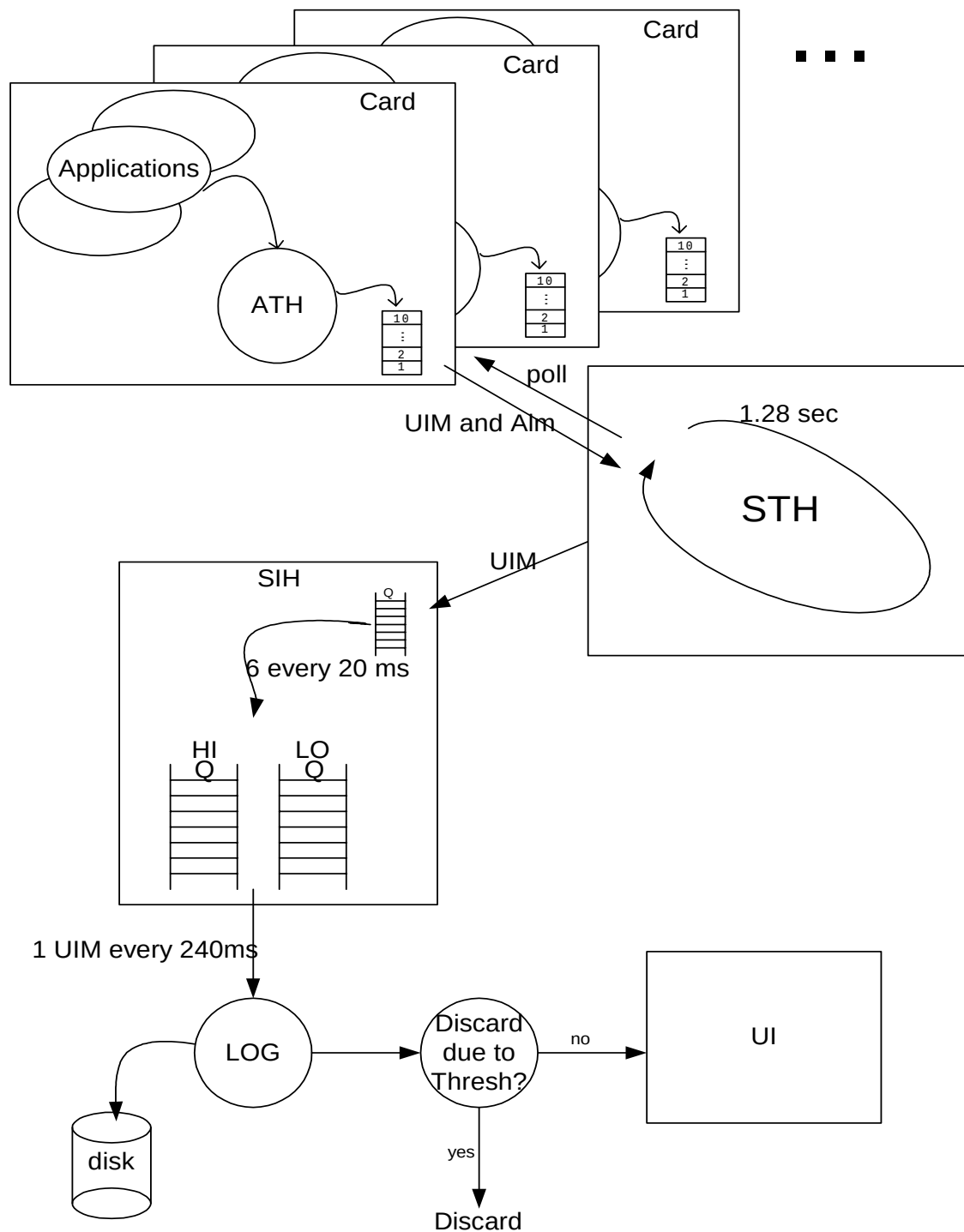
Figure 5-24. Depiction of UIM Creation, Logging, and Thresholding
