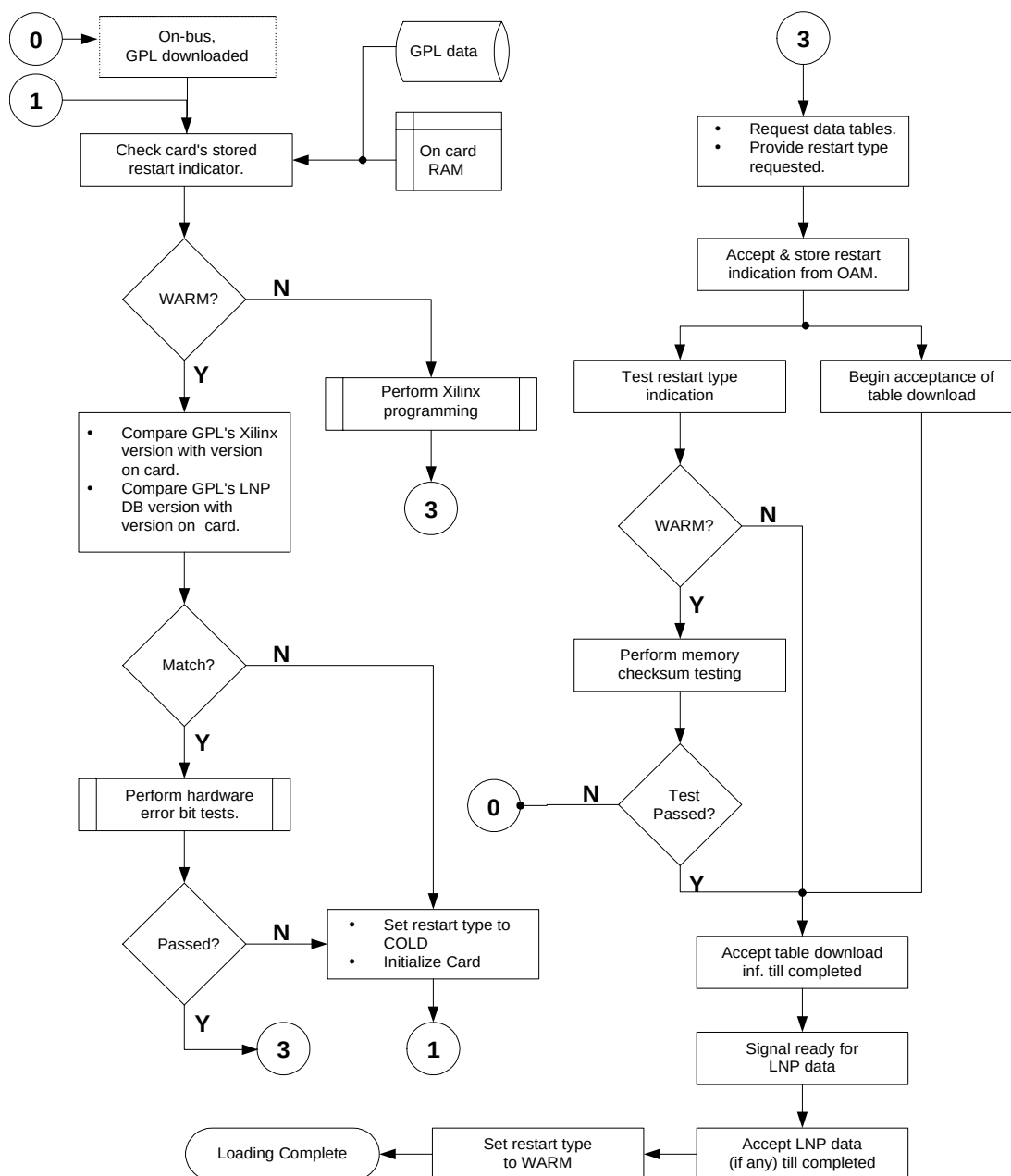
Figure 5-26. On-Card Warm Restart Decision Flow
