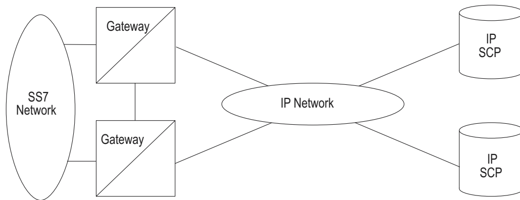
Figure 4-38. Non SCCP /ISUP Routing
