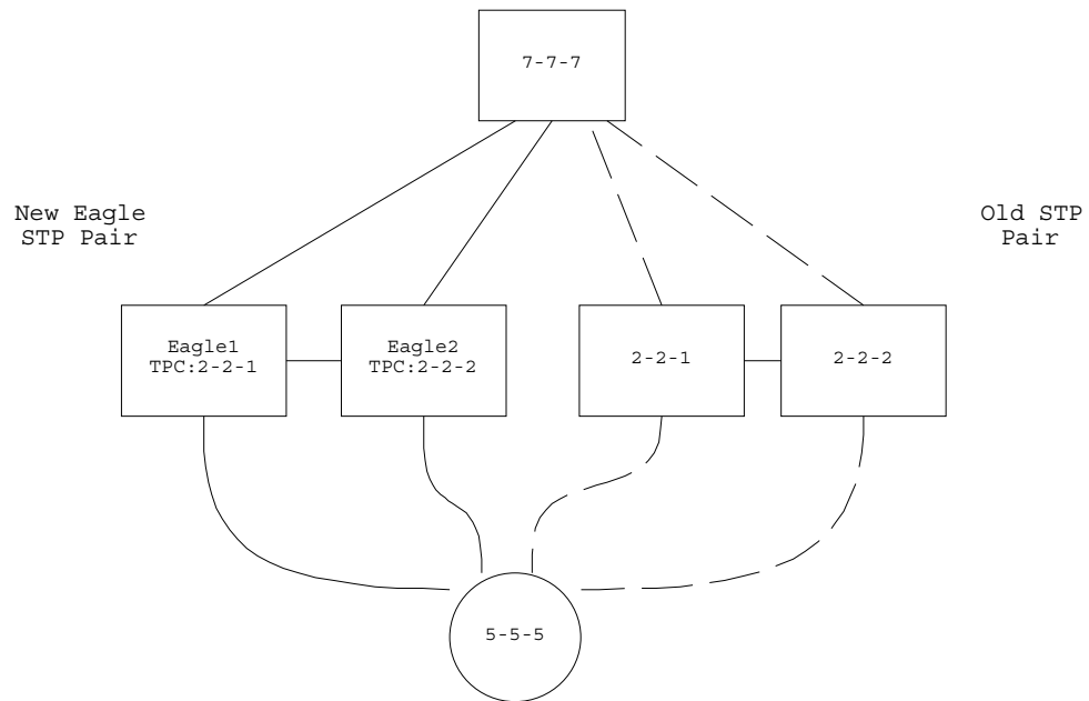
Figure 4-22. Replacing the First STP Pair
