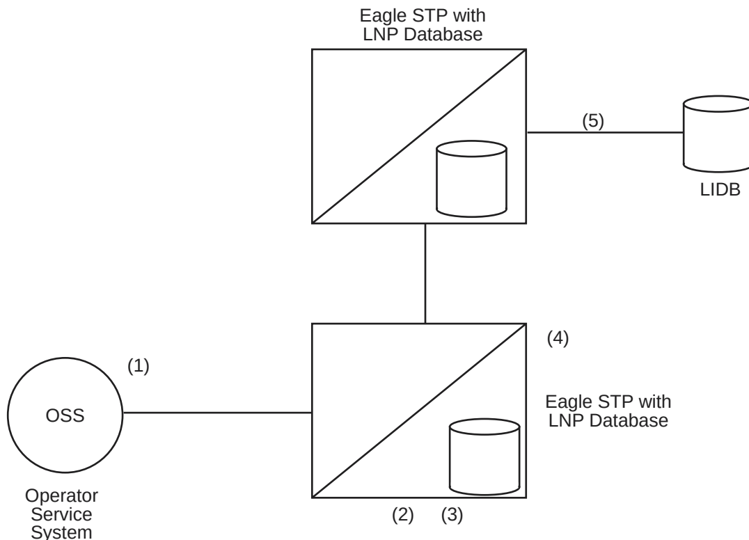
Figure 4-15. Internetwork LIDB Query with 6-Digit GTA
