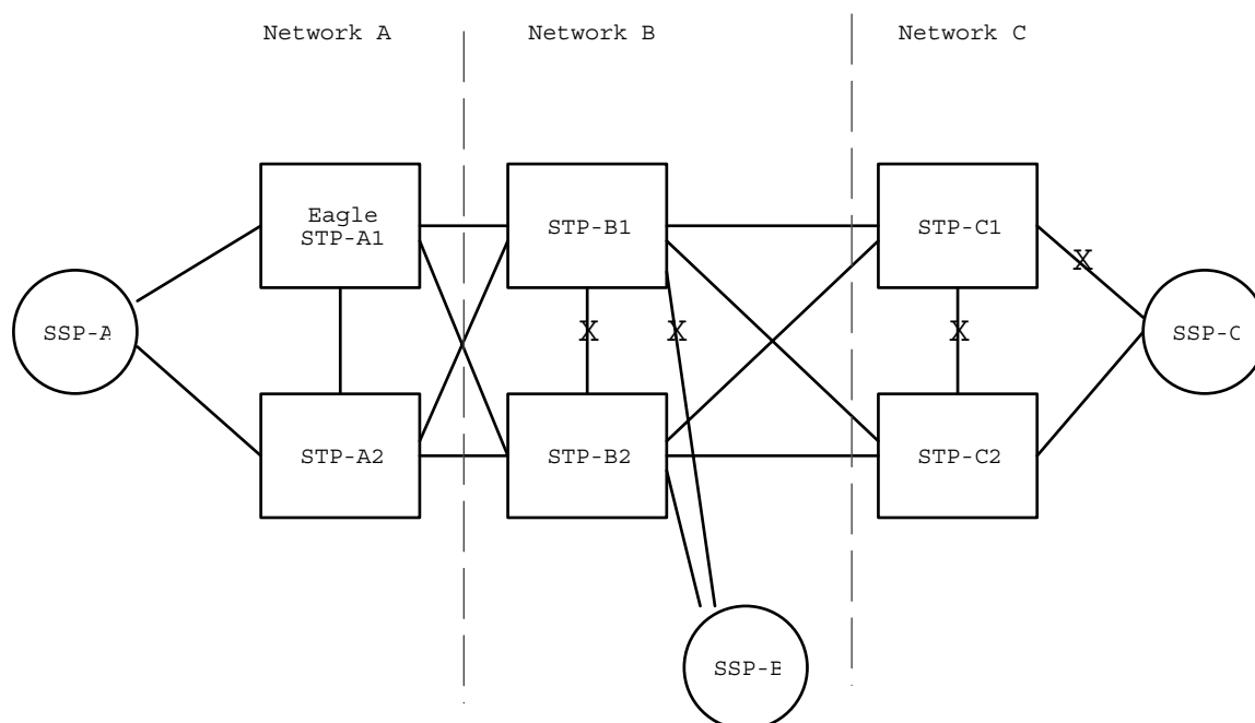
Figure 4-30. Example of Network Routing Reliability
