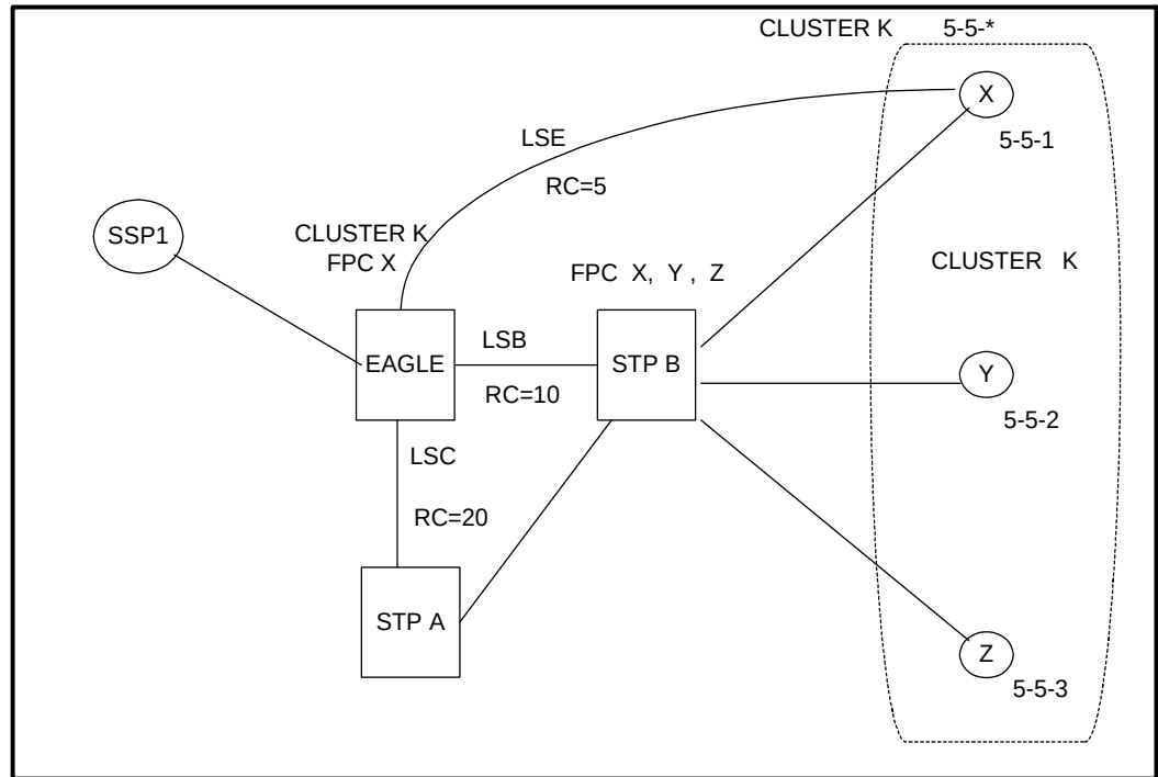
Figure 4-29. Nested Cluster Example #1
