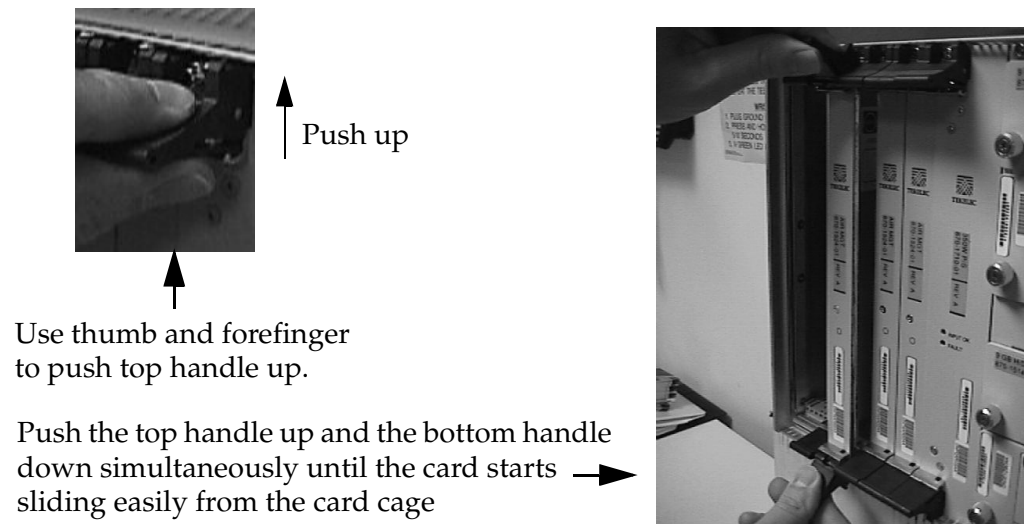
Figure 5-5. Freeing the Card from the EOAP Card Cage
