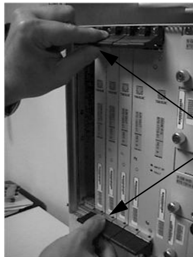
Figure 5-9. Lock the Inject/Eject Handles
