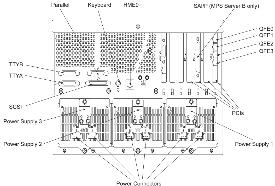
Figure 6-82. MPS Server Rear Detail
