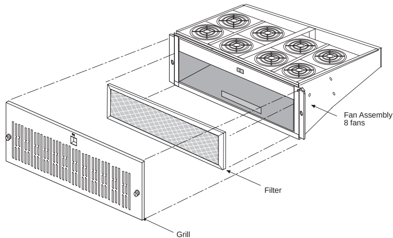
Figure 5-36. Remove Grill and Filter from Fan Assembly
