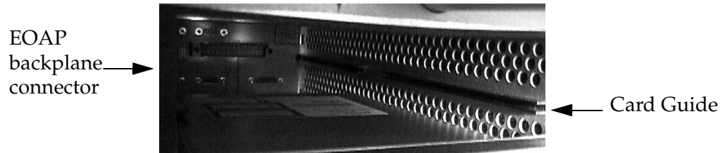
Figure 5-46. Examine EOAP Backplane Connector Pins
