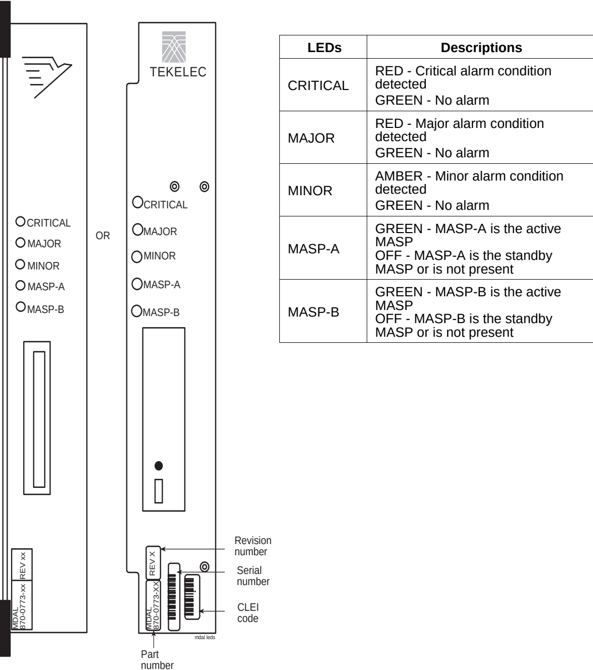
Figure A-1. MDAL LEDs
