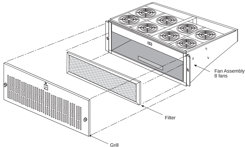
Figure 5-39. Replace Fan Filter and Grill
