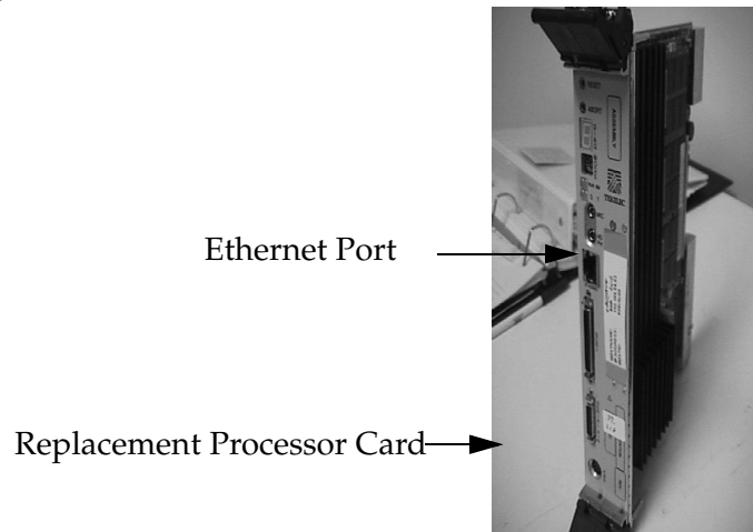
Figure 5-63. Processor Card (P/N 870-1523-01)
