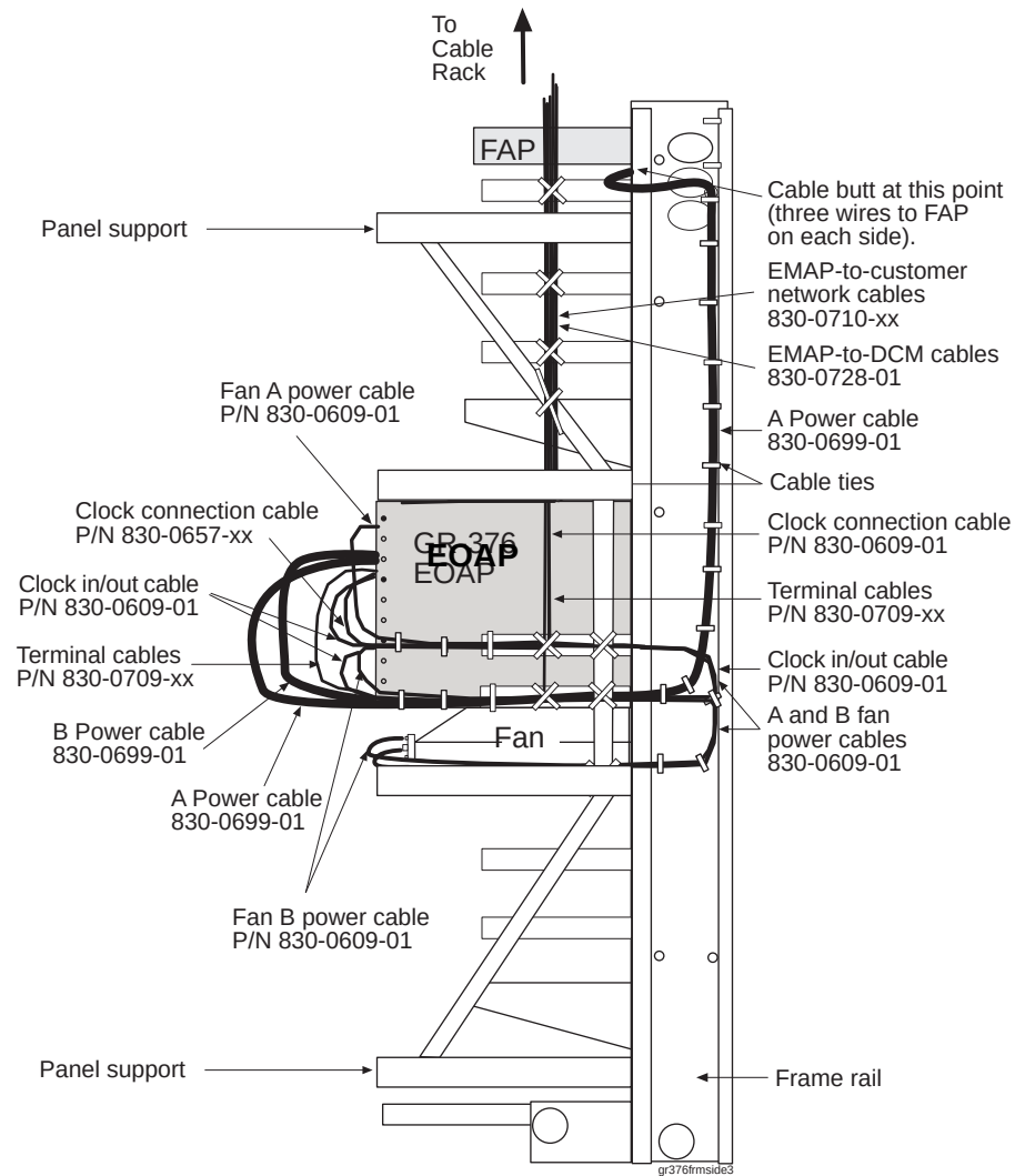
Figure 5-26. Secure Cables from EOAP to Cable Rack
