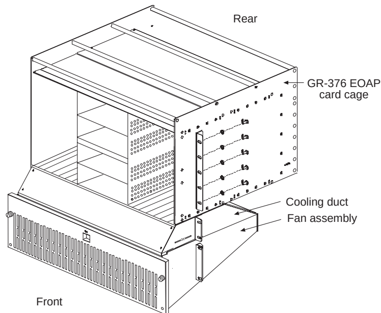
Figure 5-11. EOAP Card Cage
