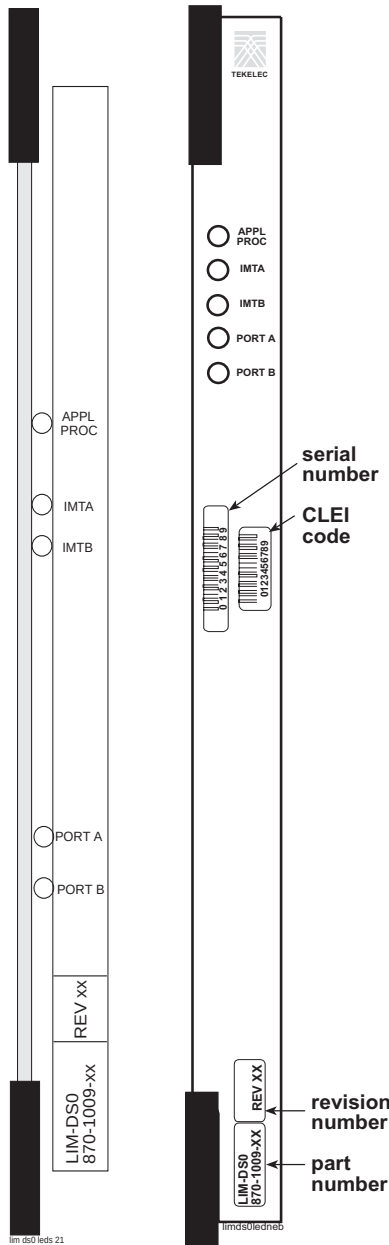
Figure A-6. DS0A-LIM LEDs
