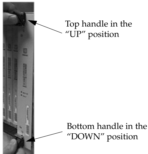
Figure 5-55. Power Supply Card Handles
