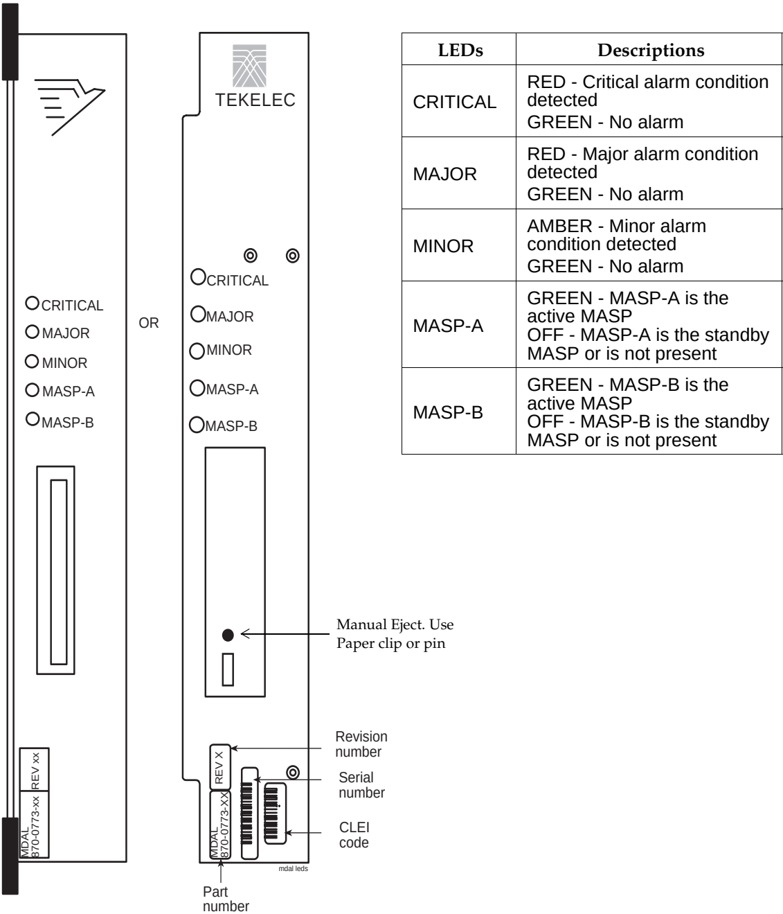
Figure 3-1. MDAL Alarm LEDs
