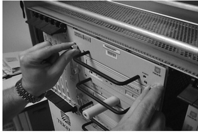
Figure 5-43. Loosen Hard Drive Card Captive Screws
