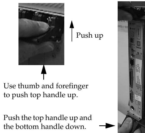
Figure 5-61. Freeing the Processor Card from the EOAP Card Cage
