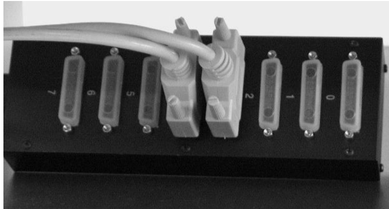
Figure 6-7. 8-Port Serial Connector Box
