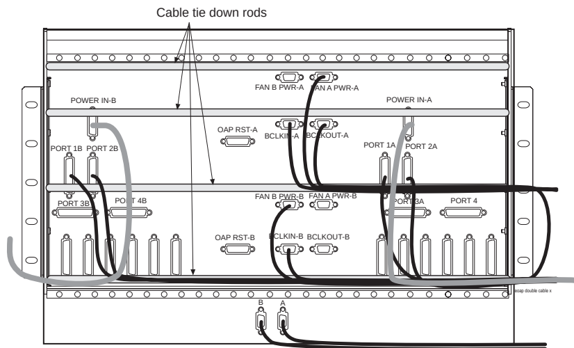
Figure 5-22. Locate Cables on EOAP Backplane (Single Configuration)
