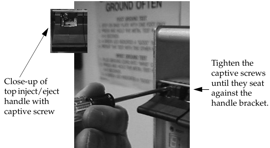
Figure 5-67. Tightening Captive Screws
