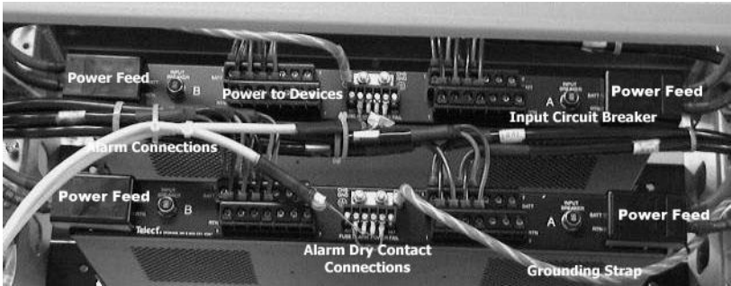
Figure 6-5. Rear of Breaker Panel
