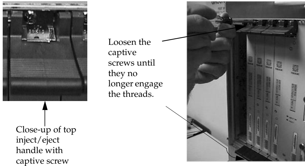
Figure 5-4. Top Handle and Captive Screw of Air Management Card
