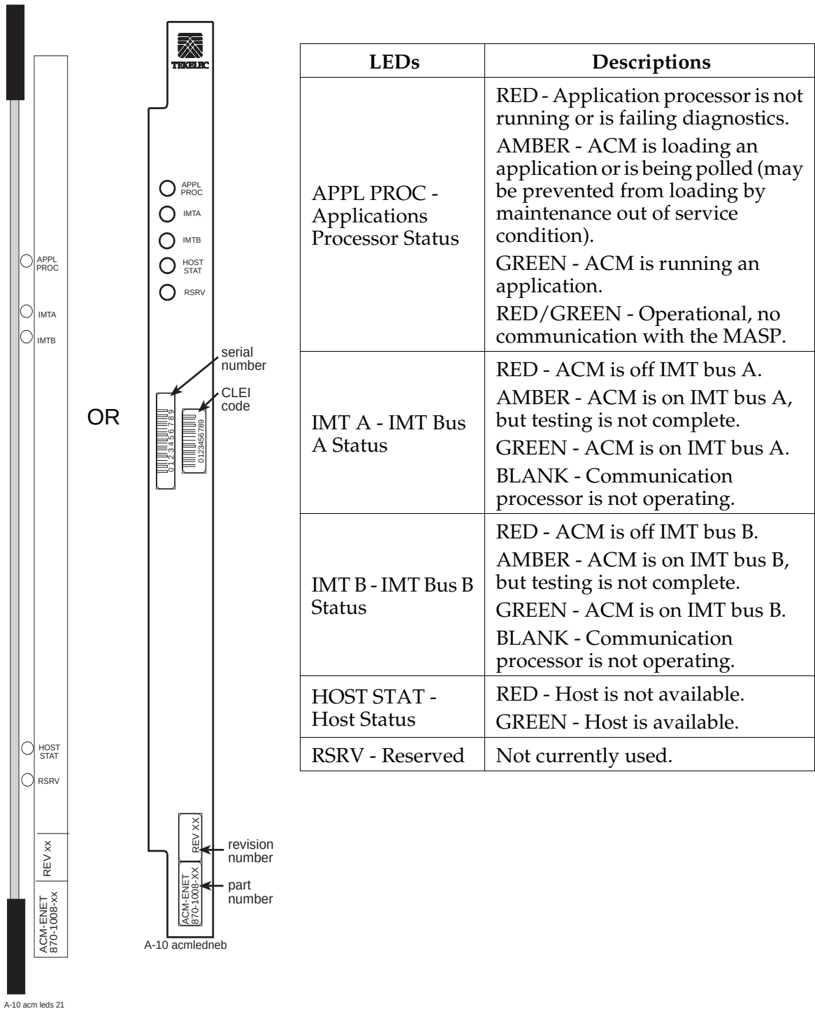
Figure A-12. ACM LEDs
