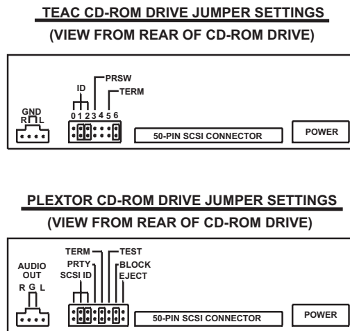
Figure 5-2. CD-ROM SCSI Jumper Settings
