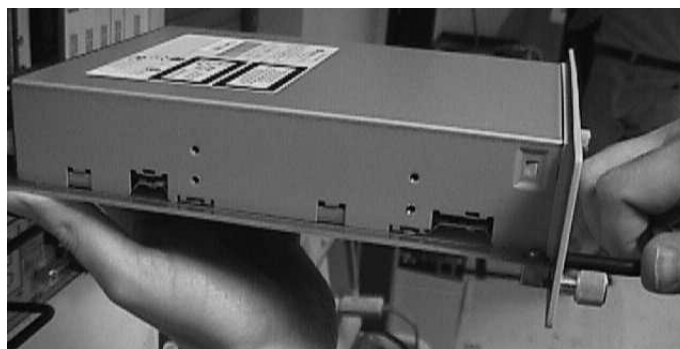
Figure 5-30. Support the CD-ROM Drive Card With Both Hands
