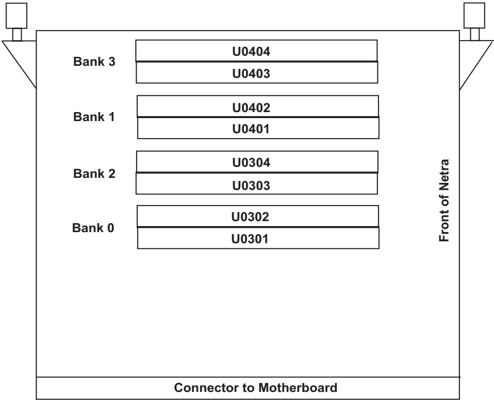
Figure 6-84. Memory Riser Card Memory Bank Layout
