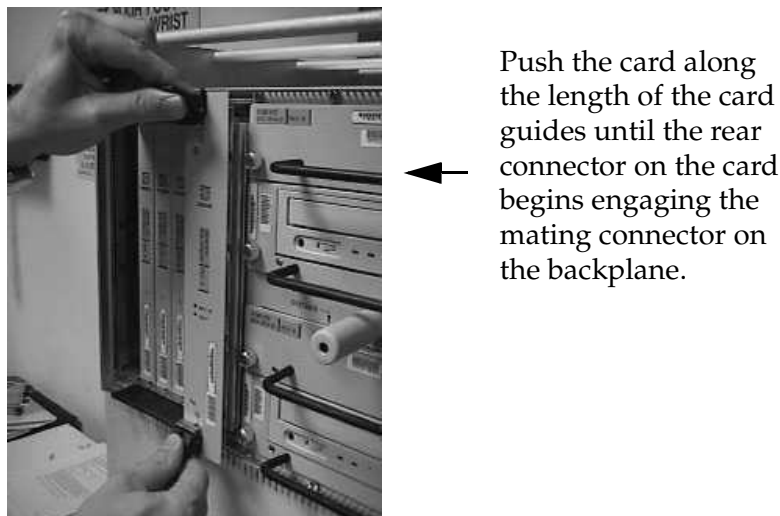
Figure 5-56. Inserting the Power Supply Card
