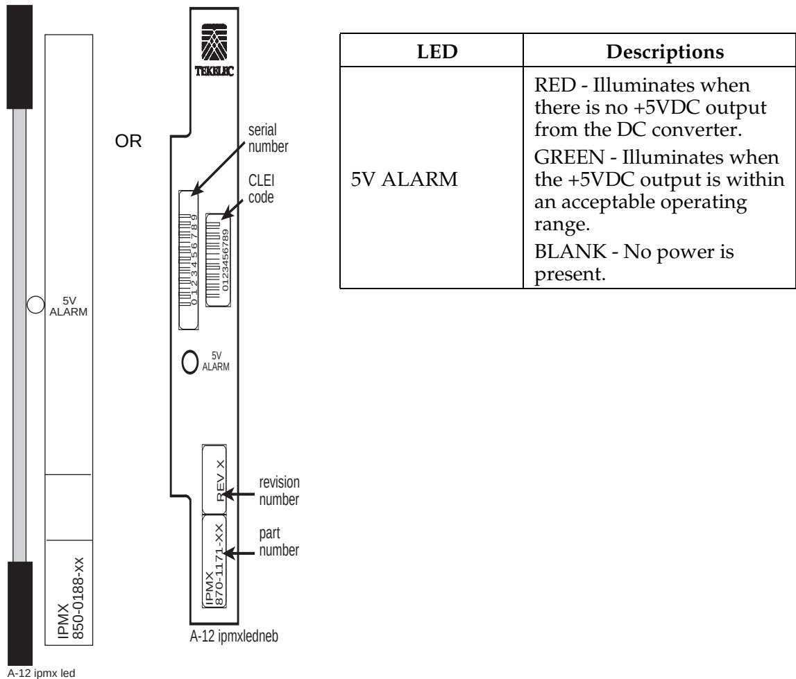
Figure A-4. IPMX LED
