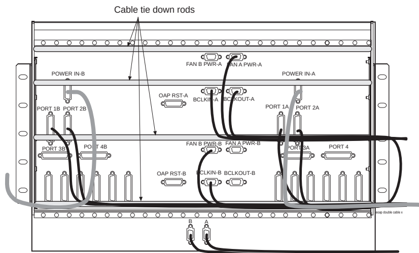
Figure 5-23. Locate Cables on EOAP Backplane (Dual Configuration)
