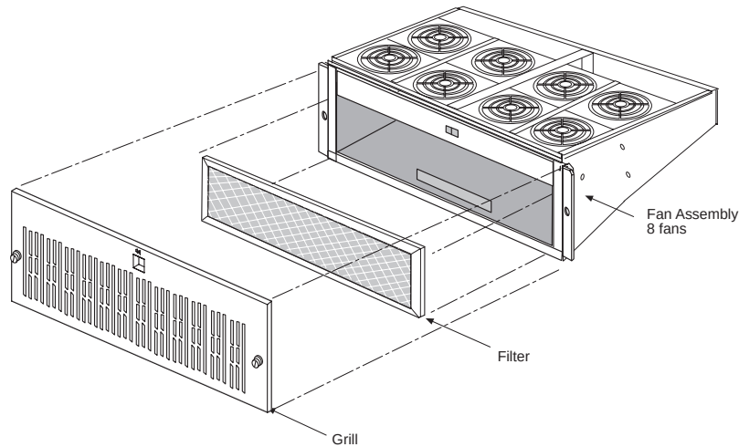
Figure A-29. Replace Fan Filter and Grill
