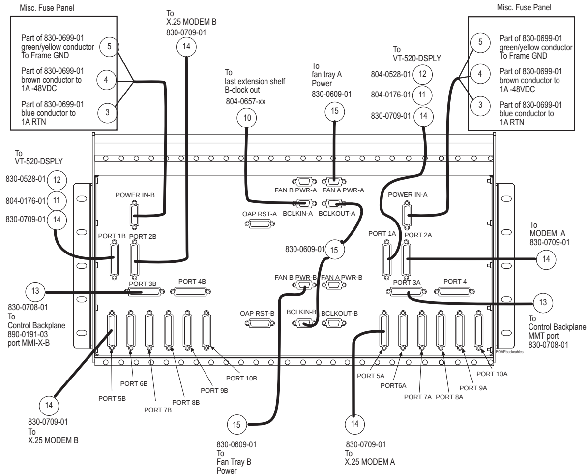
Figure 5-20. Cable Connections on EOAP Backplane (Dual Configuration)
