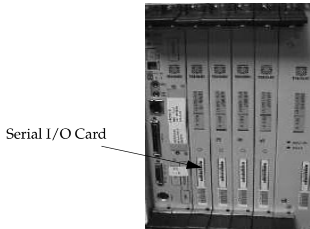
Figure 5-69. Location of Serial Card
