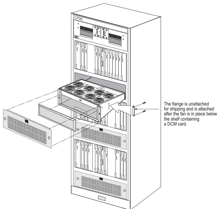
Figure A-26. Insert Fan Assembly Below DCM Card
