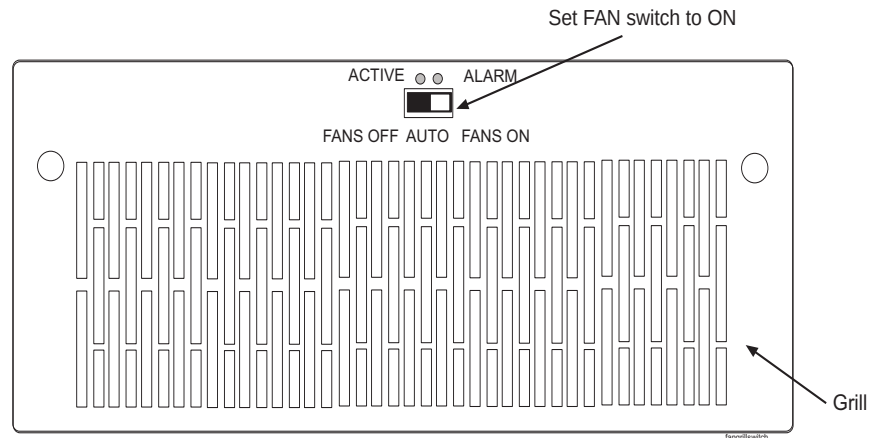
Figure A-30. Fan Switch Set to ON
