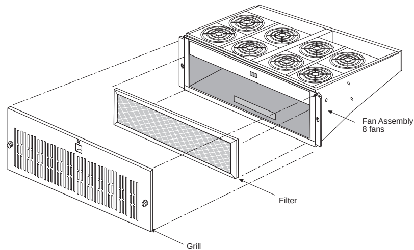
Figure A-25. Remove Grill and Filter from Fan Assembly
