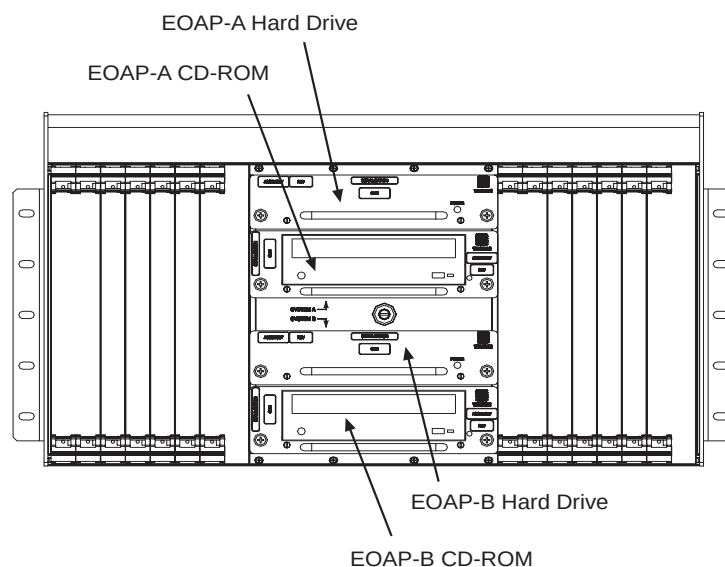
Figure 5-28. EOAP-A and EOAP-B Drive Assemblies
