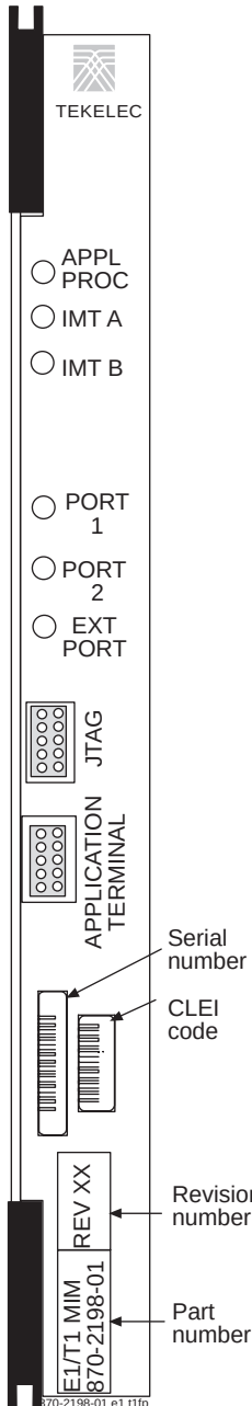
Figure A-8. E1/T1 MIM (P/N 870-2198-xx)
