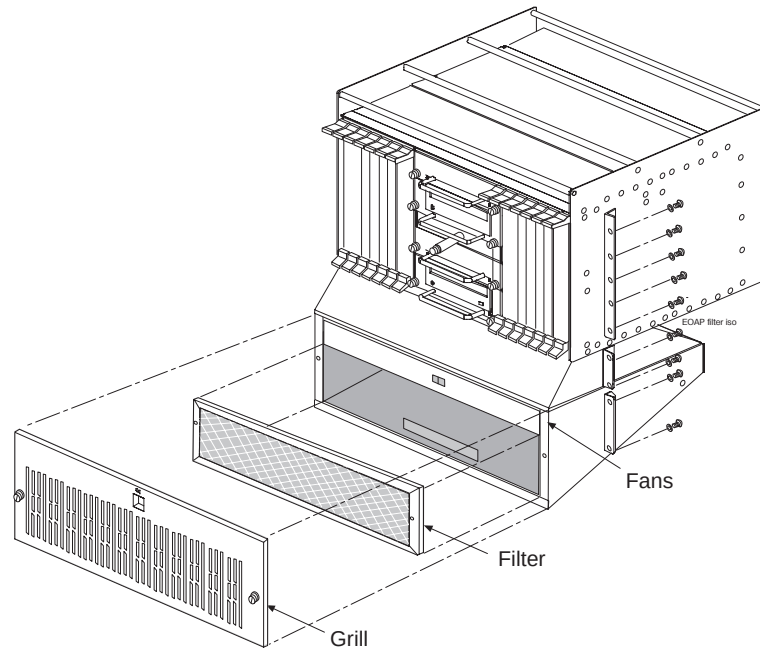
Figure 2-9. Fan Filter Replacement
