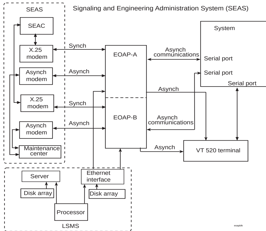
Figure 5-68. EOAP Serial and Ethernet Connections
