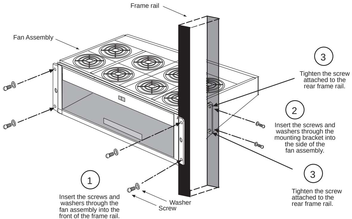
Figure A-28. Attach Fan Assembly to Front of Frame Rail
