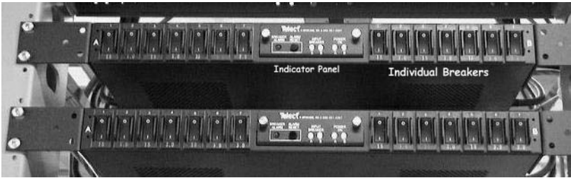
Figure 6-4. Front of Breaker Panel
