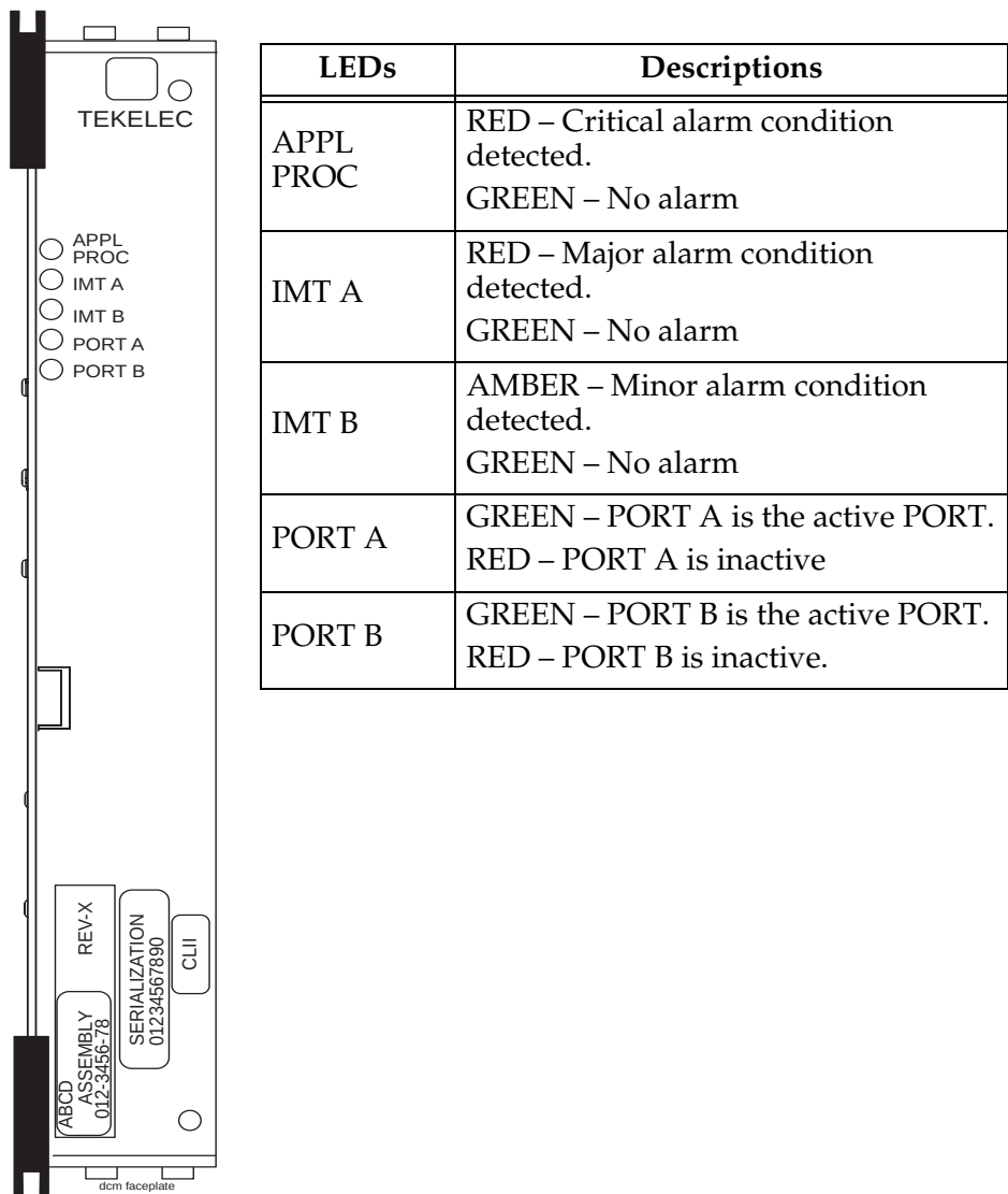
Figure A-13. DCM LEDs
