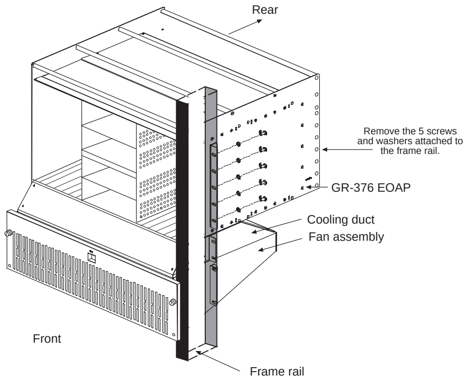
Figure 5-15. Remove Screws and Washers from Frame Rail
