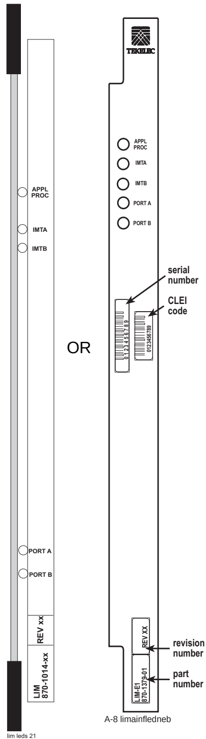
Figure 3-9. Card LEDs
