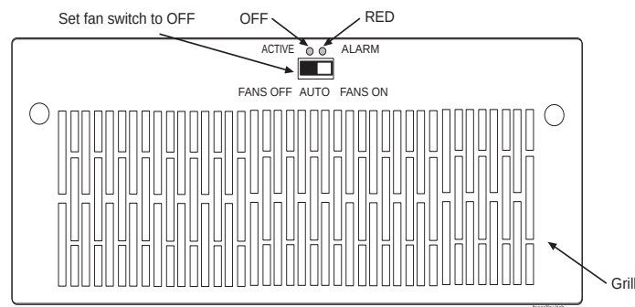
Figure 5-34. Set Fan Switch to OFF
