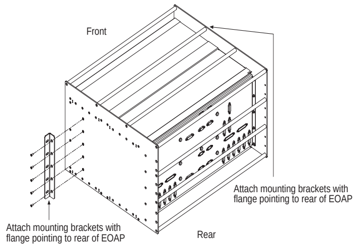
Figure 5-17. Attach Mounting Bracket to EOAP Card Cage
