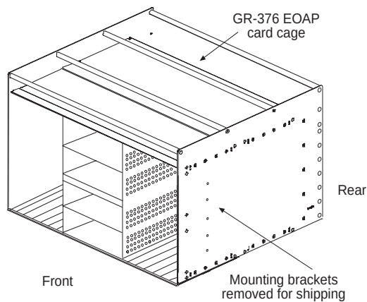
Figure 5-16. Locate Mounting Brackets for EOAP Card Cage
