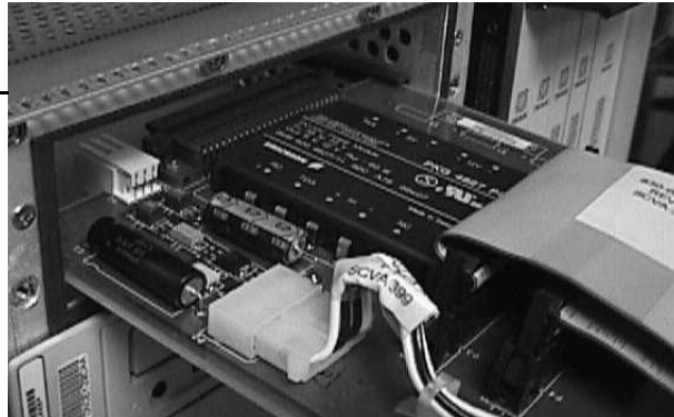
Figure 5-48. Installing the Hard Drive Card
