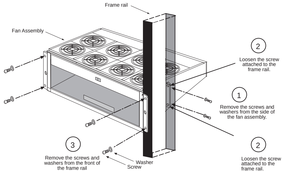
Figure 5-35. Remove Fan Assembly
