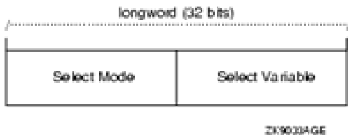
Figure 2-6 sel_filter argument
