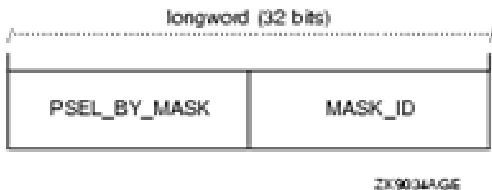
Figure 2-8 Compound Selection
