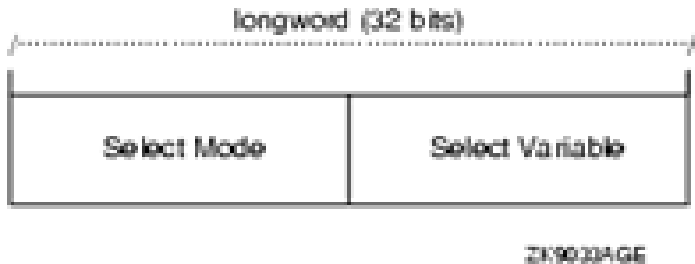
Figure 2-10 sel_filter argument
