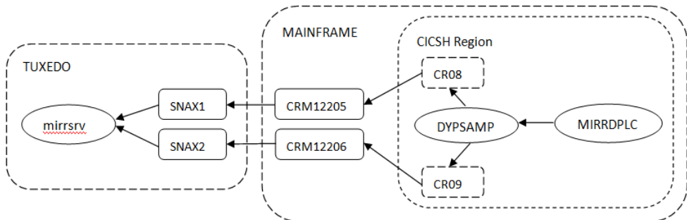
Figure 9-3 Inbound Call (from CICS to Oracle Tuxedo)
