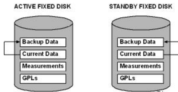
Figure 5-2. The chg-db:action=backup:dest=fixed Command
