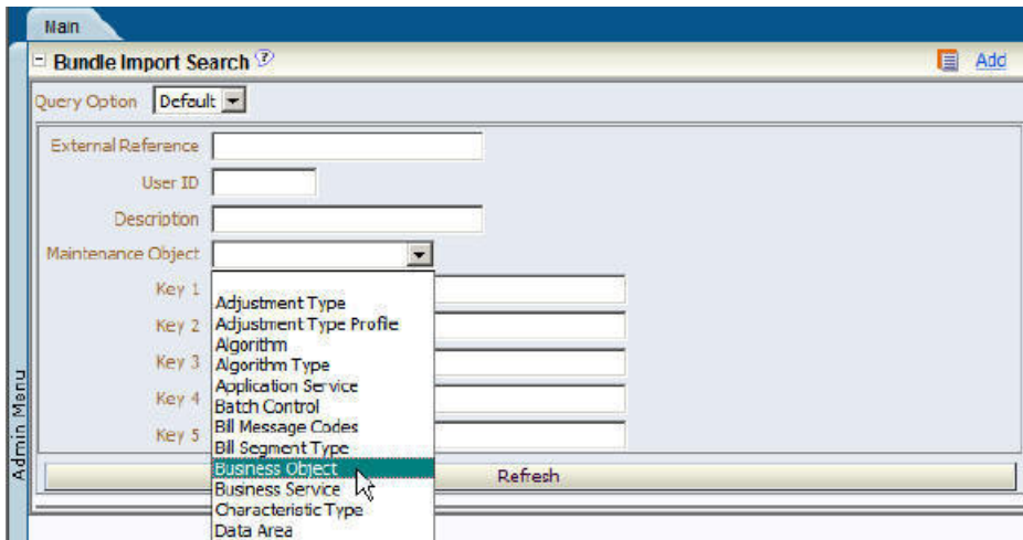
Figure 19: Multi-Query Zone
