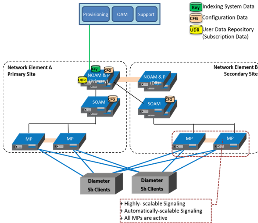
Figure 1: UDR System Architecture
