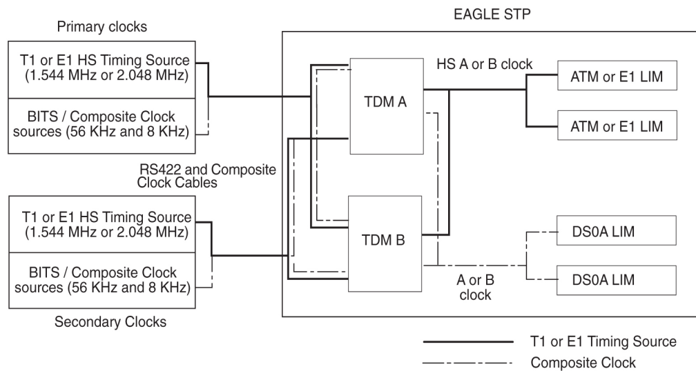
Figure 44: System Clocks
