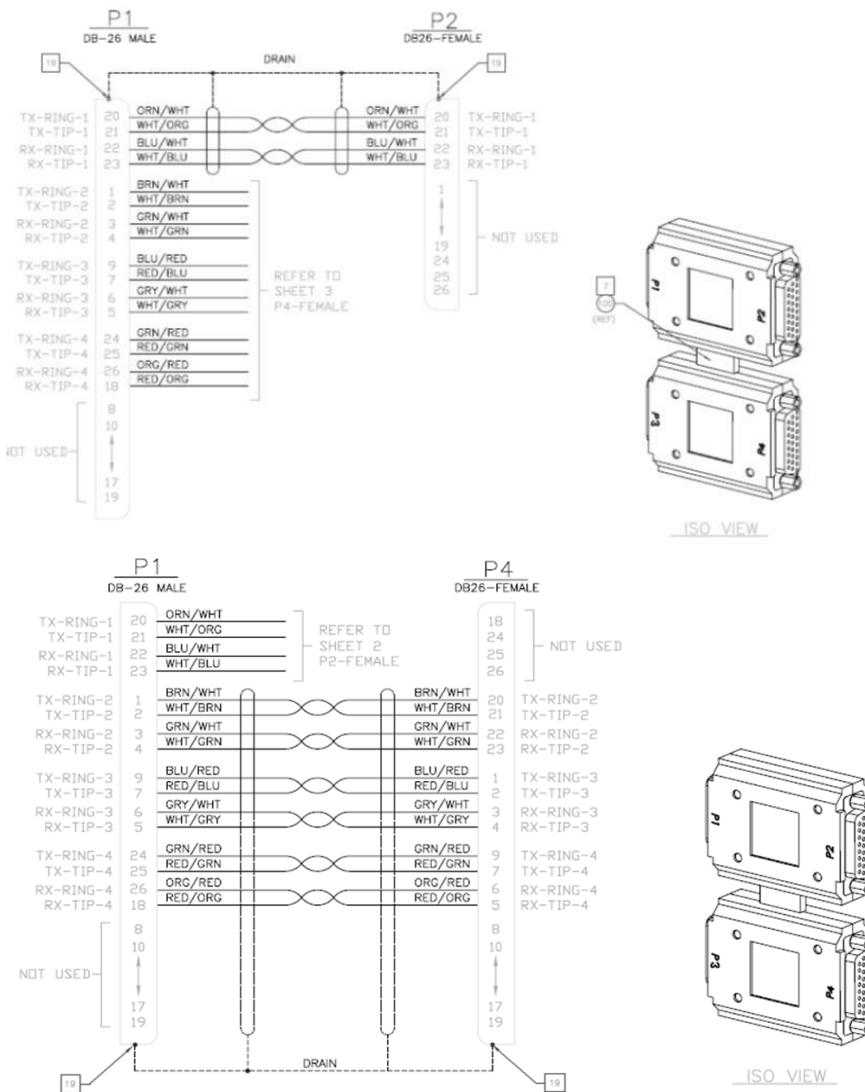
Figure 9 - 830-1342-05 ATM Adapter
