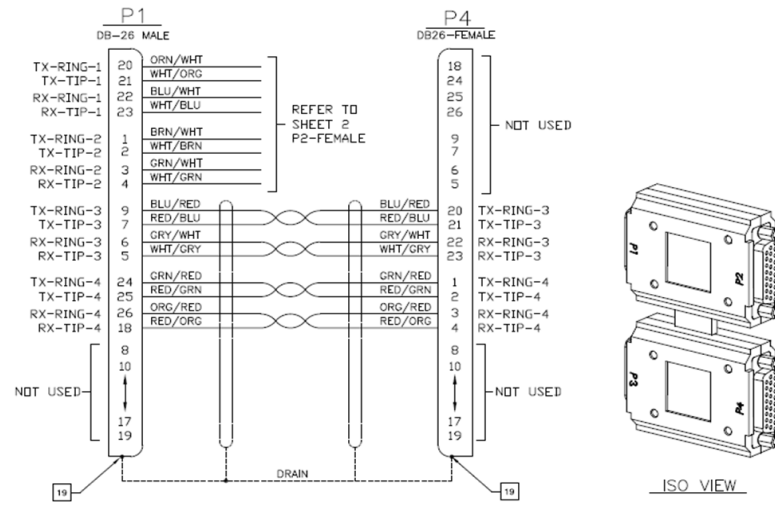
Figure 10 - 830-1342-06 ATM Adapter
