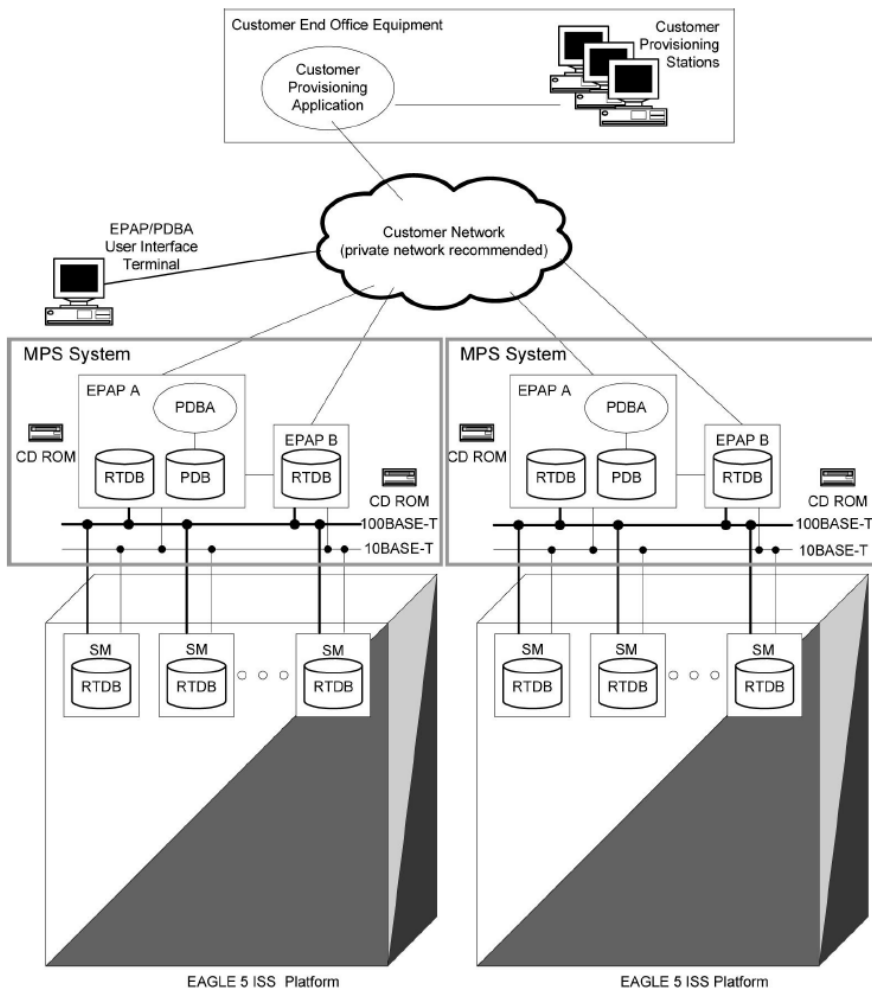
Figure 14 - EPAP Architecture
