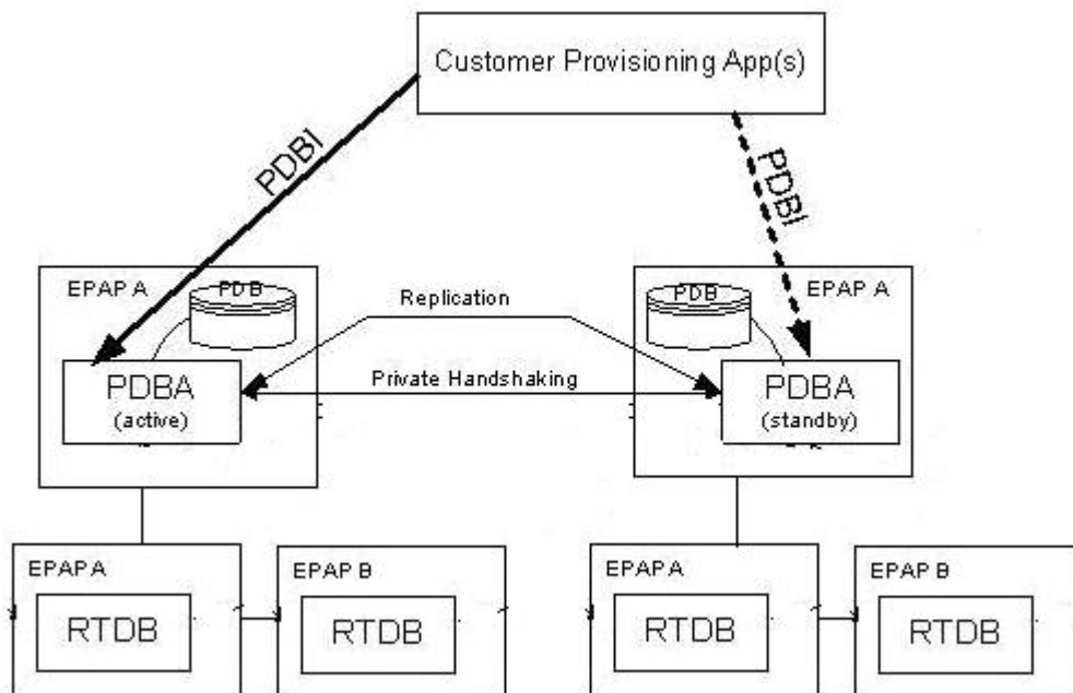
Figure 123: EPAP Standalone PDB Architecture
