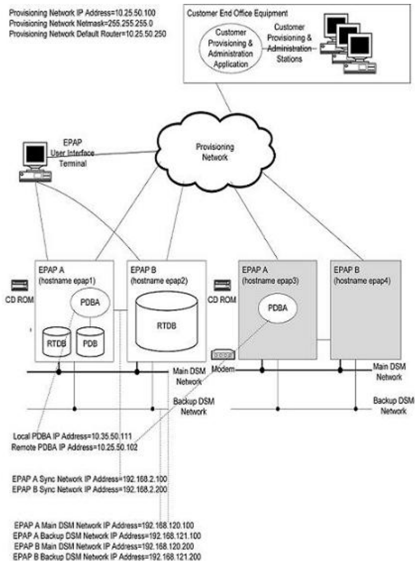
Figure 2: Example of EPAP Network IP Addresses
