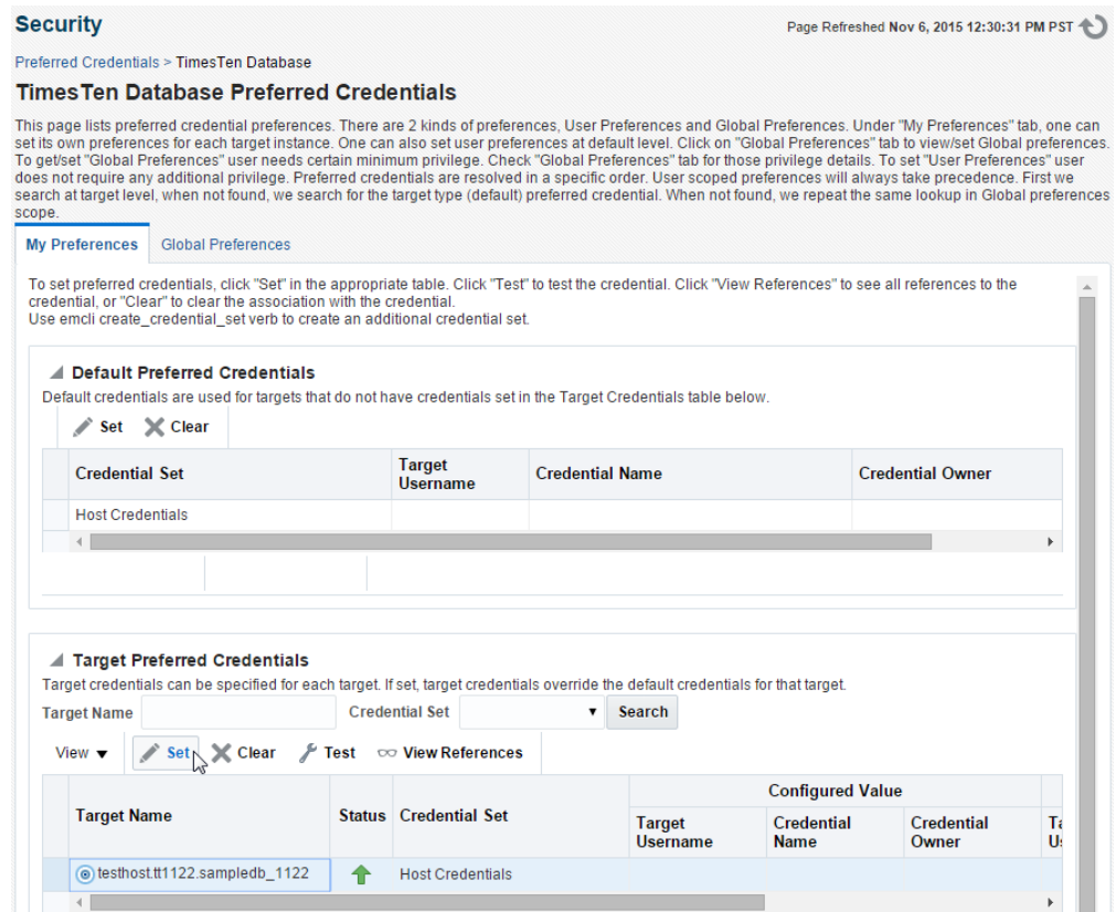
Figure 1–61 Click set
