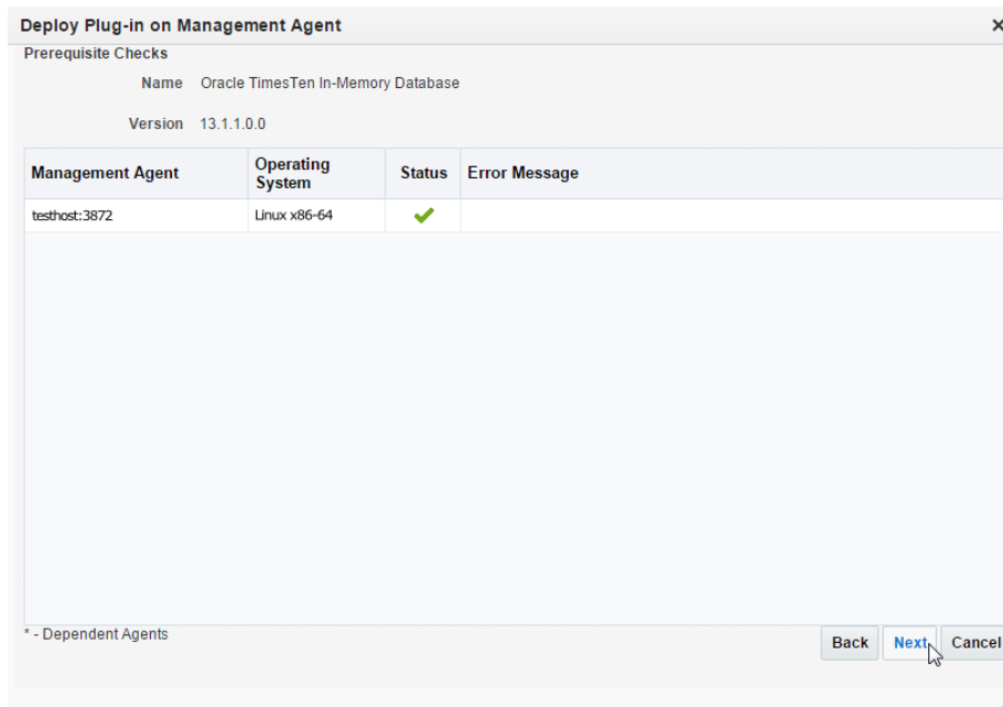
Figure 1–23 Prerequisite checks
