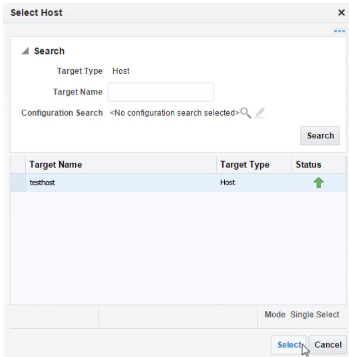
Figure 1–50 Select host
