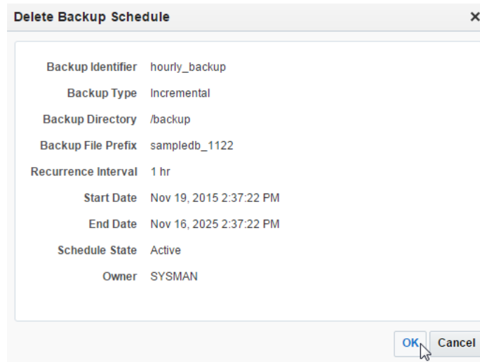
Figure 11–18 Click OK
