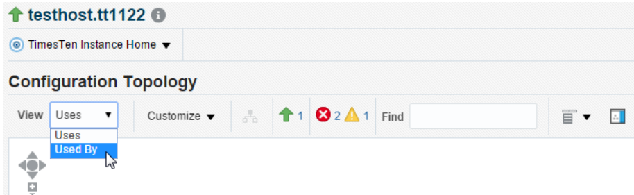
Figure 15–1 Select view
