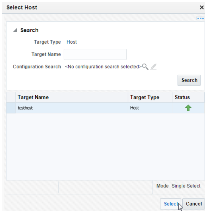
Figure 1–44 Select host
