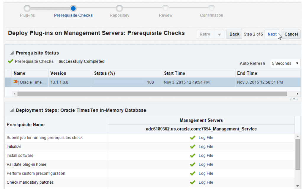
Figure 1–11 Click Next
