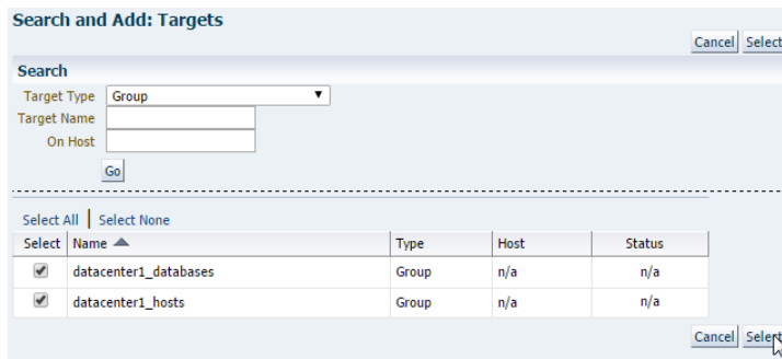
Figure 3–16 Click Select
