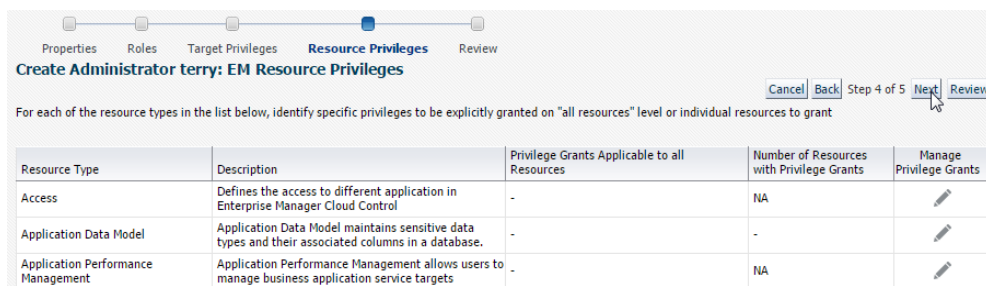
Figure 3–36 Click Next
