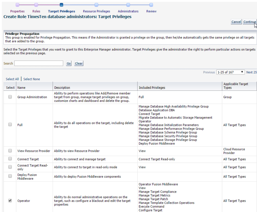
Figure 3–19 Click Continue
