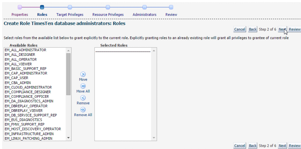
Figure 3–12 Click Next
