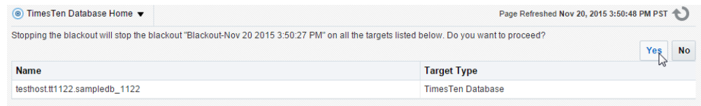
Figure 10–6 Click Yes
