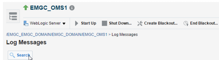
Figure 2–9 Click Search
