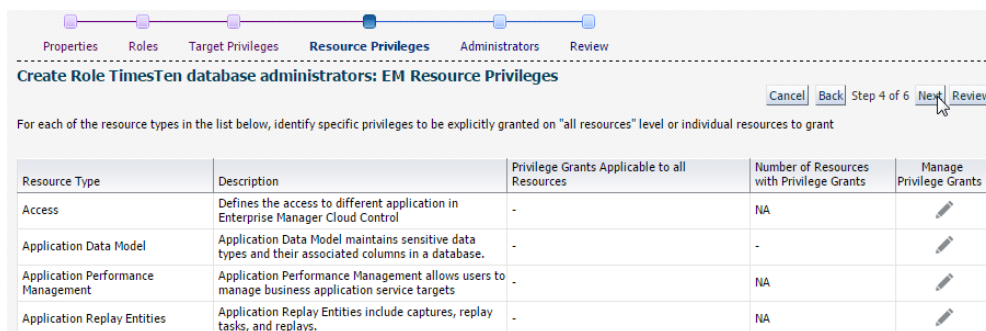
Figure 3–27 Click Next
