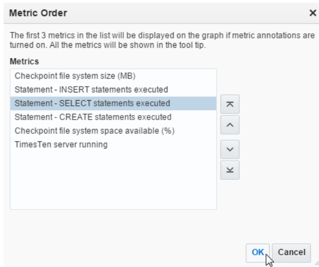
Figure 15–7 Click OK
