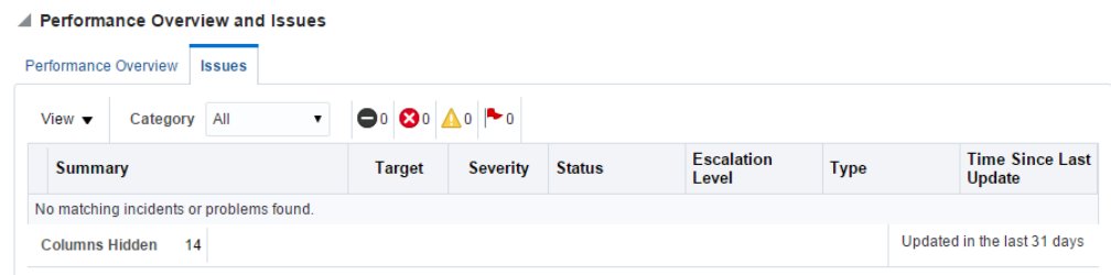
Figure 5–7 Issues region
