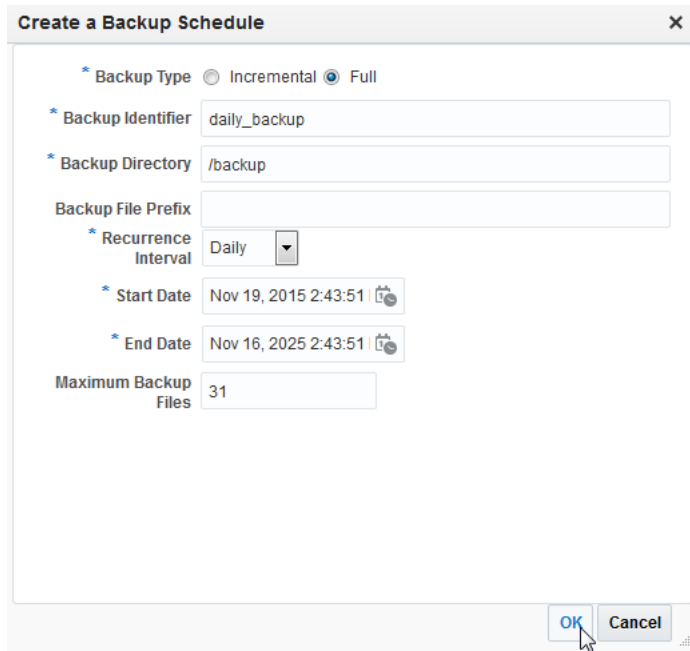
Figure 11–6 Click OK
