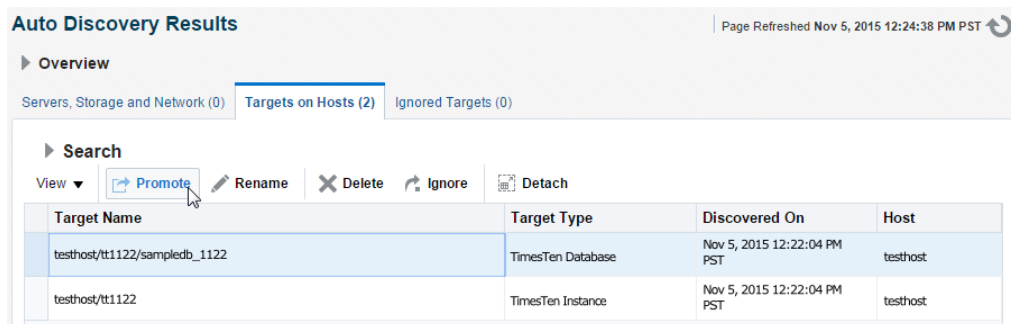
Figure 1–39 Promote target
