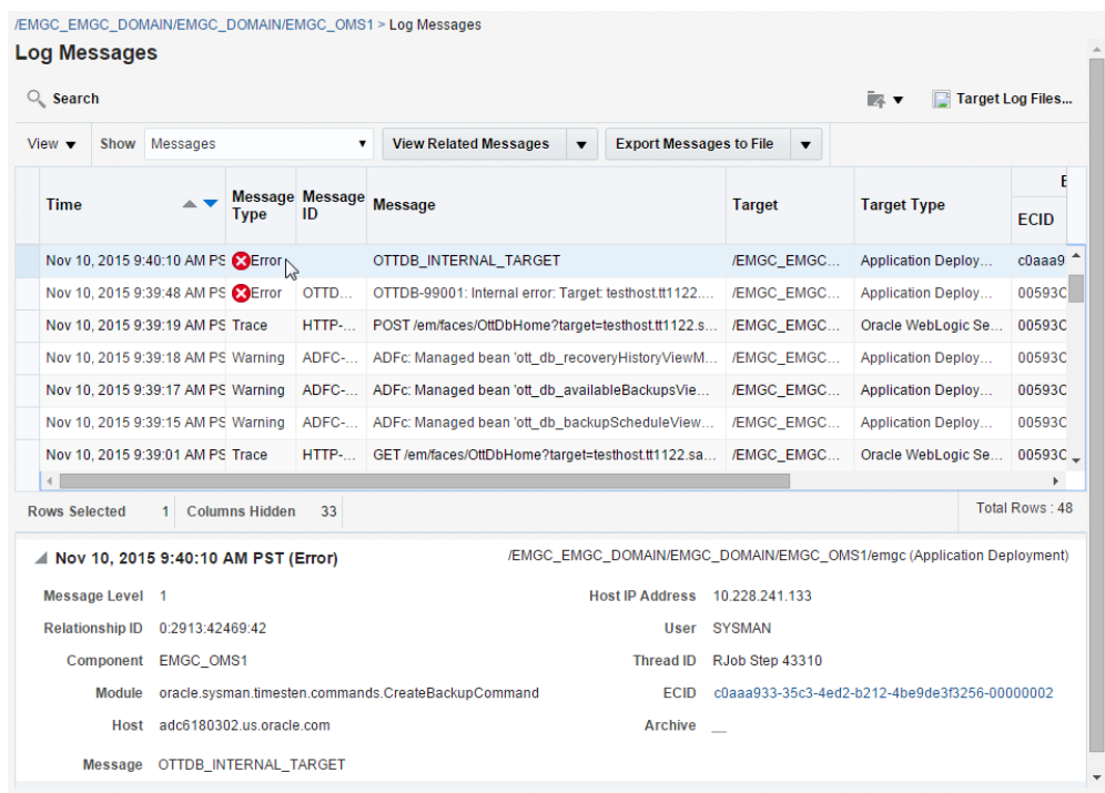
Figure 2–11 Search results
