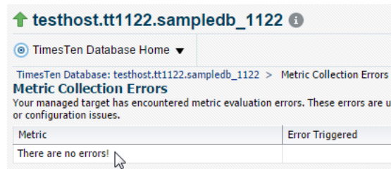
Figure 1–57 No errors
