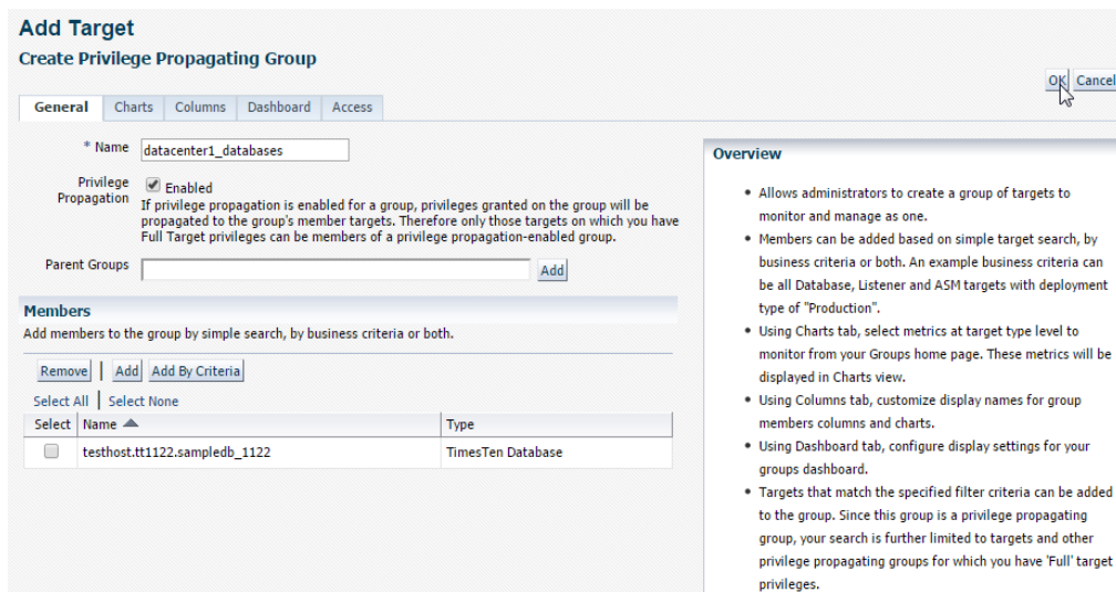
Figure 3–8 Click OK
