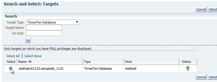
Figure 3–6 Select target
