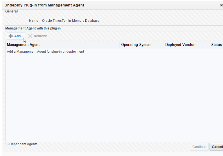
Figure 1–75 Click Add
