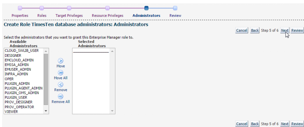
Figure 3–28 Click Next
