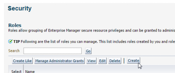
Figure 3–10 Click Create
