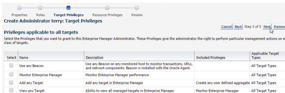
Figure 3–35 Click Next
