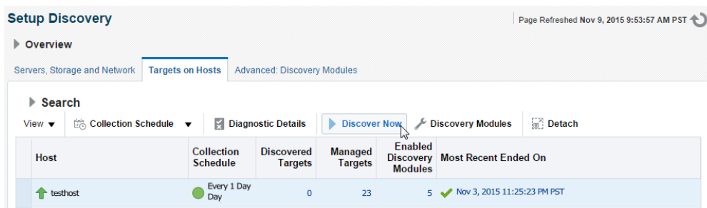
Figure 1–31 Discover Now
