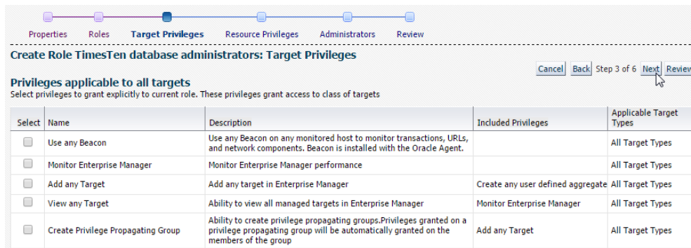
Figure 3–23 Click Next
