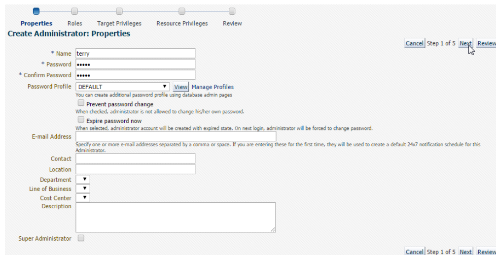
Figure 3–32 Click Next
