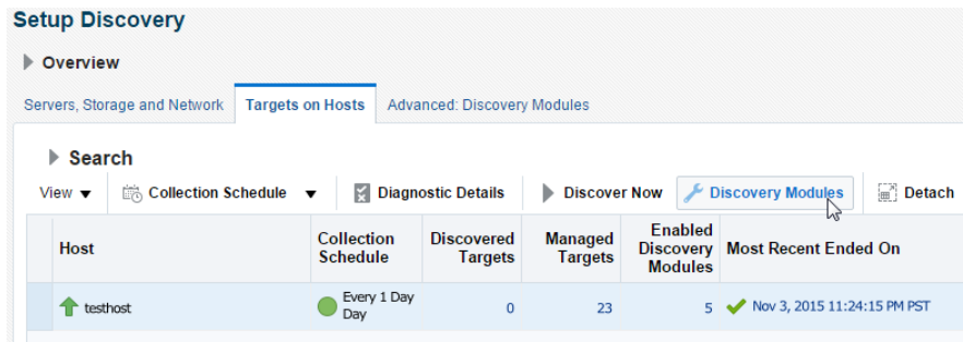
Figure 1–29 Add host
