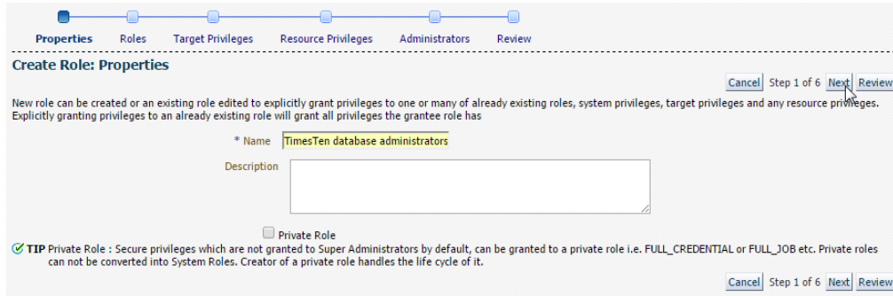
Figure 3–11 Click Next
