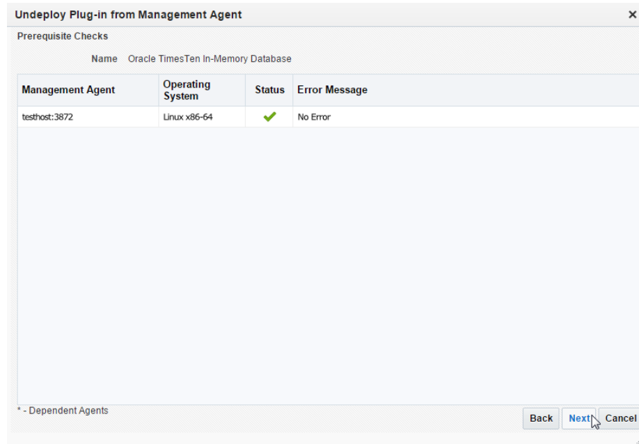
Figure 1–78 Click Next
