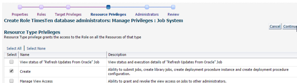
Figure 3–26 Click Continue
