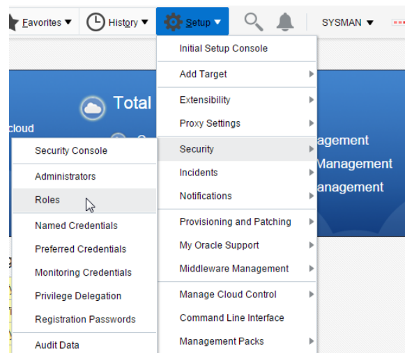
Figure 3–9 Select Roles
