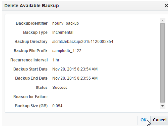
Figure 11–25 Click OK
