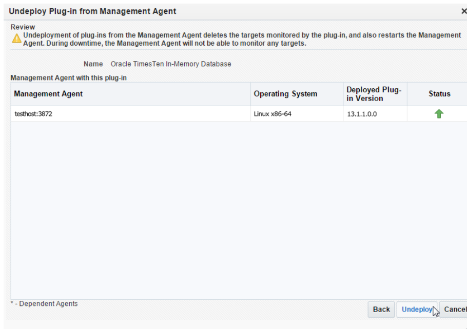
Figure 1–79 Click Undeploy
