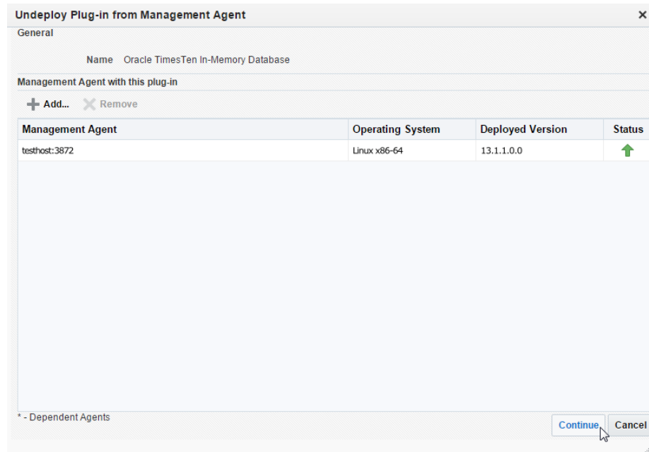
Figure 1–77 Click Continue
