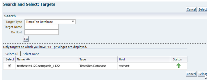
Figure 3–7 Click Select
