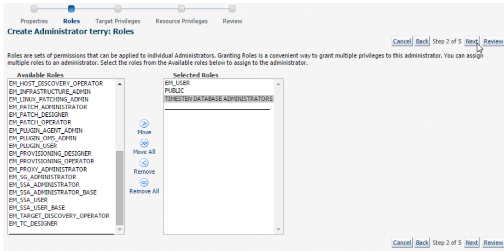
Figure 3–34 Click Next
