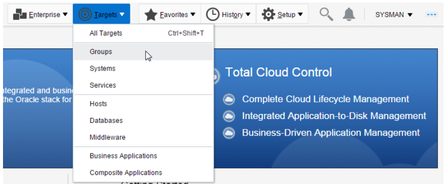
Figure 3–1 Select Groups
