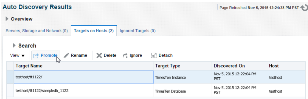
Figure 1–35 Promote target
