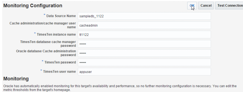
Figure 1–67 Click OK
