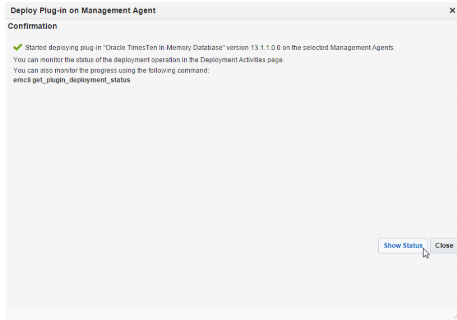
Figure 1–25 Confirmation dialog
