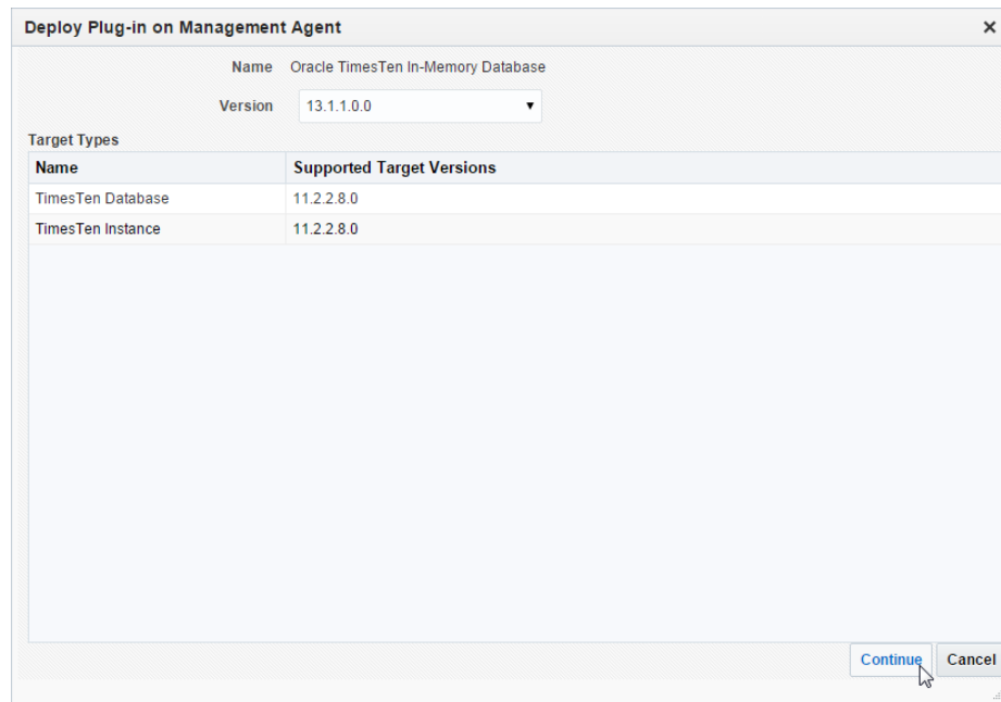
Figure 1–21 Click Continue
