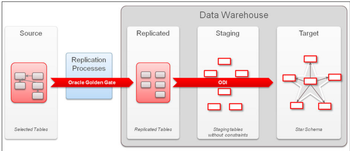
Data Flow
