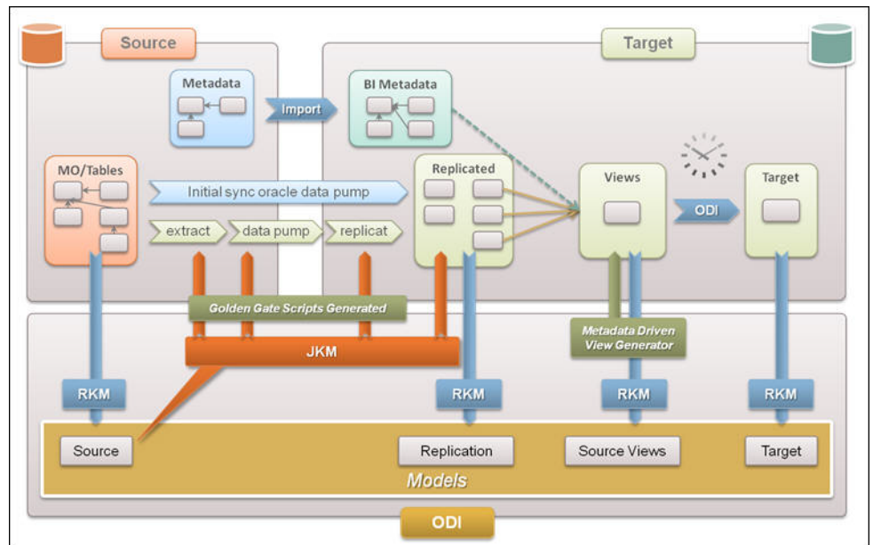
ELT Architecture
