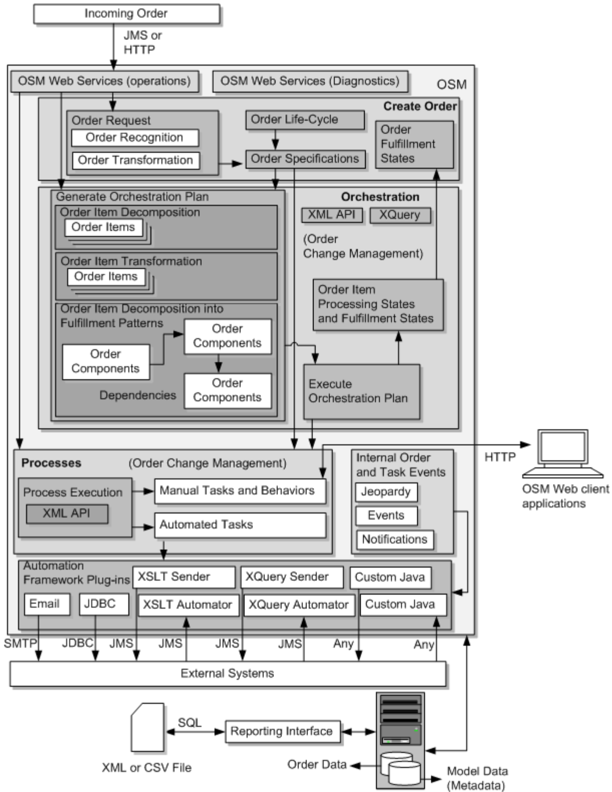
Figure 9-1 shows the three primary stages in order management: create the order, generate and execute an orchestration plan, and run processes and tasks.
