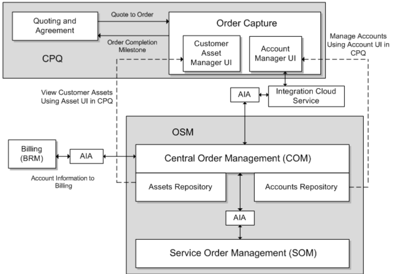
Figure 7-1 Order Flow Using Customer Asset Manager and Account Manager
