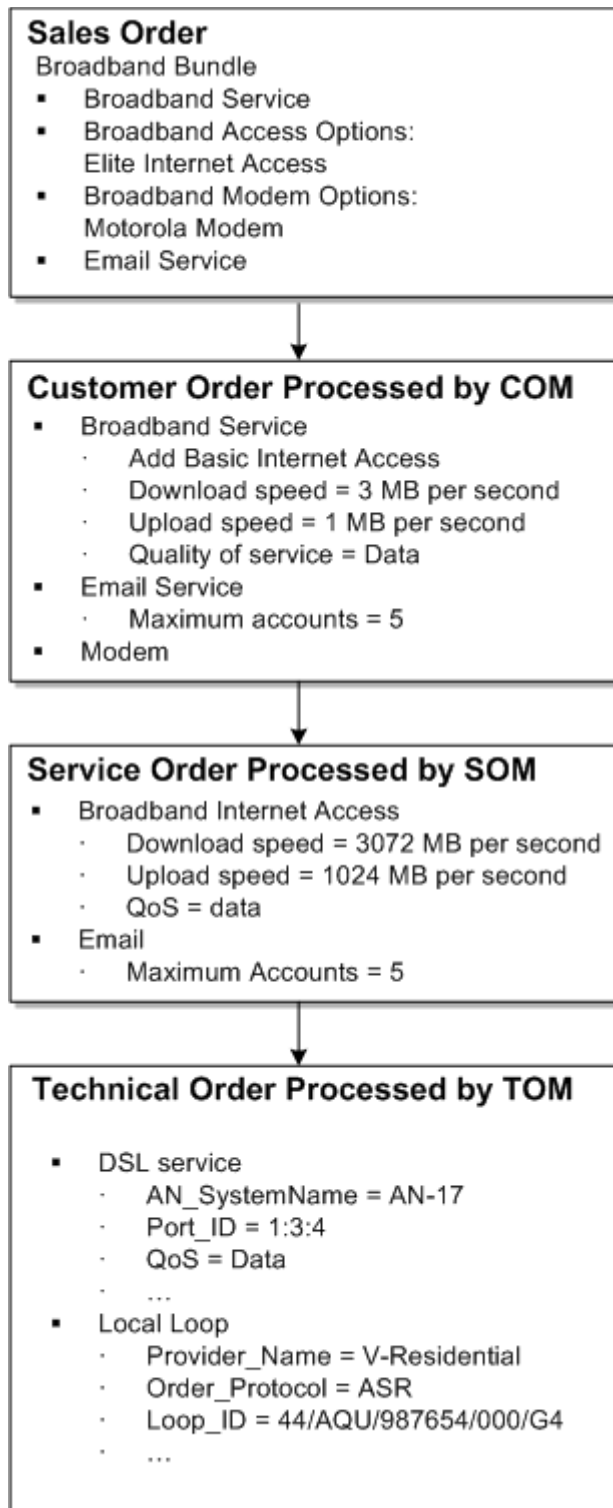
Figure 4-7 Order Items in COM, SOM, and TOM
